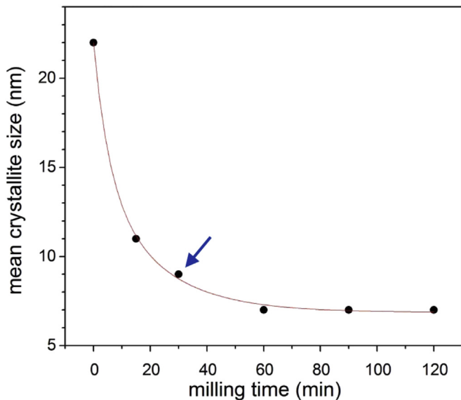
Fig. 2. Crystallite size of the system \text{LaNi}_5 -type at different milling times.
