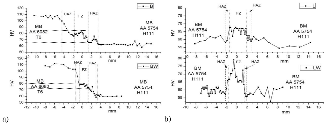
Fig. 5: Micro hardness Vickers evaluated through the cross-sections of the butt joints (a) and the lap joints (b)
