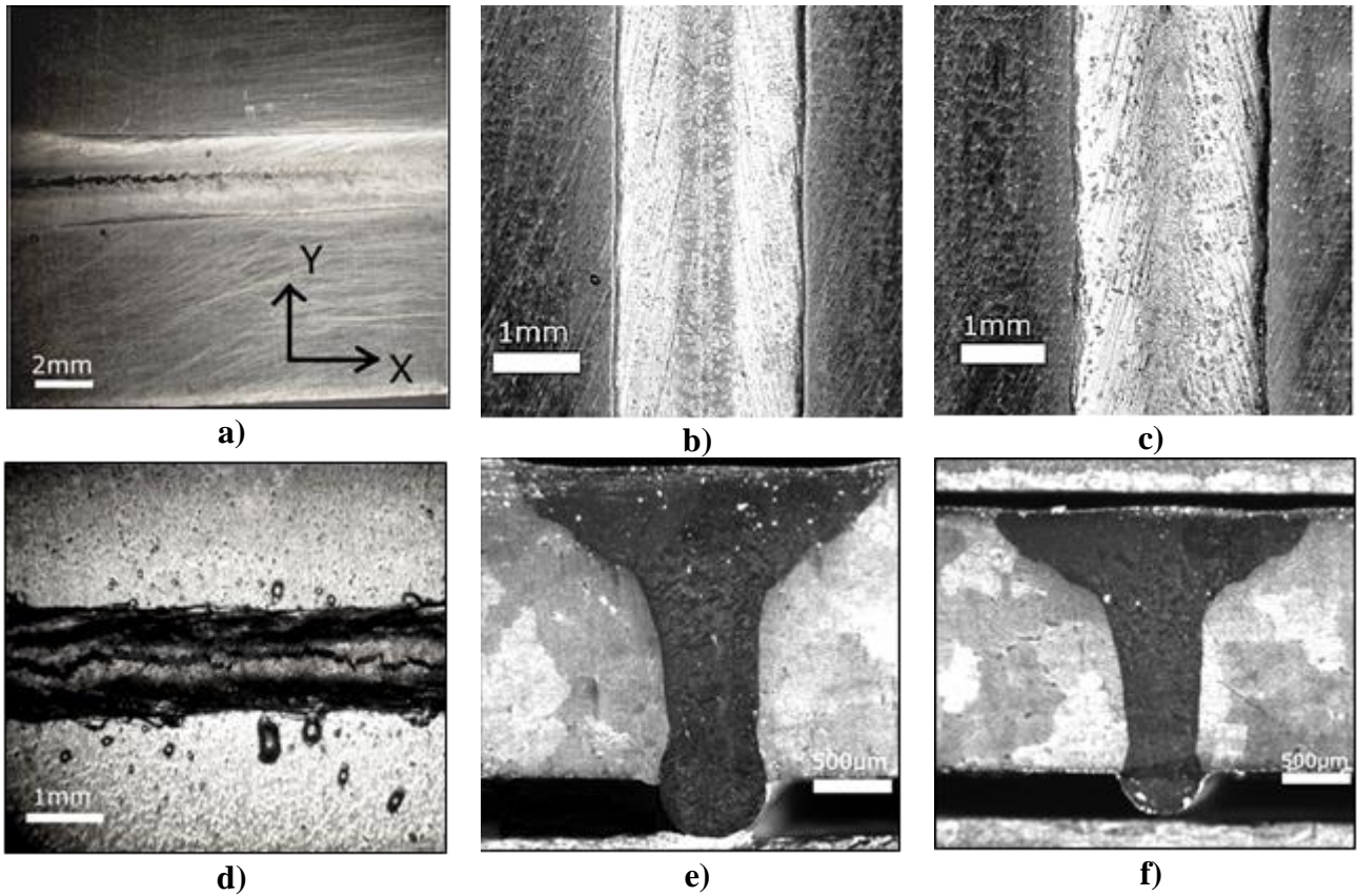
Fig. 2- Seams of the samples EB welded with pre-heating at 200 °C: pass speed of 1.0 m/min (a-d), 1.5 m/min (b-e) and 2.0 m/min (c-f). The image in d) is the opposite side of a). Cross-sections of the seams displayed in b) and c) are shown in e) and f), respectively.
