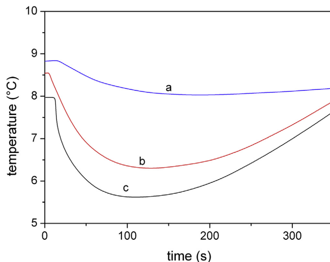
Fig. 14. Cooling effect of the Metal Hydride Cooling System during the active refrigerating phase. The curve a represents the temperature values measured inside the refrigerated van in function of the time. The curves b and c represent the temperature values as measured for the inlet and outlet cooling water circulating into the internal heat exchanger placed inside the refrigerated.
