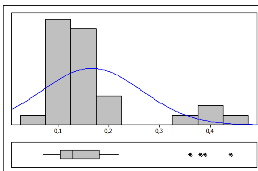
Ratio between the CAS's electricity consumption and the produced compressed air (cross-sectorial).
