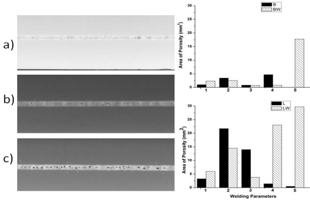
Fig.2: Digital radiography results: (left) samples a),b),c) with increasing porosity; (right) influence of the welding parameters on the cumulative area (mm 2 ) of porosity in 100 mm length welds for butt joints (up) and lap joints (down).
