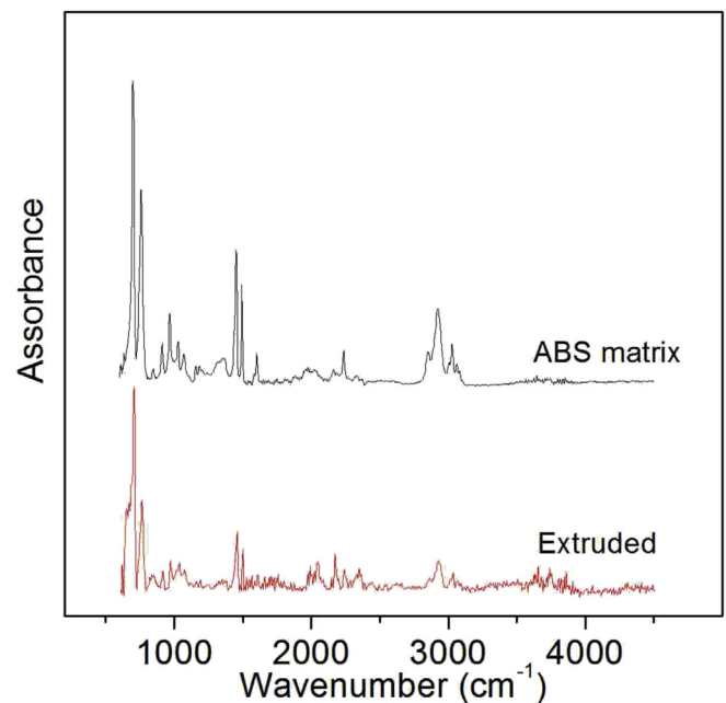
Fig. 7. Comparison of infrared spectra obtained in ATR mode of the extruded composite and pure ABS copolymer. The signals are typical from ABS and can be respectively assigned to: 650\text{--}800\text{ cm}^{-1} C-H aromatic bending out plane; 730\text{--}665\text{ cm}^{-1} C-H bending alkene; 1000\text{--}1300\text{ cm}^{-1} C-H aromatic bending out plane; 1400\text{--}1600\text{ cm}^{-1} C-C aromatic ring stretching; 1661\text{ cm}^{-1} C=C stretching alkene; 2230\text{ cm}^{-1} stretching nitrile; 2300\text{ cm}^{-1} \text{CO}_2 asymmetric stretching; 2300\text{--}2900\text{ cm}^{-1} C-H stretching of the alkene; 3000\text{--}3100\text{ cm}^{-1} C-H aromatic stretching.
