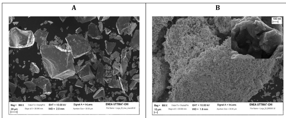
Fig. 3. Scanning Electron Microscopy images of \text{LaNi}_5 -type alloy as received (A) and milled for 30 min (B).
