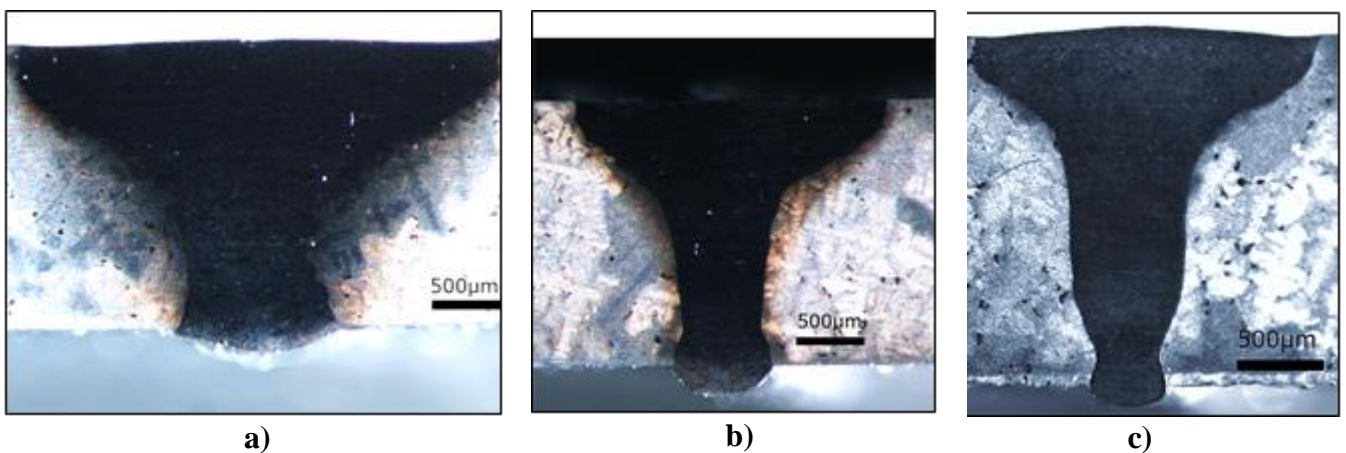
Fig. 3- Cross-sections of the seams obtained by EB welding with pre-heating at 300 °C: pass speed of 1.5 m/min (a), 2.0 m/min (b) and 2.5 m/min (c).
