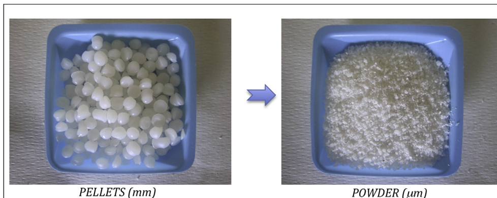
Fig. 4. The Acrylonitrile Butadiene Styrene copolymer in form of commercial pellets and as reduced in powder by means of centrifugal milling after material embrittlement in liquid nitrogen.
