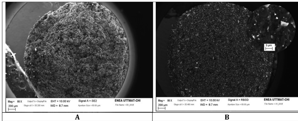
Fig. 8. Scanning Electron Microscopy analyses of the extruded metal hydride-polymer composite. The images refer to transversal sections of the extruded cylindrical pellets.
