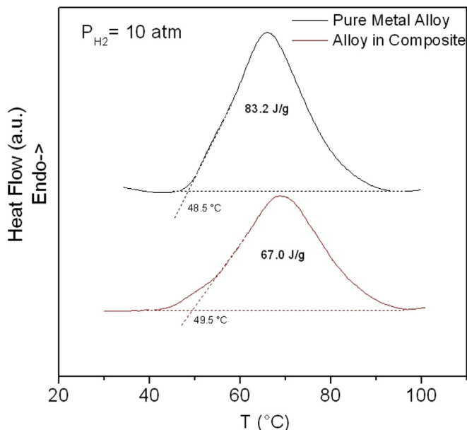
Fig. 9. Differential Scanning Calorimetry traces of obtained at 10 atm H 2 pressure for the extruded metal hydride-polymer composite in comparison with that one obtained for the pristine pure LaNi 5 -type metal hydride. Data are relative to the dehydriding process.
