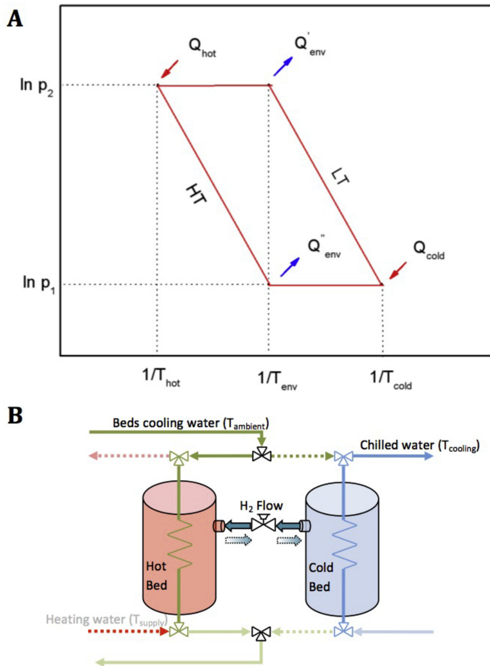
Fig. 11. (A) Schematic thermodynamic cycle of the single stage/single effect configuration as represented in the van't Hoff plane; (B) Conceptual layout of a single stage MHCS in cooling mode. The system comprises a pair of reactors, the hot bed (HB) containing a high temperature hydride (HT) and the cold bed (CB) containing a low temperature hydride (LT). Two energy streams are fed to the cycle, one at high temperature ( Q_{hot} at T_{hot} , coming from the source heat that is at T_{supply} \geq T_{hot} ), and one at low temperature ( Q_{cold} at T_{cold} , which is the energy stream removed from the area to be cooled down at T_{ref} \geq T_{cold} ). Removed heat is expelled toward the external environment, characterized by the third thermal level, T_{env} .
