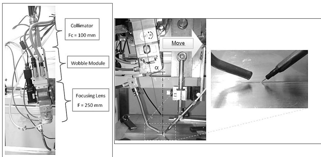
Fig.1, welding head constituted by a collimator, a wobble module and a focusing lens (left); welding set up (right).
