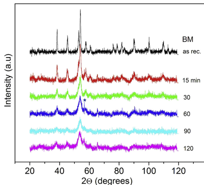
Fig. 1. X-ray diffraction pattern sequence of LaNi_5 -type alloy as a function of different milling times.
