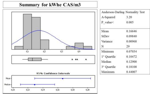
Fig. 3. Results of the analysis conducted on the ratio between the amount of energy consumed for the production of compressed air and the compressed air produced.
