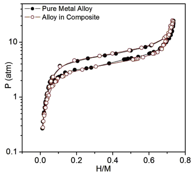
Fig. 10. Normalised Pressure Composition Temperature isotherms obtained at 40 °C for the extruded metal hydride-polymer composite in comparison with that for the pristine pure LaNi 5 -type metal hydride. Data are relative to a complete hydriding/dehydriding cycle.
