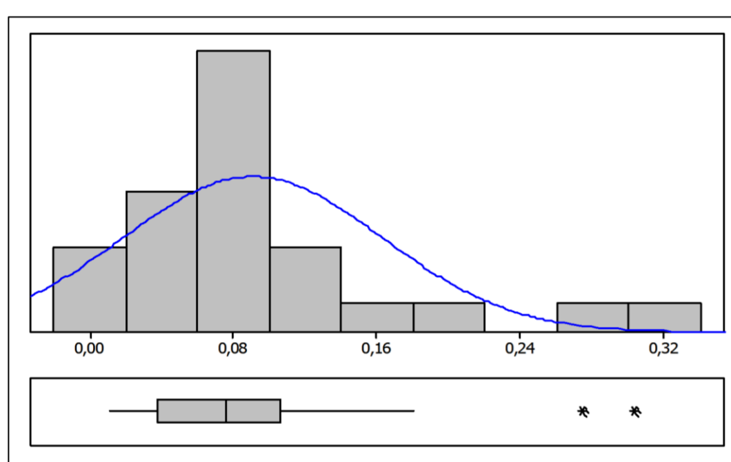
Ratio between the CAS's and the total electricity consumption (sectorial, manufacture of basic metals shown as an example).
