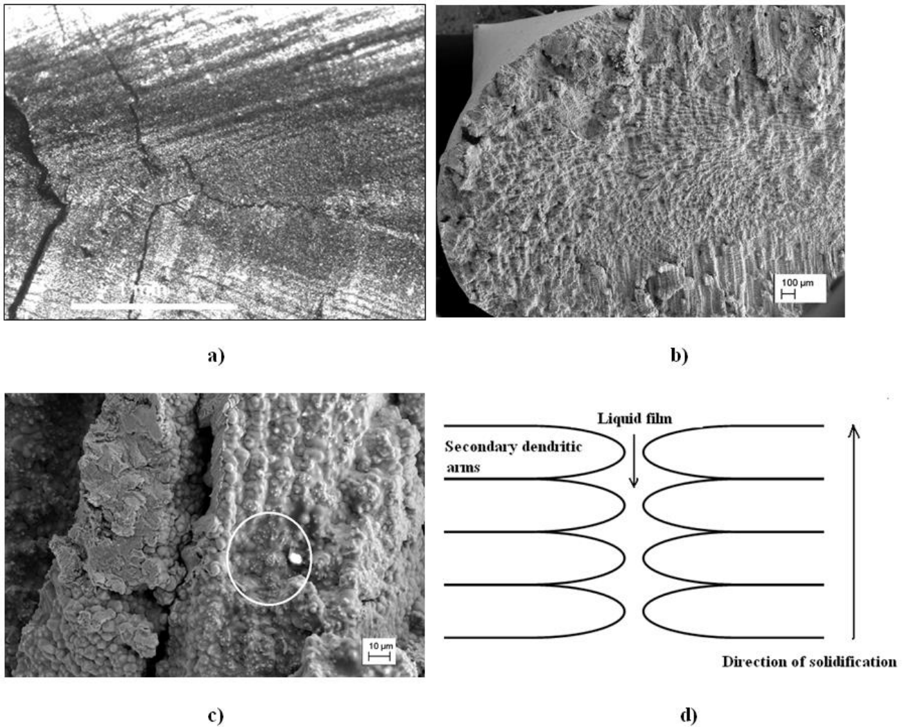
Fig. 1- Sample welded without pre-heating: cracks and pores are observed in the seam (a); fracture surfaces clearly show the dendritic structure (b-c). Schematic view of the mechanism leading to interdendritic fracture (d).
