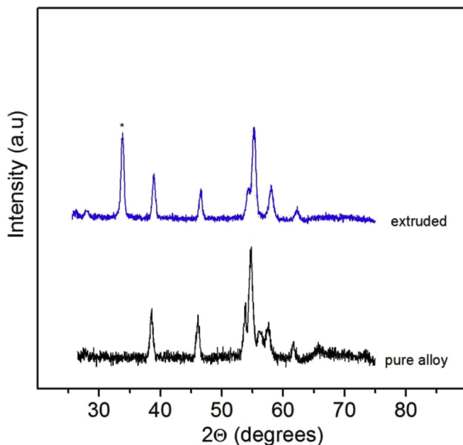
Fig. 6. X-ray diffraction patterns of the extruded metal hydride-polymer composite and the pristine pure \text{LaNi}_5 -type metal hydride.
