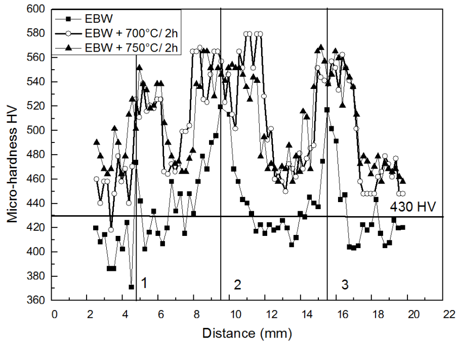
Fig. 5- Micro-hardness profiles across three parallel seams realized by EB welding with pre-heating at 300 °C. The different conditions are compared: as-welded, heat treated at 700 °C and 750 °C for 2 hours.
