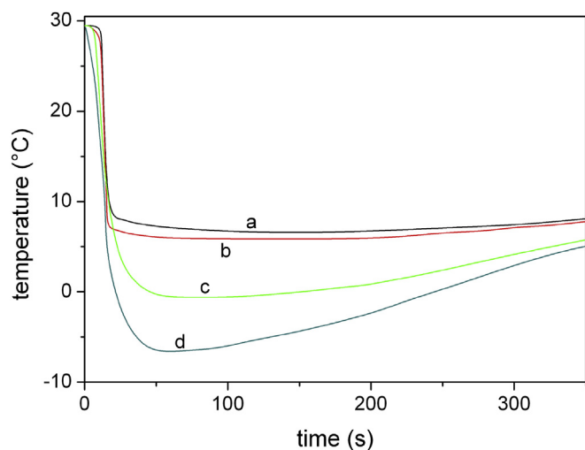
Fig. 13. Thermal behaviour of cold bed in the active refrigerating phase of the Metal Hydride Cooling System. The curves a and b represent the inlet and the outlet temperatures of the heat exchanging water in function of the time. The curves c and d represent the temperature values in function of the time as measured inside the cold bed at the two ends of the cylindrical reactor containing the active material.
