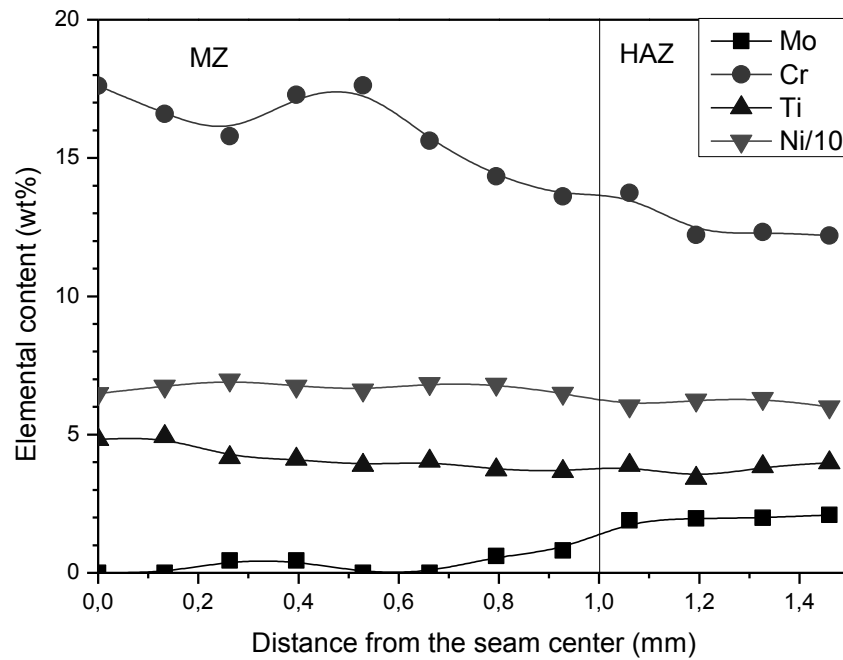
Fig. 4- EB welds obtained with pre-heating at 300 °C and pass speed of 2.5 m/min. Auger line scan of elemental content (wt%) determined from the Mo MNN, Cr LMM, Ti LMM and Ni LMM peak areas, respectively.
