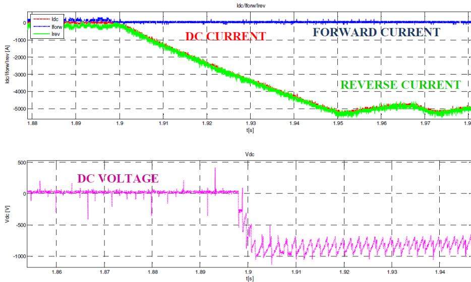
Figure 9 - Test number 4 for voltage consign.
