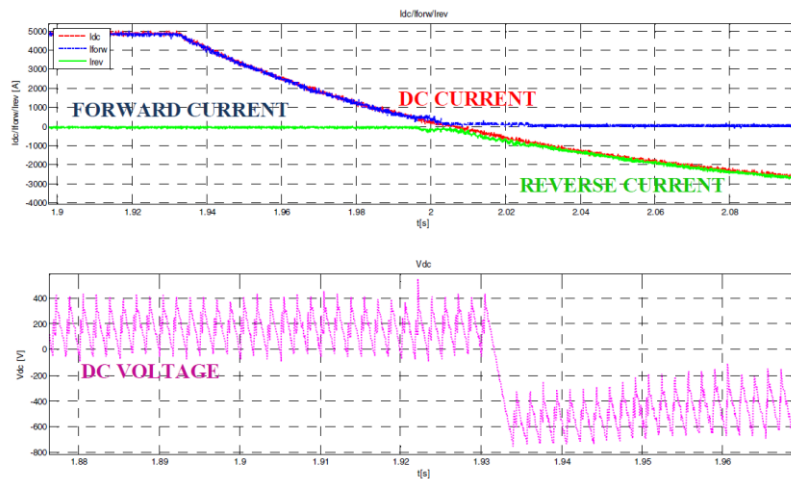
Figure 4 - Test number 2 for current consign
