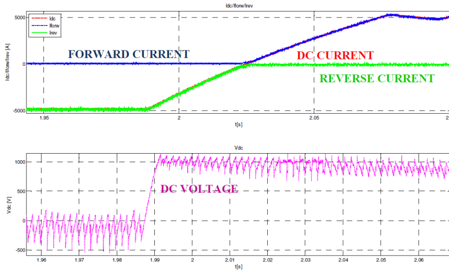
Figure 8 - Test number 3 for voltage consign.
