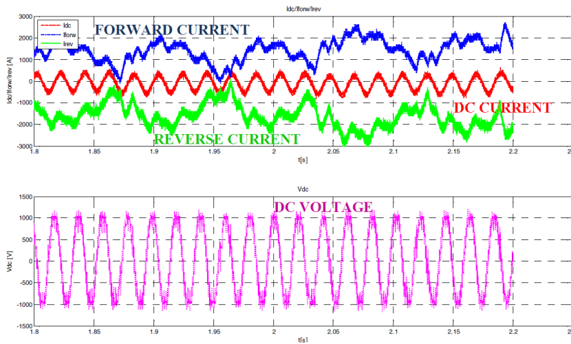
Figure 13 - Test number 10 for voltage consign at variable frequency.
