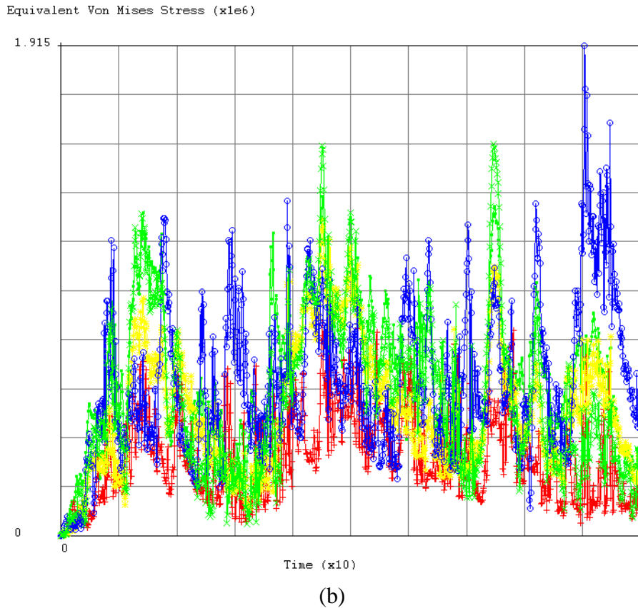
Figure 17 ó Von Mises stress distribution along the inner vessel at t = 5.75 s (a) and mean value far from the nozzle area (b).
