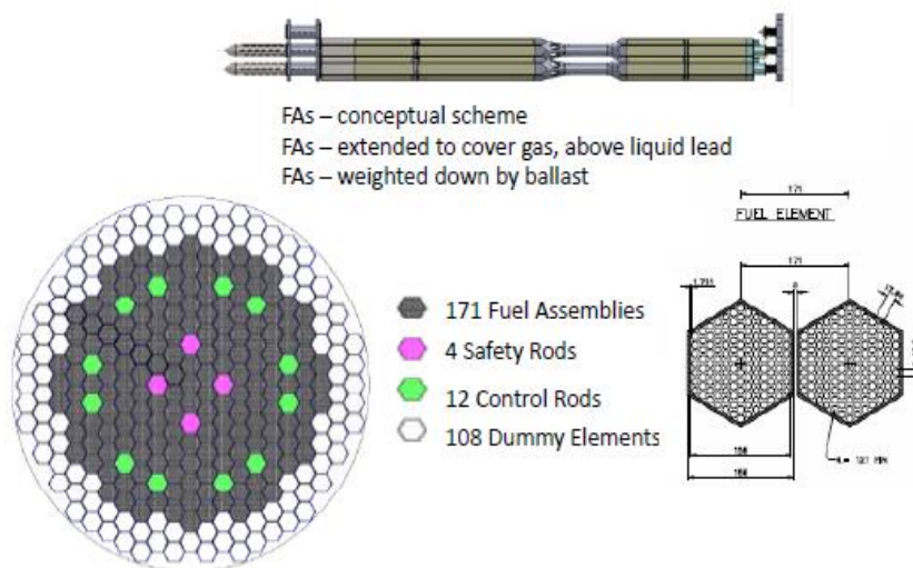
Figure 4 - Core and fuel assembly configuration.
