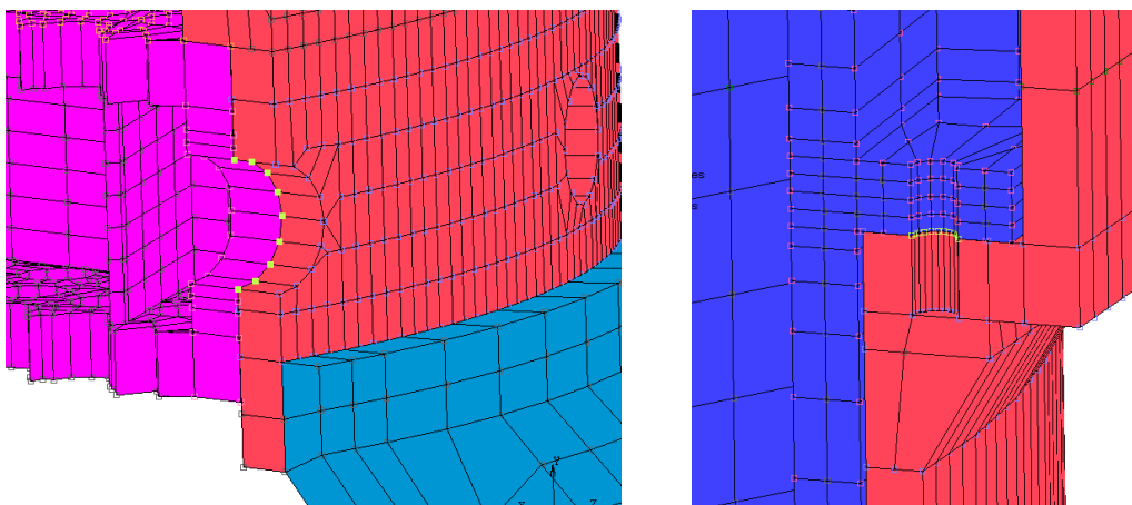
Figure 10 6 Detail of the connection between the lower and upper grid and the inner vessel.
