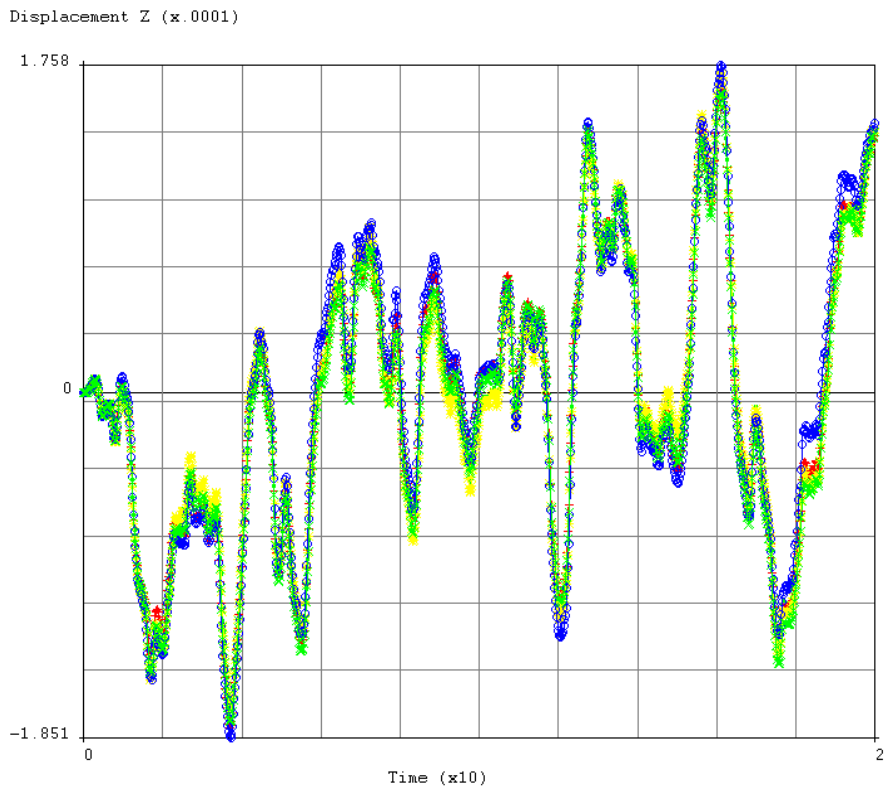
Figure 14 ó Displacements along the overall inner vessel.
