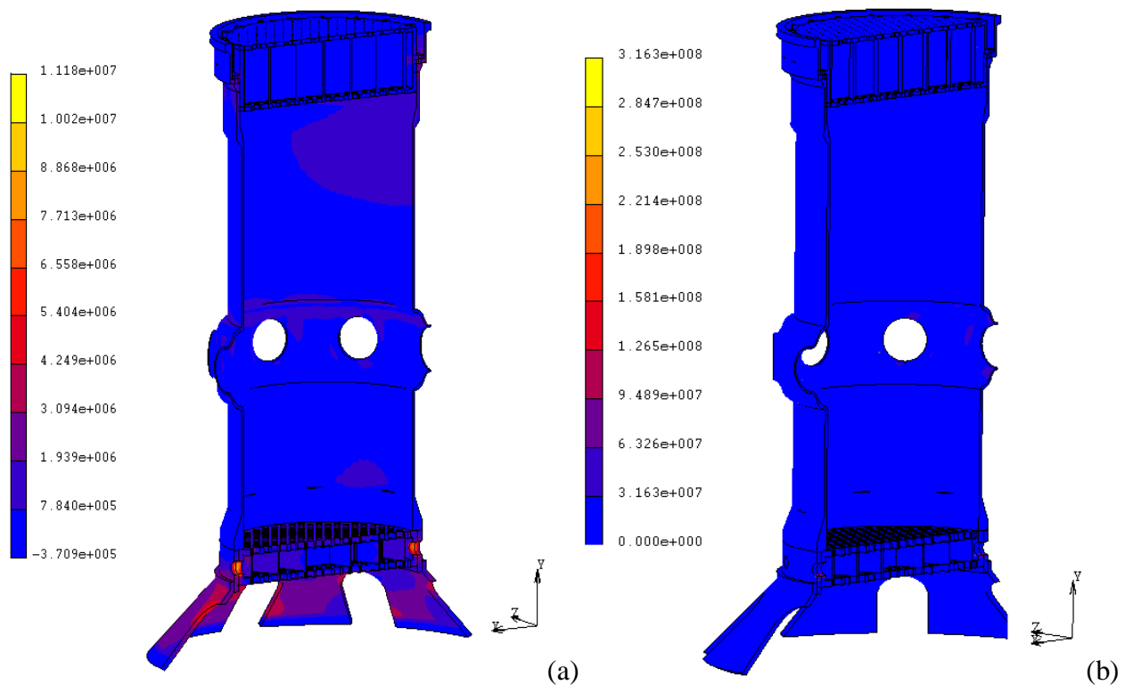
Figure 12 ó Von Mises stress without (a) and with contact and friction forces influence (b).
