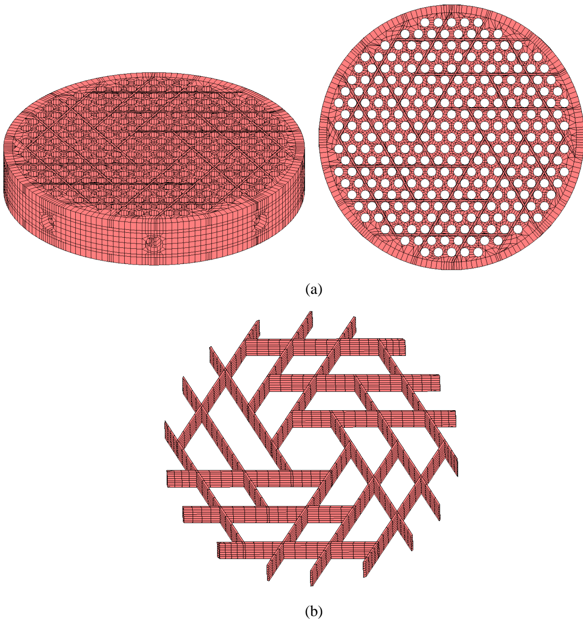
Figure 7 ó Details of the implemented FEM model of the lower grid: plates (a) and spacer grid (b).
