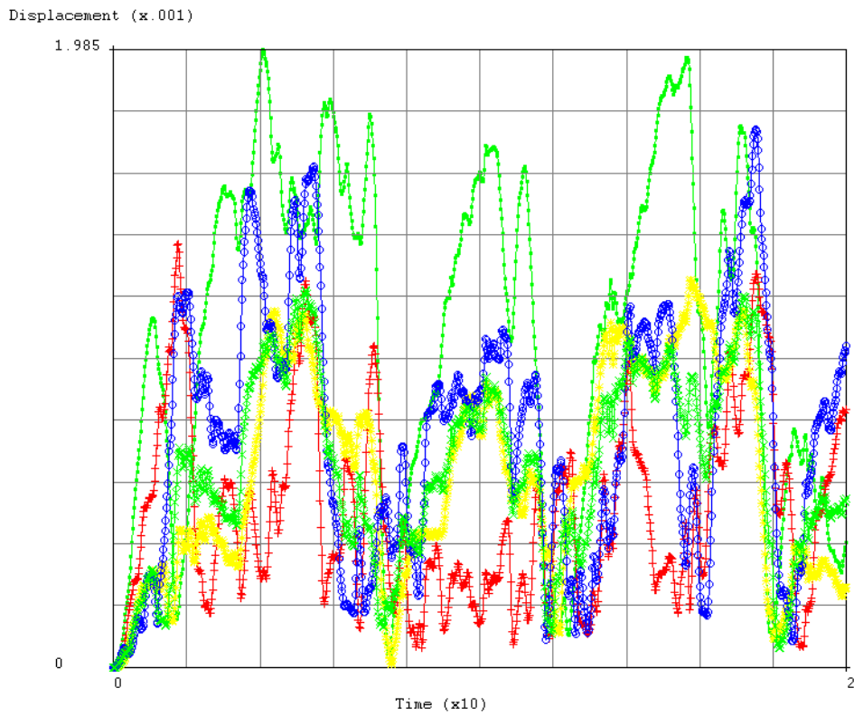
Figure 15 ó Total displacement along the overall inner vessel.
