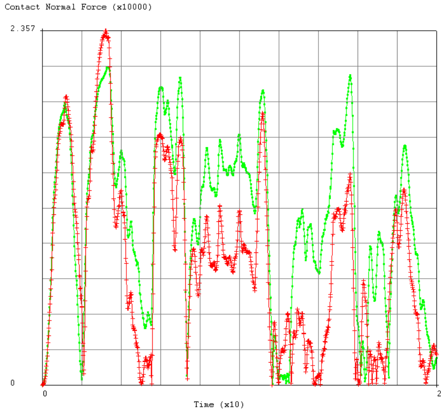
Figure 18 Contact normal force at the surface between upper (green line) and bottom grid (red line) and the inner vessel.
