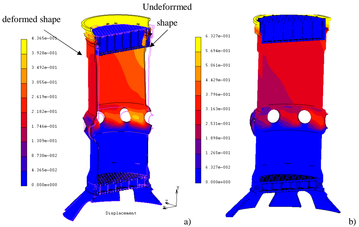
Figure 13 Displacement along the overall inner vessel at 4 s and 5.5 s.
