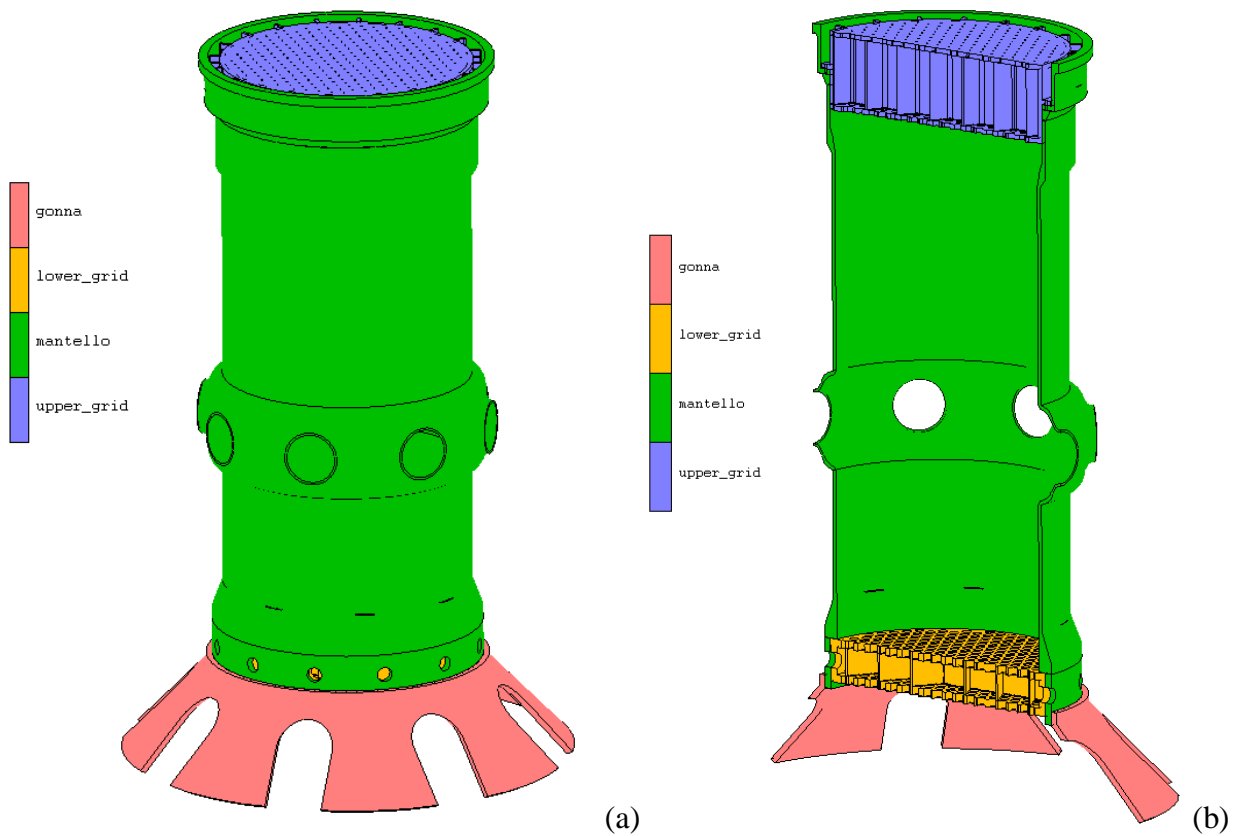
Figure 6 ó FEM model of the inner cylindrical vessel: view (a) and vertical section (b).
