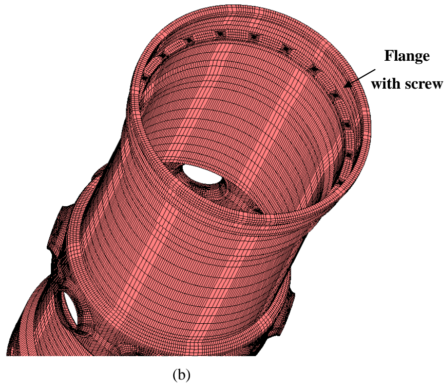
Figure 8 6 Details of the FEM model of the inner vessel: bottom part with lower late and diagrid (a) and upper part with flange for the positioning of upper grid (b).
