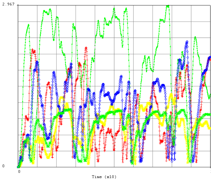
Figure 20 ó Total displacement close to the upper (green line) and bottom grid (red line).
