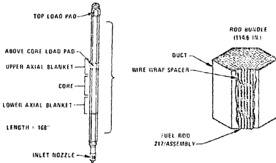
Figure 3 ó General scheme of fuel restraints.
