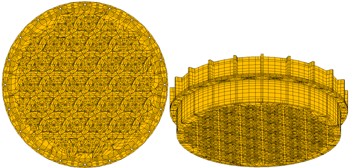
Figure 9 ó Details of the implemented FEM model of the upper grid.
