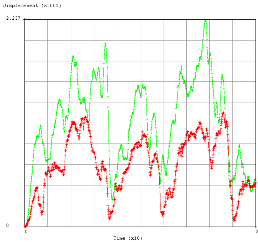
Figure 16 ó Total displacement close to the upper (green line) and bottom grid (red line).
