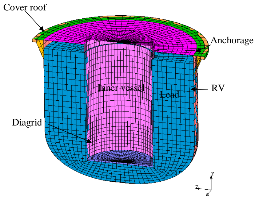
Figure 5 ó FEM model of the RV.
