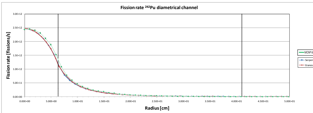
Figure 16 – ^{242}\text{Pu} fission rate in the diametrical channel.
