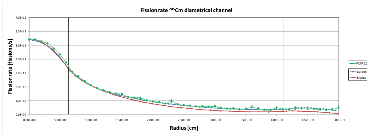
Figure 28 – 245 Cm fission rate in the diametrical channel.
