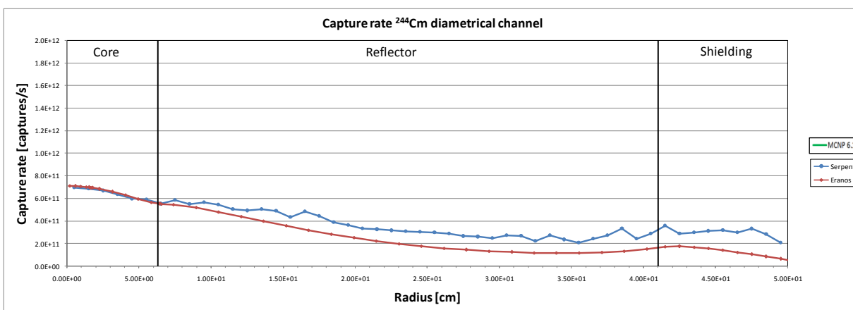
Figure 30 – 244 Cm capture rate in the diametrical channel.
