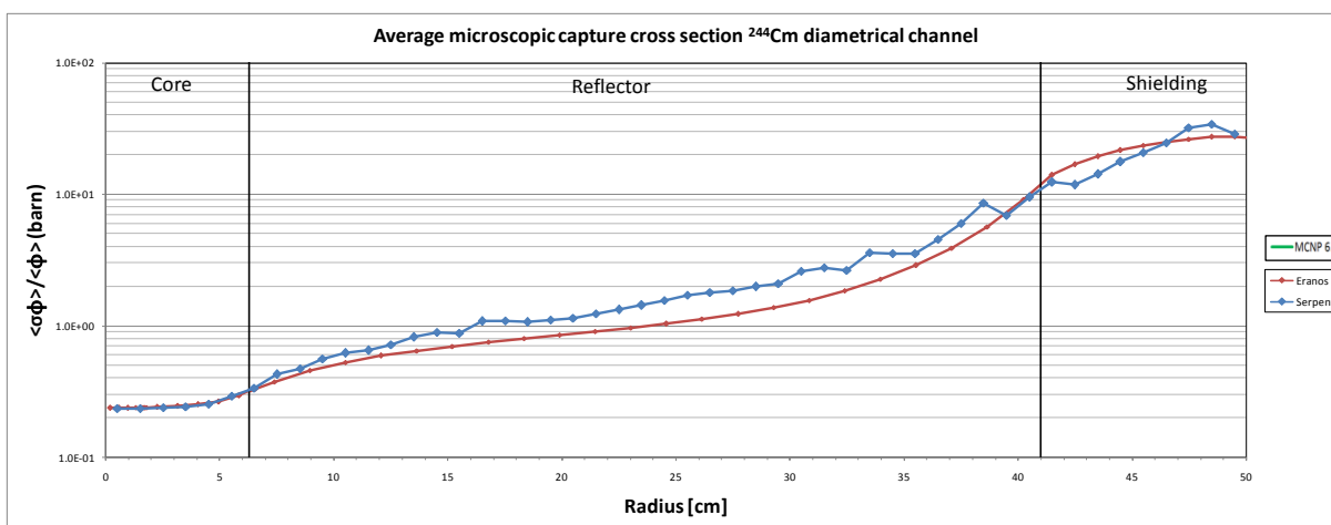
Figure 52 – ^{244}\text{Cm} average microscopic capture cross section
