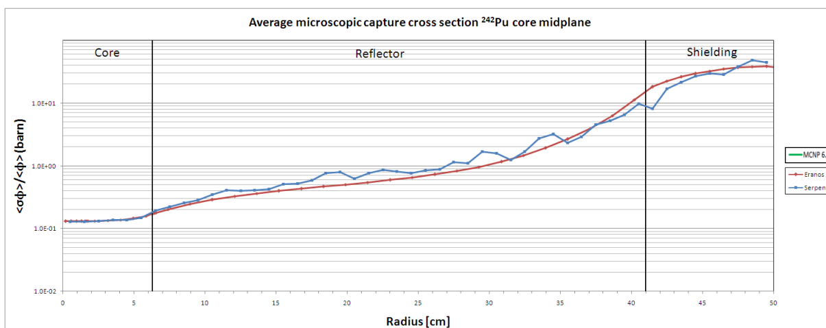
Figure 41 – ^{242}\text{Pu} average microscopic capture cross sections
