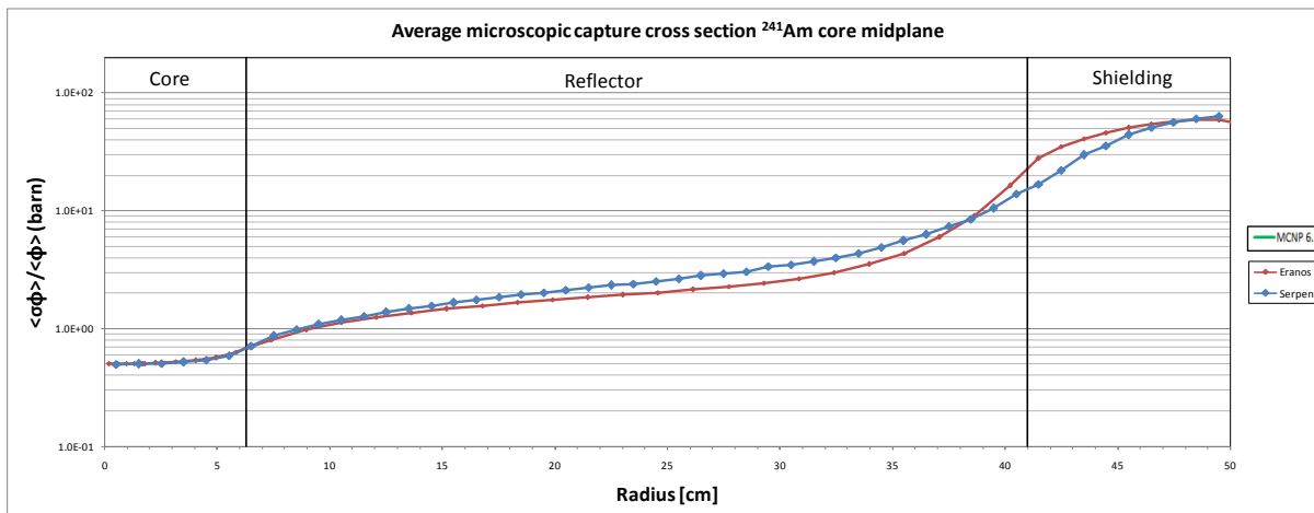
Figure 46 – 241 Am average microscopic capture cross section
