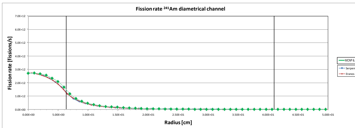
Figure 22 – ^{241}\text{Am} fission rate in the diametrical channel.
