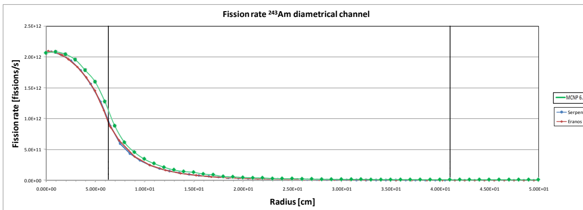
Figure 23 – 243 Am fission rate in the diametrical channel.
