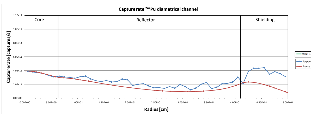
Figure 19 – 242 Pu capture rate in the diametrical channel.
