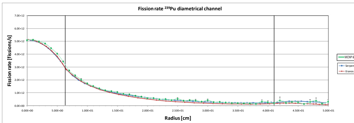
Figure 14 – ^{239}\text{Pu} fission rate in the diametrical channel.
