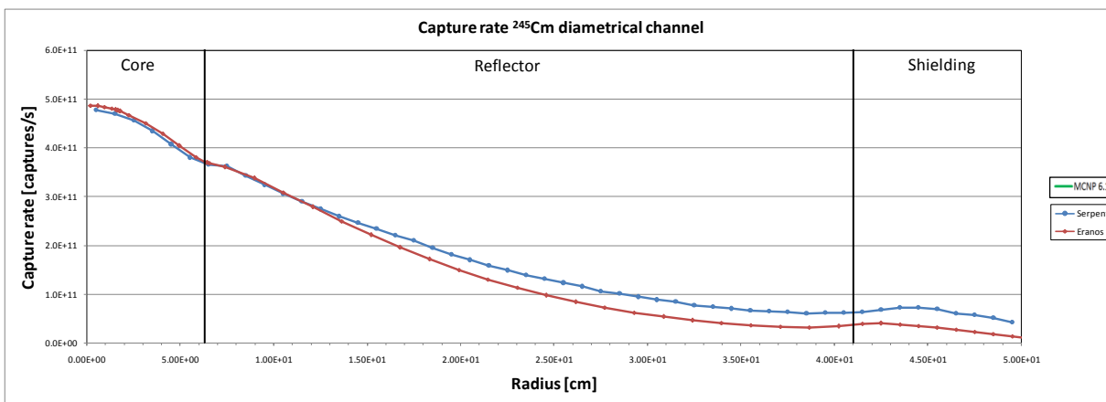
Figure 31 – 245 Cm capture rate in the diametrical channel.
