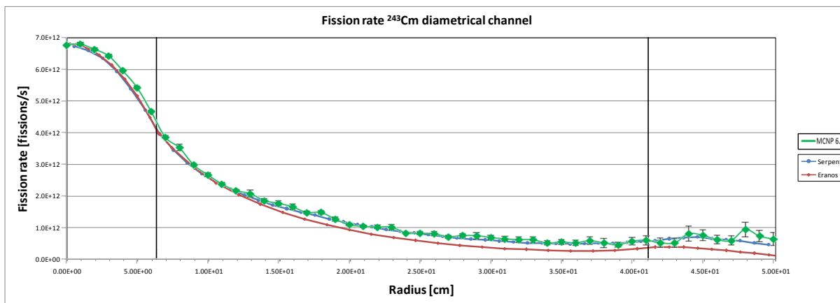
Figure 26 – 243 Cm fission rate in the diametrical channel.
