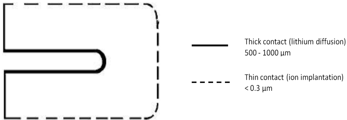
Figure 69 - HPGe detector
