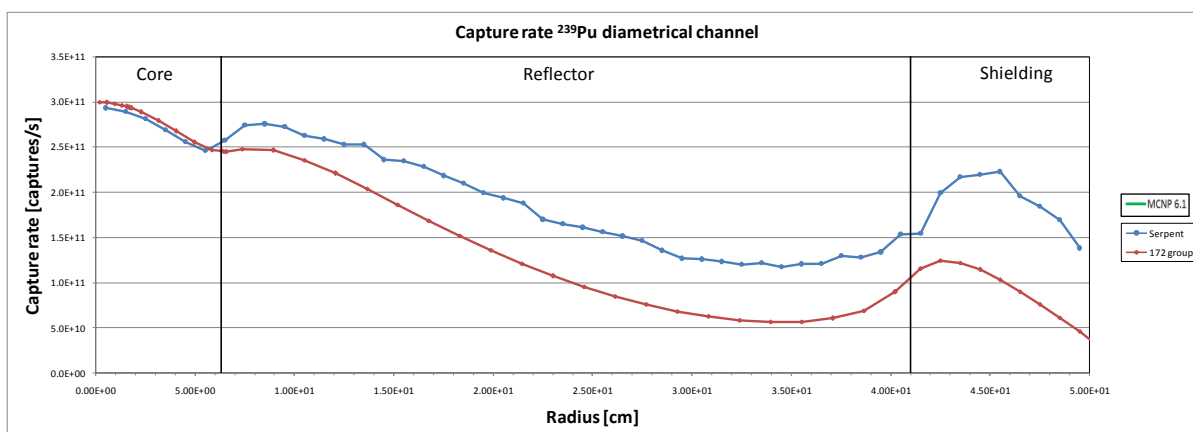
Figure 17 – 239 Pu capture rate in the diametrical channel.
