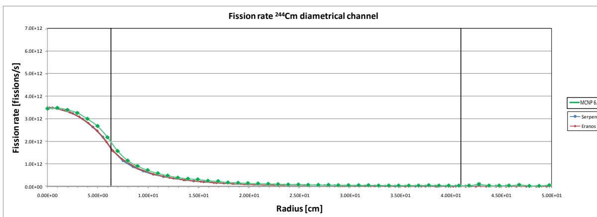
Figure 27 – 244 Cm fission rate in the diametrical channel.
