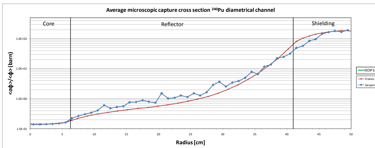
Figure 40 – ^{240}\text{Pu} average microscopic capture cross sections
