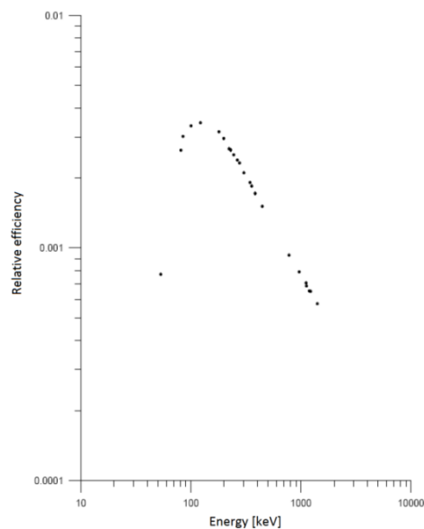
Figure 70 - Detector efficiency.
