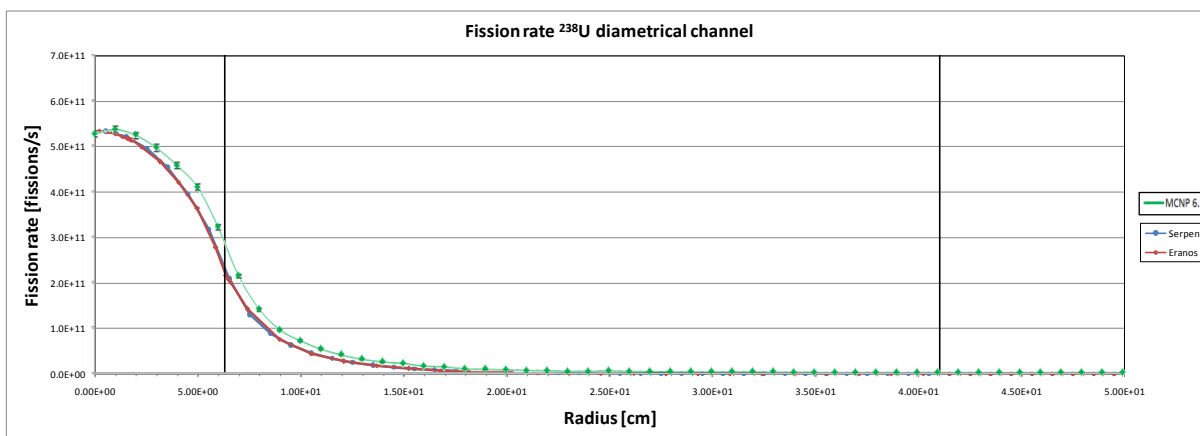
Figure 11 - 238 U fission rate in the diametrical channel.
