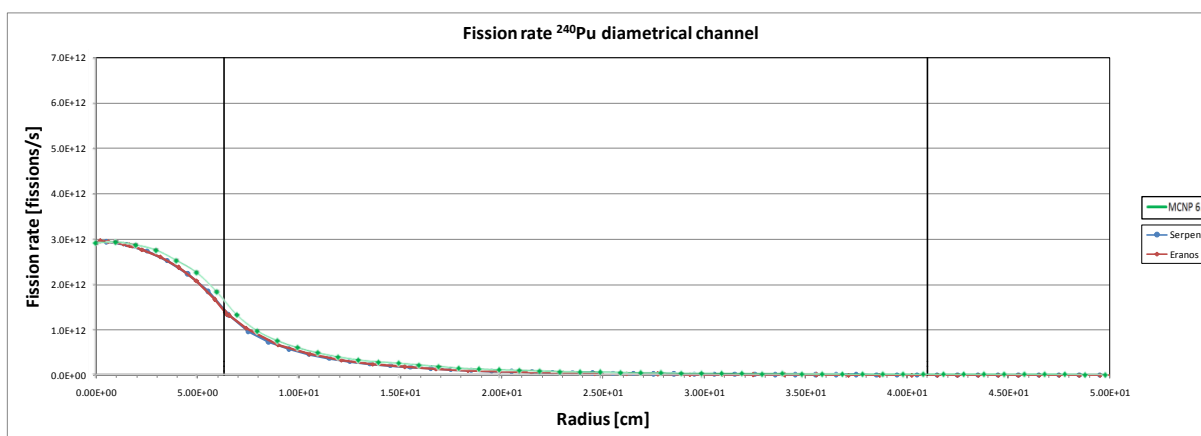
Figure 15 – ^{240}\text{Pu} fission rate in the diametrical channel.
