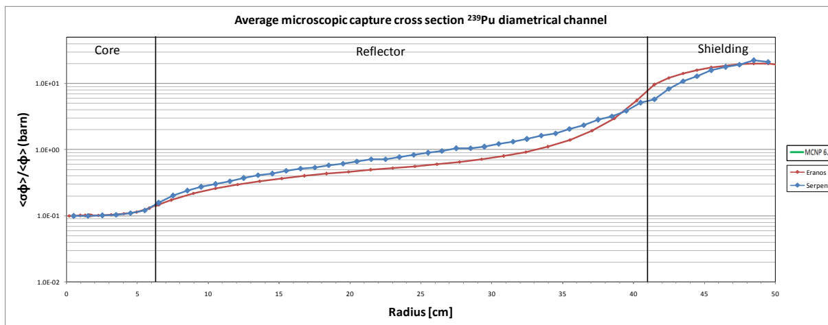
Figure 39 – ^{239}\text{Pu} average microscopic capture cross sections
