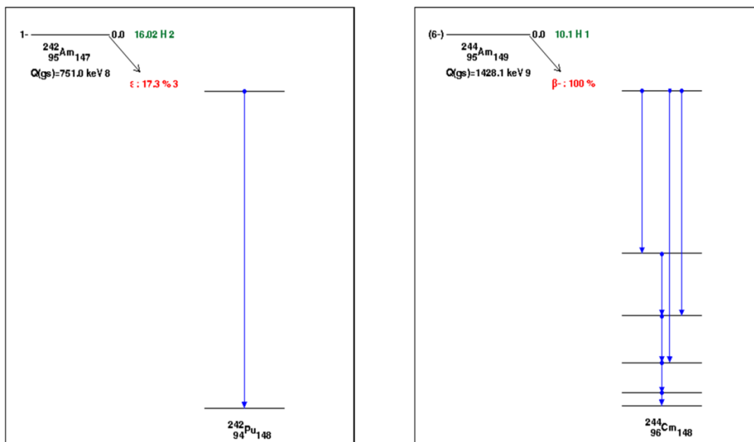
Figure 68 - Decay schemes for 242 Am and 244 Am.
