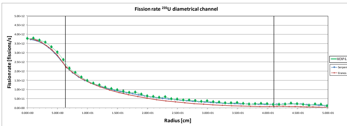
Figure 10 - 235 U fission rate in the diametrical channel.
