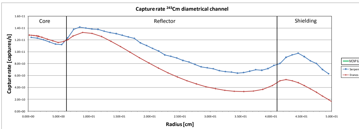
Figure 29 – 243 Cm capture rate in the diametrical channel.
