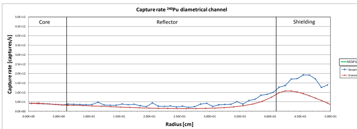
Figure 18 – 240 Pu capture rate in the diametrical channel.
