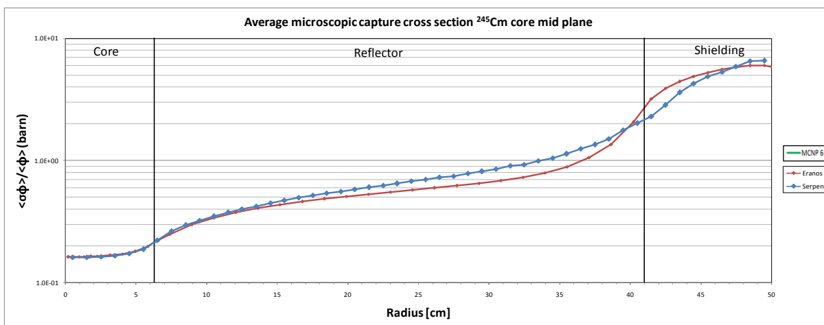
Figure 53 – ^{245}\text{Cm} average microscopic capture cross section
