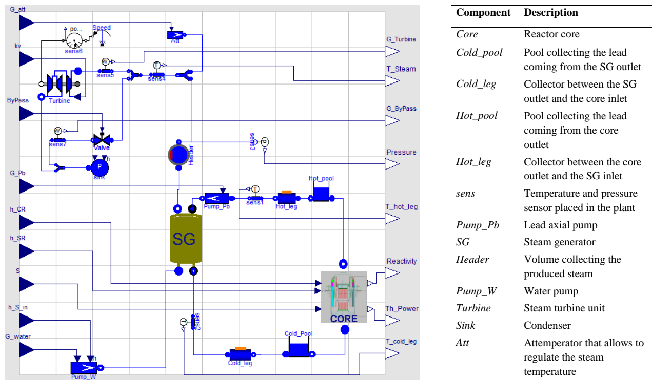
Figure 8. ALFRED object-oriented model.
