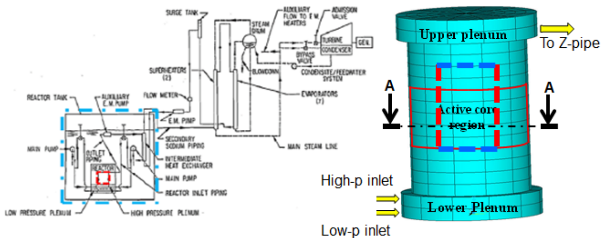
Figure 16. Computational domain of FRENATIC simulation (red-dashed line, left) vs. computational domain of RELAP5-3D© simulation by ENEA (blue-dashed line, left) and representation of axial computational domain of FRENATIC (right).
