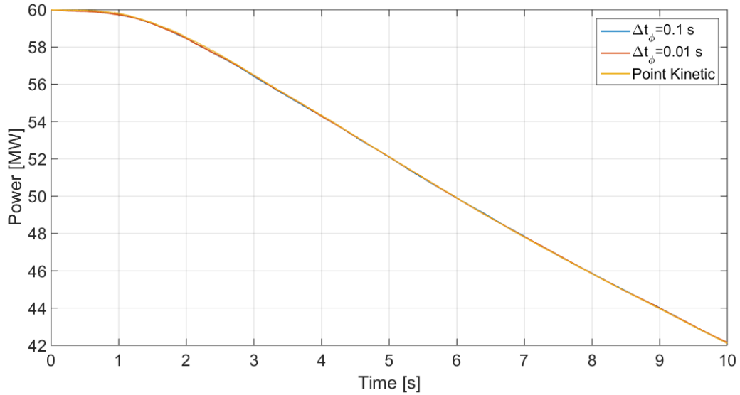
Figure 59. Total power computed by point kinetic and quasi-static algorithms for first 10 s of the transient.
