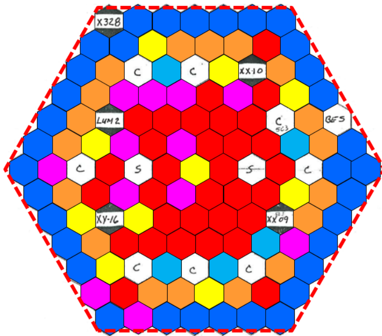
Figure 17. Core loading pattern of SHRT-17 transient: portion of the core considered in the FRENETIC calculations.
