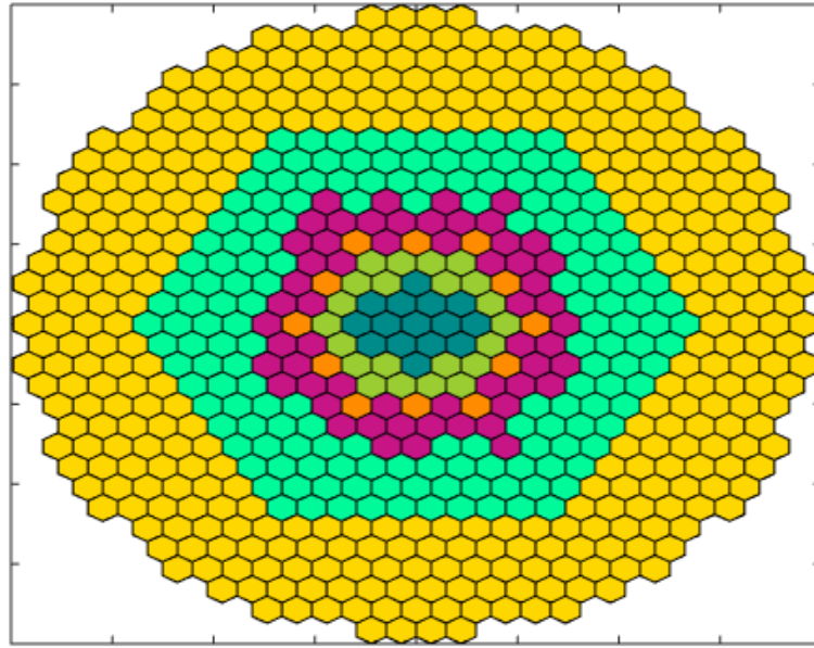
Figure 54. Radial zones. From centre: inner core, medium core, control region, outer core, radial reflector and blanket.
