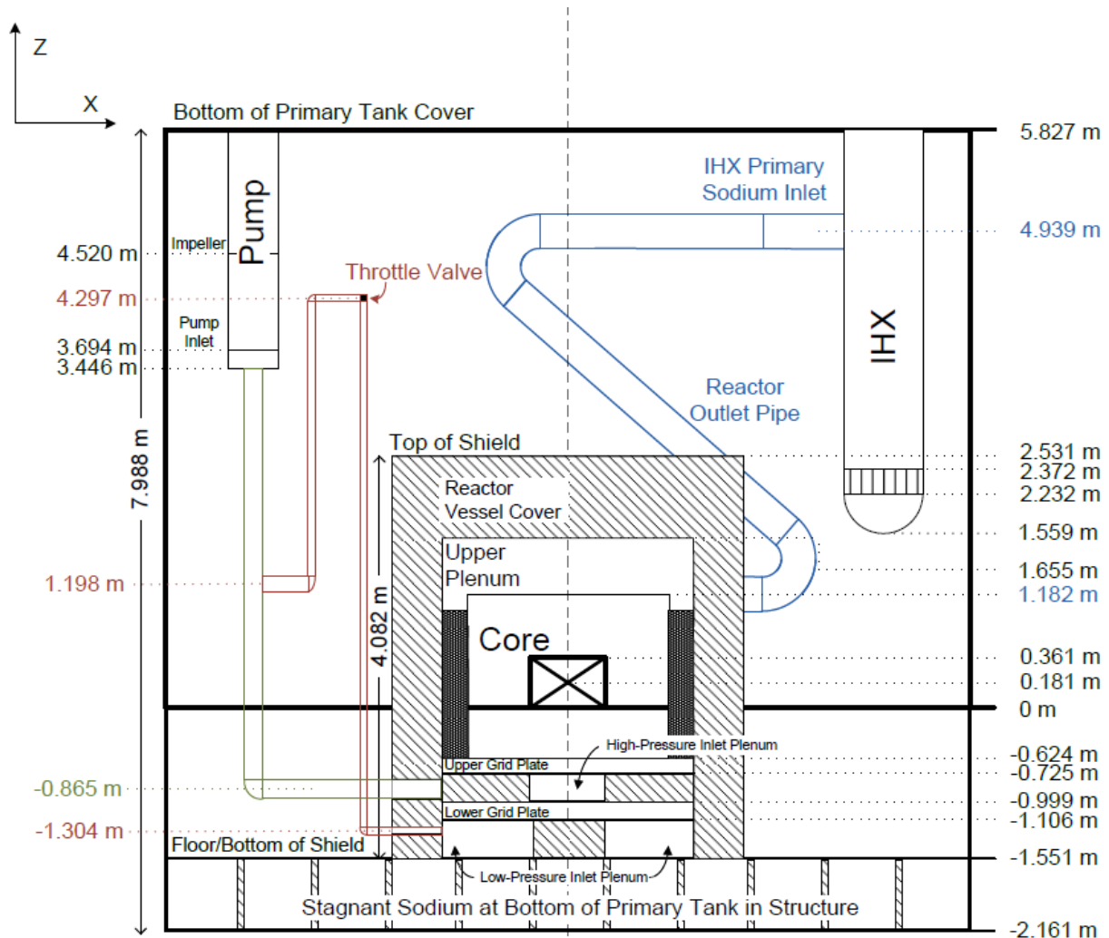
Figure 7. Benchmark model of primary vessel components, elevation view [13].
