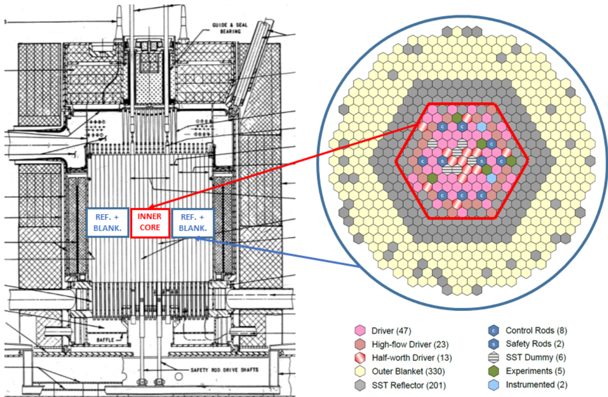
Figure 4. EBR-II reactor pool with HAs (left) and core pattern of the SHRT-45R transient (right) [15].
