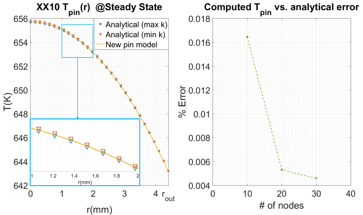
Figure 42. XX10 steady state distribution at a height z = 0.16 m with new radial model vs. full cylinder analytical solution and error with respect to analytical solution.
