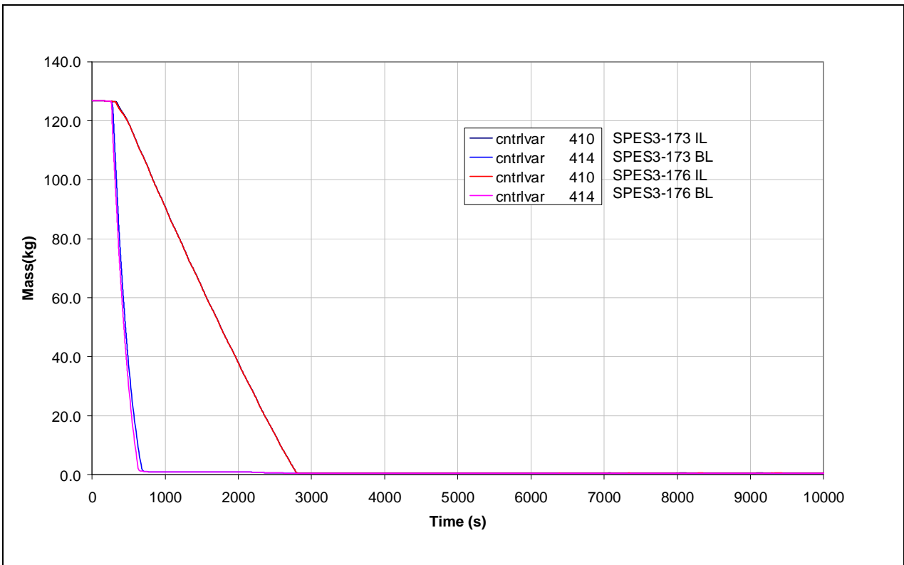
Fig.8. 61 – SPES3-173 and SPES3-176 EBT mass
