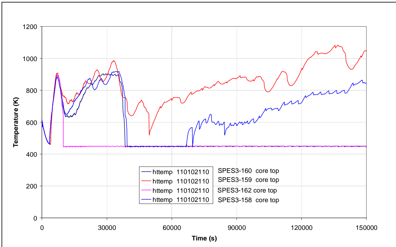
Fig.5. 13 – SPES3-159, 162, 158 and 160 Core heater rod clad surface temperature (normal rods)
