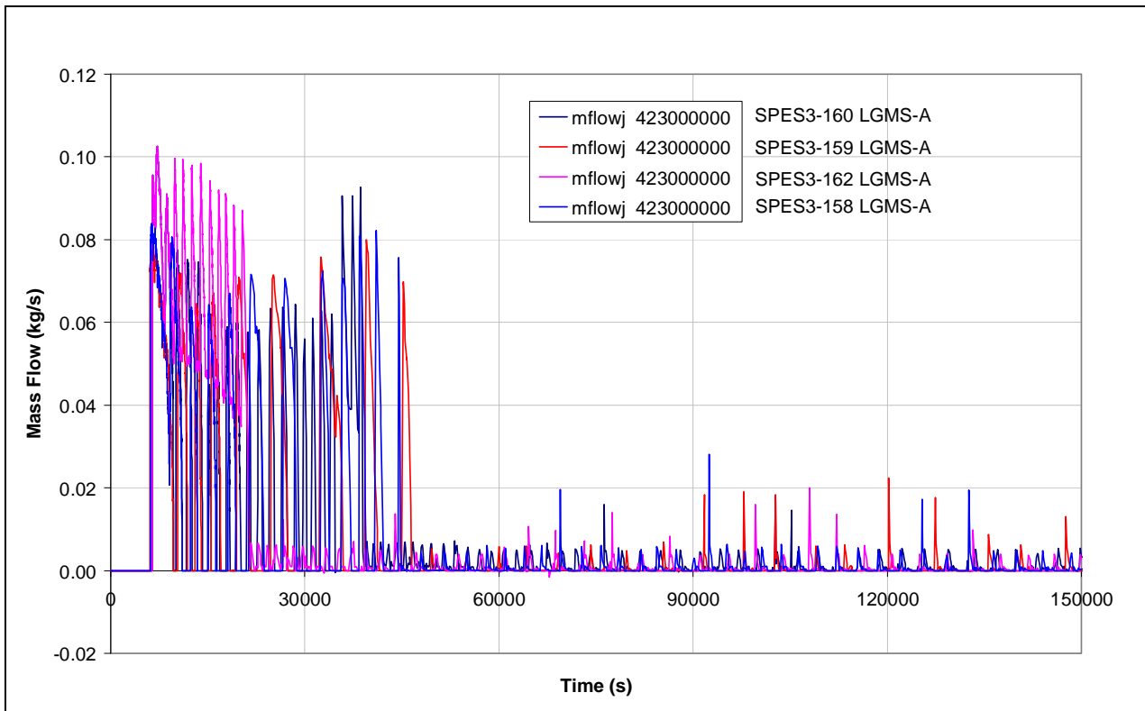
Fig.5. 9 – SPES3-159, 162, 158 and 160 LGMS to DVI line mass flow (intact loop)
