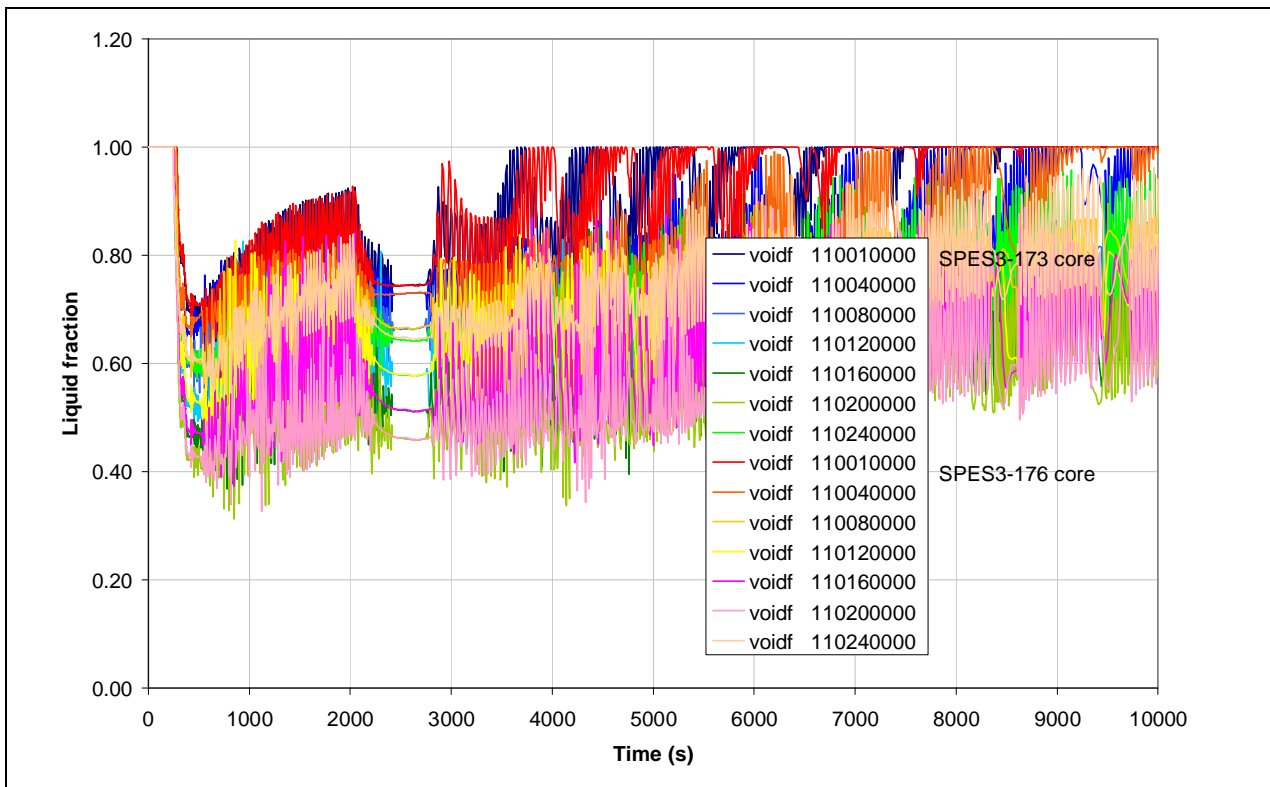
Fig.8. 64 – SPES3-173 and SPES3-176 Core liquid fraction (window)
