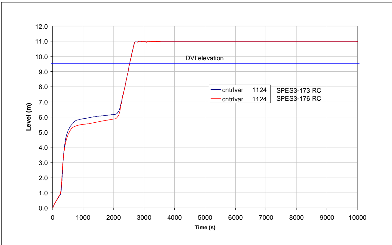
Fig.8. 37 – SPES3-173 and SPES3-176 RC level (window)
