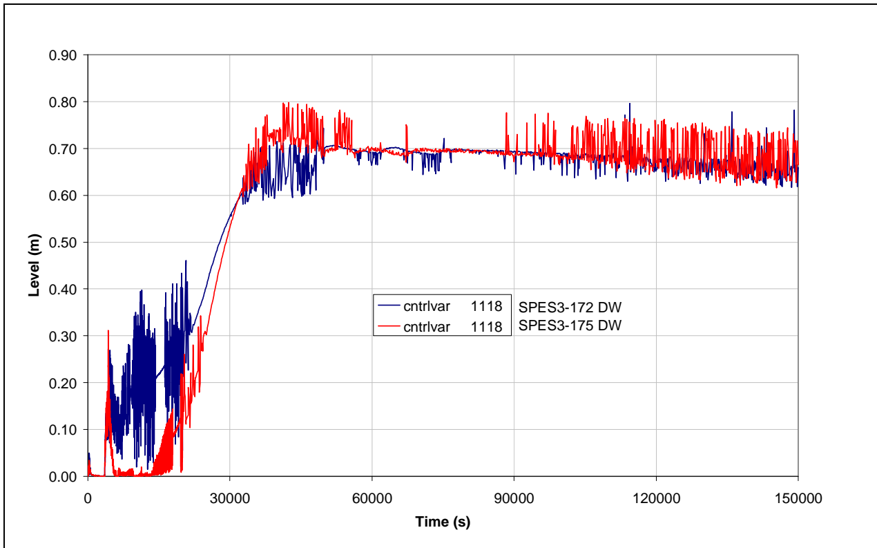
Fig.7. 67 - SPES3-172 and SPES3-175 DW level
