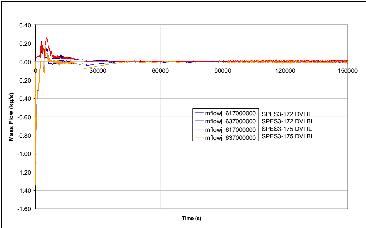
Fig.7. 69 - SPES3-172 and SPES3-175 DVI mass flow
