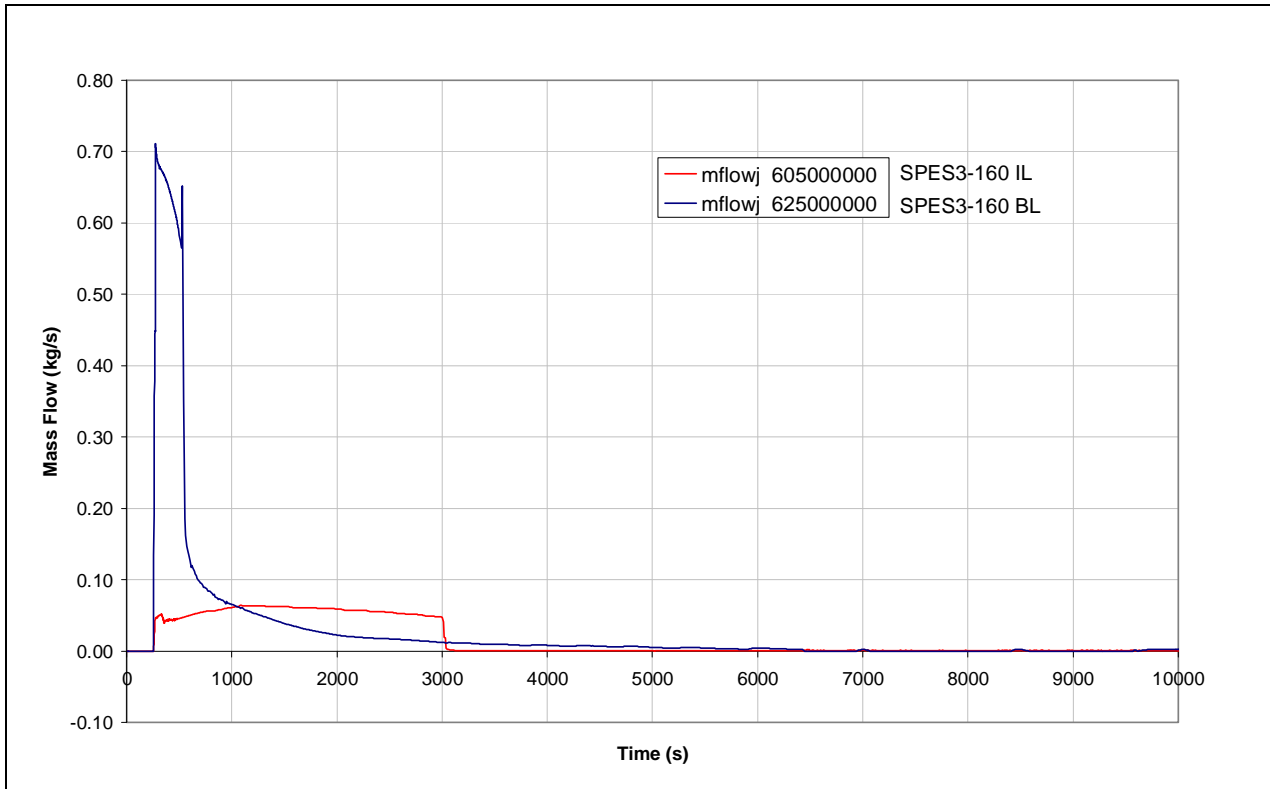
Fig.4.3 – SPES3-160 EBT injection mass flow (window)
