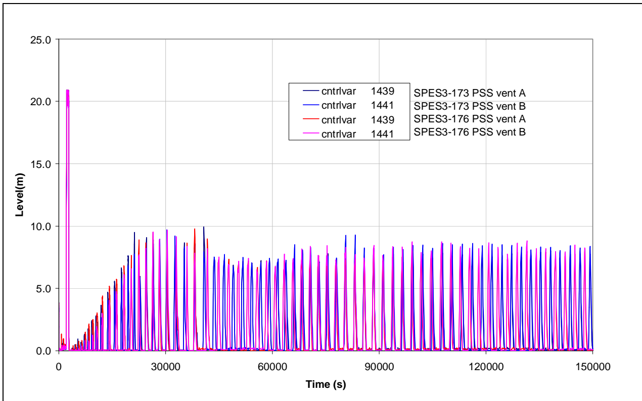
Fig.8. 33 – SPES3-173 and SPES3-176 PSS vent pipe level
