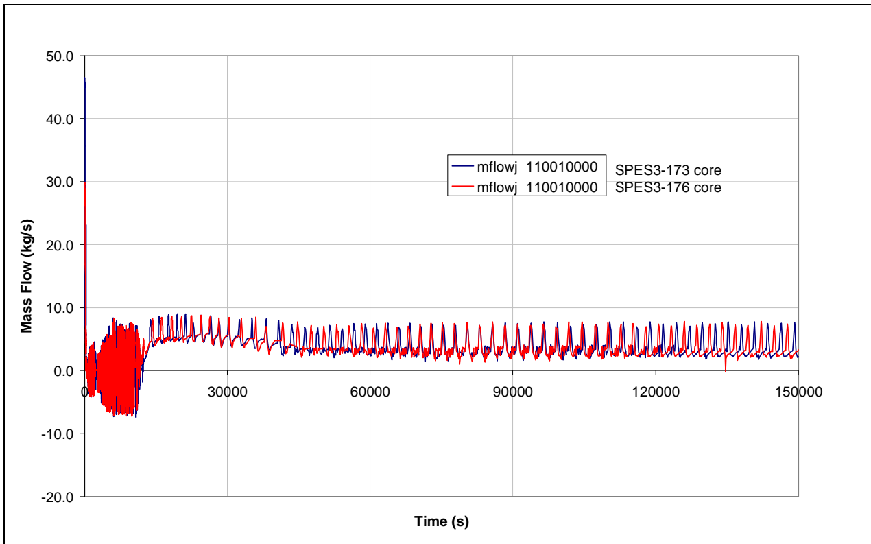
Fig.8. 57 – SPES3-173 and SPES3-176 core inlet flow
