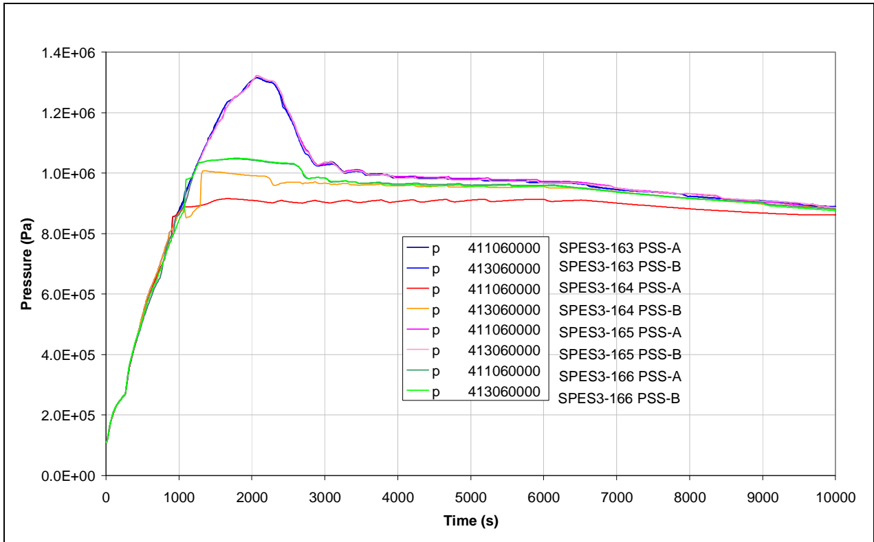
Fig.5. 17 – SPES3-163, 164, 165 and 166 PSS pressure (window)
