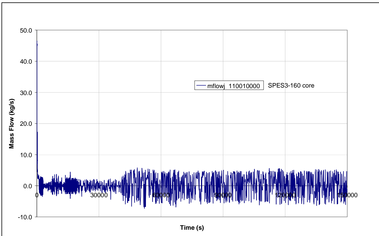
Fig.4.48 – SPES3-160 core inlet flow
