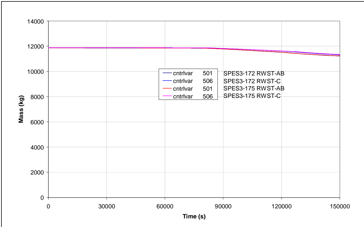
Fig.7. 75 - SPES3-172 and SPES3-175 RWST mass
