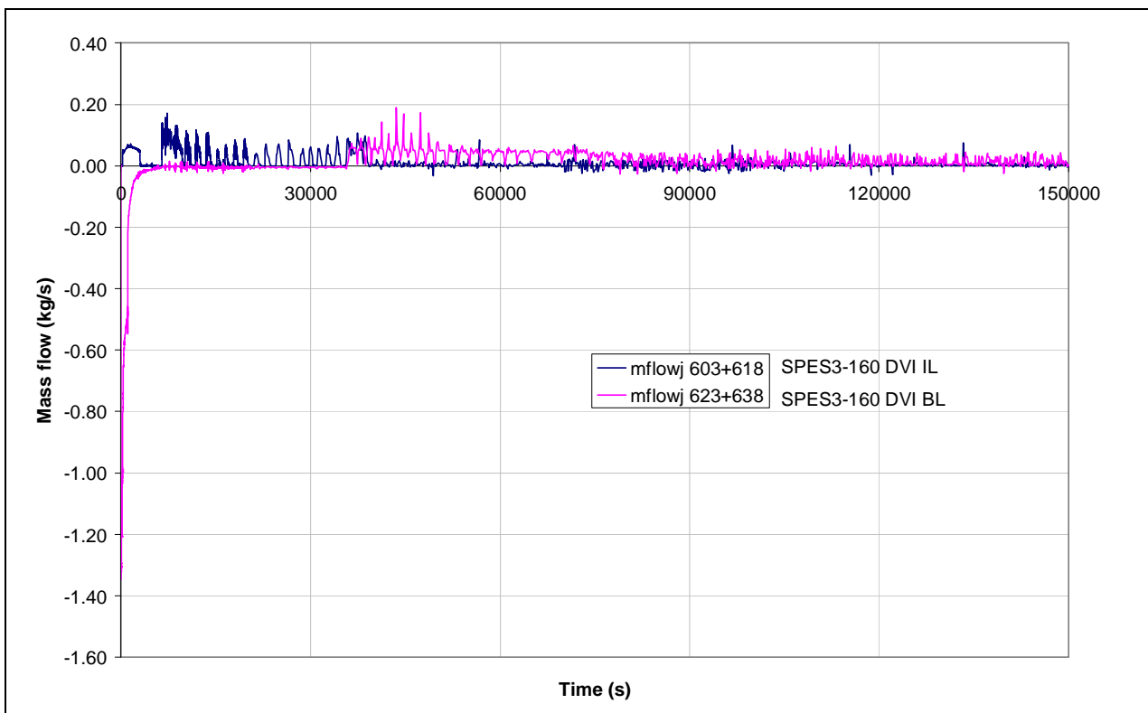
Fig.4.64 – SPES3-160 DVI line mass flow
