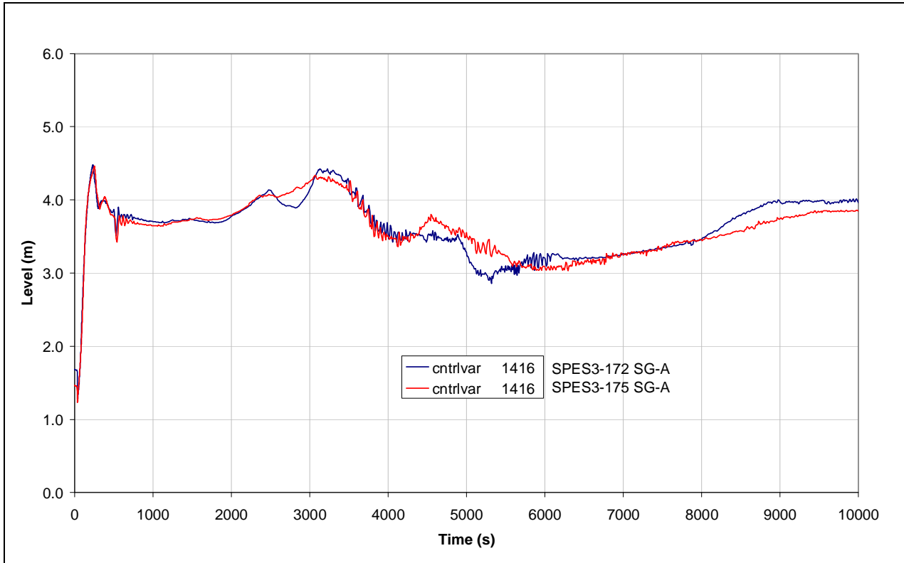
Fig.7. 43 - SPES3-172 and SPES3-175 SG-Ass collapsed level (window)
