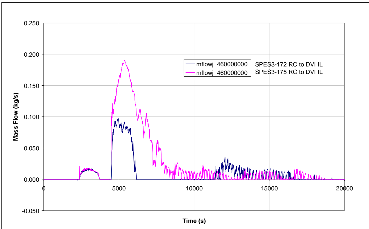
Fig.7. 56 - SPES3-172 and SPES3-175 RC to DVI mass flow IL (window)
