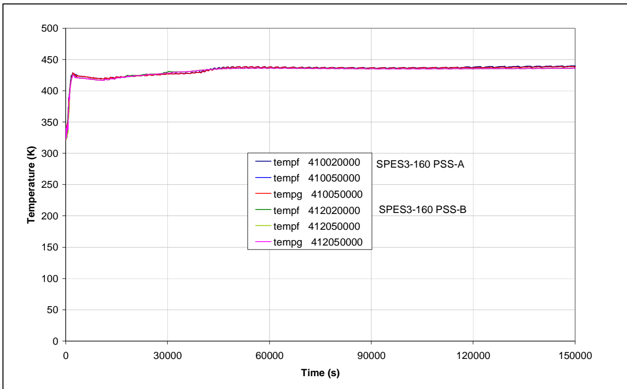
Fig.4.36 – SPES3-160 PSS temperature
