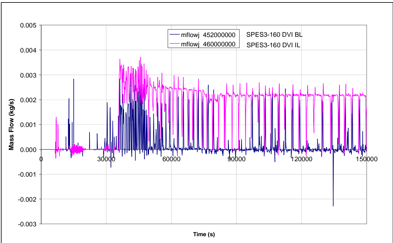
Fig.4.62 – SPES3-160 RC to DVI line mass flow
