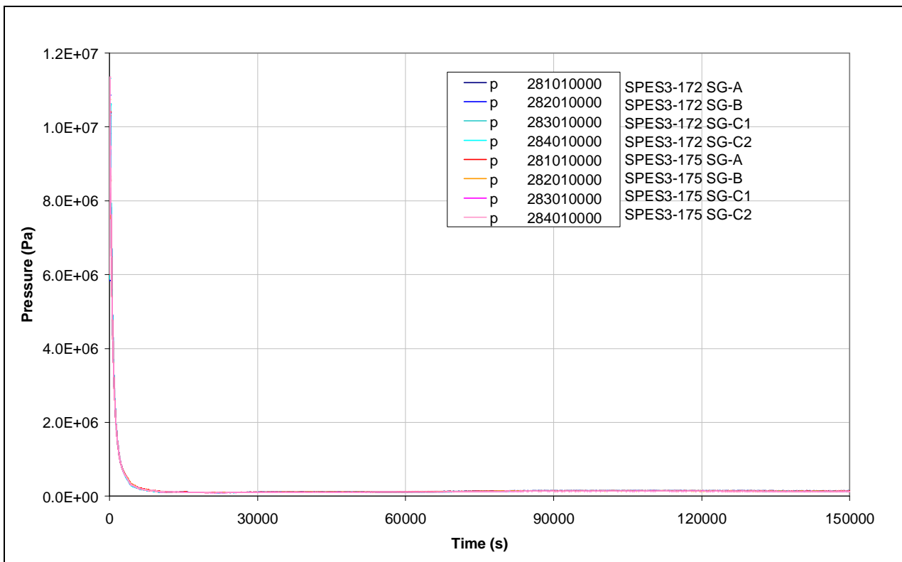
Fig.7. 42 - SPES3-172 and SPES3-175 SG ss outlet pressure
