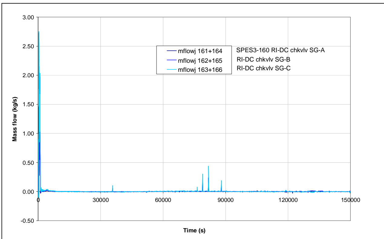
Fig.4.50 – SPES3-160 RI-DC check valve mass flow
