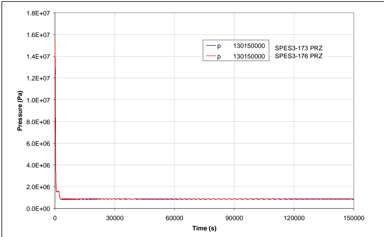
Fig.8. 17 – SPES3-173 and SPES3-176 PRZ pressure
