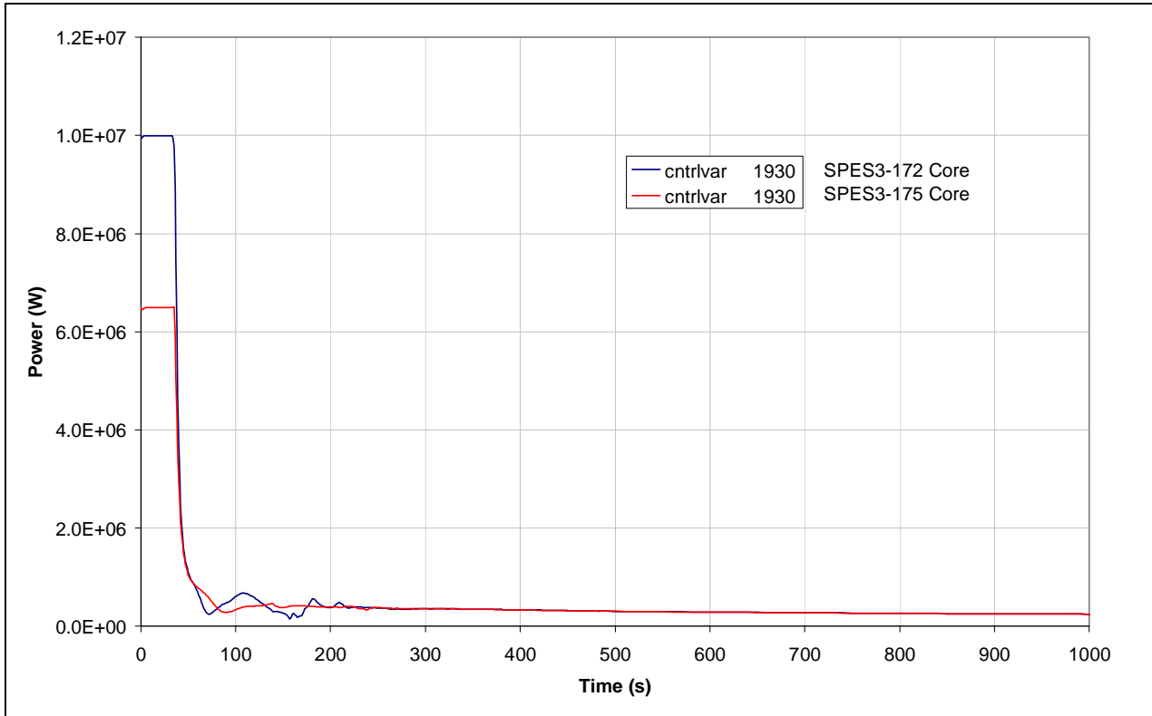
Fig.7. 31 - SPES3-172 and SPES3-175 Core power (window)
