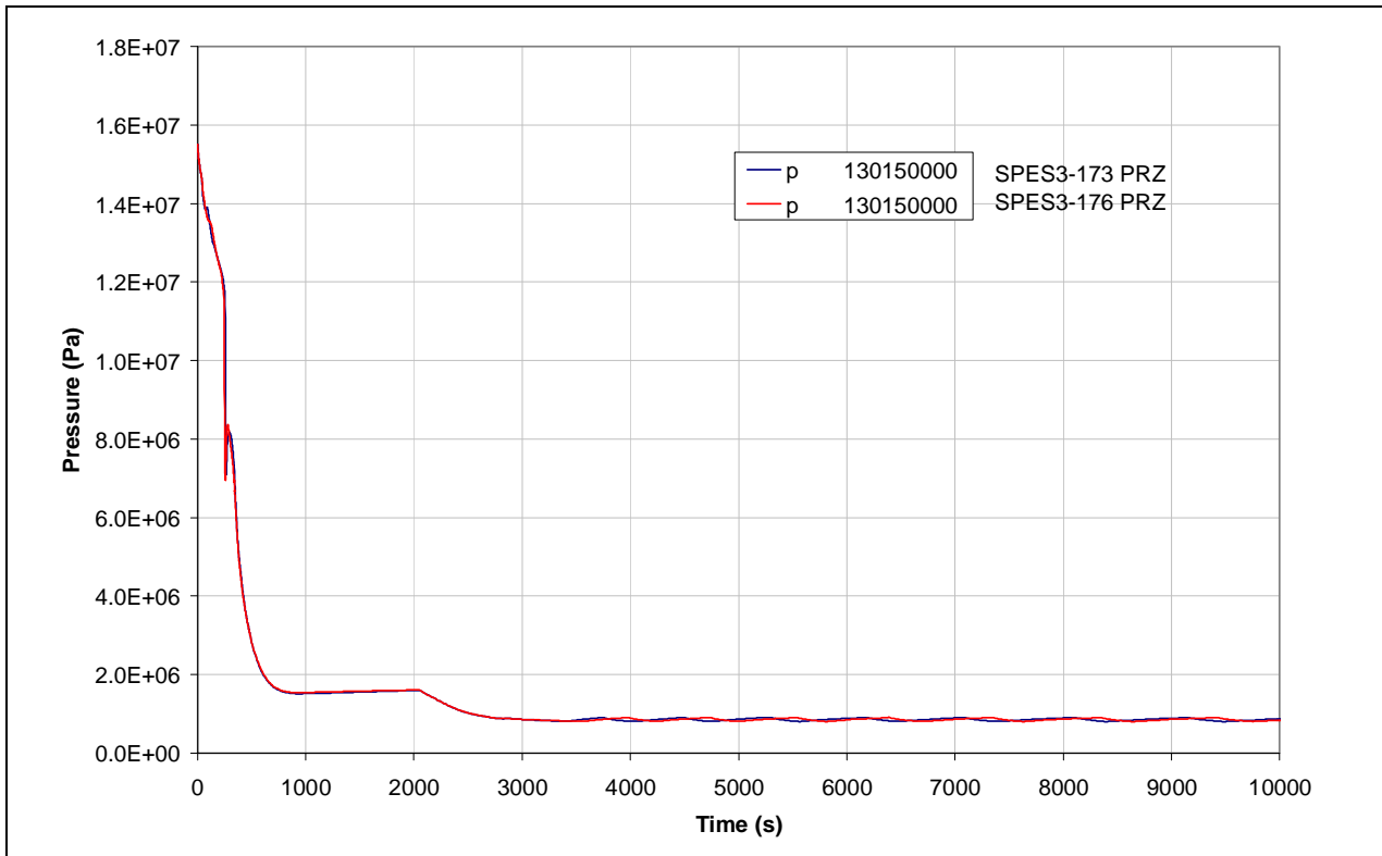
Fig.8. 16 – SPES3-173 and SPES3-176 PRZ pressure (window)
