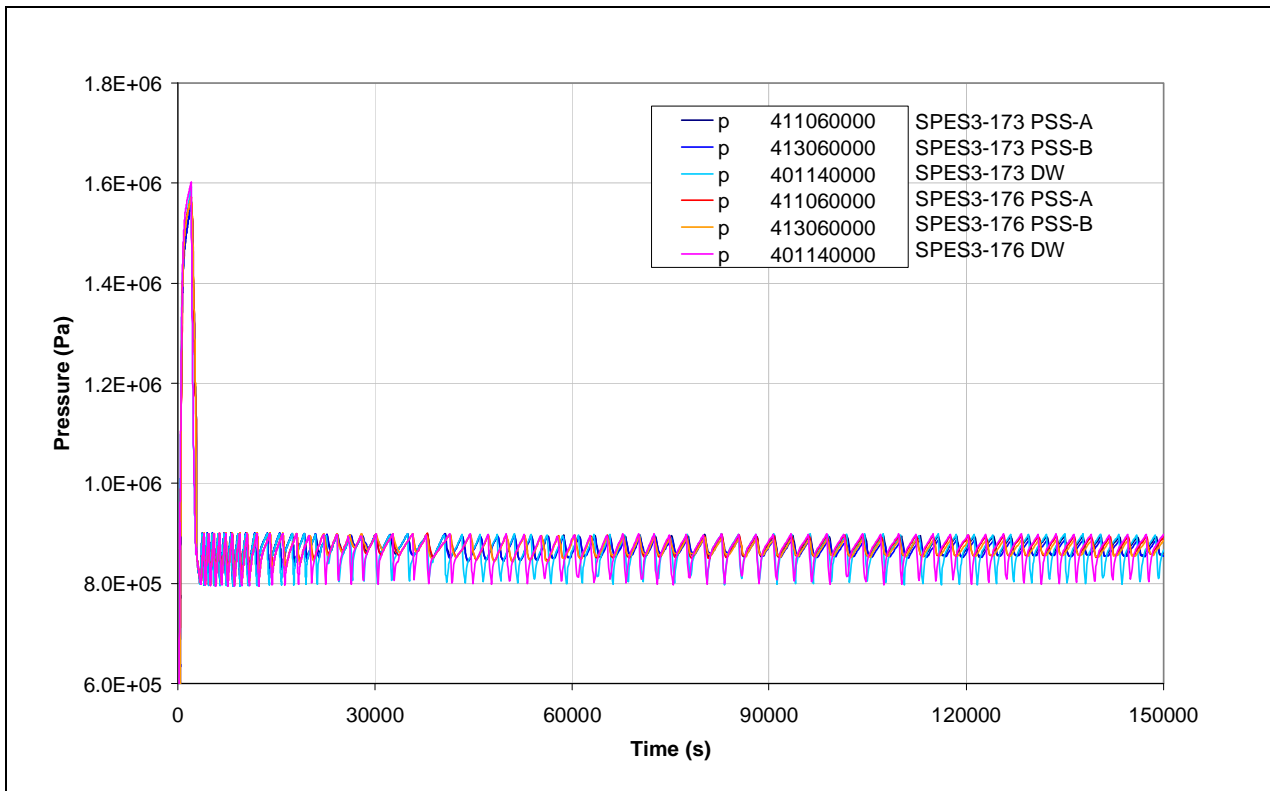
Fig.8. 31 – SPES3-173 and SPES3-176 PSS and DW pressure
