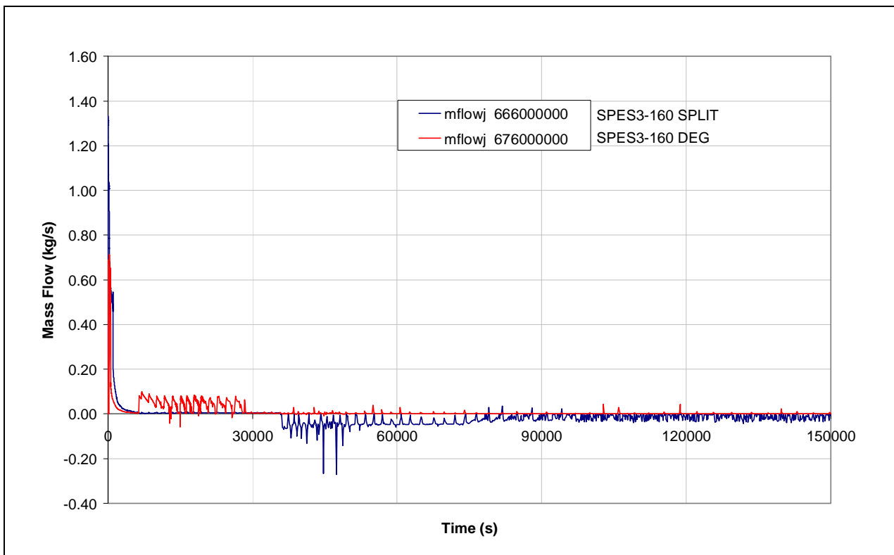
Fig.4.2 – SPES3-160 DVI line break flow
