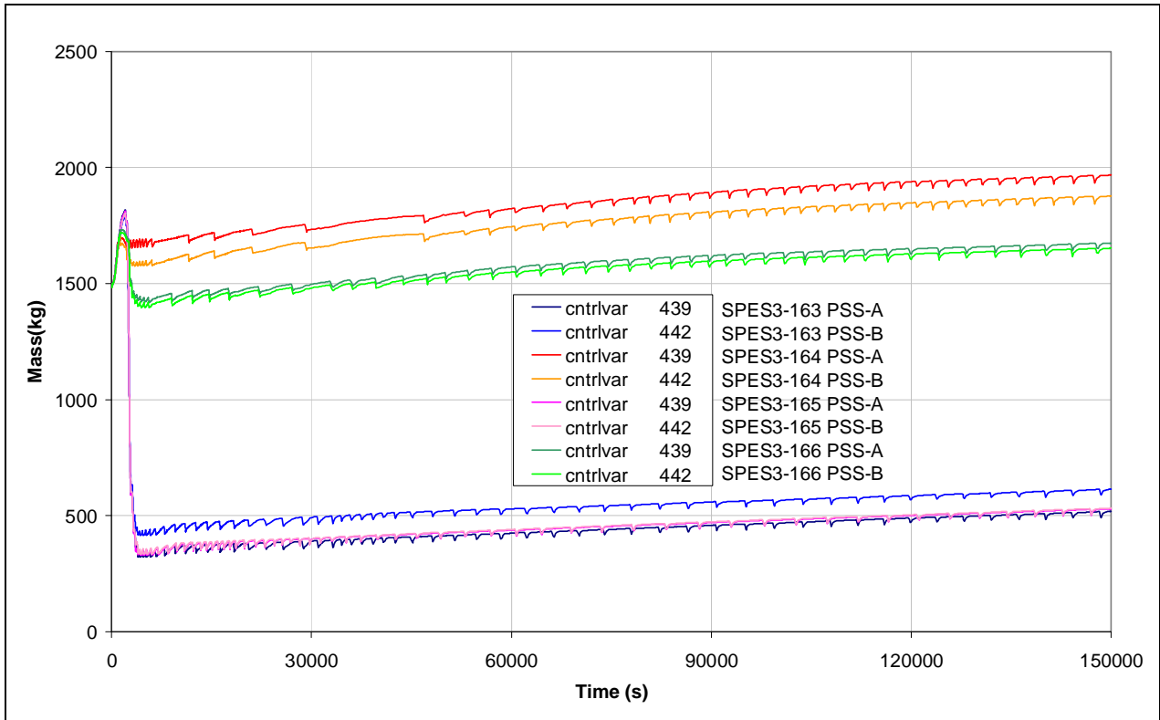
Fig.5. 21 – SPES3-163, 164, 165 and 166 PSS mass
