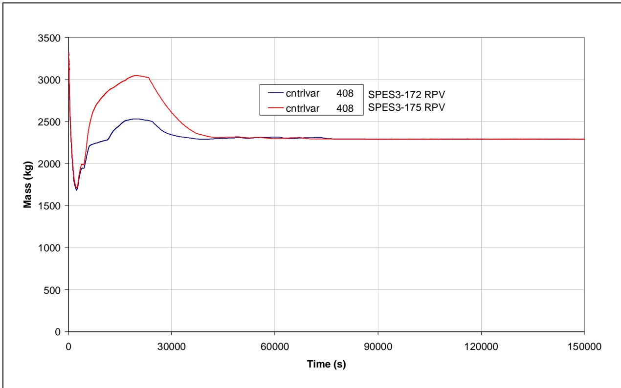
Fig.7. 53 - SPES3-172 and SPES3-175 RPV mass
