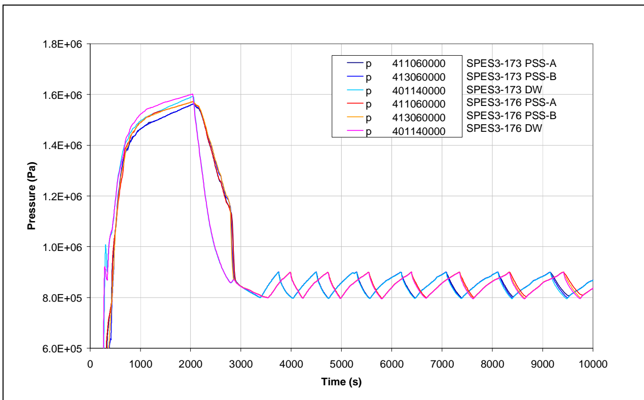
Fig.8. 30 – SPES3-173 and SPES3-176 PSS and DW pressure (window)
