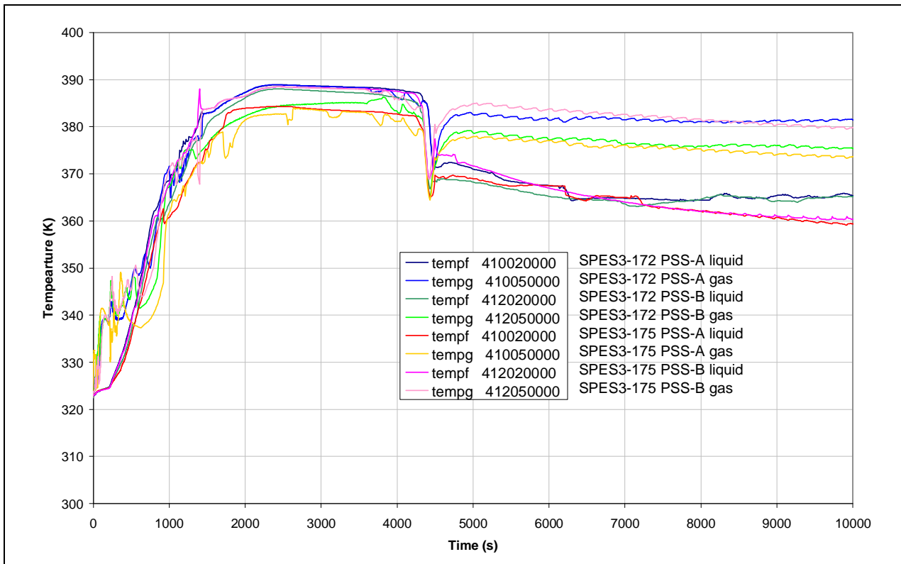
Fig.7. 29 - SPES3-172 and SPES3-175 PSS temperatures (window)
