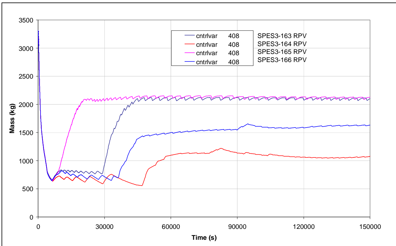
Fig.5. 26 – SPES3-163, 164, 165 and 166 RPV mass
