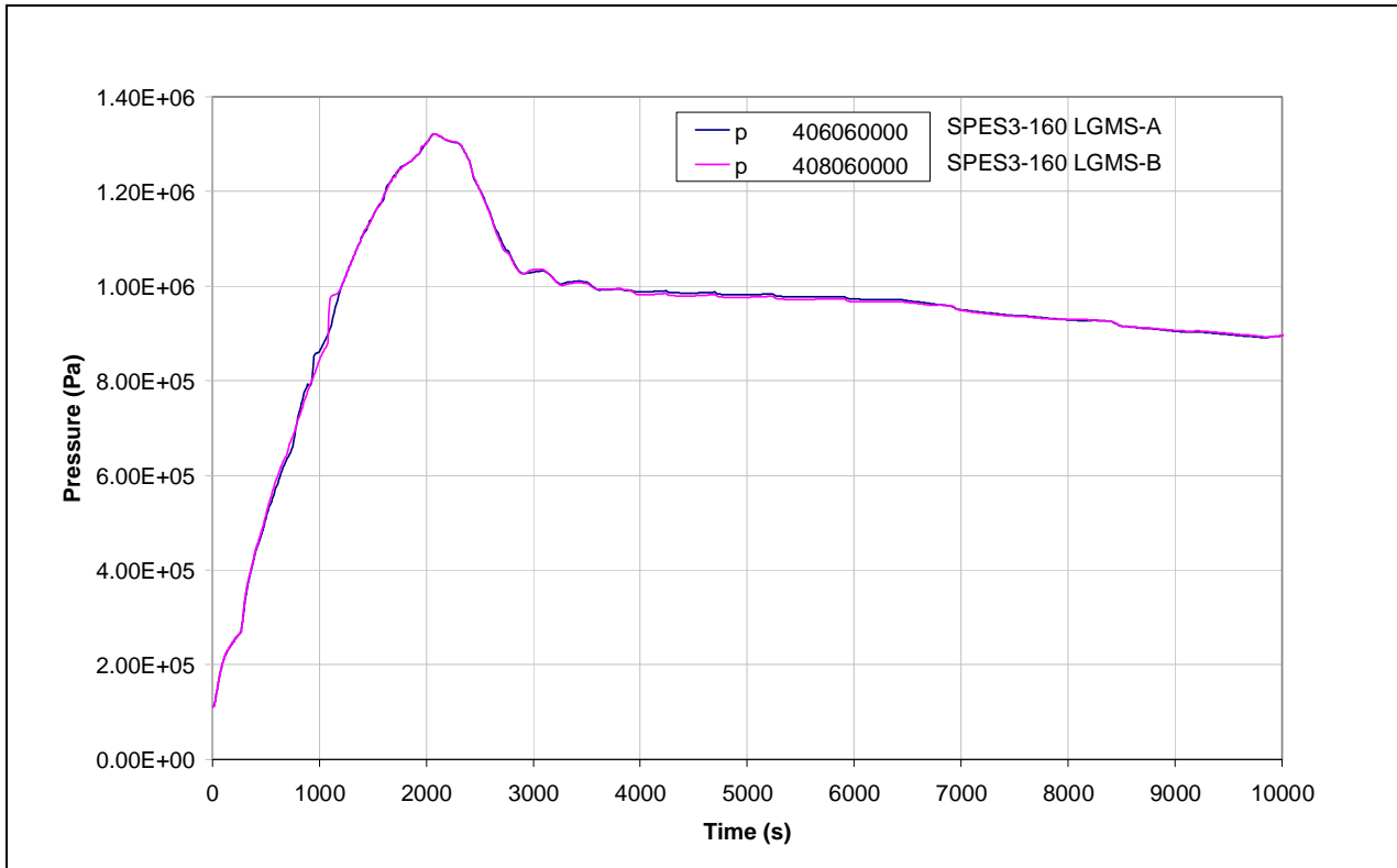
Fig.4.21 – SPES3-160 LGMS pressure (window)
