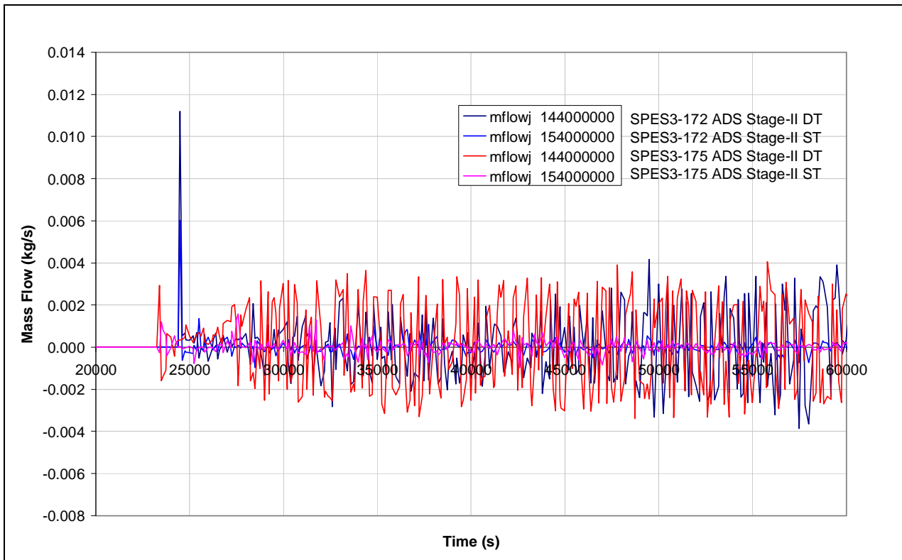
Fig.7. 72 - SPES3-172 and SPES3-175 ADS Stage-II mass flow (window)
