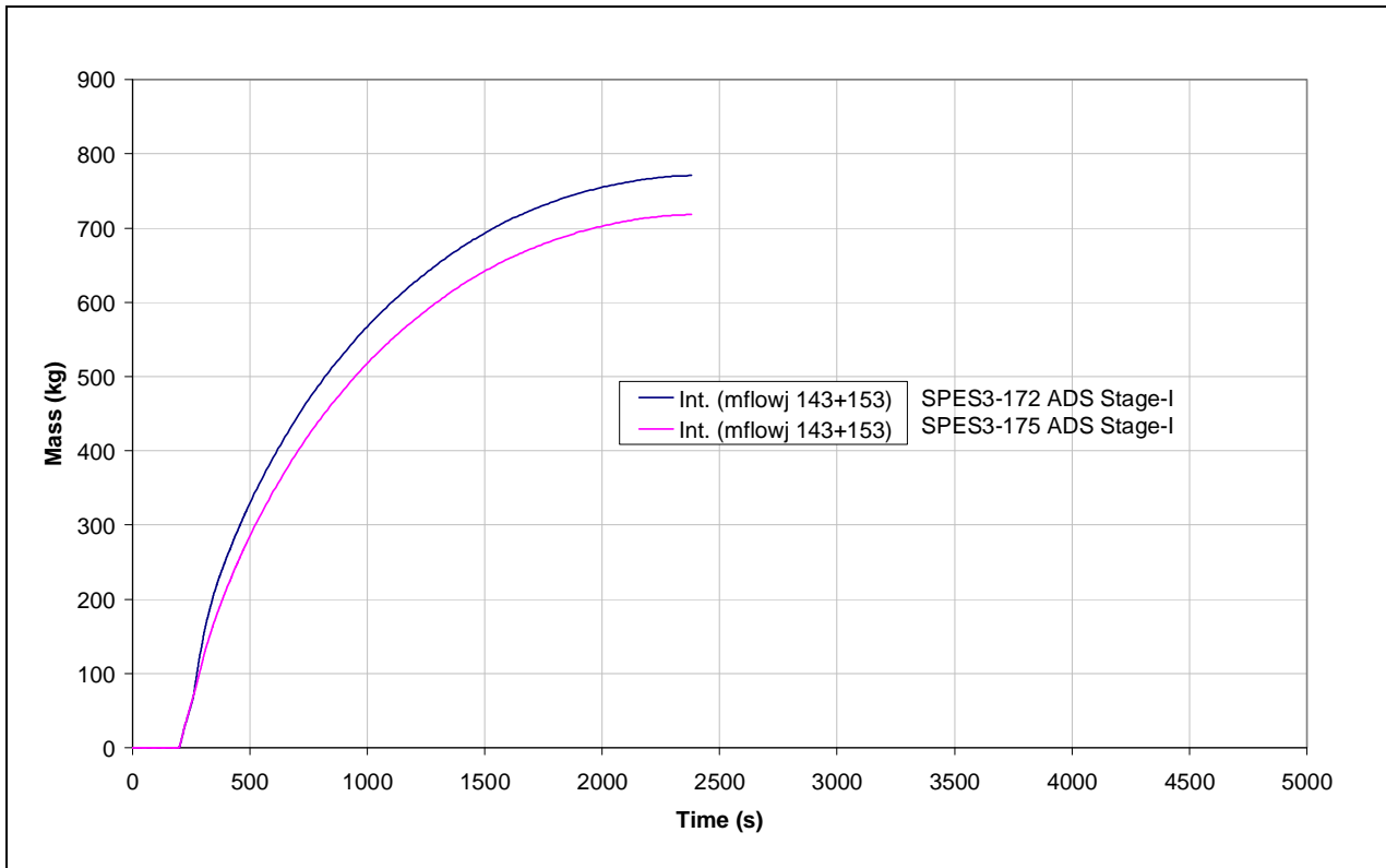
Fig.7. 55 - SPES3-172 and SPES3-175 ADS Stage-I integral flow
