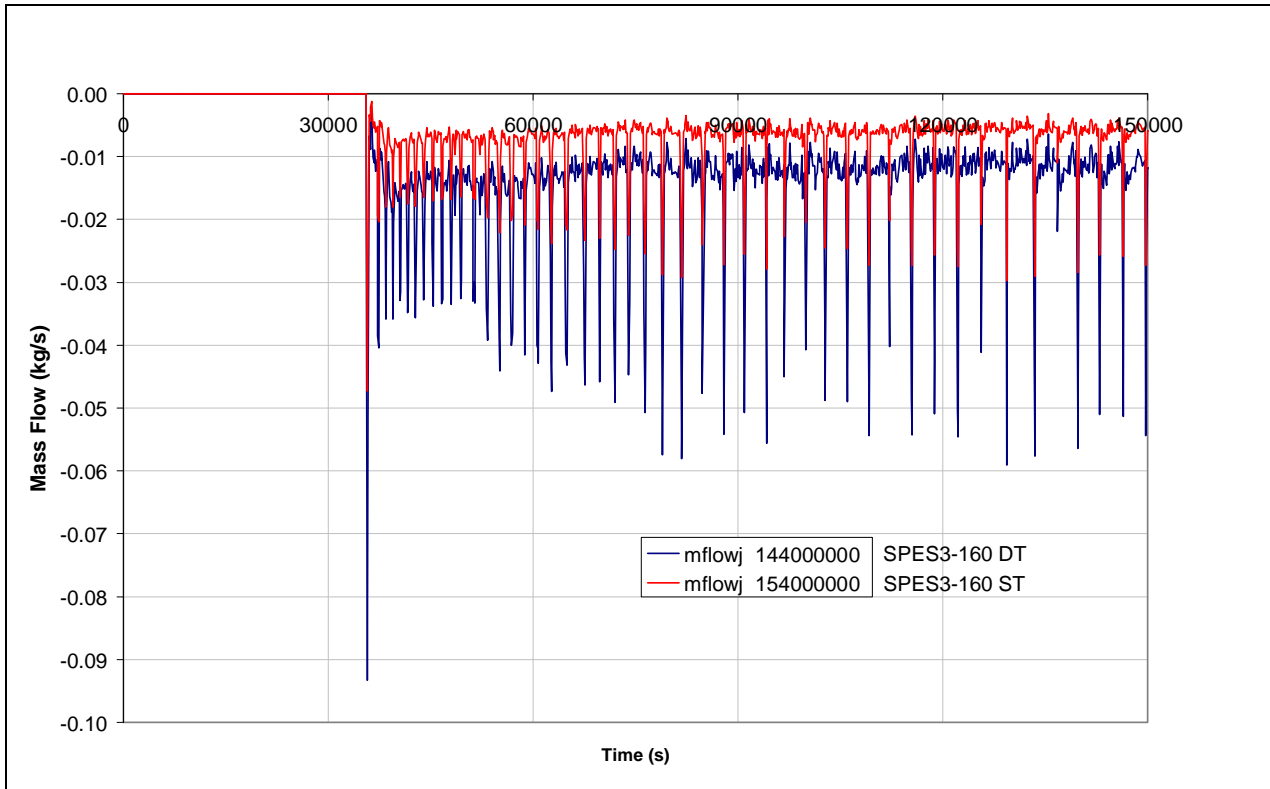
Fig.4.5 – SPES3-160 ADS Stage-II mass flow
