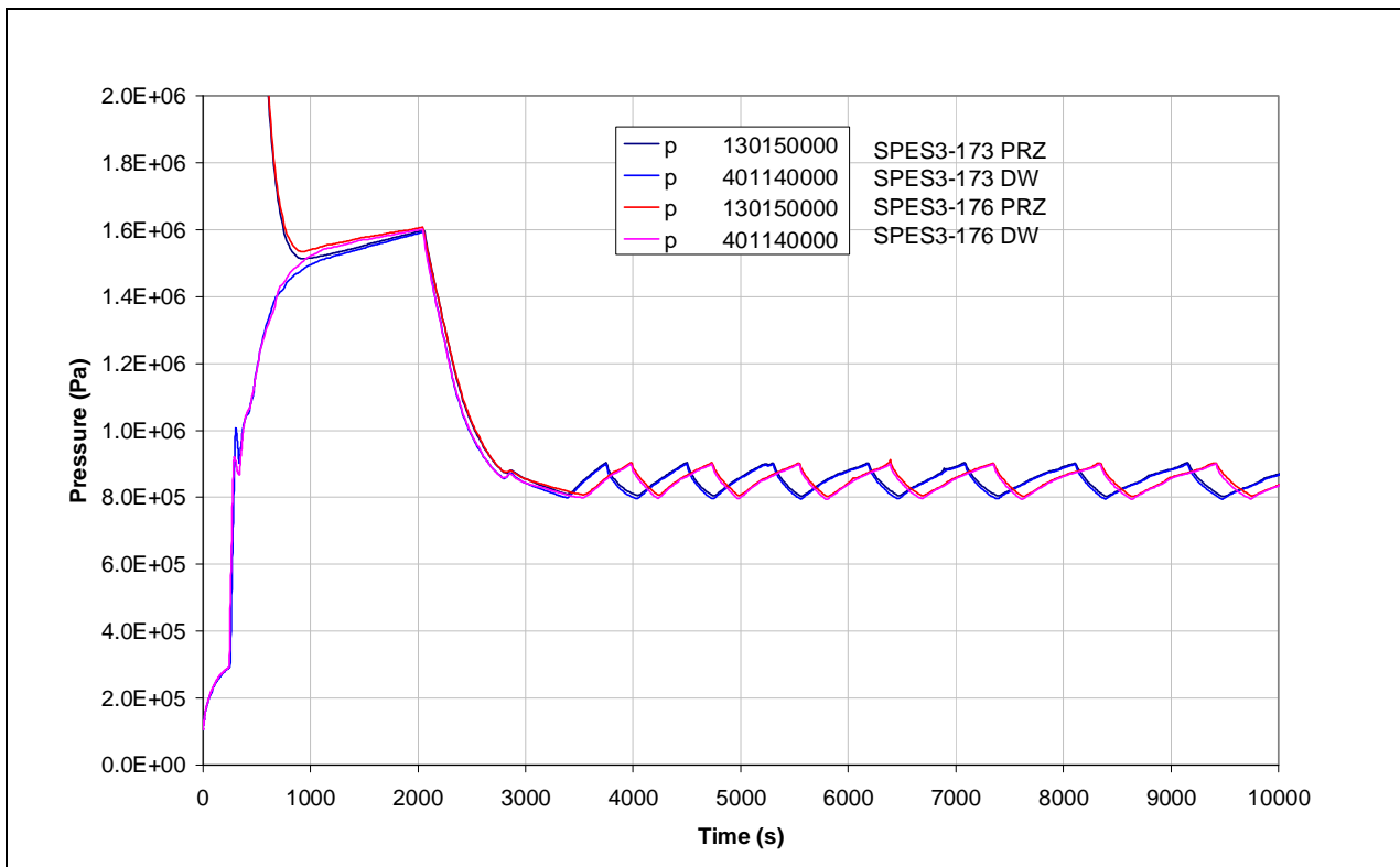
Fig.8. 12 – SPES3-173 and SPES3-176 PRZ and DW pressures (window)
