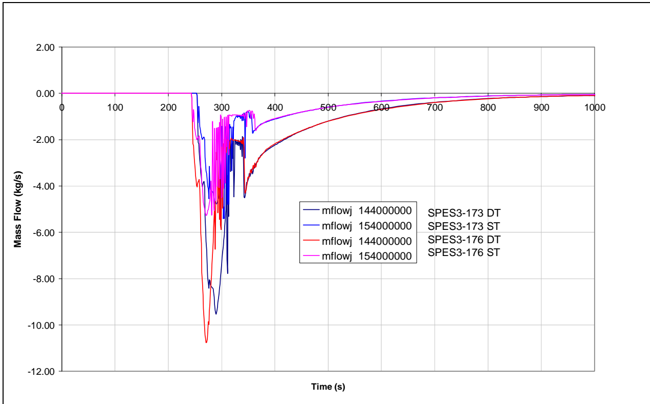
Fig.8. 9 – SPES3-173 and SPES3-176 ADS Stage-II mass flow (window)
