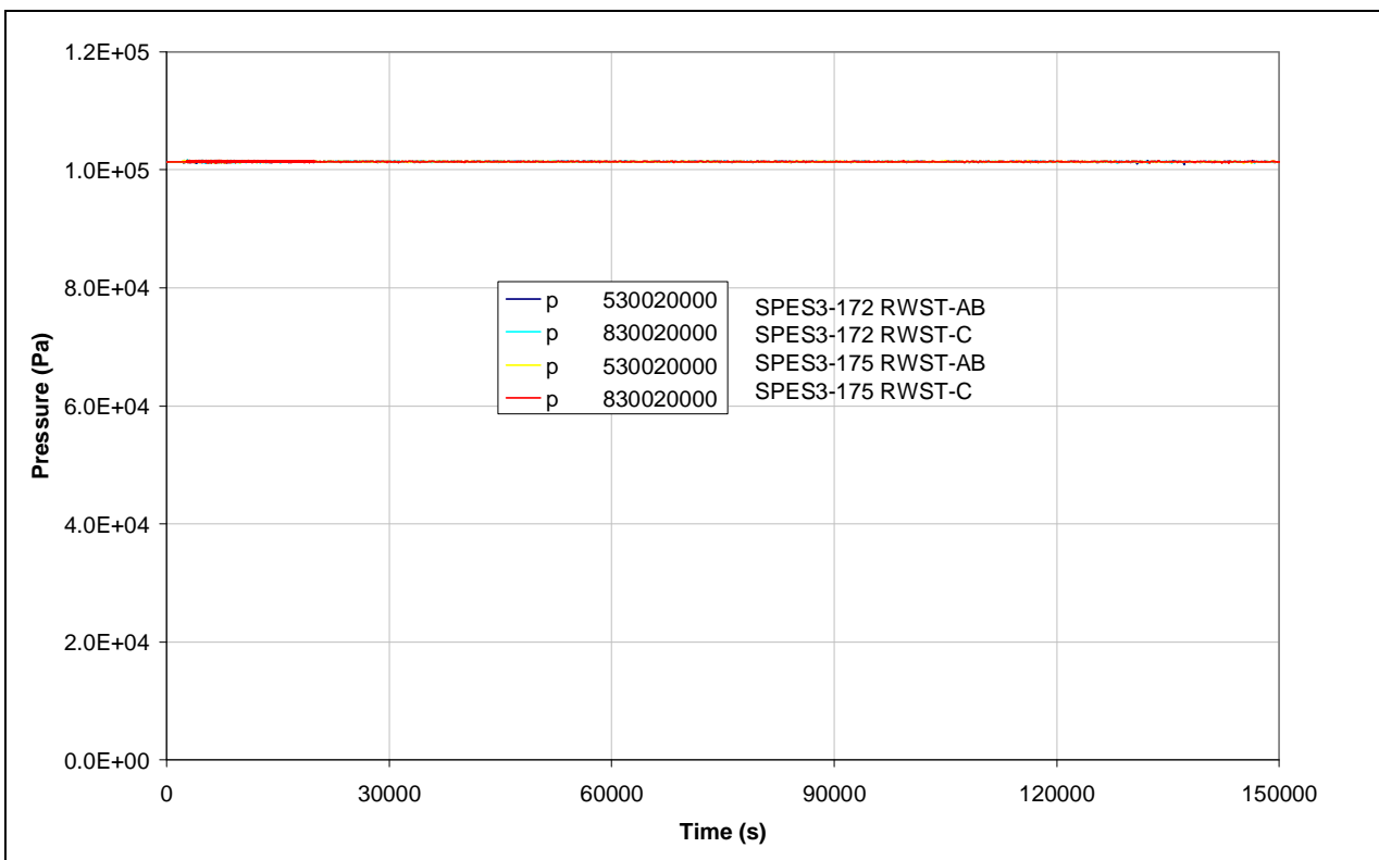
Fig.7. 76 - SPES3-172 and SPES3-175 RWST pressure
