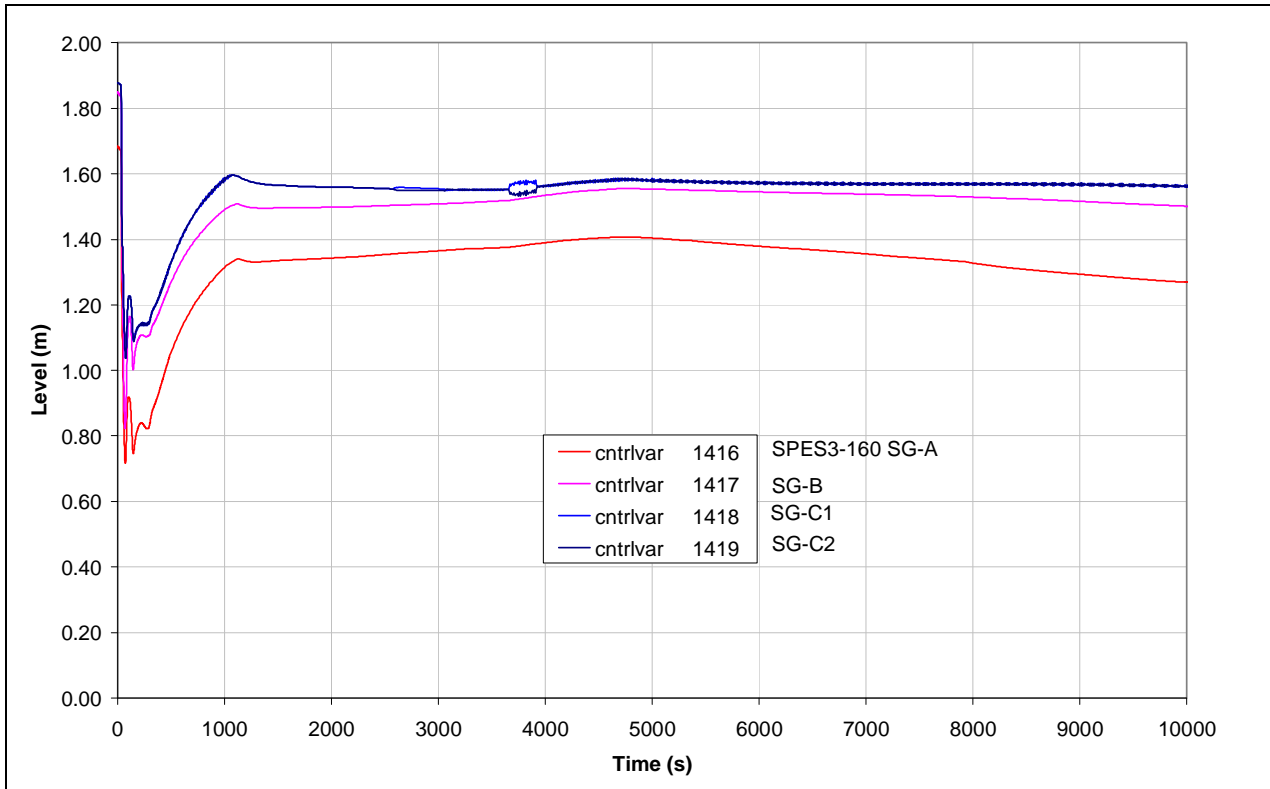
Fig.4.43 – SPES3-160 SG-A ss level (window)
