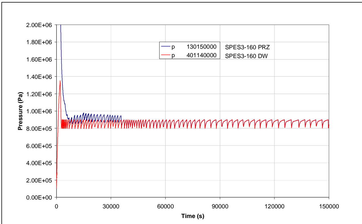
Fig.4.6 – SPES3-160 PRZ and DW pressures (window)
