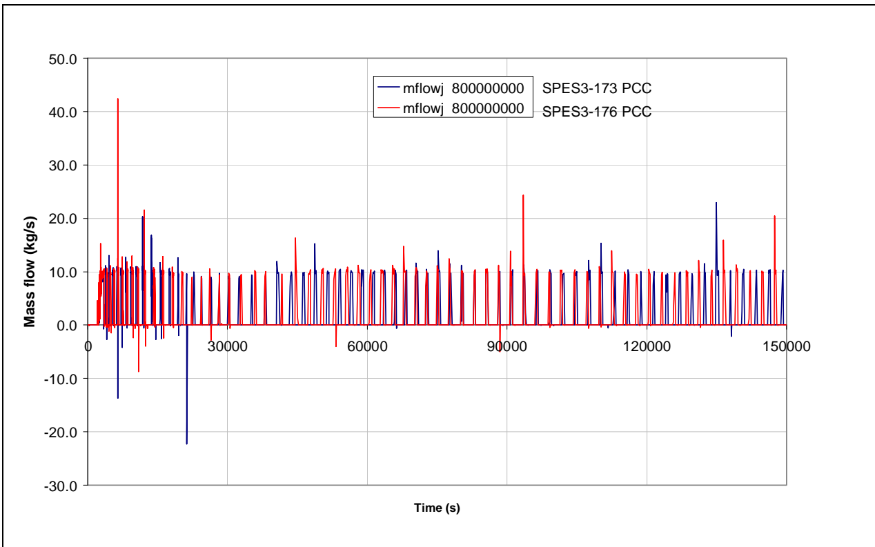
Fig.8. 75 – SPES3-173 and SPES3-176 PCC mass flow
