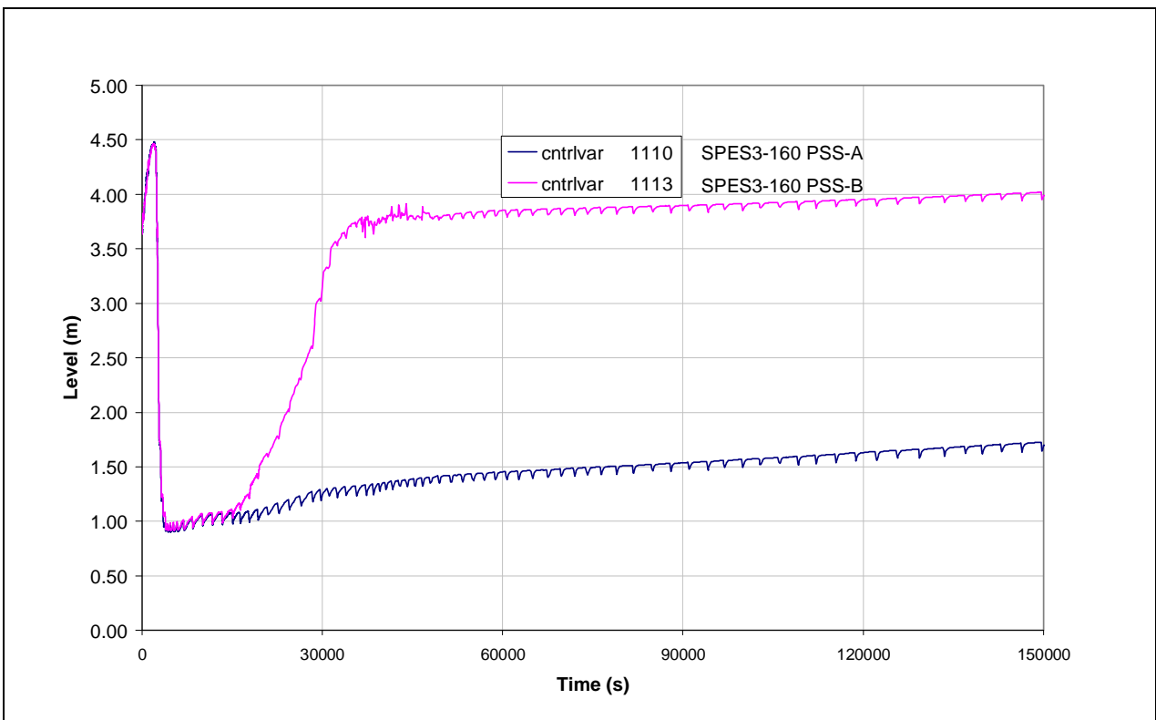
Fig.4.28 – SPES3-160 PSS level
