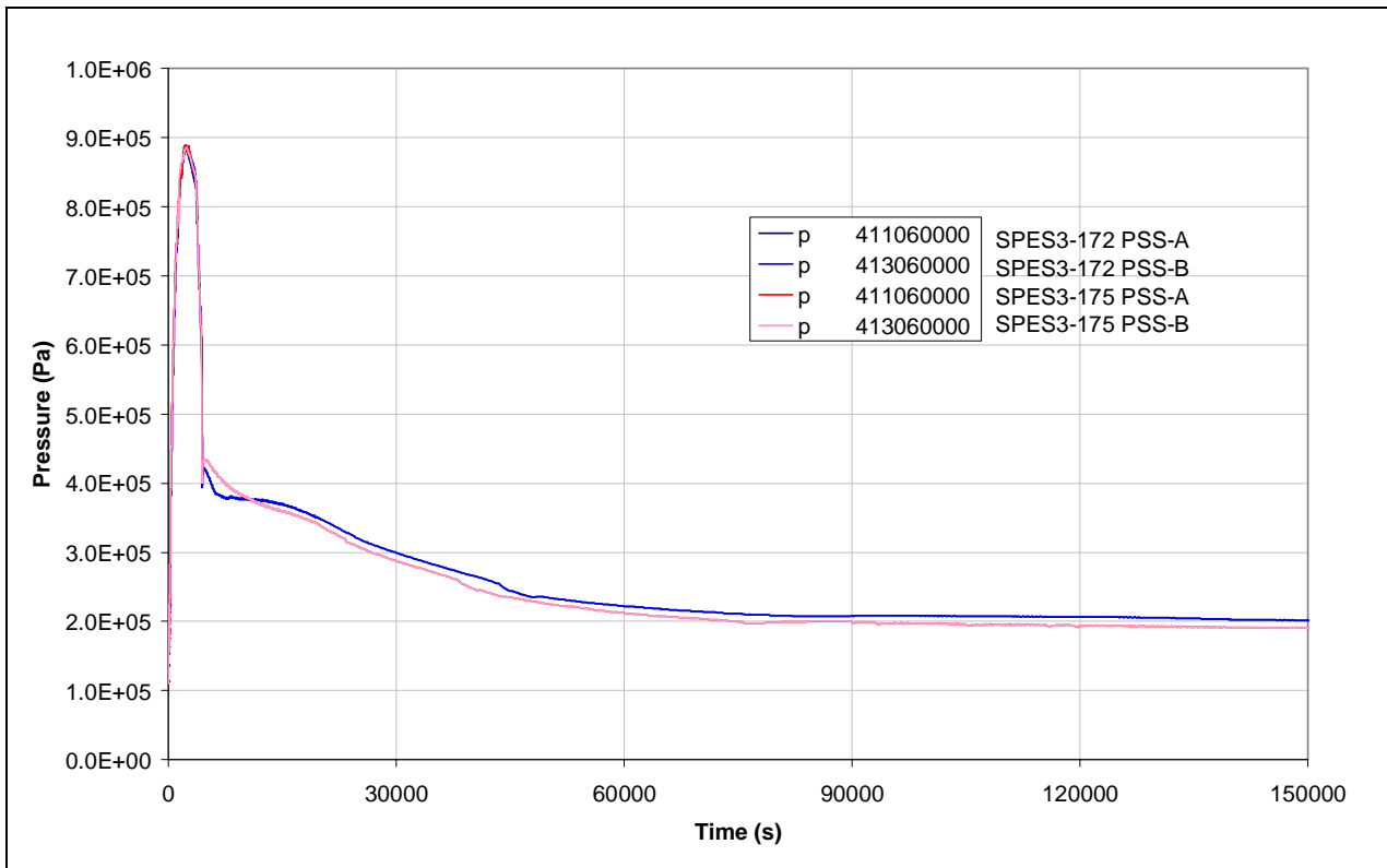
Fig.7. 23 - SPES3-172 and SPES3-175 PSS pressure
