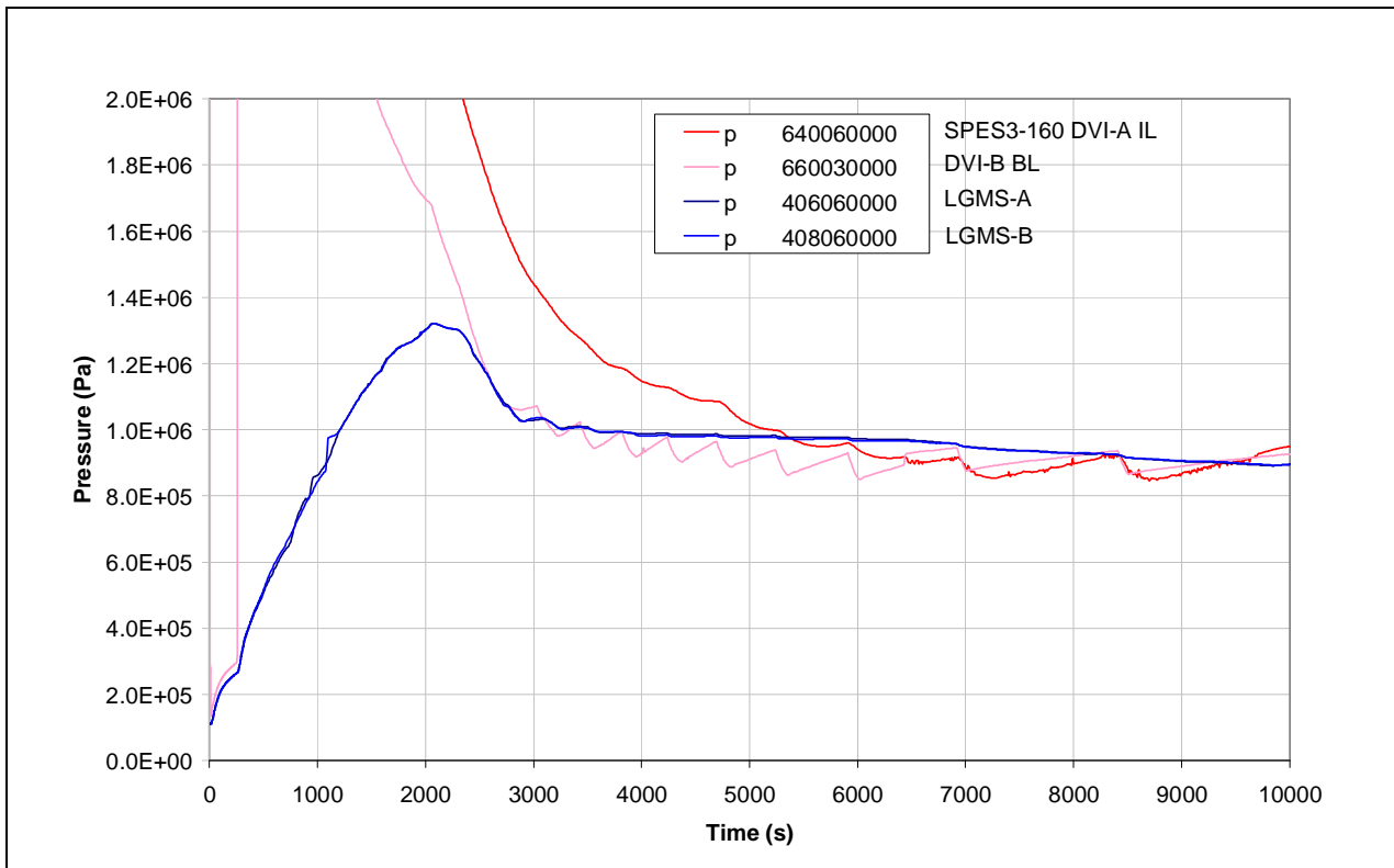
Fig.4.71 – SPES3-160 LGMS and DVI pressure (window)
