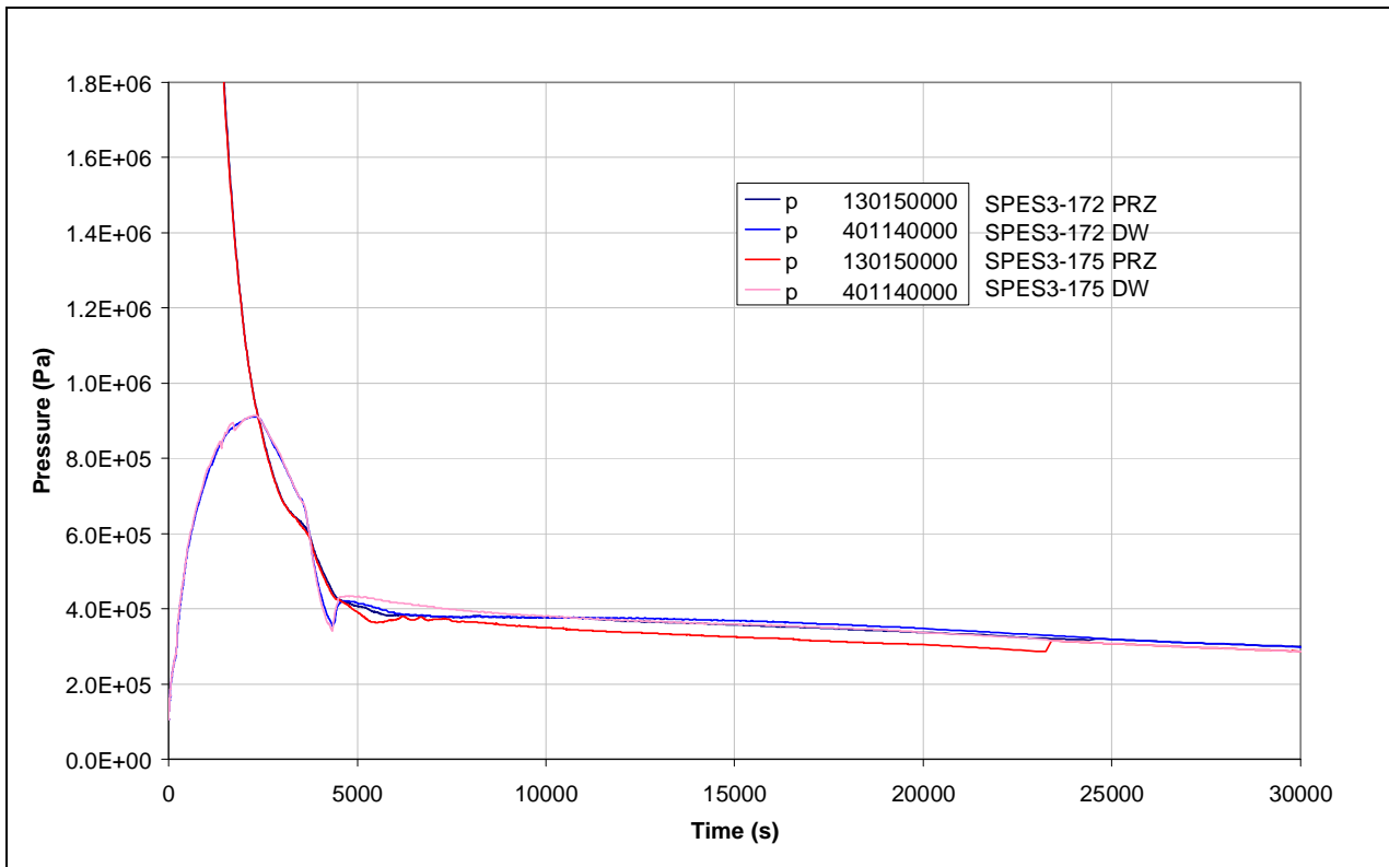
Fig.7. 15 - SPES3-172 and SPES3-175 PRZ and DW pressures (window)
