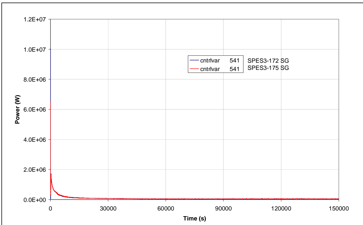
Fig.7. 34 - SPES3-172 and SPES3-175 SG power
