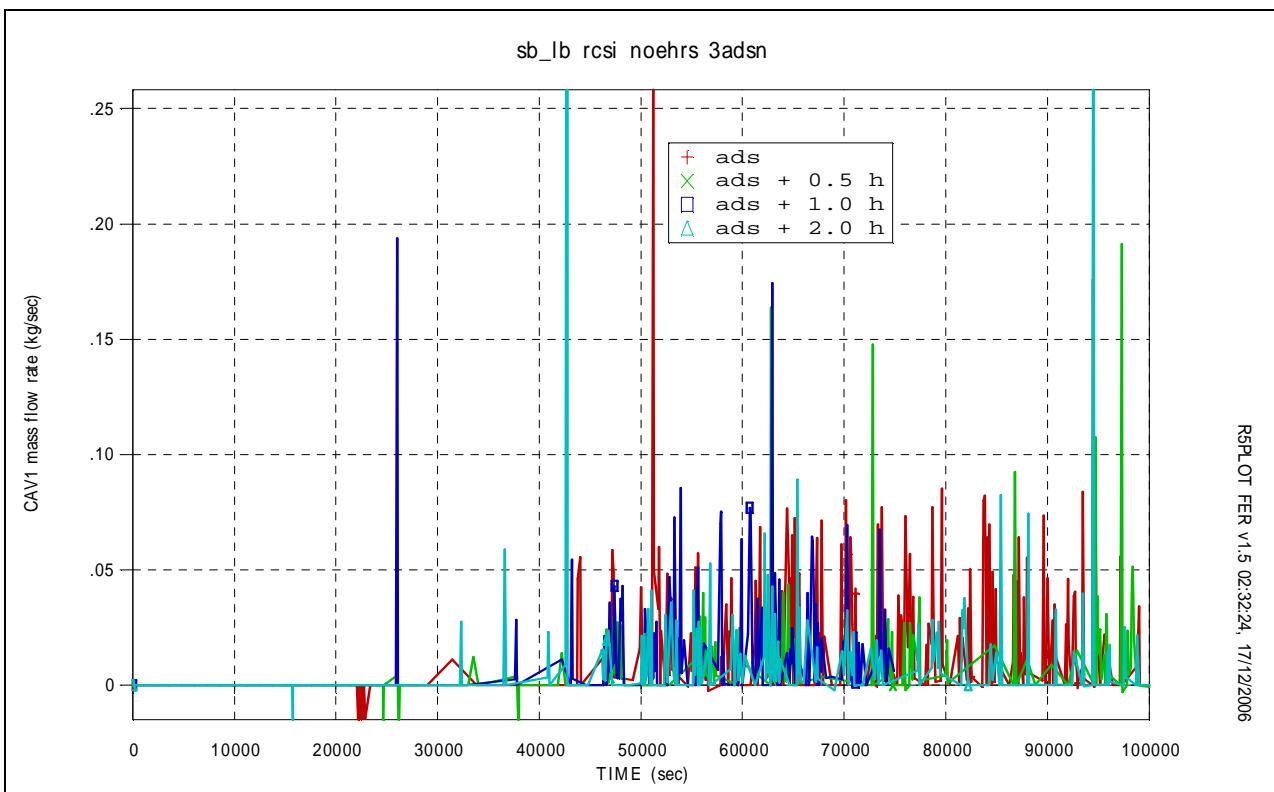
Fig.5. 34 – IRIS plant RC to DVI mass flow
