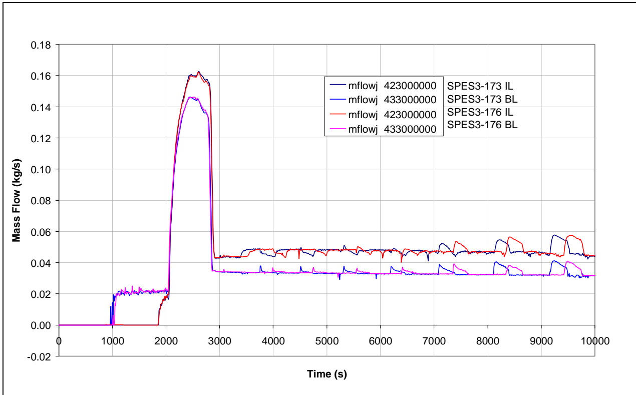
Fig.8. 5 – SPES3-173 and SPES3-176 LGMS injection mass flow (window)
