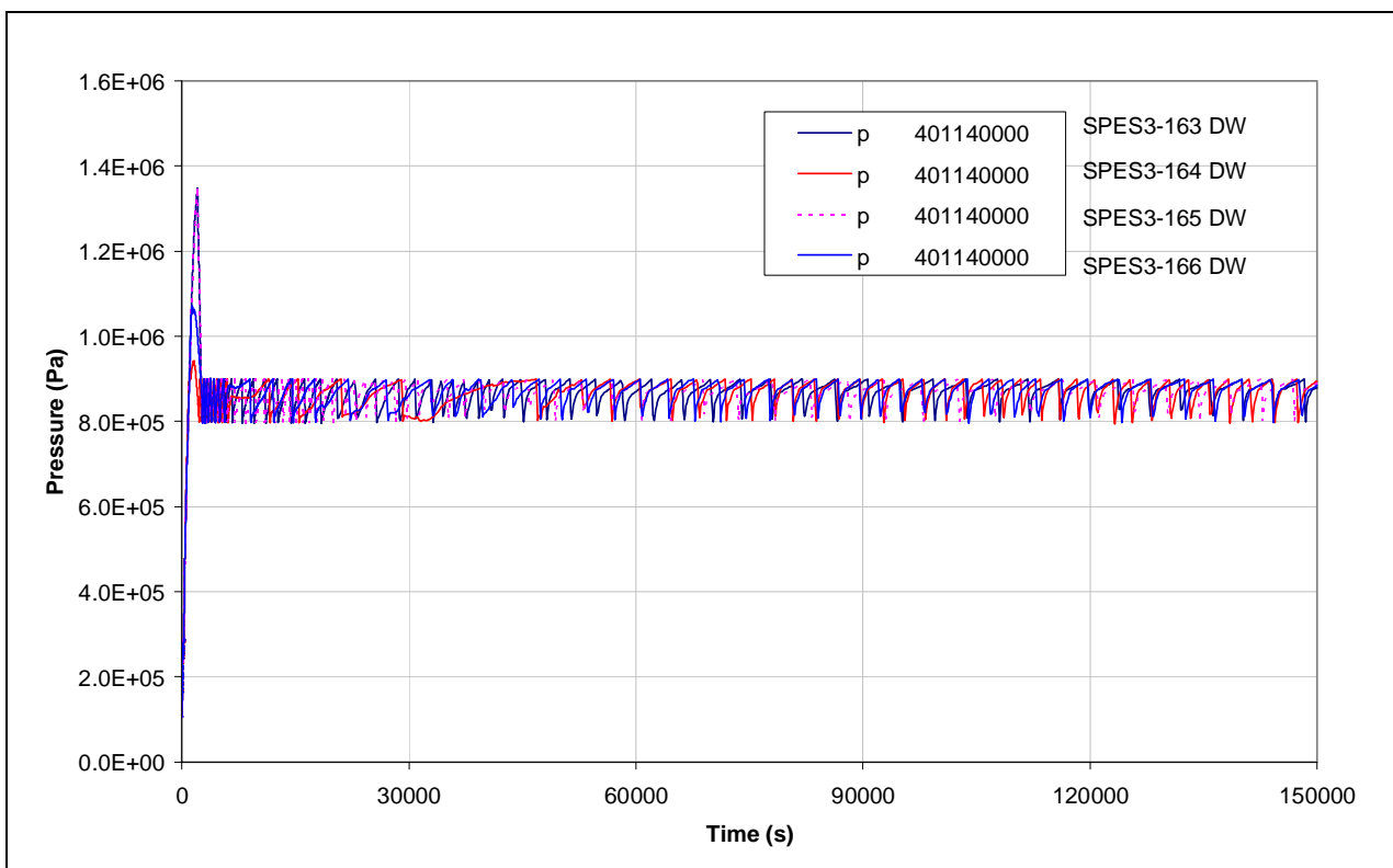
Fig.5. 16 – SPES3-163, 164, 165 and 166 DW pressure
