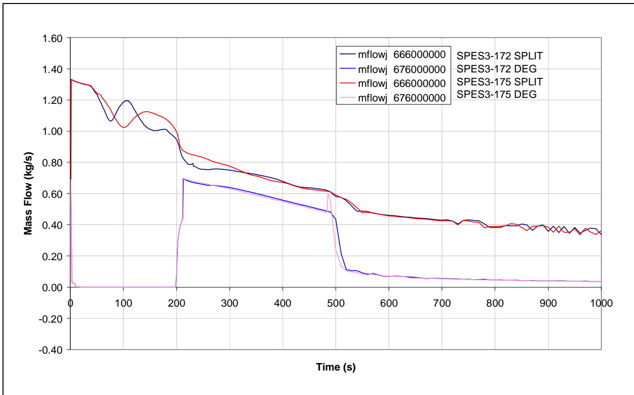
Fig.7. 1 - SPES3-172 and SPES3-175 DVI break mass flow (window)
