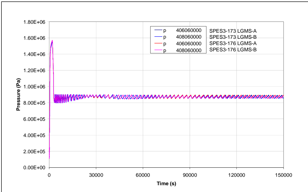
Fig.8. 29 – SPES3-173 and SPES3-176 LGMS pressure
