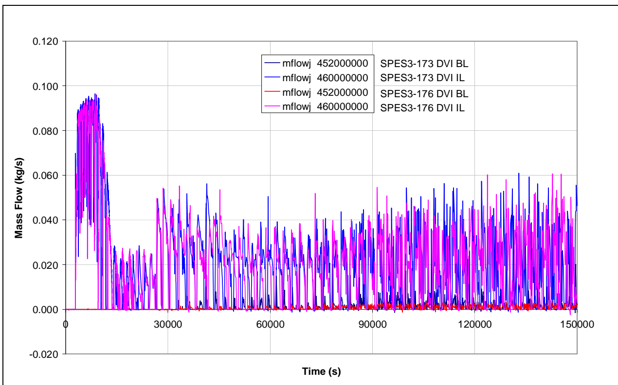
Fig.8. 66 – SPES3-173 and SPES3-176 RC to DVI line mass flow
