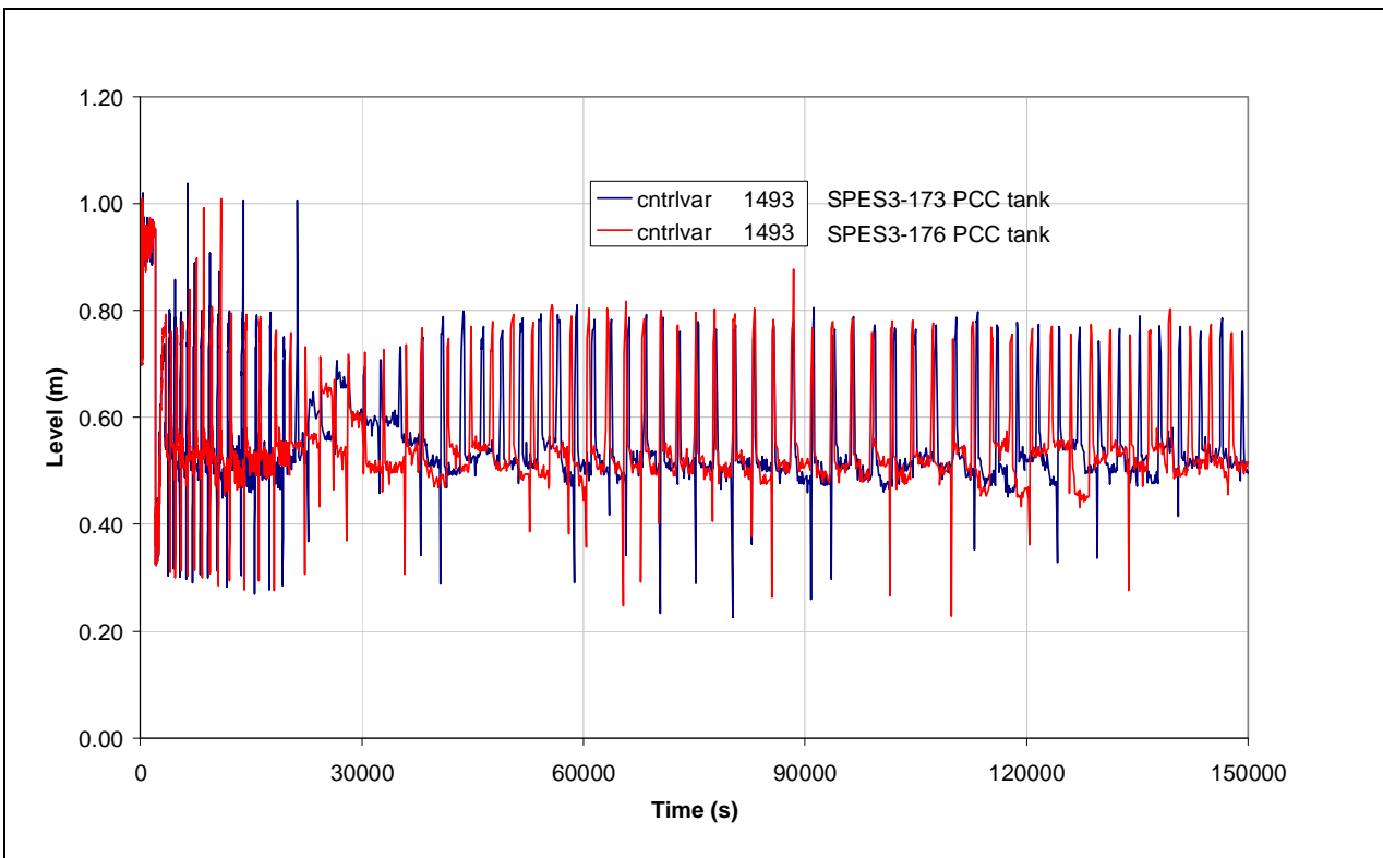
Fig.8. 76 – SPES3-173 and SPES3-176 PCC tank level
