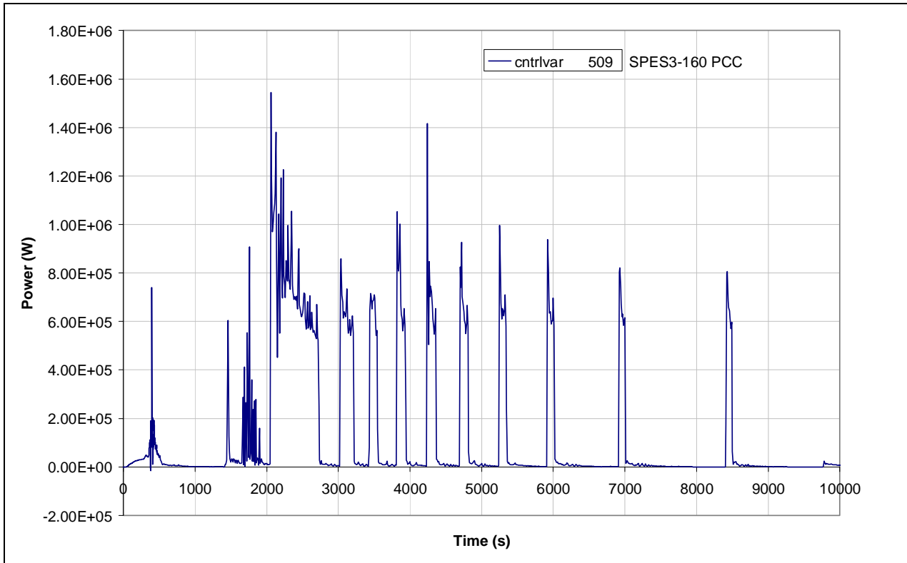
Fig.4.13 – SPES3-160 PCC power (window)
