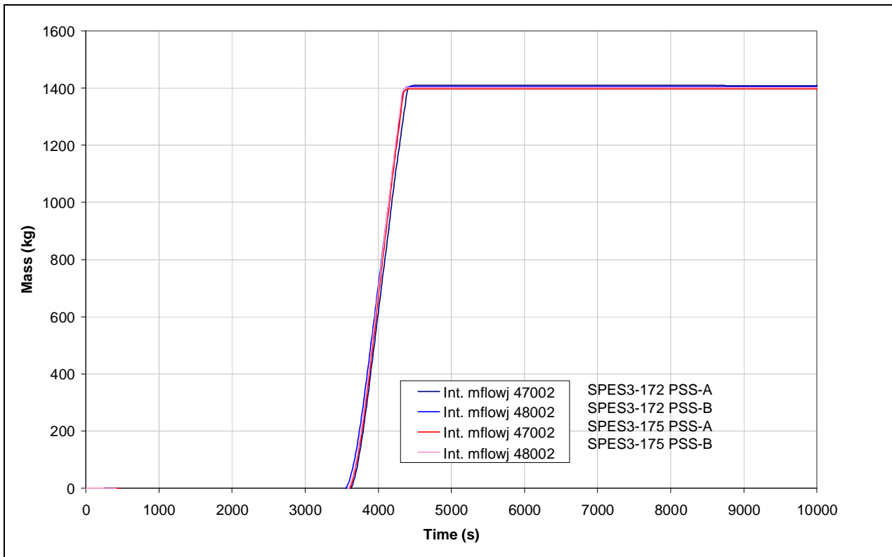
Fig.7. 19 - SPES3-172 and SPES3-175 PSS to DW integral flow (window)
