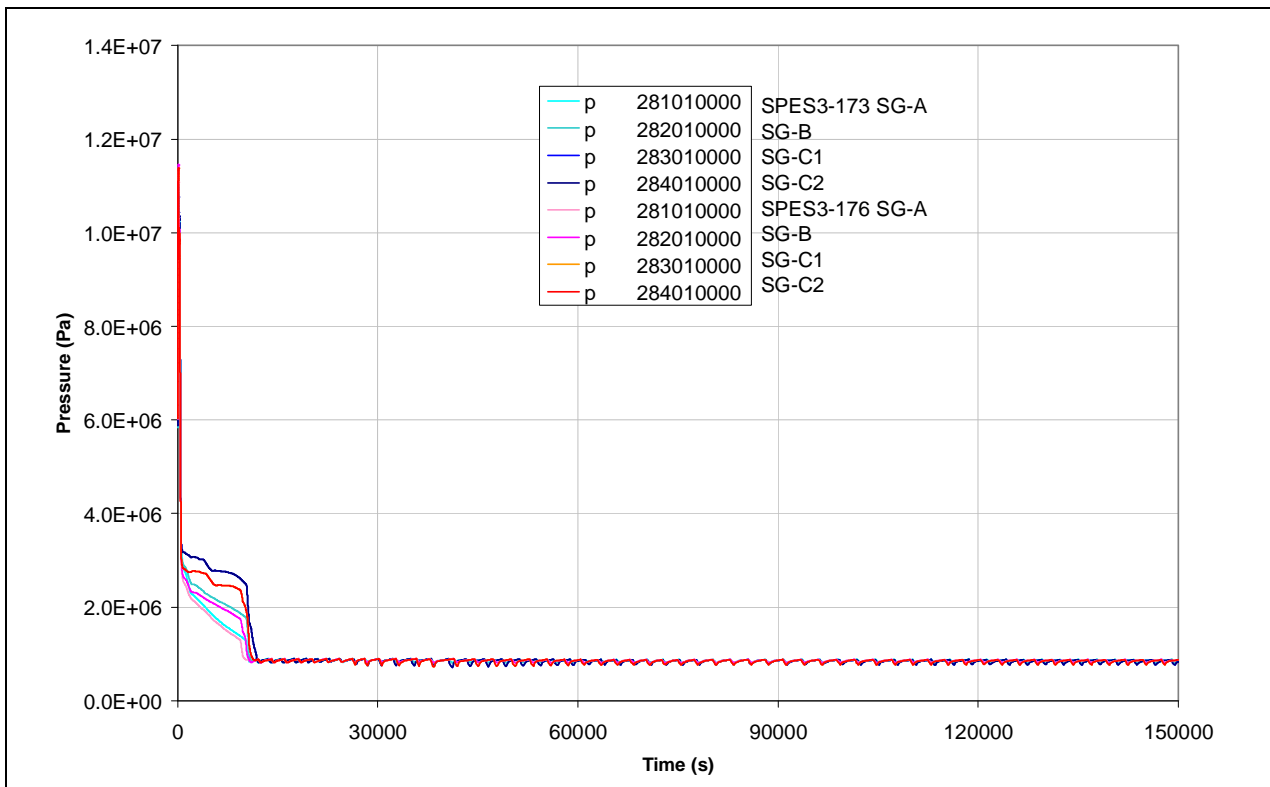
Fig.8. 50 – SPES3-173 and SPES3-176 SG ss outlet pressure
