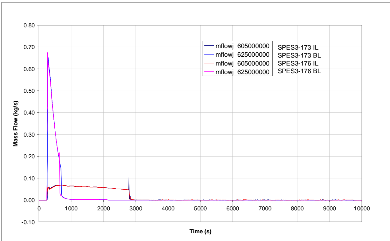
Fig.8. 4 – SPES3-173 and SPES3-176 EBT injection mass flow (window)
