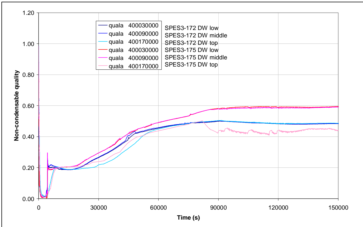
Fig.7. 21 - SPES3-172 and SPES3-175 DW non-condensable gas quality
