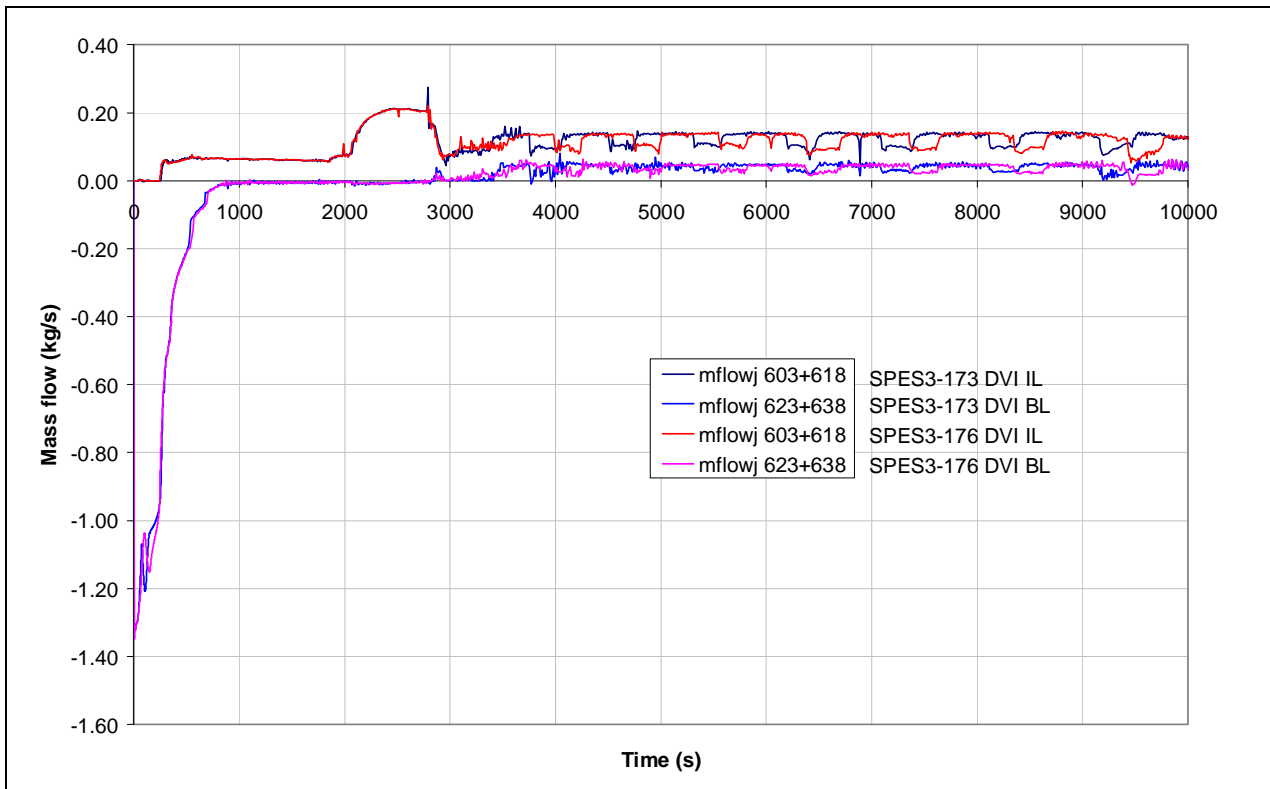
Fig.8. 67 – SPES3-173 and SPES3-176 DVI line mass flow (window)
