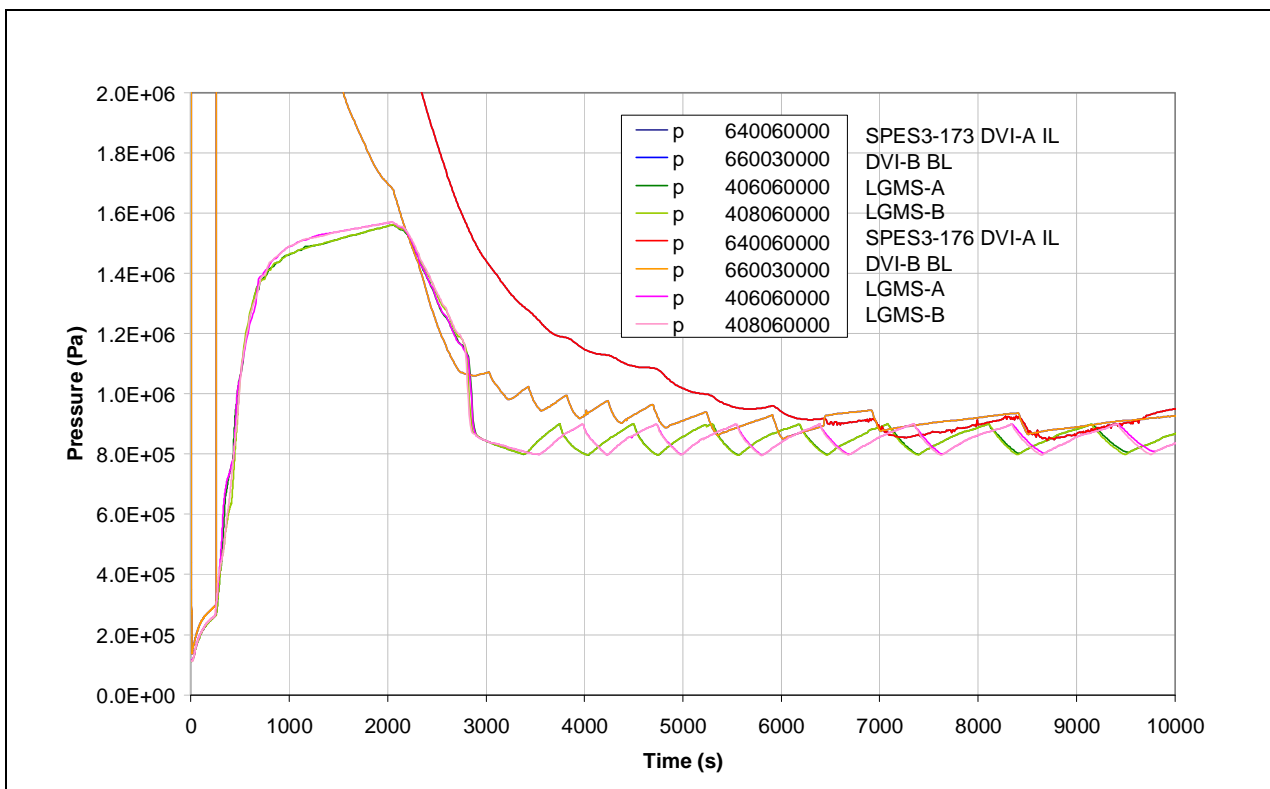
Fig.8. 82 – SPES3-173 and SPES3-176 LGMS and DVI pressure (window)
