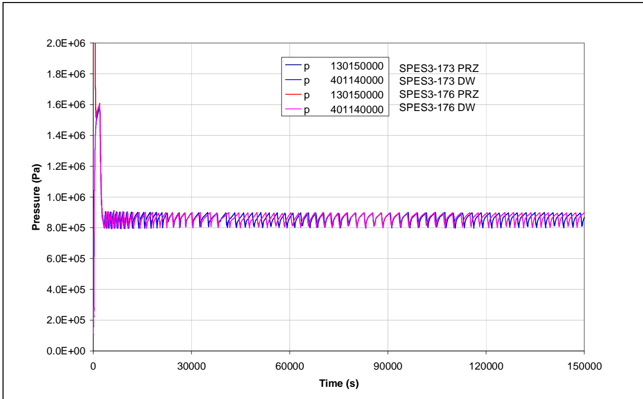
Fig.8. 13 – SPES3-173 and SPES3-176 PRZ and DW pressures (window)
