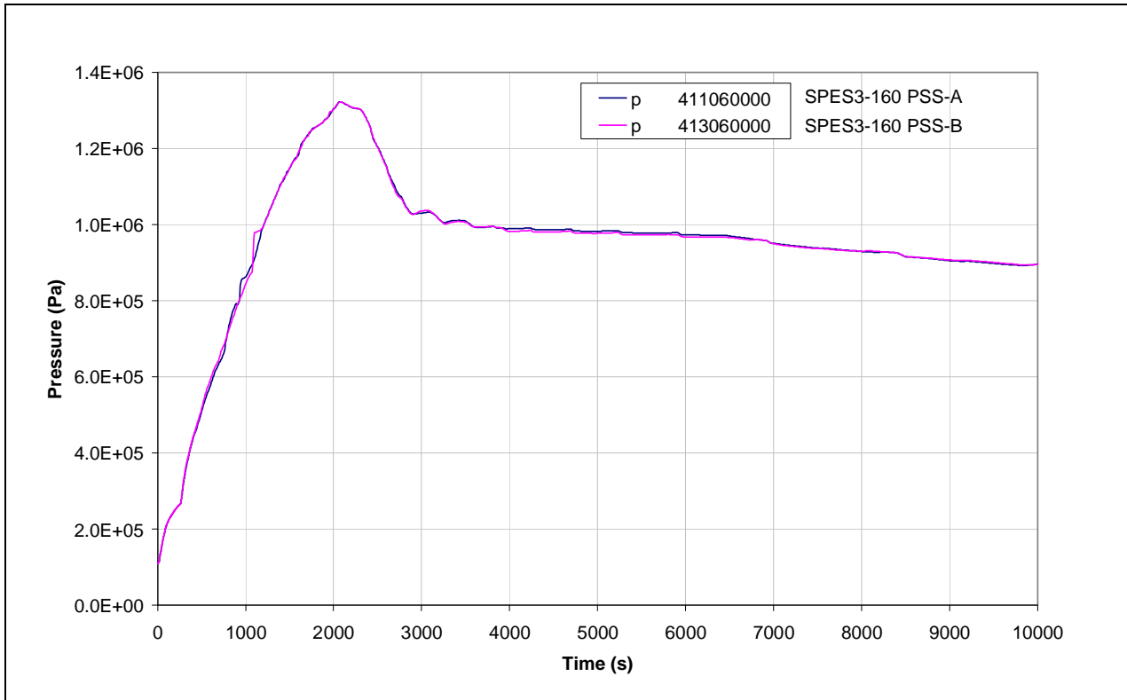
Fig.4.19 – SPES3-160 PSS pressure (window)
