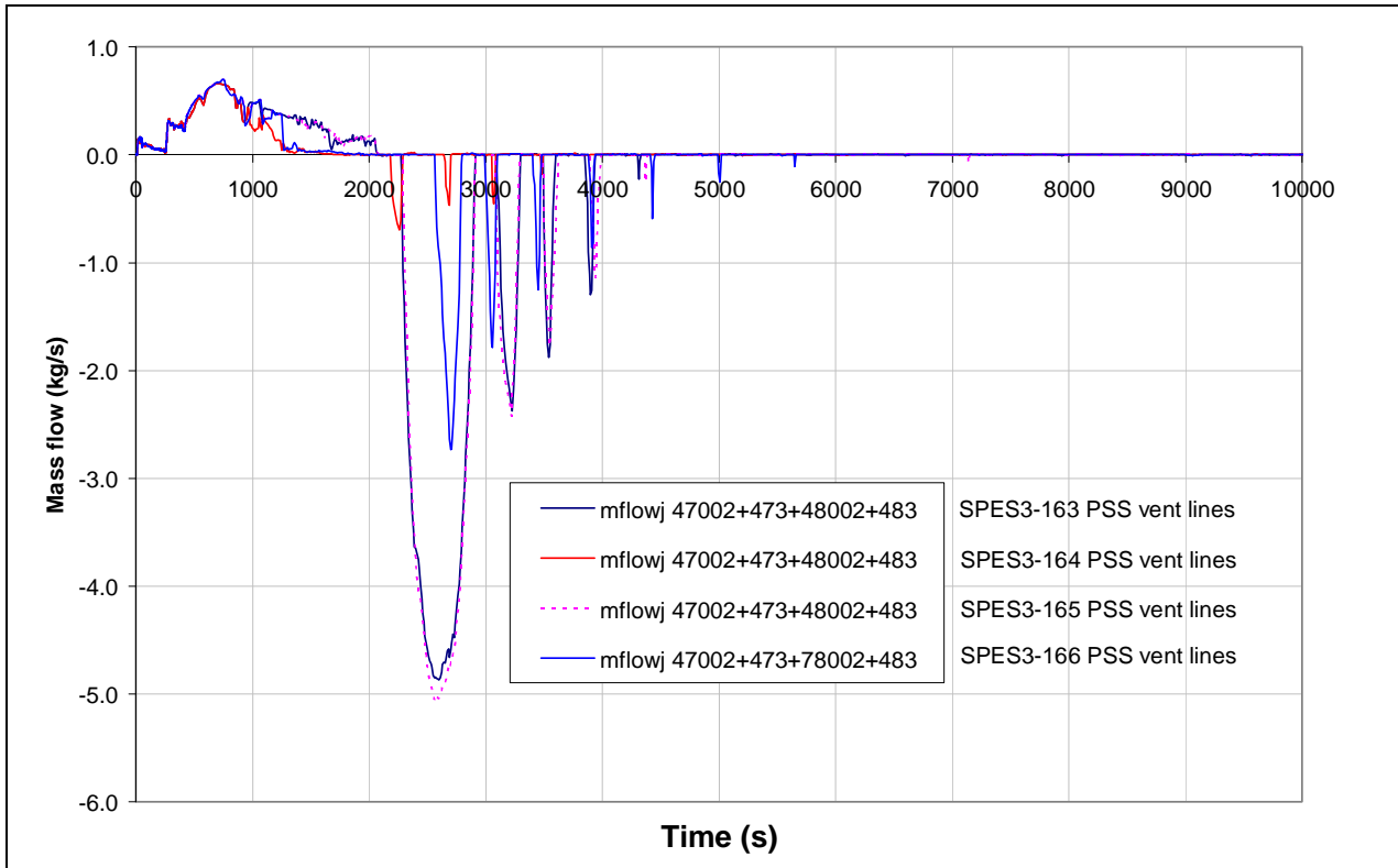
Fig.5. 19 – SPES3-163, 164, 165 and 166 PSS to DW mass flow (window)
