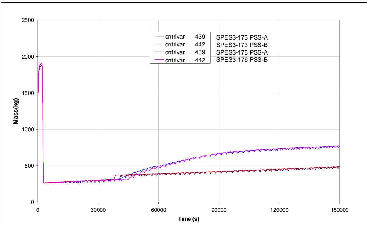
Fig.8. 36 – SPES3-173 and SPES3-176 PSS mass
