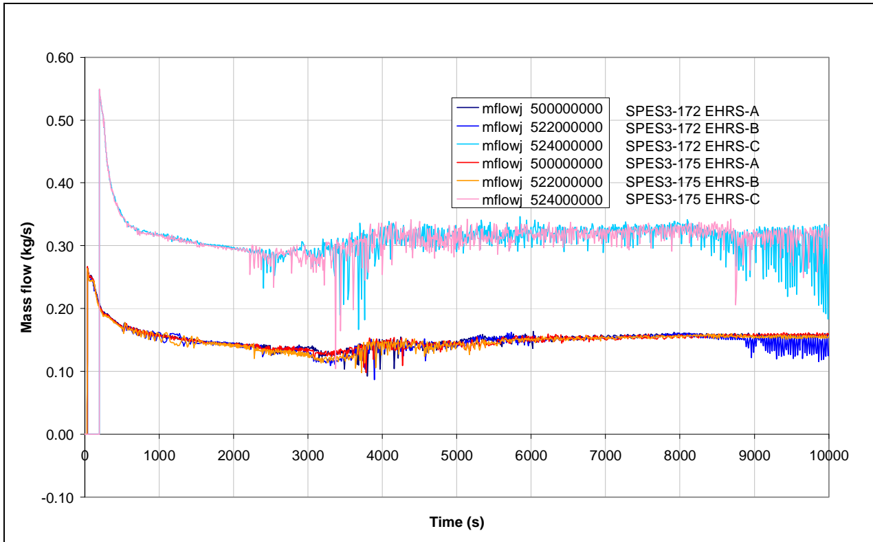
Fig.7. 37 - SPES3-172 and SPES3-175 EHRs cold leg mass flow (window)
