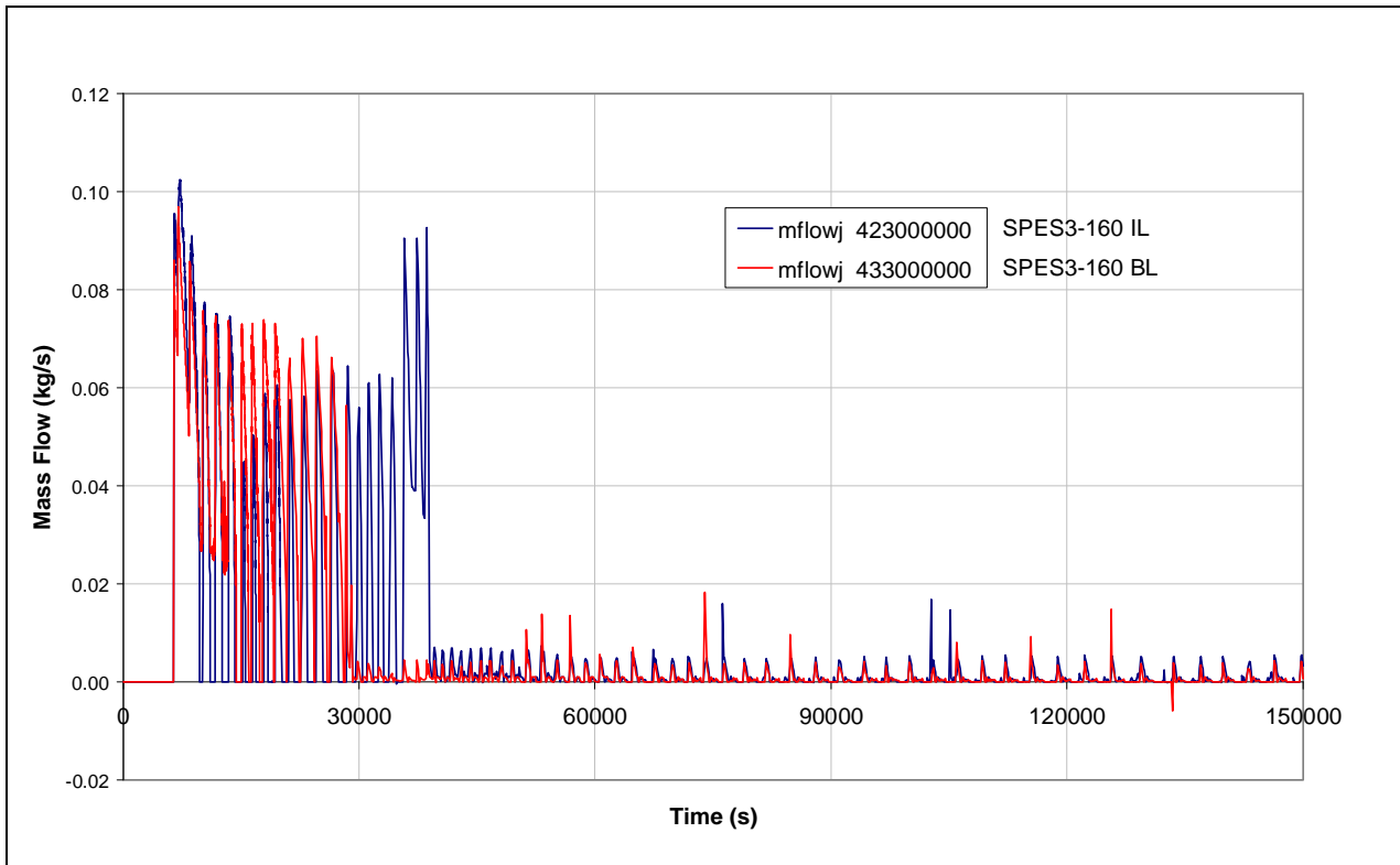
Fig.4.4 – SPES3-160 LGMS injection mass flow
