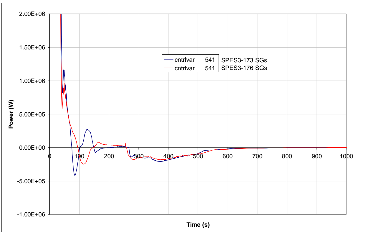
Fig.8. 46 – SPES3-173 and SPES3-176 SG power (window)
