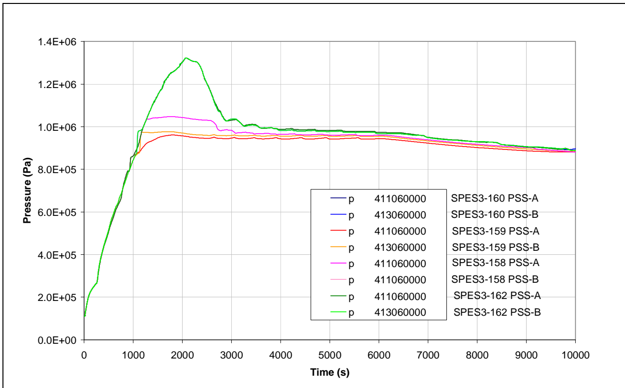
Fig.5. 3 – SPES3-159, 162, 158 and 160 PSS pressure (window)
