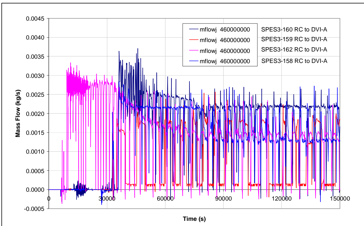
Fig.5. 10 – SPES3-159, 162, 158 and 160 RC to DVI line mass flow (intact loop)
