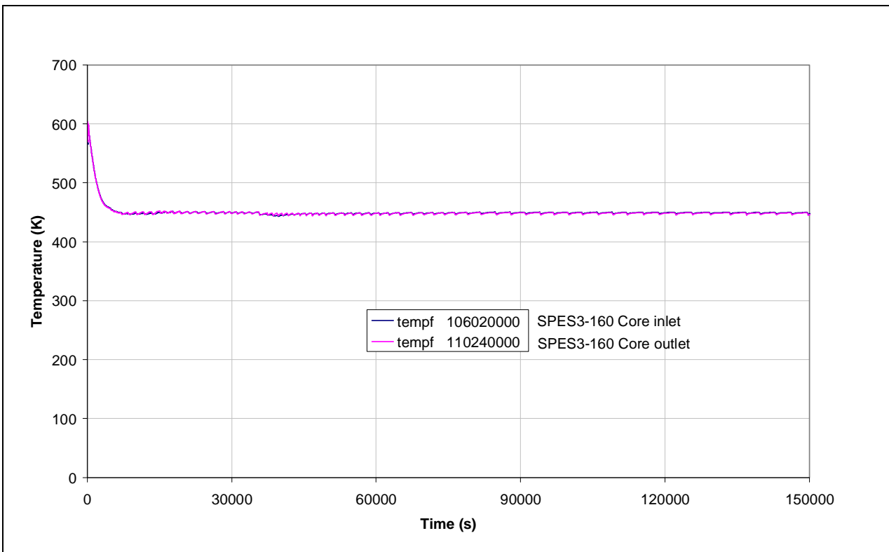
Fig.4.58 – SPES3-160 Core inlet and outlet temperatures
