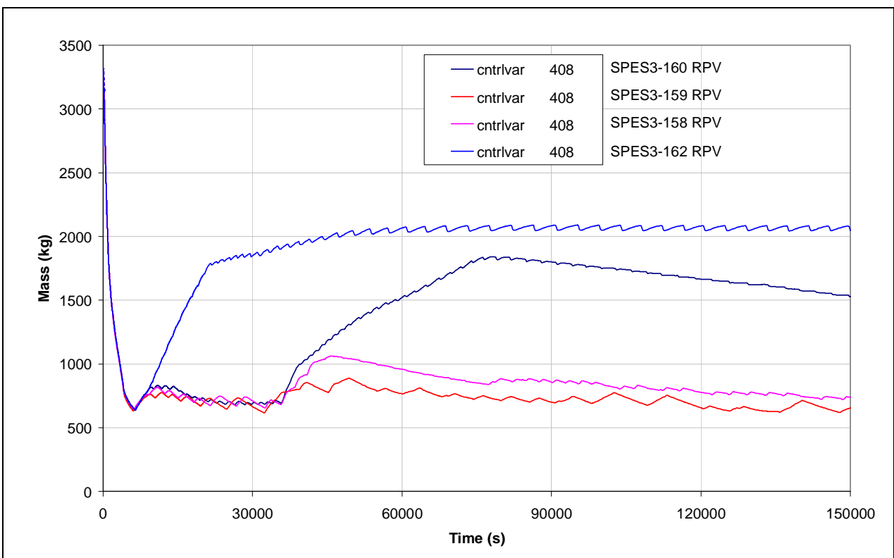
Fig.5. 12 – SPES3-159, 162, 158 and 160 RPV mass
