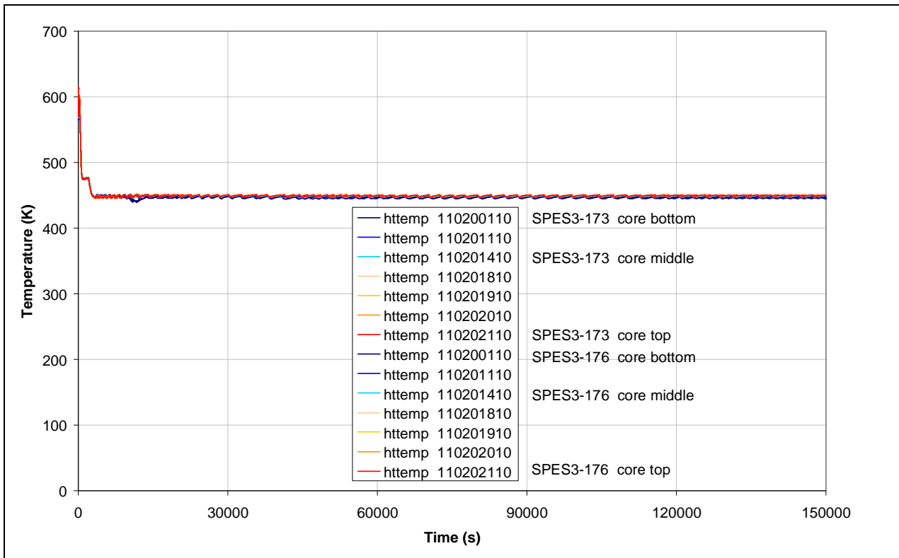
Fig.8. 74 – SPES3-173 and SPES3-176 Core heater rod clad surface temperatures (hot rods)
