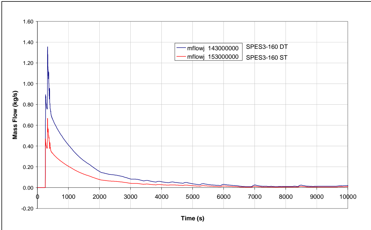
Fig.4.11 – SPES3-160 ADS Stage-I mass flow (window)
