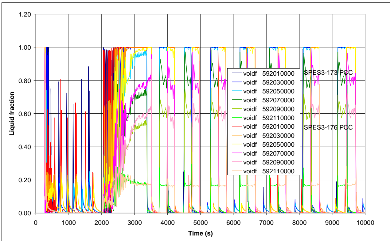
Fig.8. 78 – SPES3-173 and SPES3-176 PCC liquid void fraction (window)
