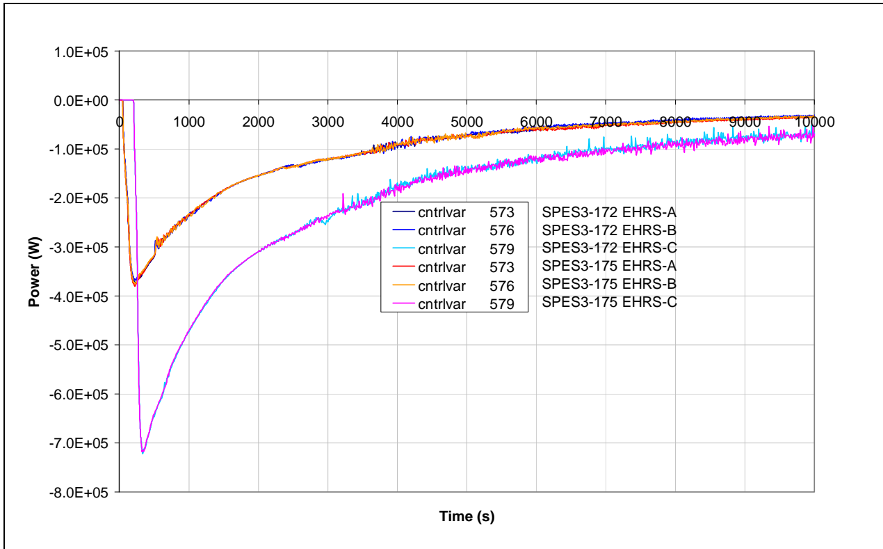
Fig.7. 39 - SPES3-172 and SPES3-175 EHR power (window)
