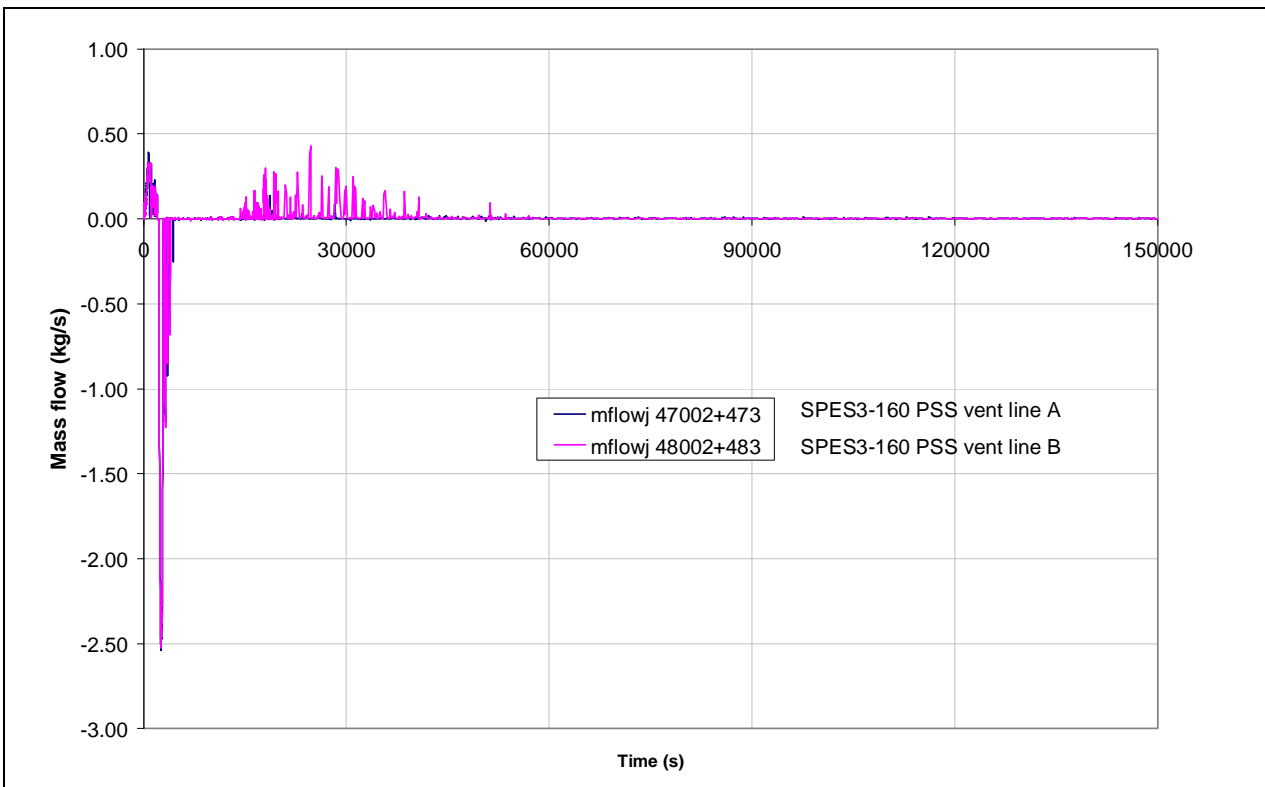
Fig.4.16 – SPES3-160 PSS to DW flow
