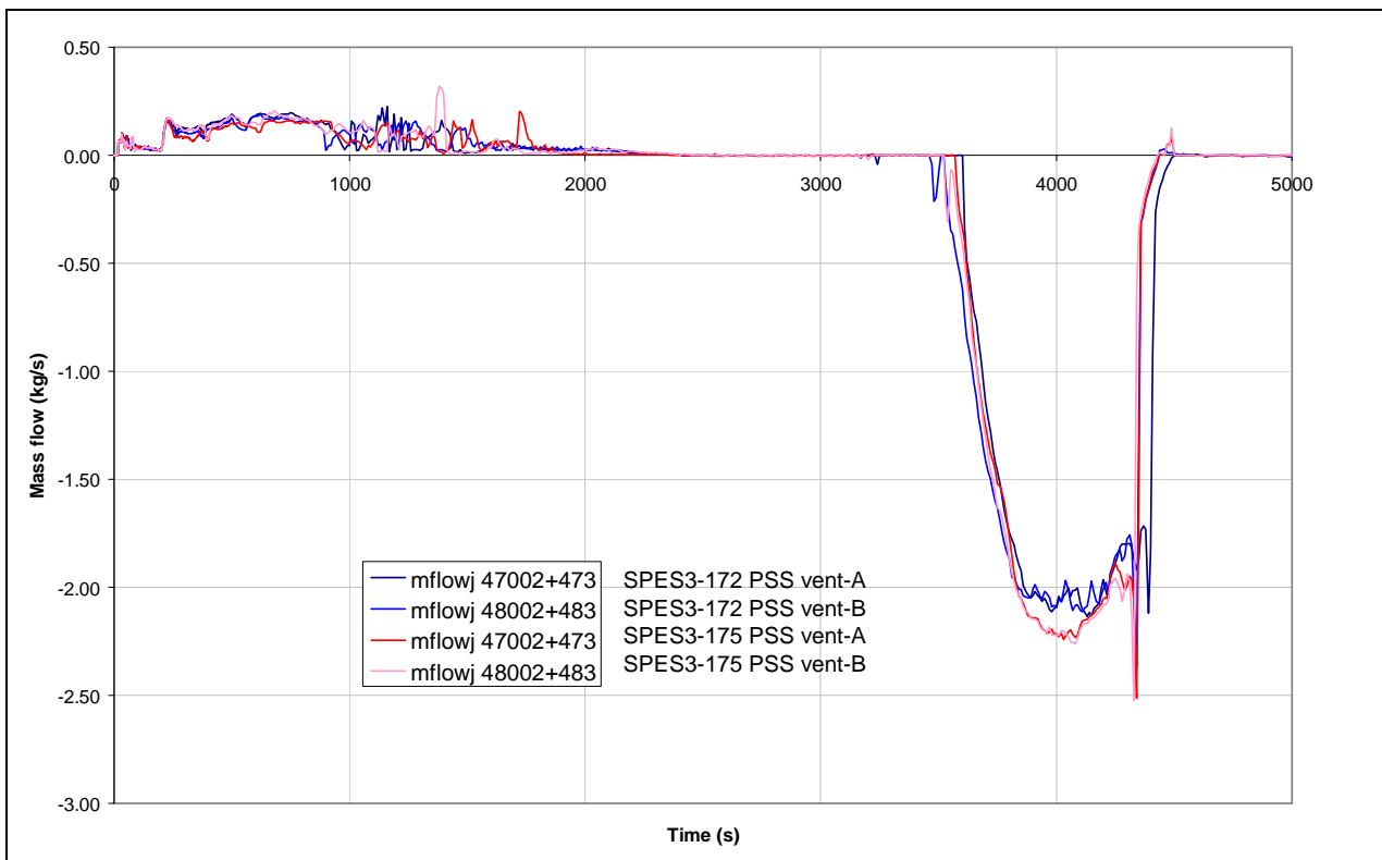
Fig.7. 18 - SPES3-172 and SPES3-175 DW to PSS mass flow (window)
