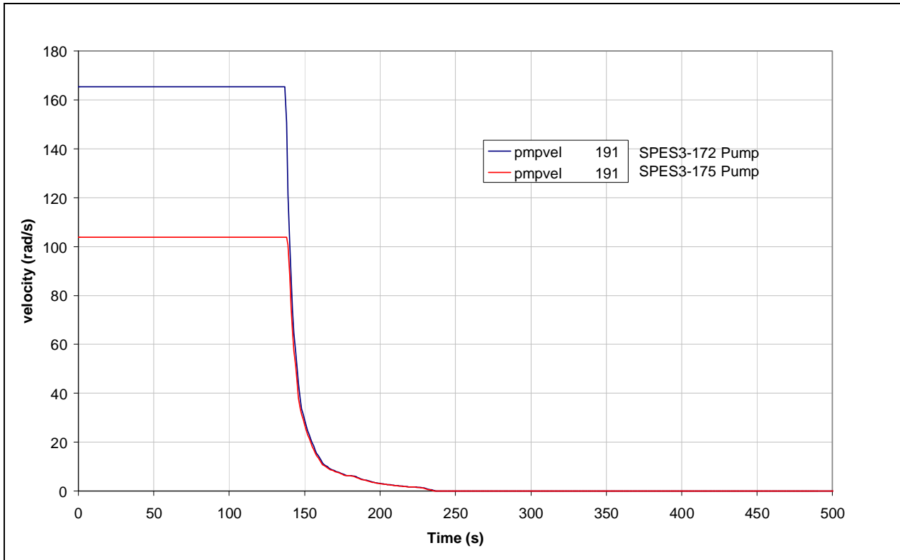
Fig.7. 47 - SPES3-172 and SPES3-175 Pump velocity (window)
