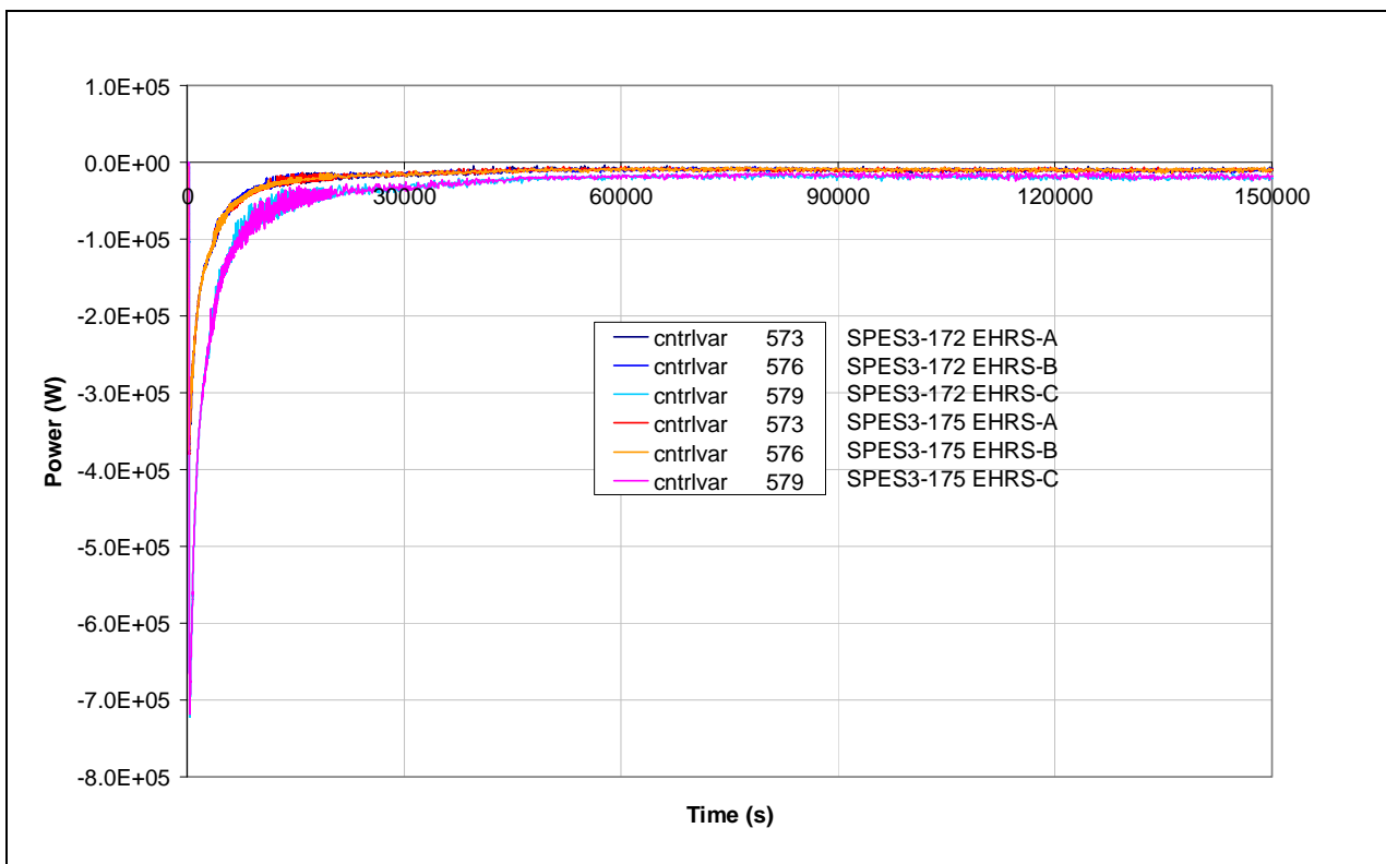
Fig.7. 40 - SPES3-172 and SPES3-175 EHR power
