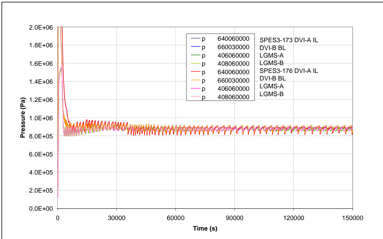
Fig.8. 83 – SPES3-173 and SPES3-176 LGMS and DVI pressure (window)
