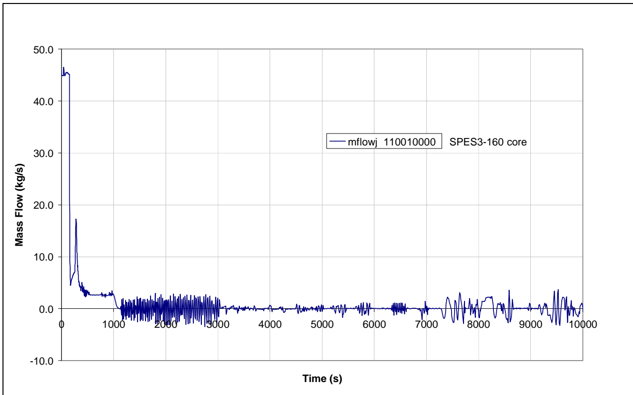
Fig.4.47 – SPES3-160 core inlet flow (window)
