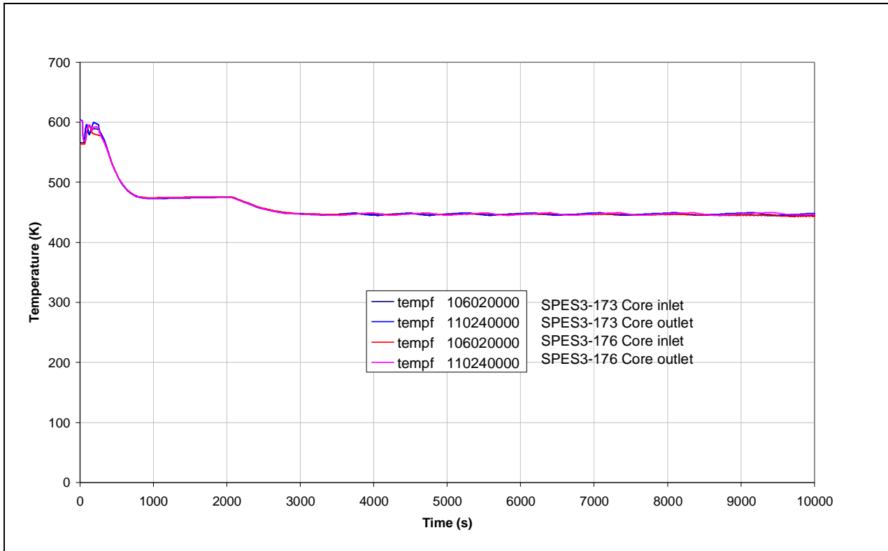
Fig.8. 69 – SPES3-173 and SPES3-176 Core inlet and outlet temperatures (window)
