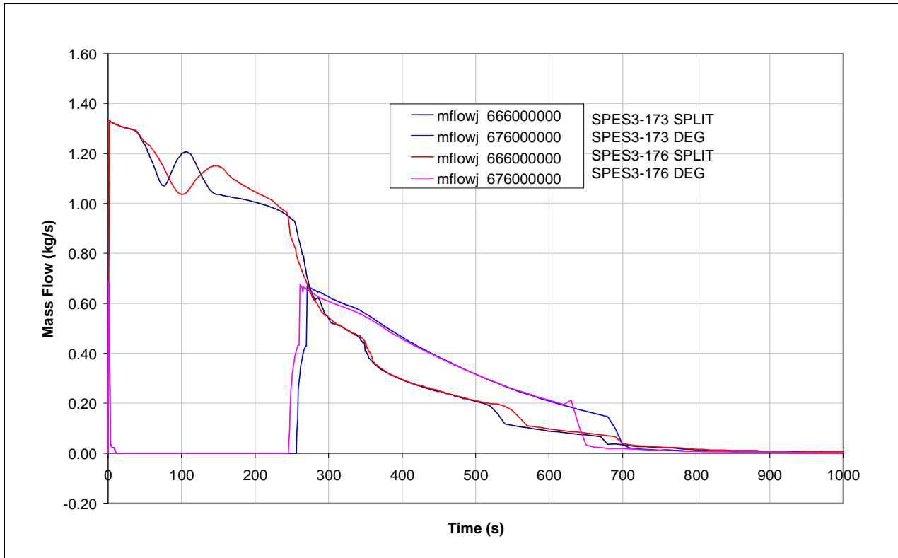
Fig.8. 1 – SPES3-173 and SPES3-176 DVI line break flow (window)
