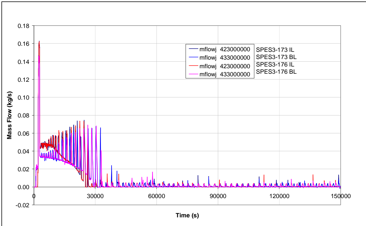
Fig.8. 6 – SPES3-173 and SPES3-176 LGMS injection mass flow
