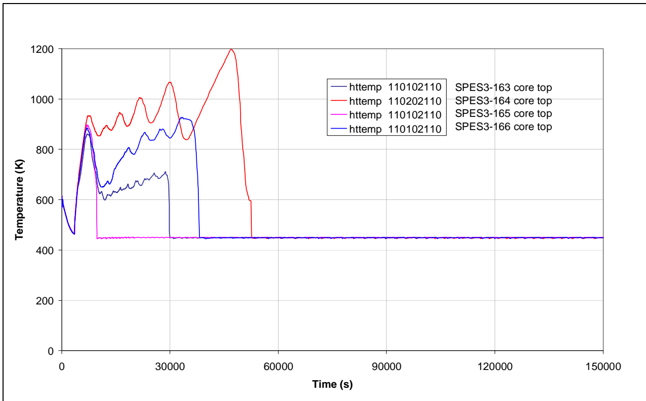
Fig.5. 27 – SPES3-163, 164, 165 and 166 Core heater rod clad surface temperature (normal rods)
