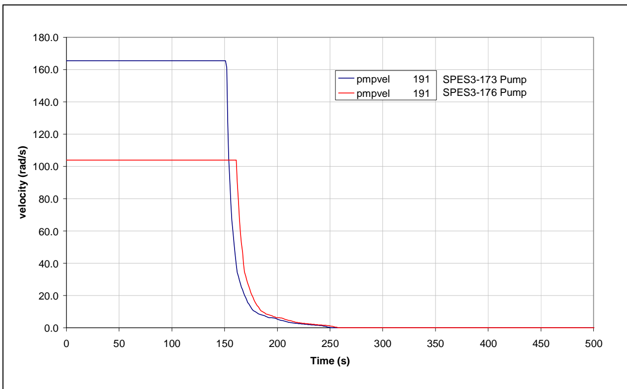
Fig.8. 54 – SPES3-173 and SPES3-176 Pump velocity
