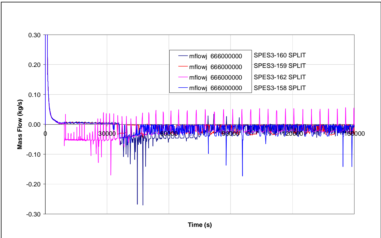
Fig.5. 11 – SPES3-159, 162, 158 and 160 DVI break line (RPV side) mass flow (window)
