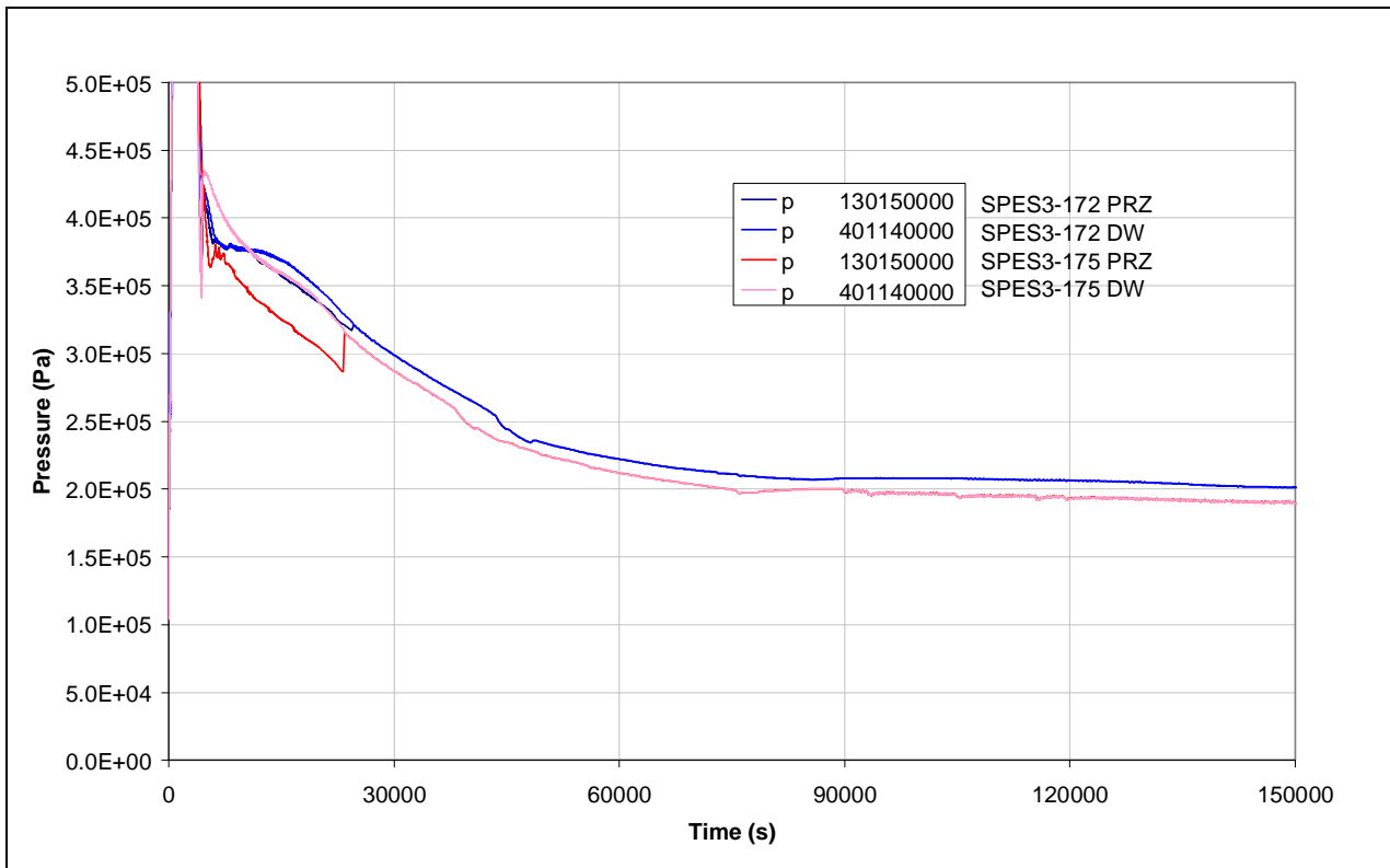
Fig.7. 17 - SPES3-172 and SPES3-175 PRZ and DW pressures (detail)
