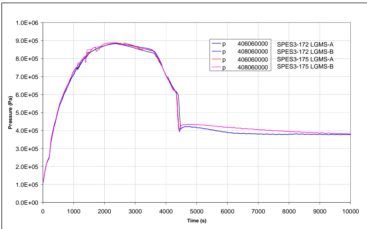
Fig.7. 24 - SPES3-172 and SPES3-175 LGMS pressure (window)
