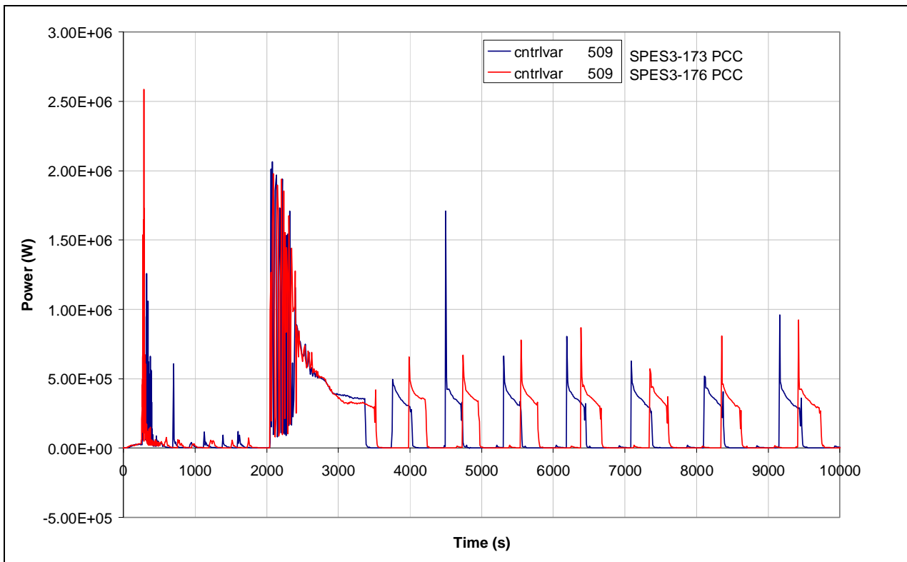
Fig.8. 20 – SPES3-173 and SPES3-176 PCC power (window)
