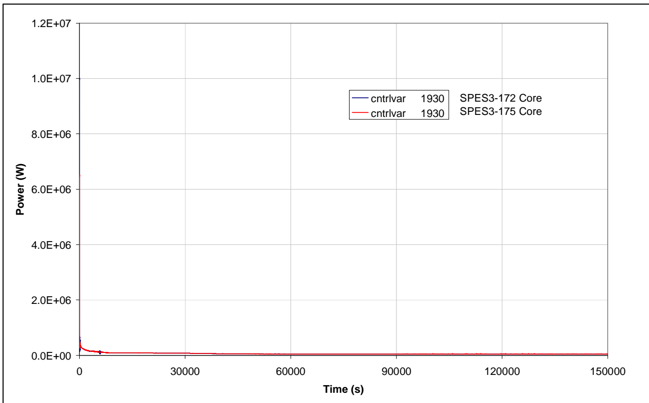
Fig.7. 32 - SPES3-172 and SPES3-175 Core power
