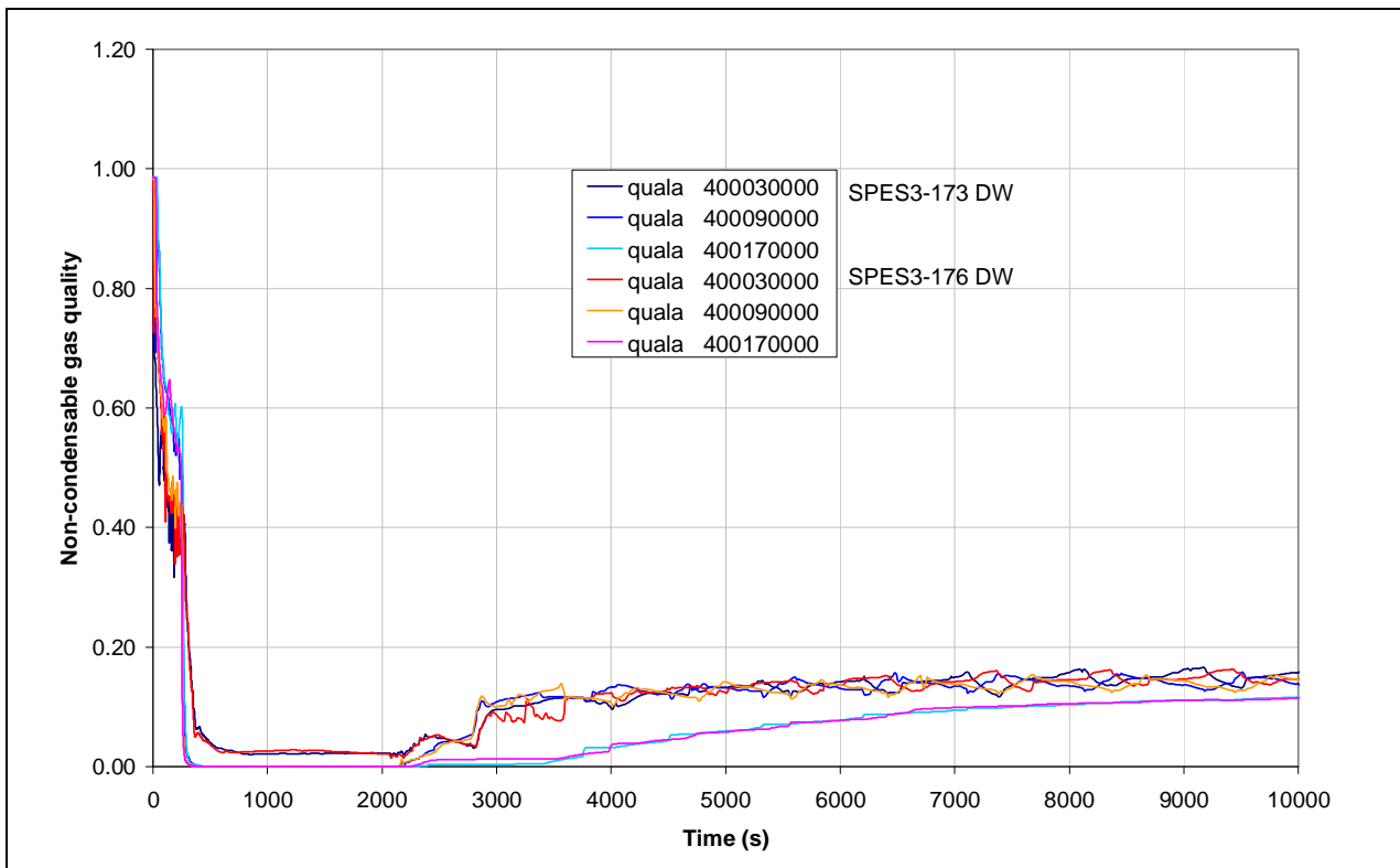
Fig.8. 24 – SPES3-173 and SPES3-176 DW non-condensable quality (window)
