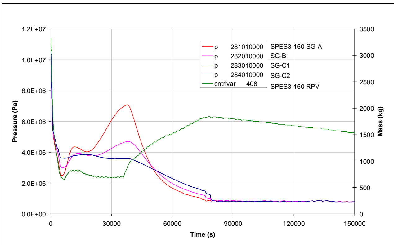
Fig.4.42 – SPES3-160 SG ss outlet pressure and RPV mass
