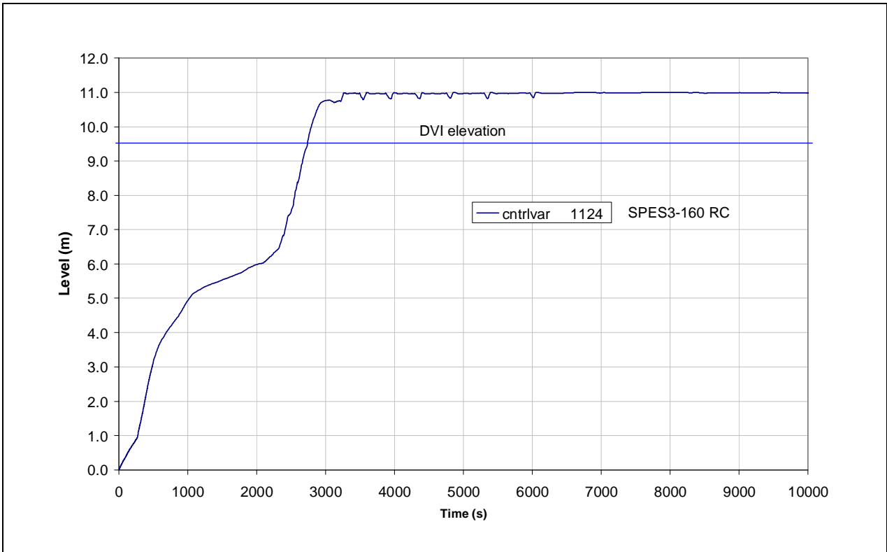
Fig.4.29 – SPES3-160 RC level (window)
