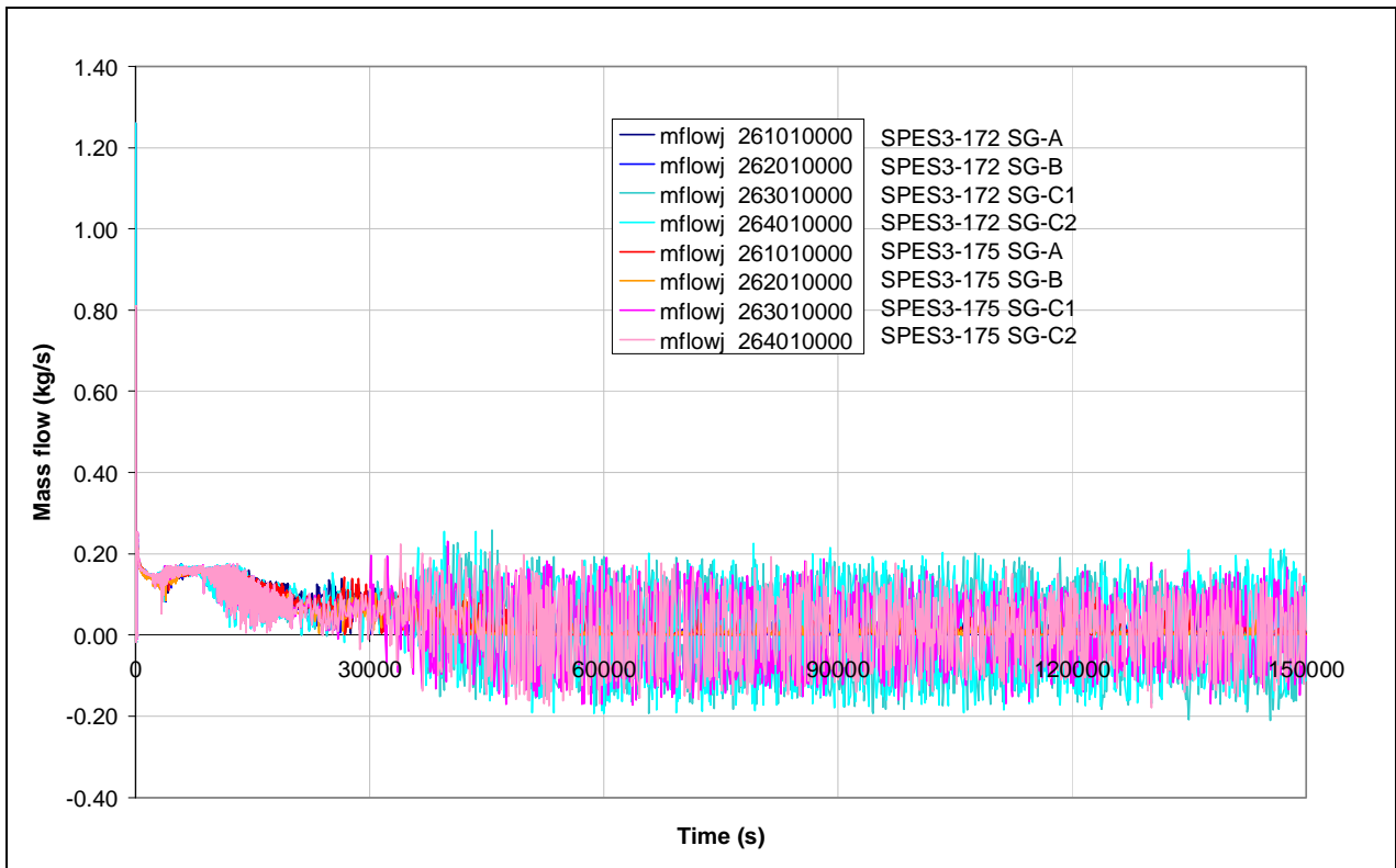
Fig.7. 36 - SPES3-172 and SPES3-175 SG ss mass flow
