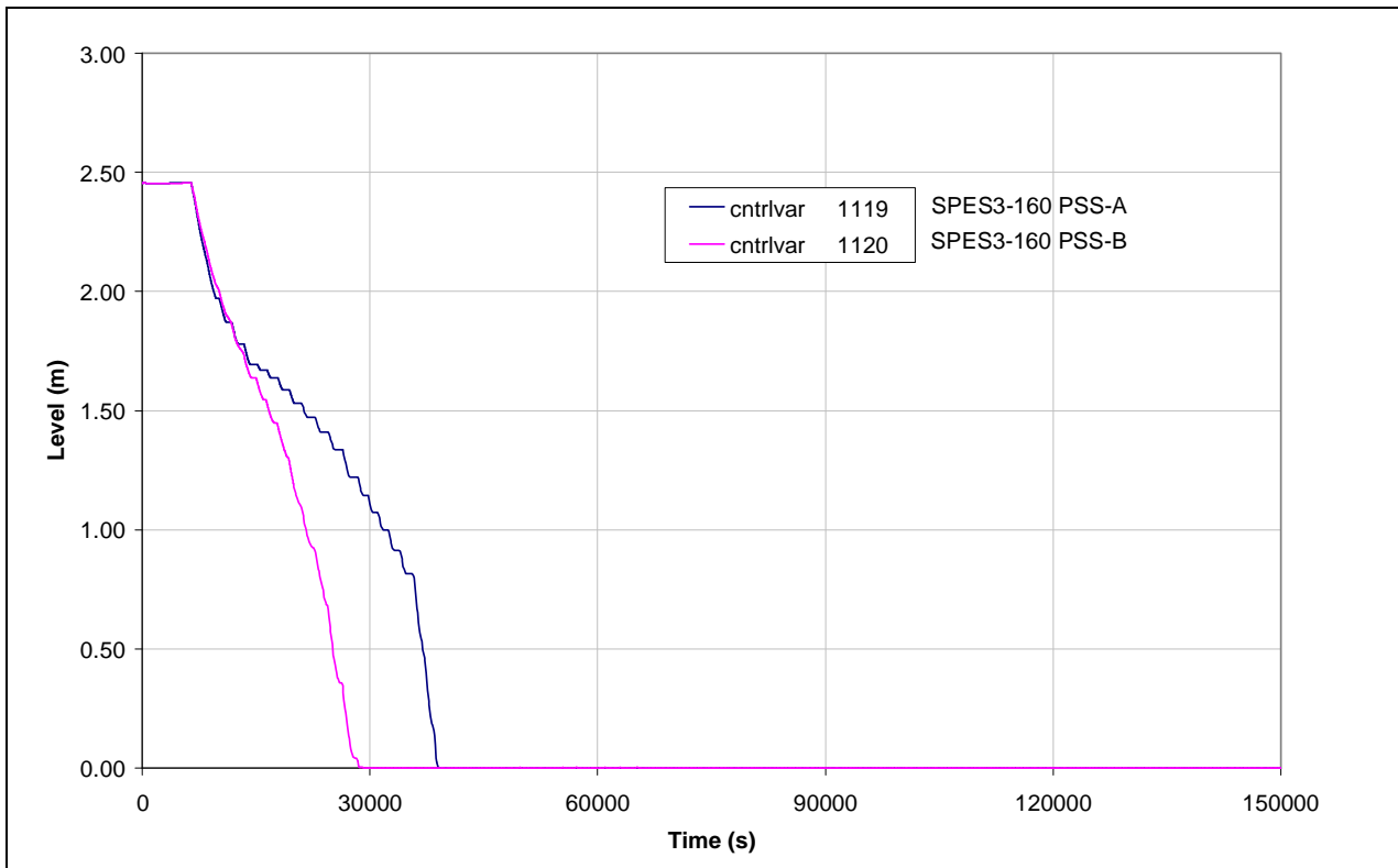
Fig.4.33 – SPES3-160 LGMS level
