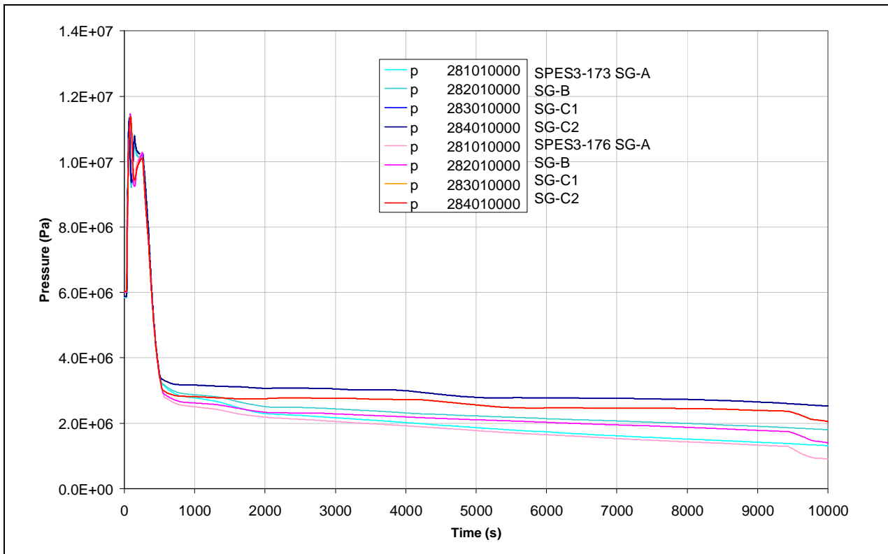
Fig.8. 49 – SPES3-173 and SPES3-176 SG ss outlet pressure (window)
