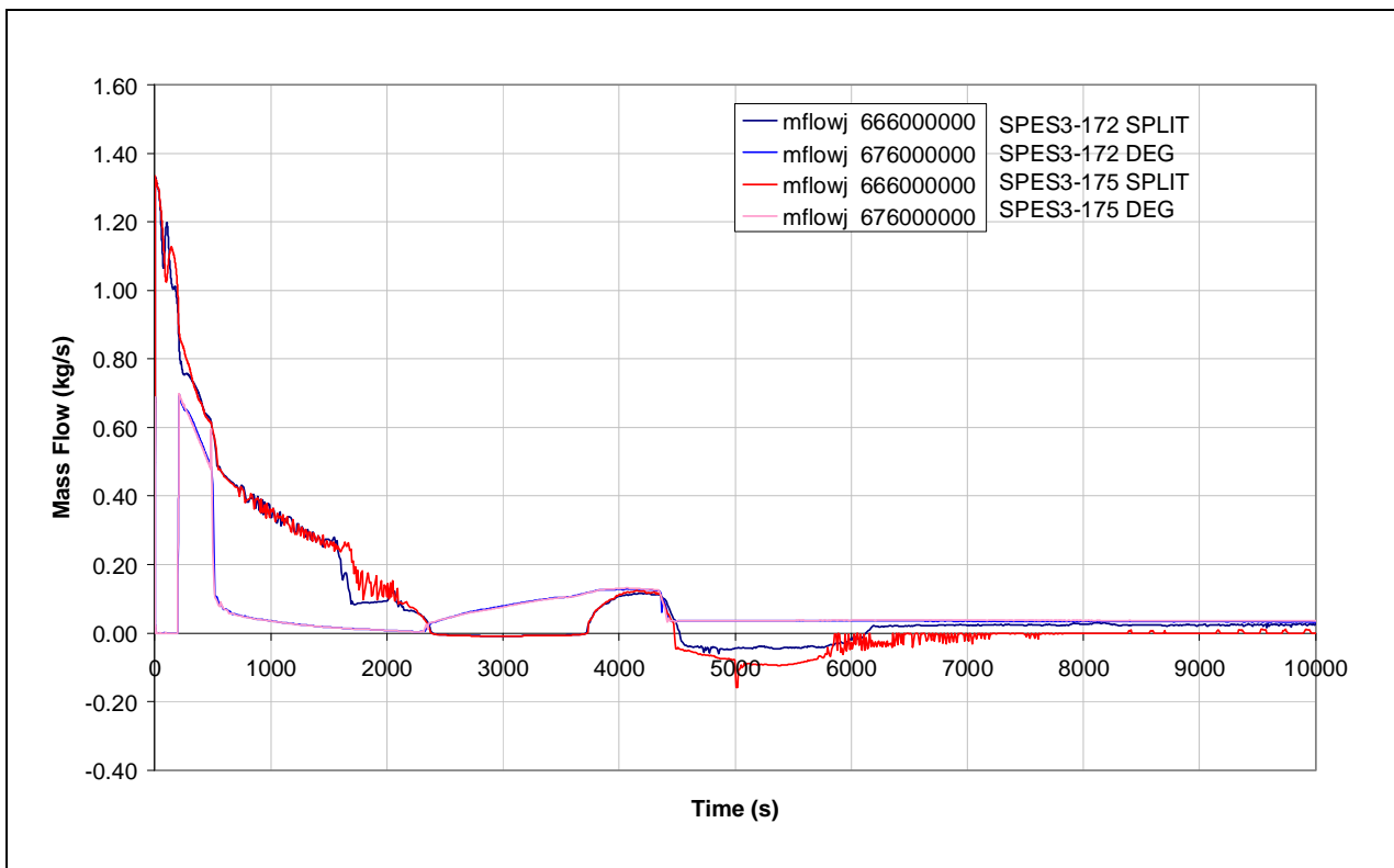
Fig.7. 2 - SPES3-172 and SPES3-175 DVI break mass flow (window)
