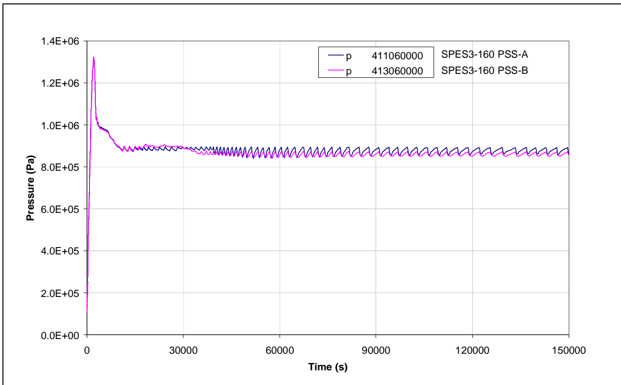
Fig.4.20 – SPES3-160 PSS pressure
