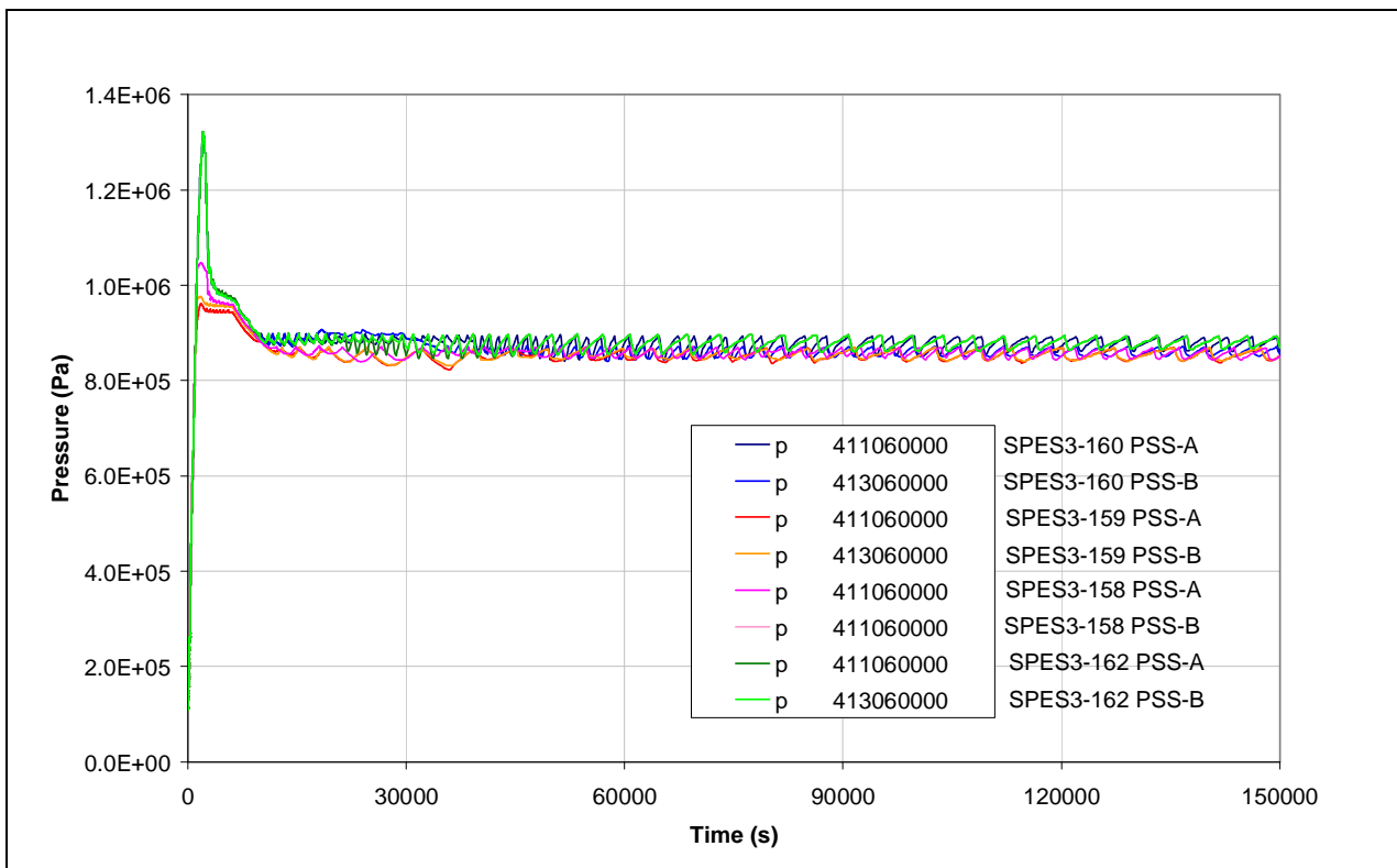
Fig.5. 4 – SPES3-159, 162, 158 and 160 PSS pressure
