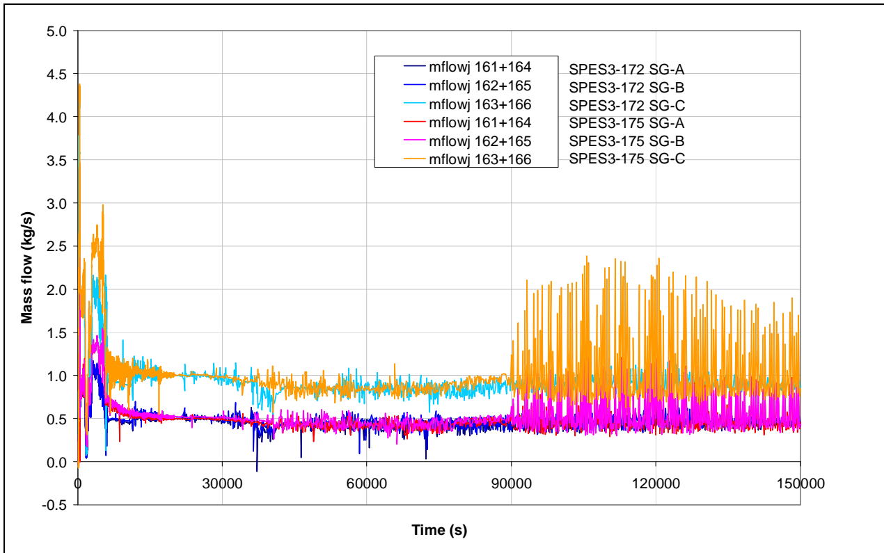
Fig.7. 51 - SPES3-172 and SPES3-175 RI-DC check valve mass flow
