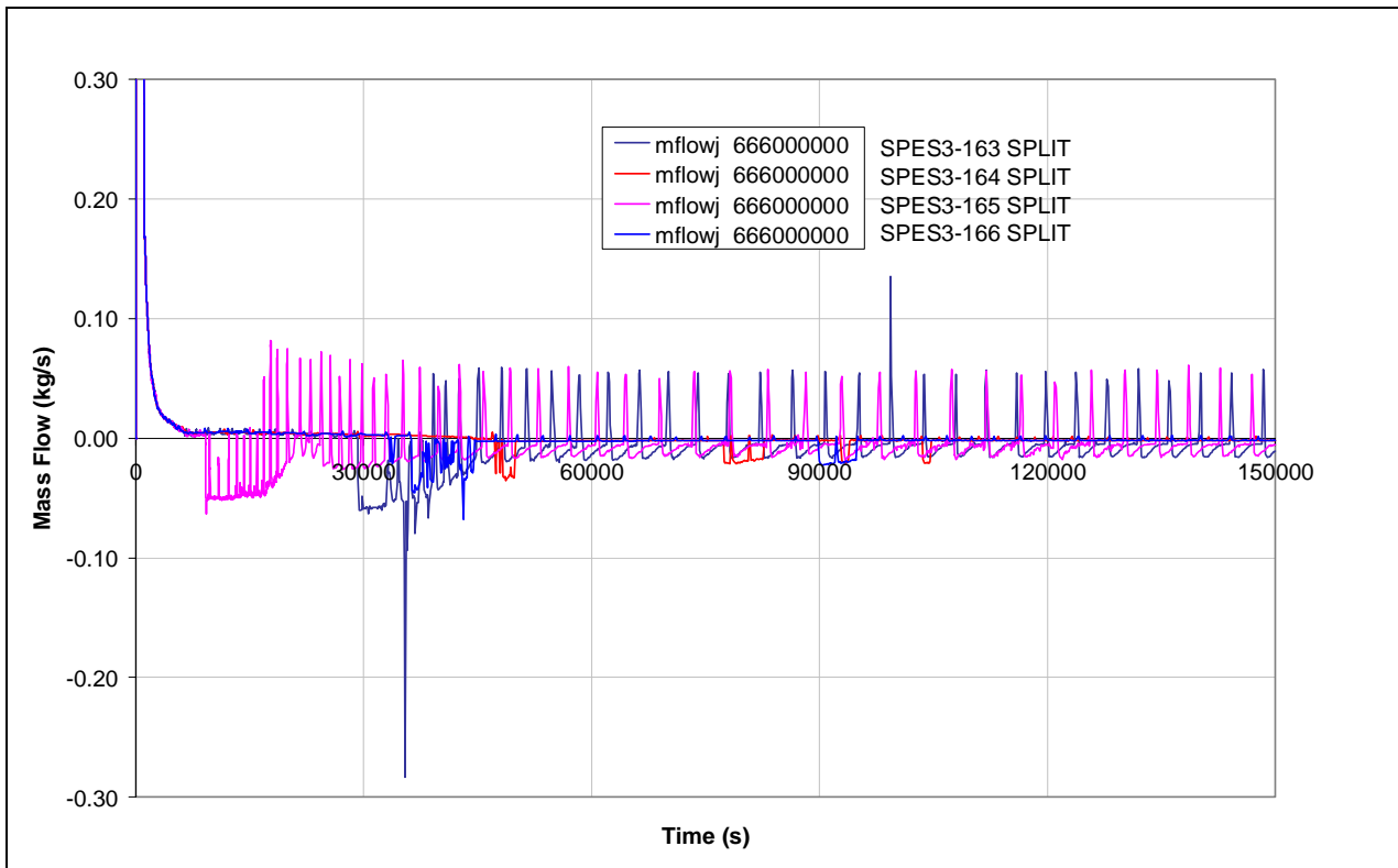
Fig.5. 25 – SPES3-163, 164, 165 and 166 DVI break line (RPV side) mass flow (window)
