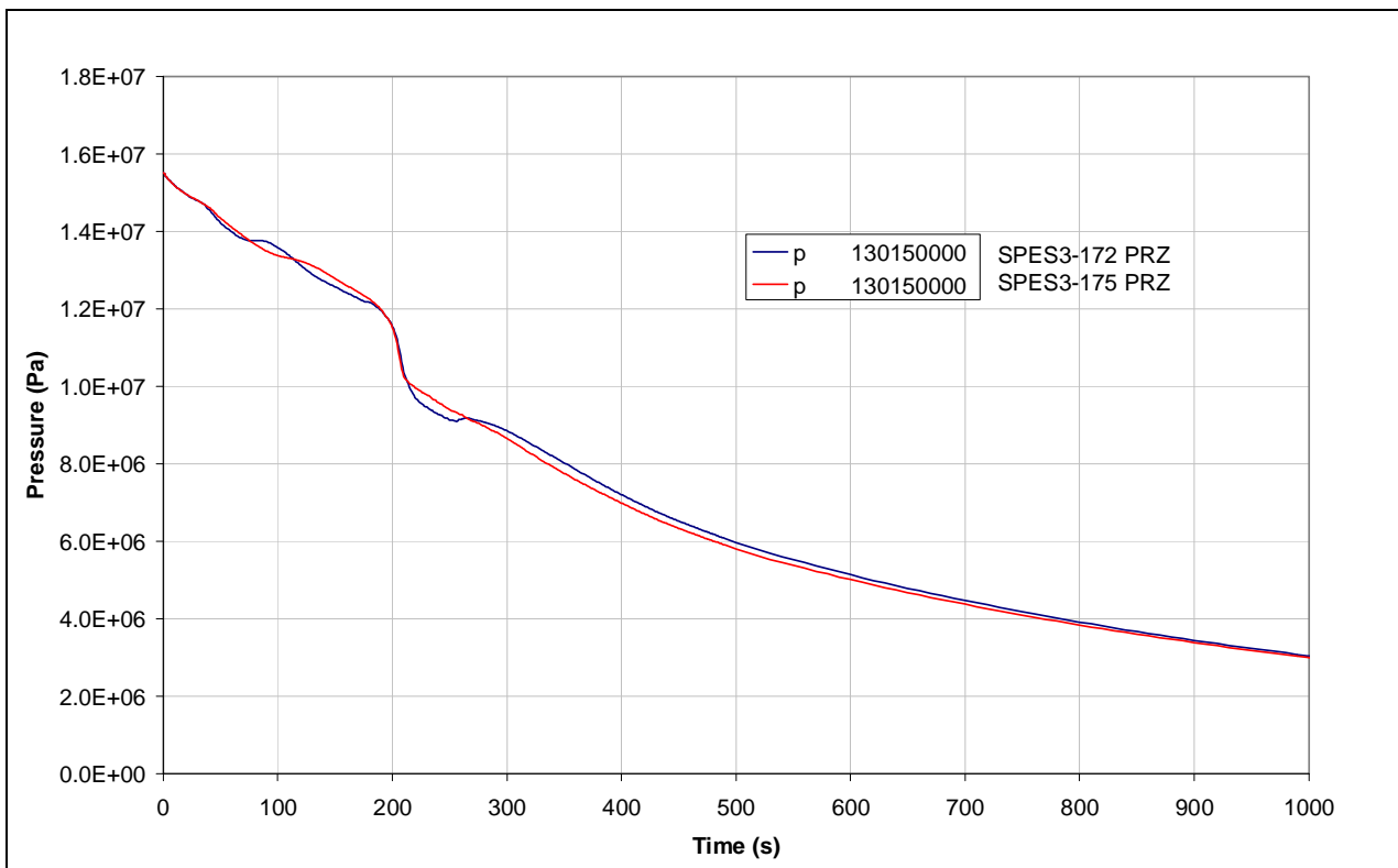
Fig.7. 8 - SPES3-172 and SPES3-175 PRZ pressure (window)
