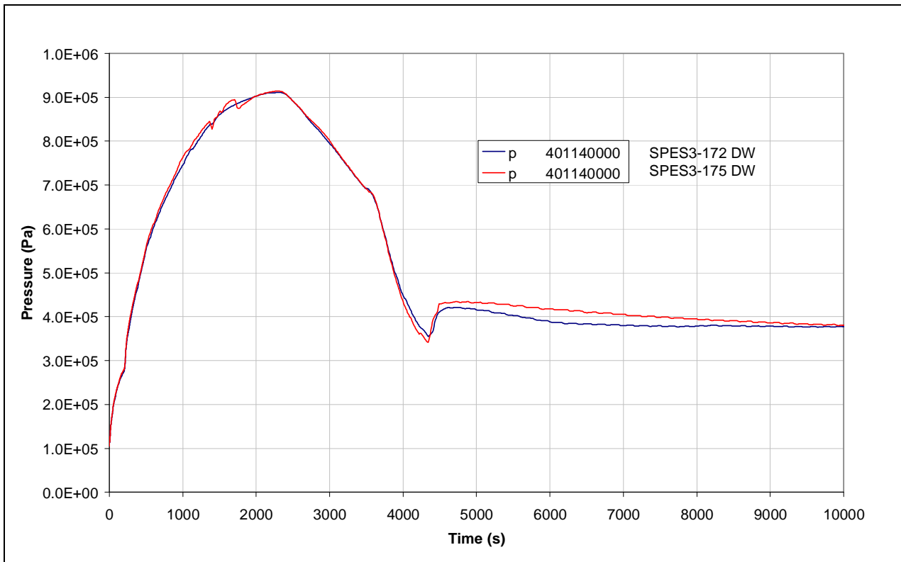
Fig.7. 11 - SPES3-172 and SPES3-175 DW pressure (window)
