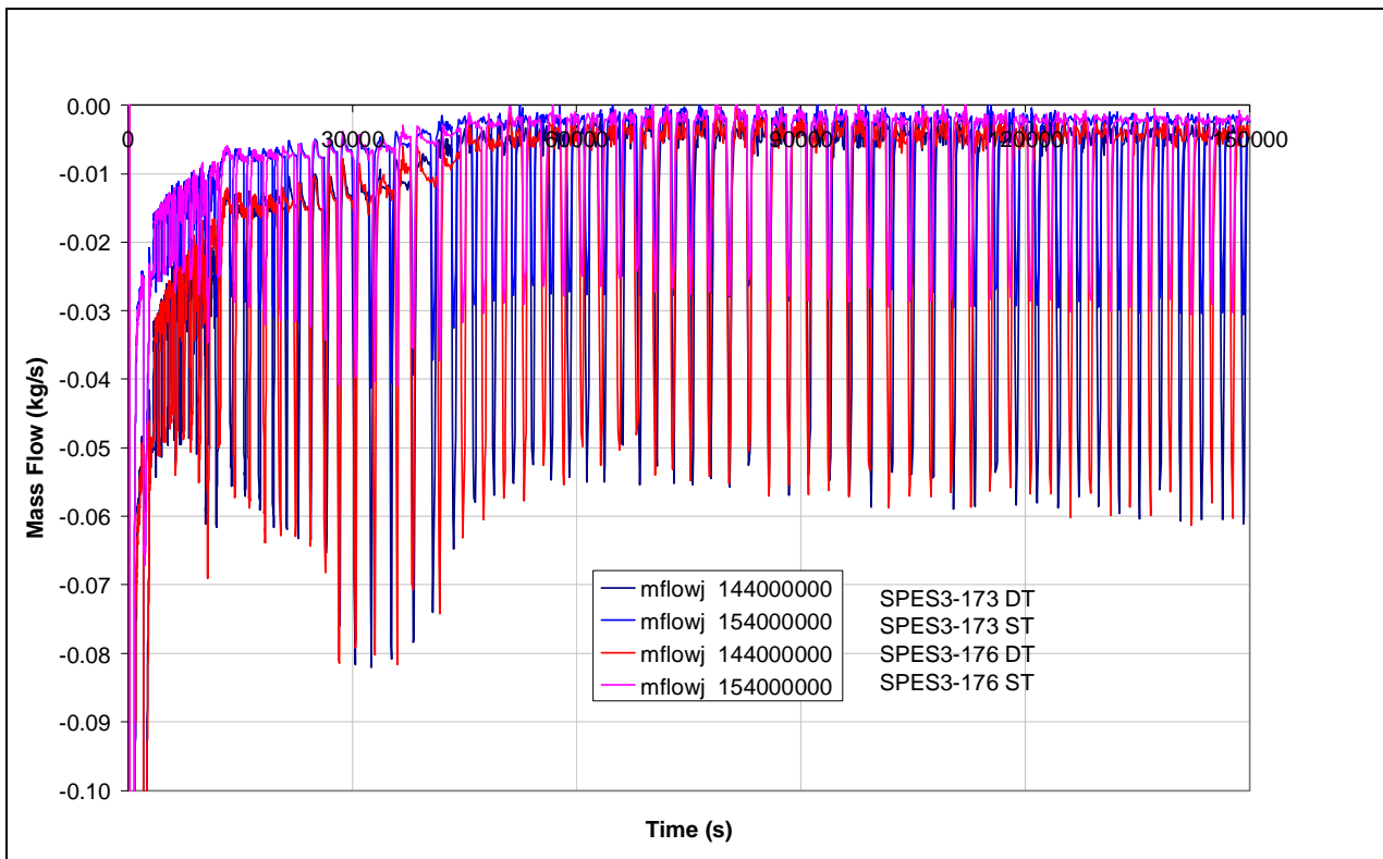
Fig.8. 10 – SPES3-173 and SPES3-176 ADS Stage-II mass flow (window)
