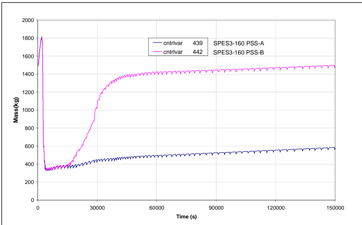
Fig.4.34 – SPES3-160 PSS mass
