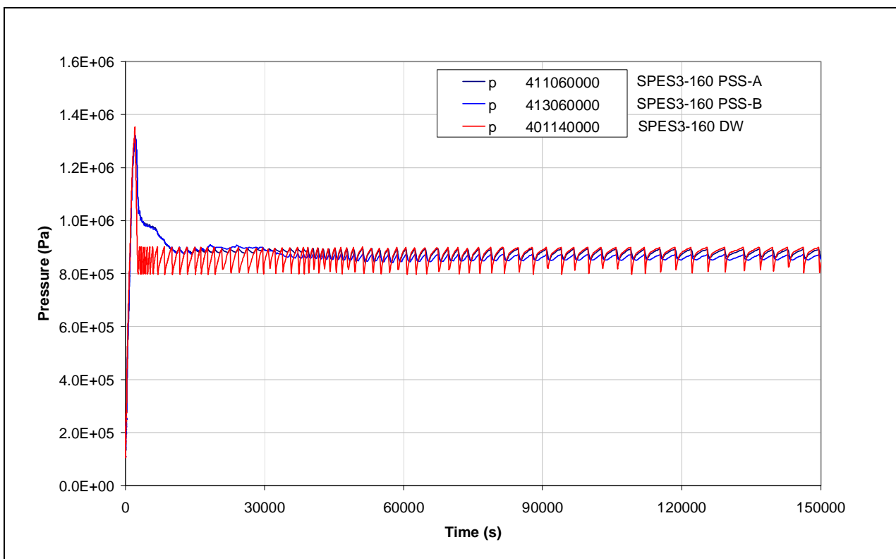
Fig.4.24 – SPES3-160 PSS and DW pressure
