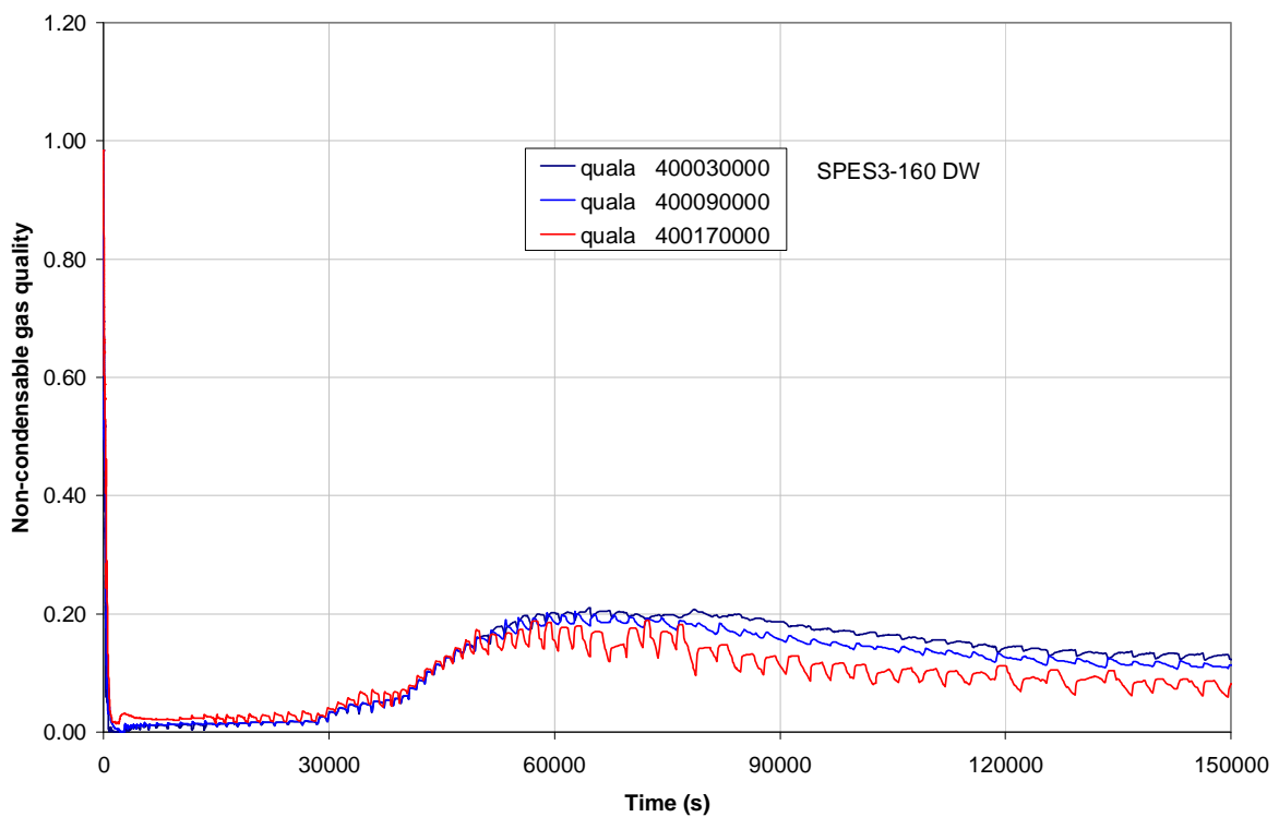
Fig.4.18 – SPES3-160 DW non-condensable gas quality
