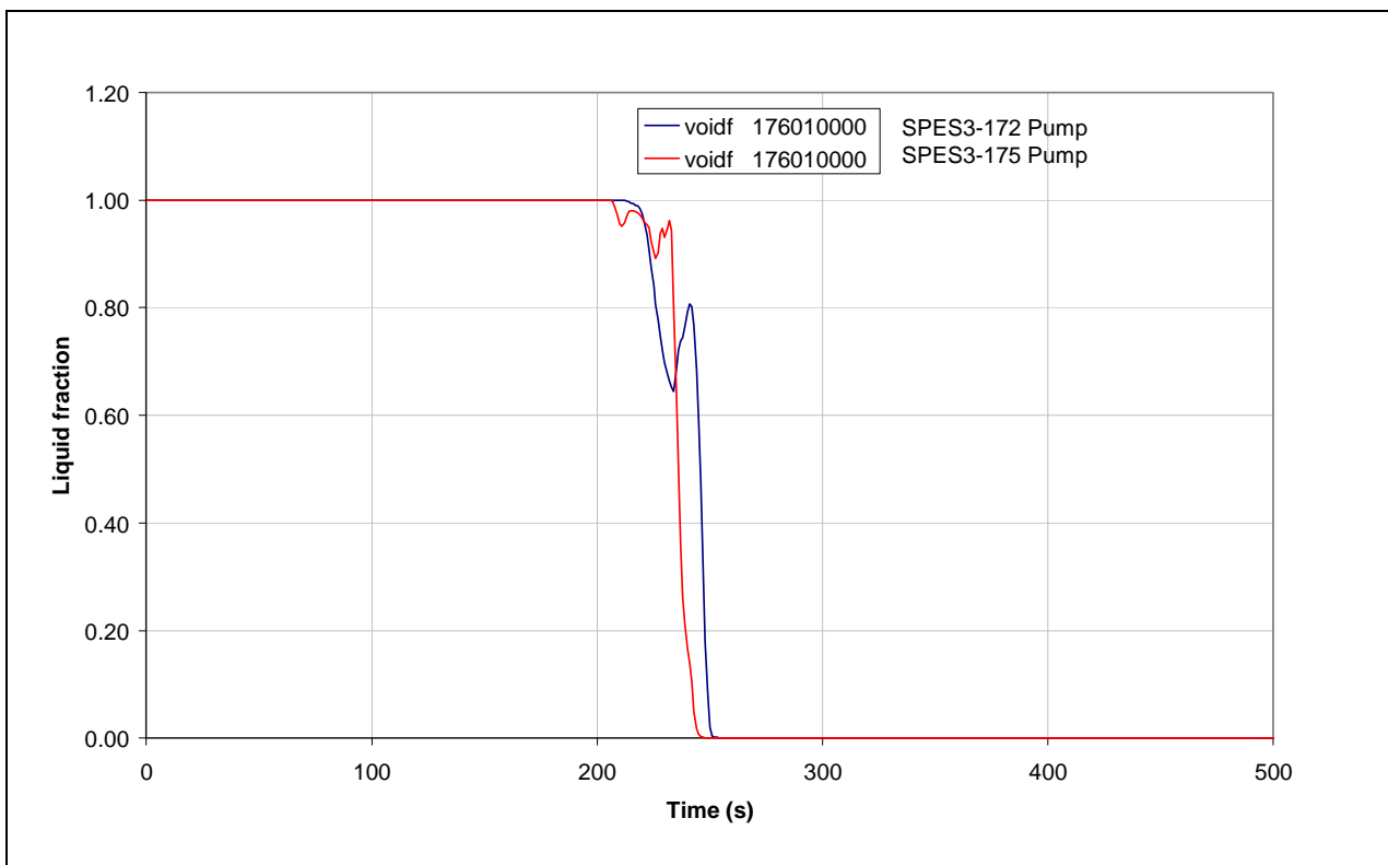
Fig.7. 46 - SPES3-172 and SPES3-175 Pump inlet liquid fraction (window)
