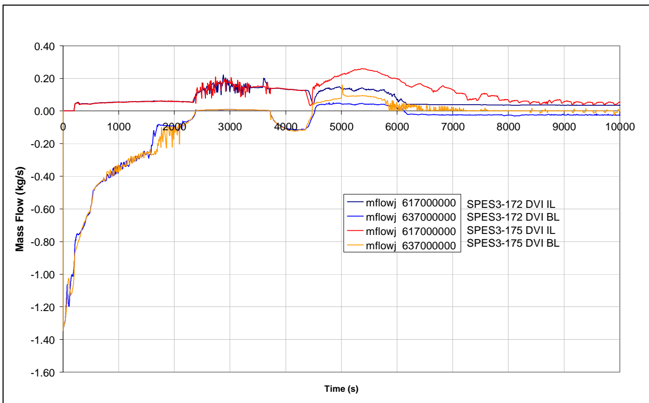
Fig.7. 68 - SPES3-172 and SPES3-175 DVI mass flow (window)
