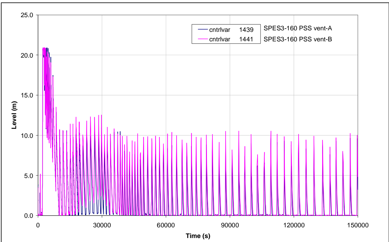
Fig.4.26 – SPES3-160 PSS vent pipe level
