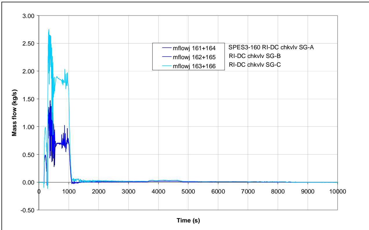
Fig.4.49 – SPES3-160 RI-DC check valve mass flow (window)
