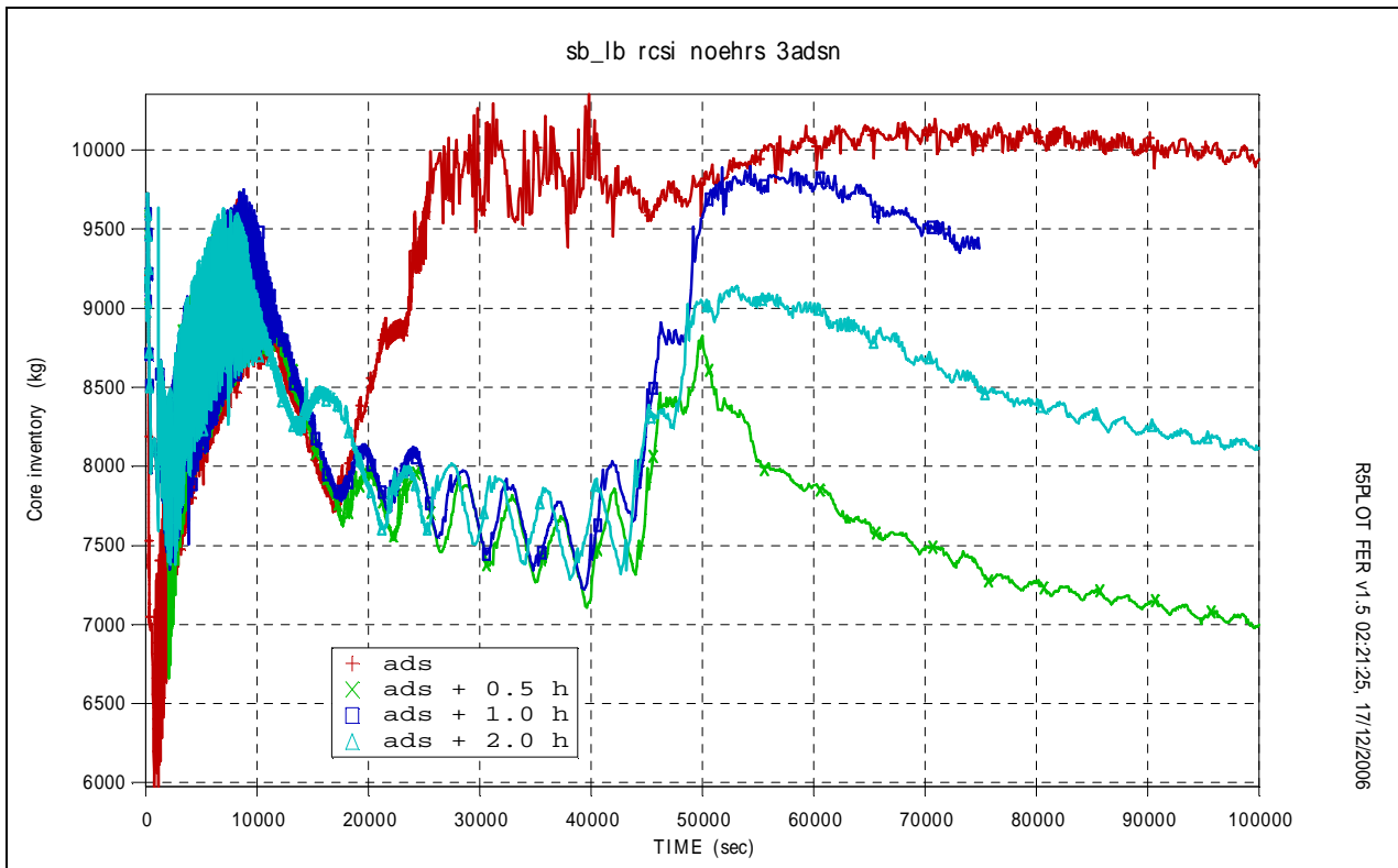
Fig.5. 30 – IRIS plant core mass
