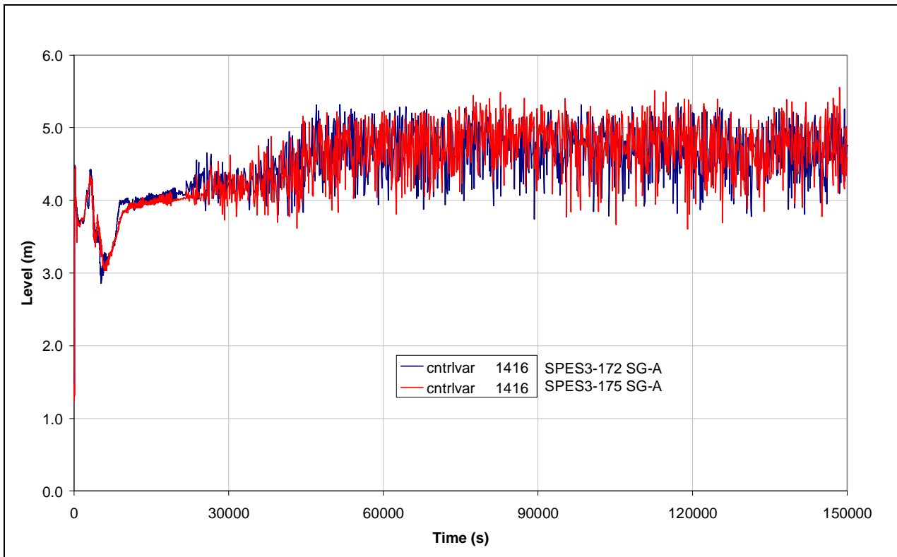
Fig.7. 44 - SPES3-172 and SPES3-175 SG-Ass collapsed level
