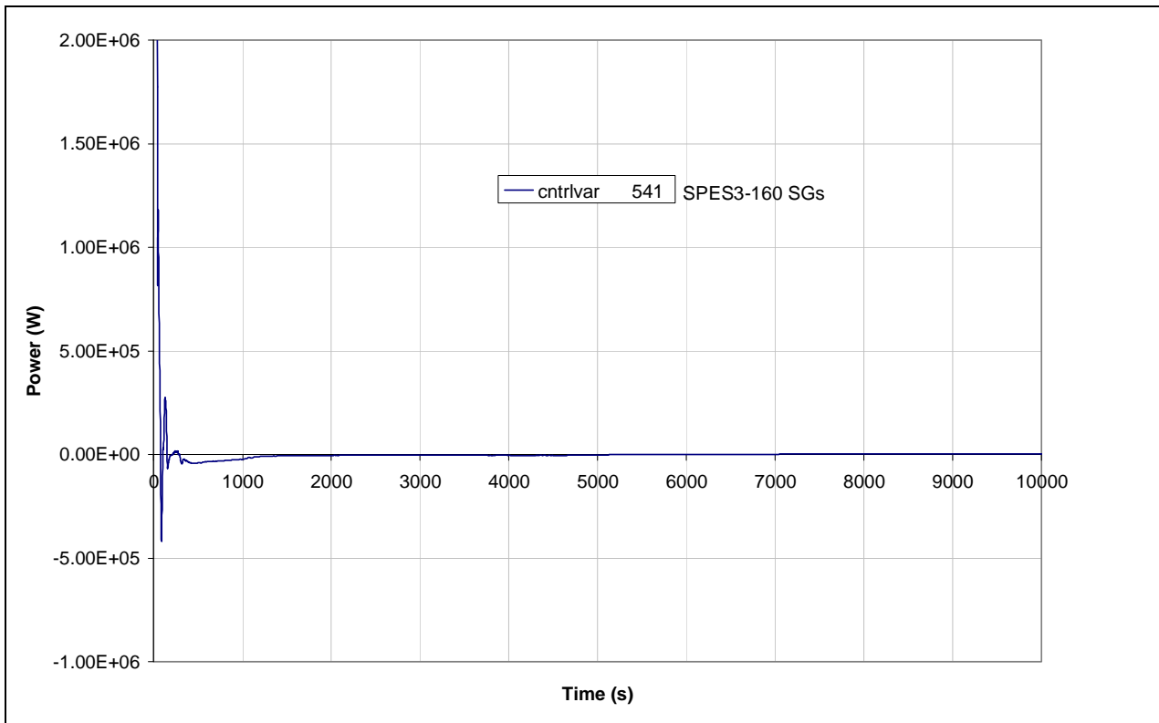
Fig.4.39 – SPES3-160 SG power (window)
