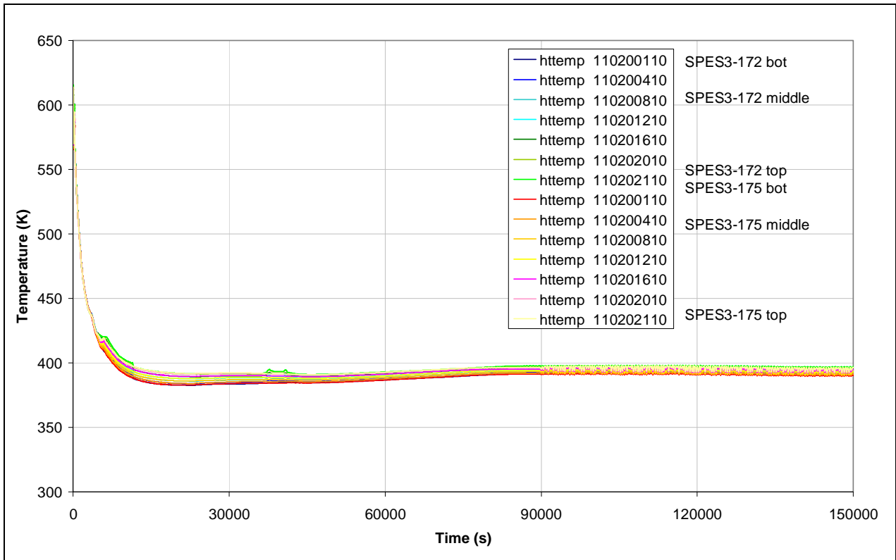
Fig.7. 65 - SPES3-172 and SPES3-175 Core heater rod surface temperature –hot rod
