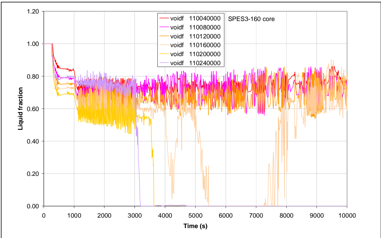
Fig.4.55 – SPES3-160 Core liquid fraction (window)
