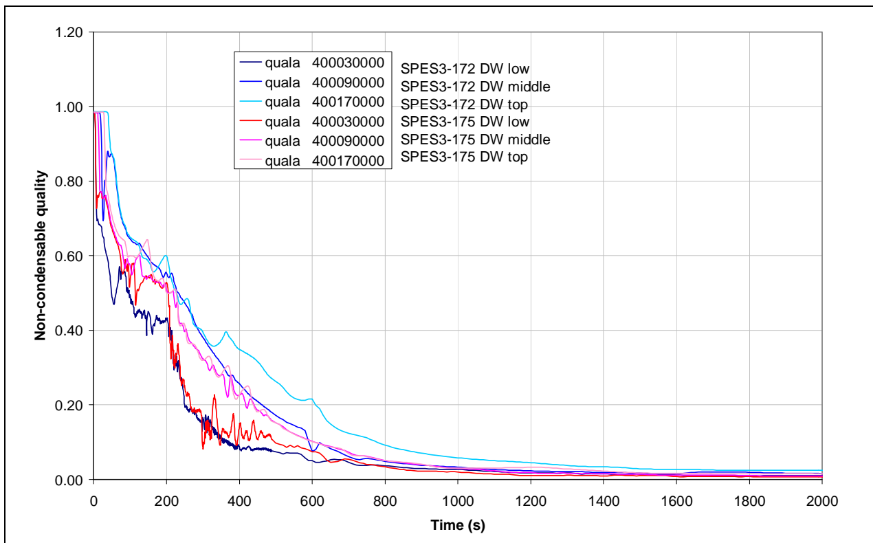
Fig.7. 20 - SPES3-172 and SPES3-175 DW non-condensable gas quality (window)
