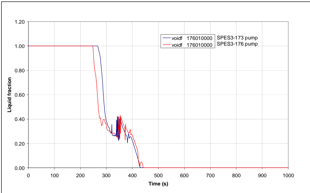
Fig.8. 55 – SPES3-173 and SPES3-176 pump inlet liquid fraction
