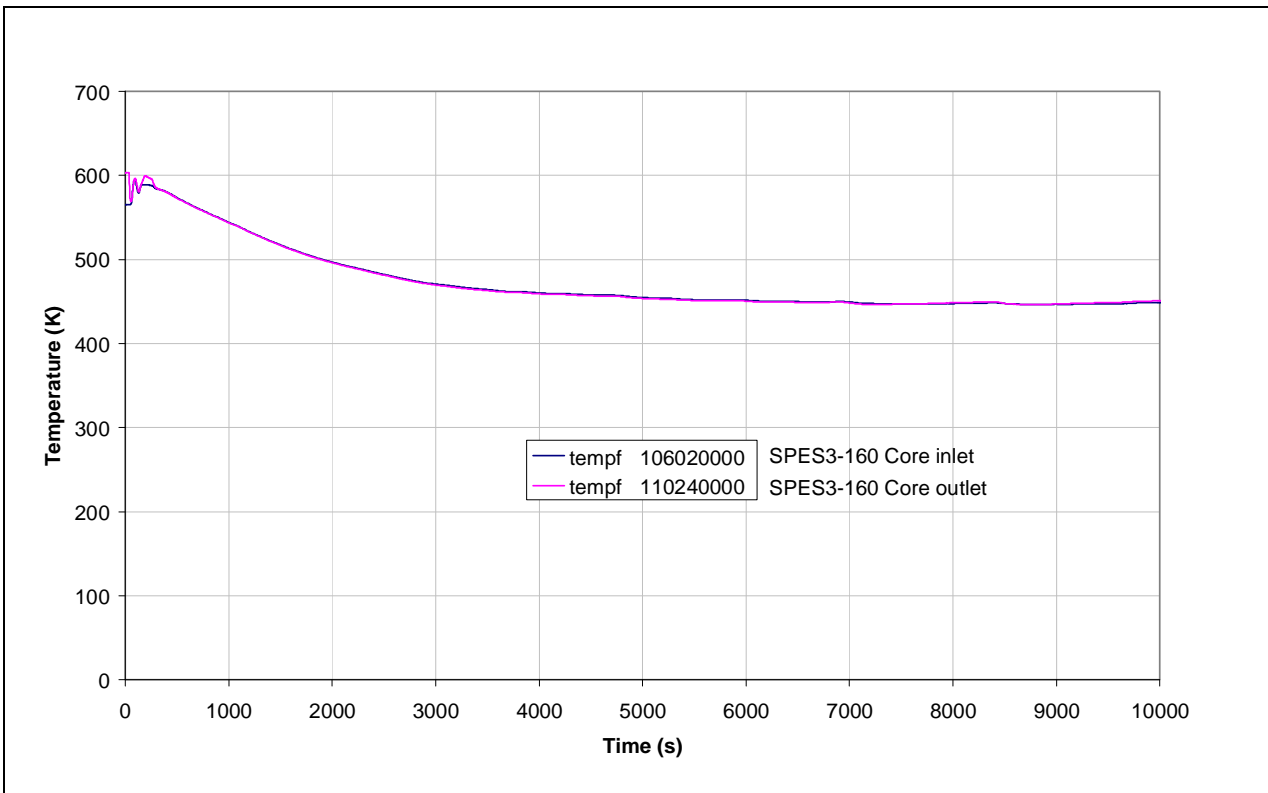
Fig.4.57 – SPES3-160 Core inlet and outlet temperatures (window)
