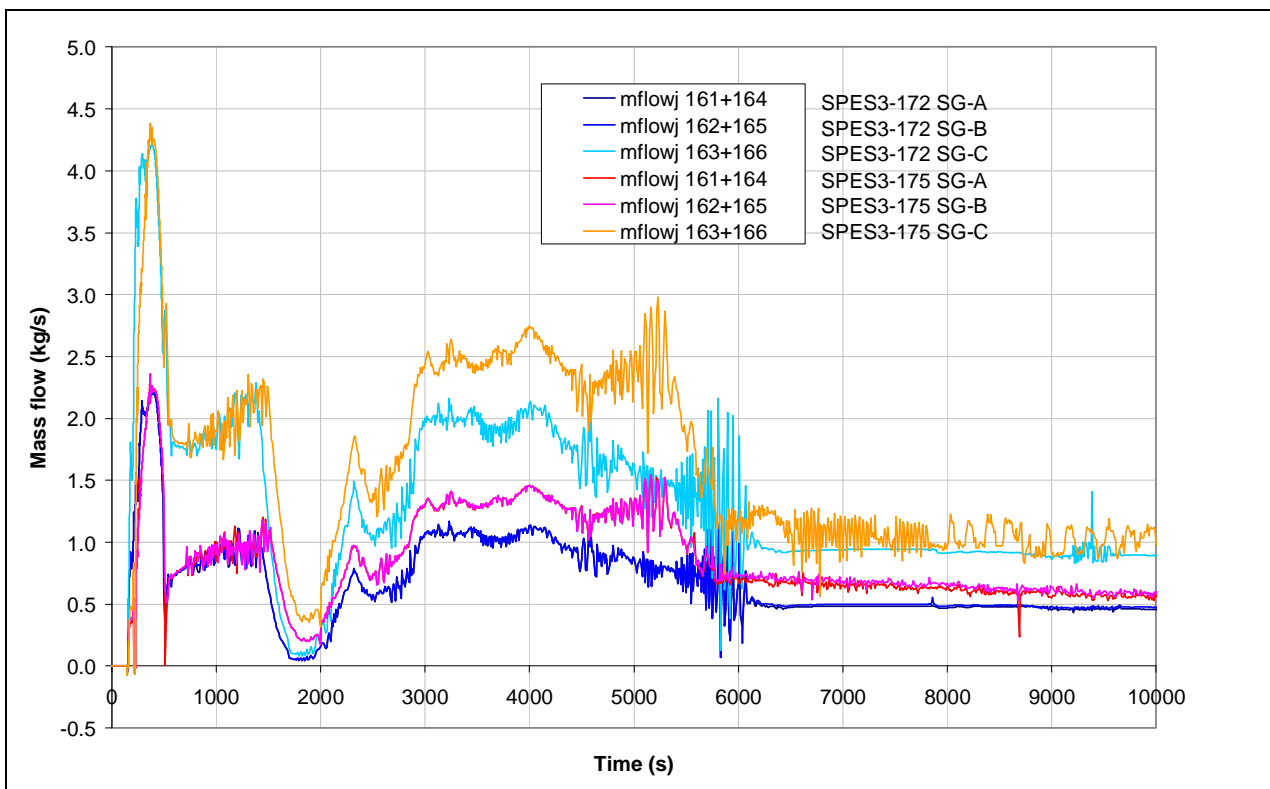
Fig.7. 50 - SPES3-172 and SPES3-175 RI-DC check valve mass flow (window)
