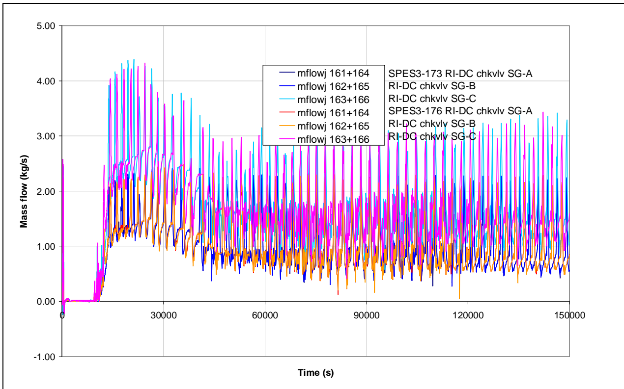
Fig.8. 59 – SPES3-173 and SPES3-176 RI-DC check valve mass flow
