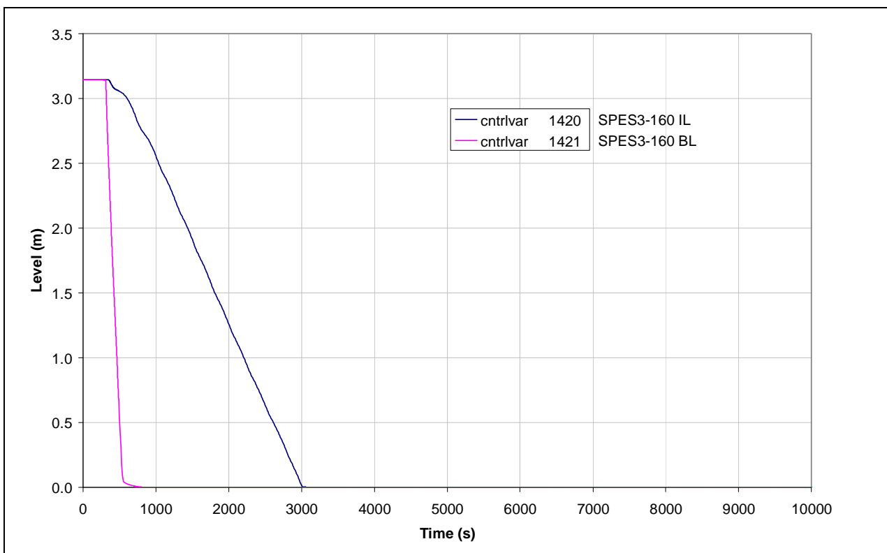
Fig.4.52 – SPES3-160 EBT level
