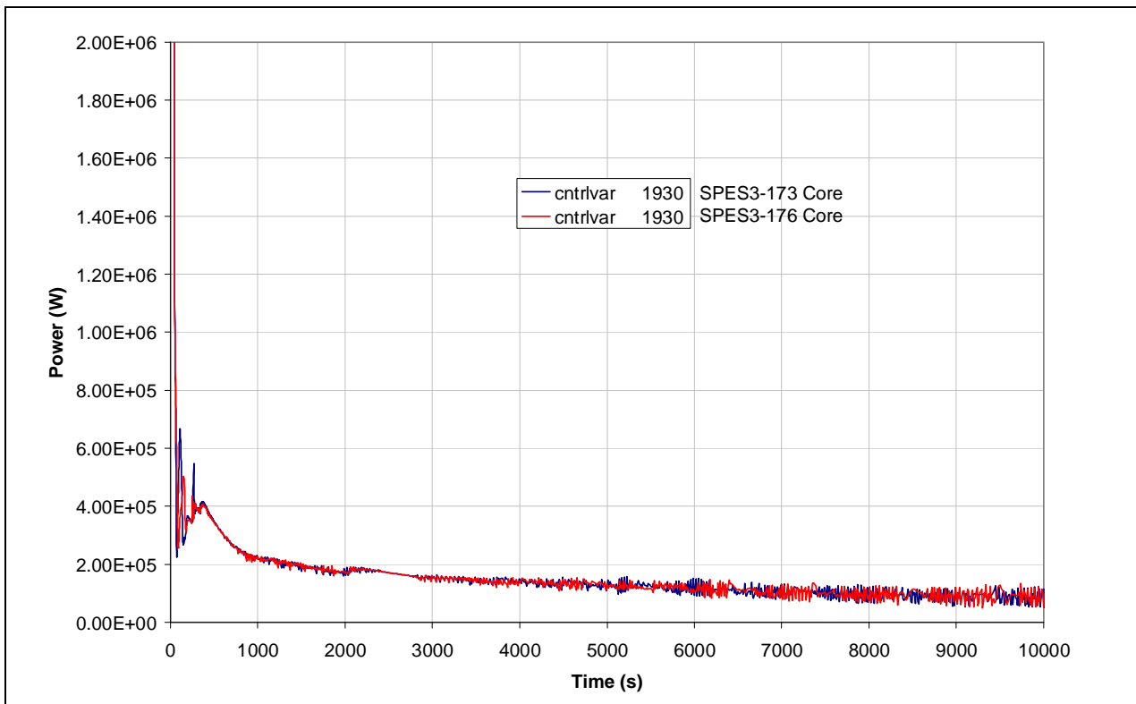
Fig.8. 44 – SPES3-173 and SPES3-176 core power (window)
