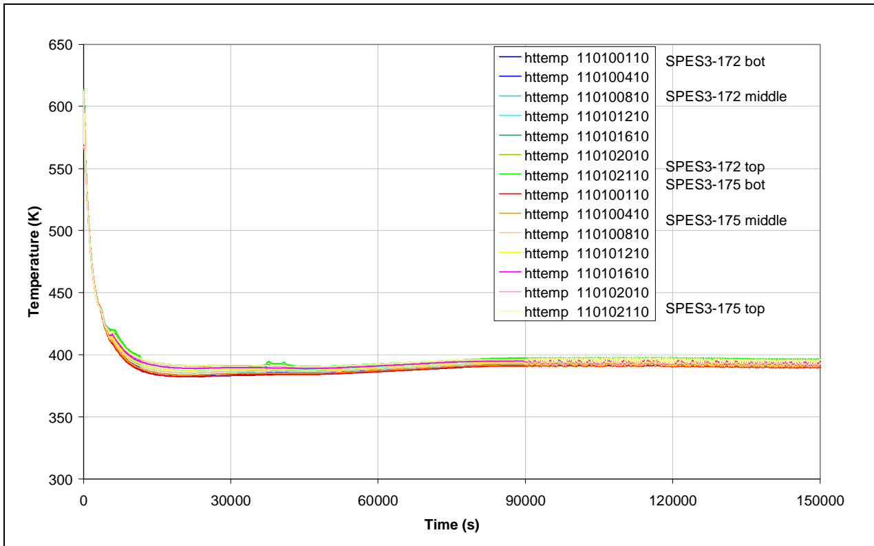
Fig.7. 63 - SPES3-172 and SPES3-175 Core heater rod surface temperature –normal rod
