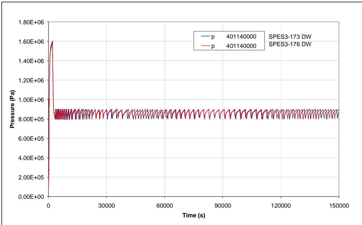
Fig.8. 19 – SPES3-173 and SPES3-176 DW pressure
