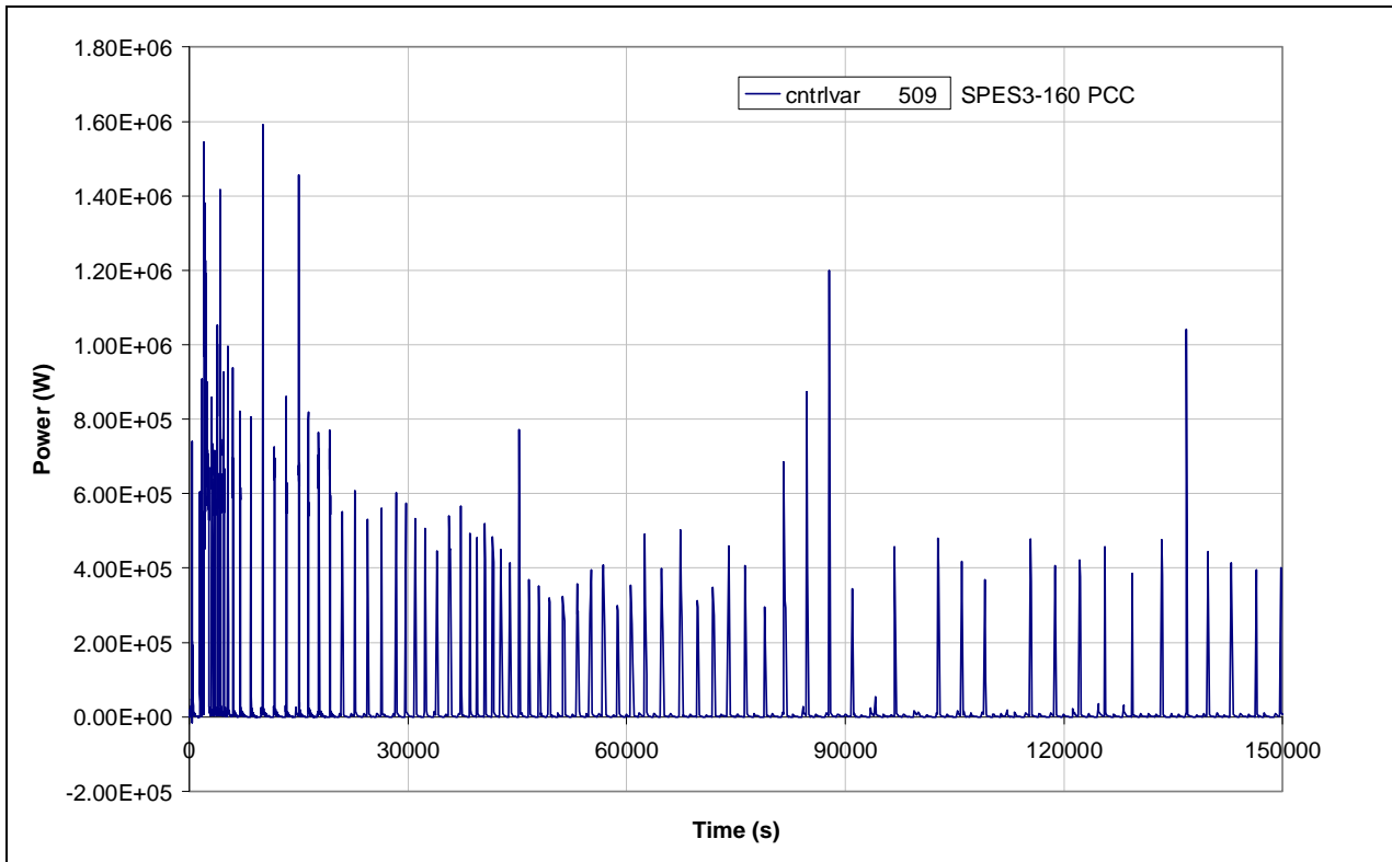
Fig.4.14 – SPES3-160 PCC power
