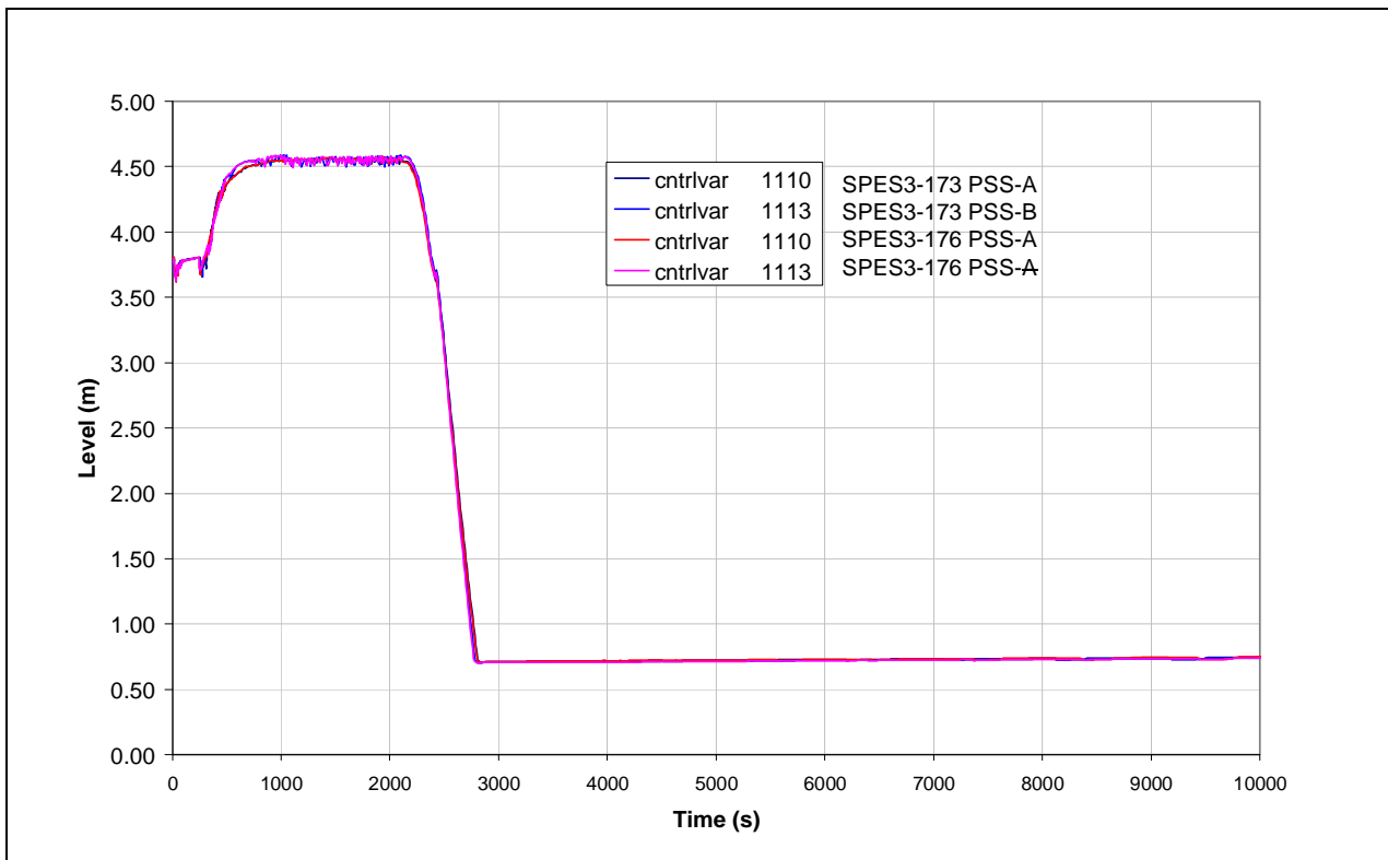
Fig.8. 34 – SPES3-173 and SPES3-176 PSS level (window)
