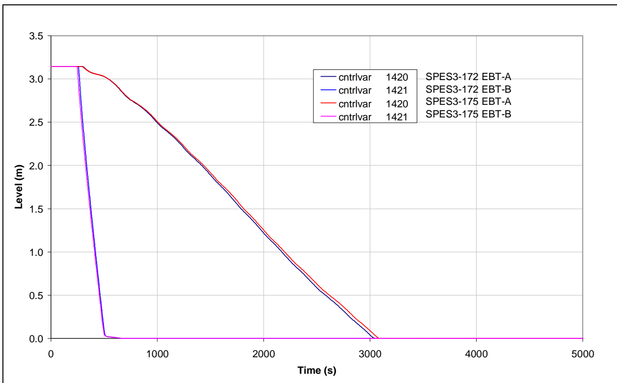
Fig.7. 58 - SPES3-172 and SPES3-175 EBT level (window)
