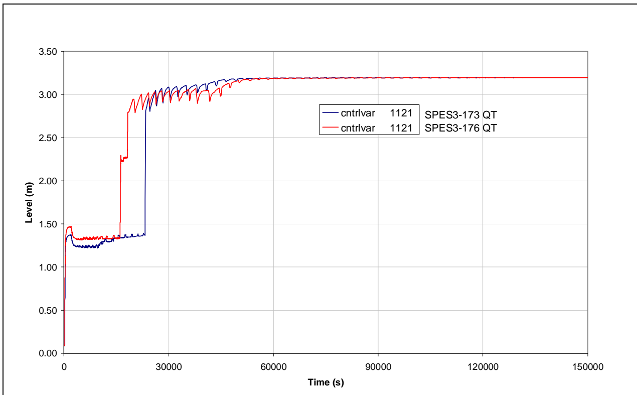
Fig.8. 40 – SPES3-173 and SPES3-176 QT level
