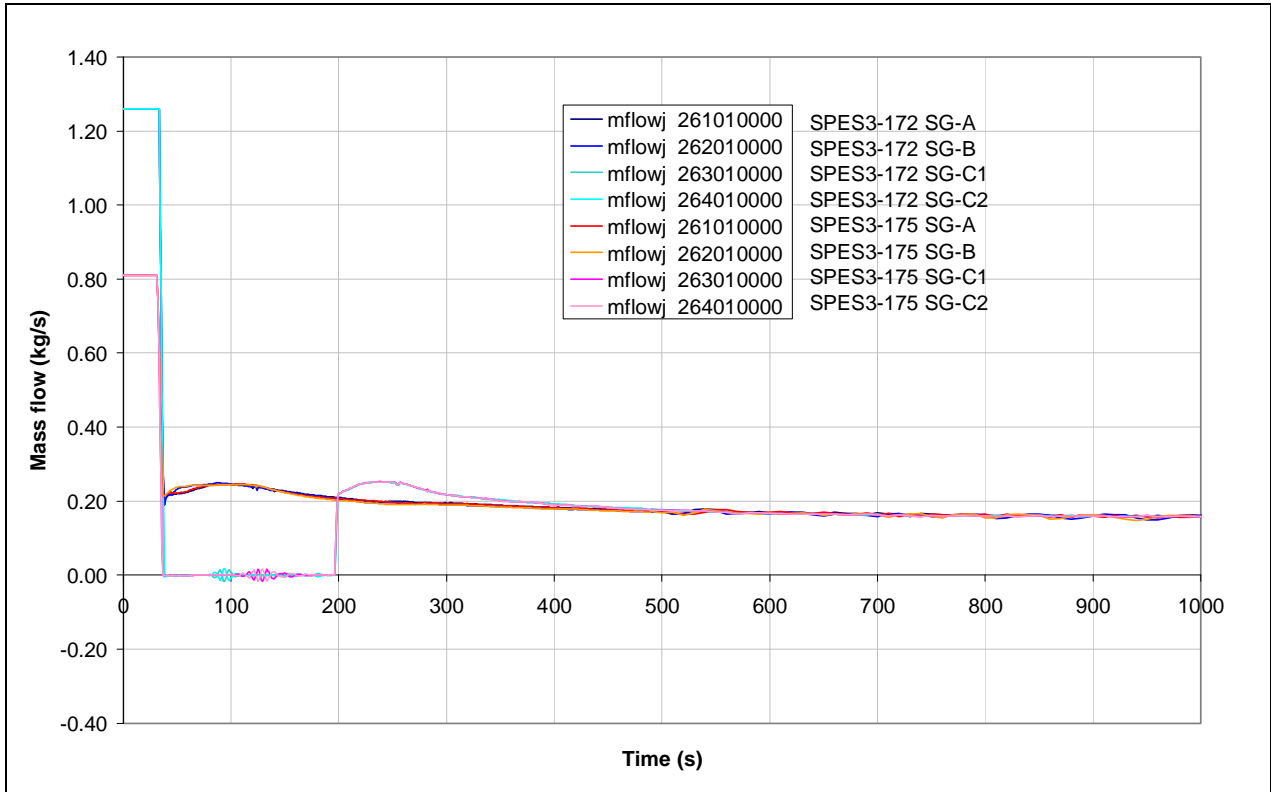
Fig.7. 35 - SPES3-172 and SPES3-175 SG ss mass flow (window)
