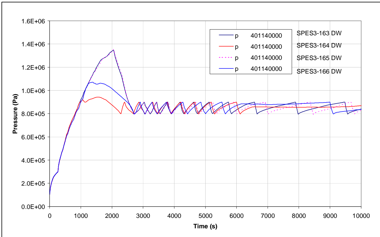
Fig.5. 15 – SPES3-163, 164, 165 and 166 DW pressure (window)
