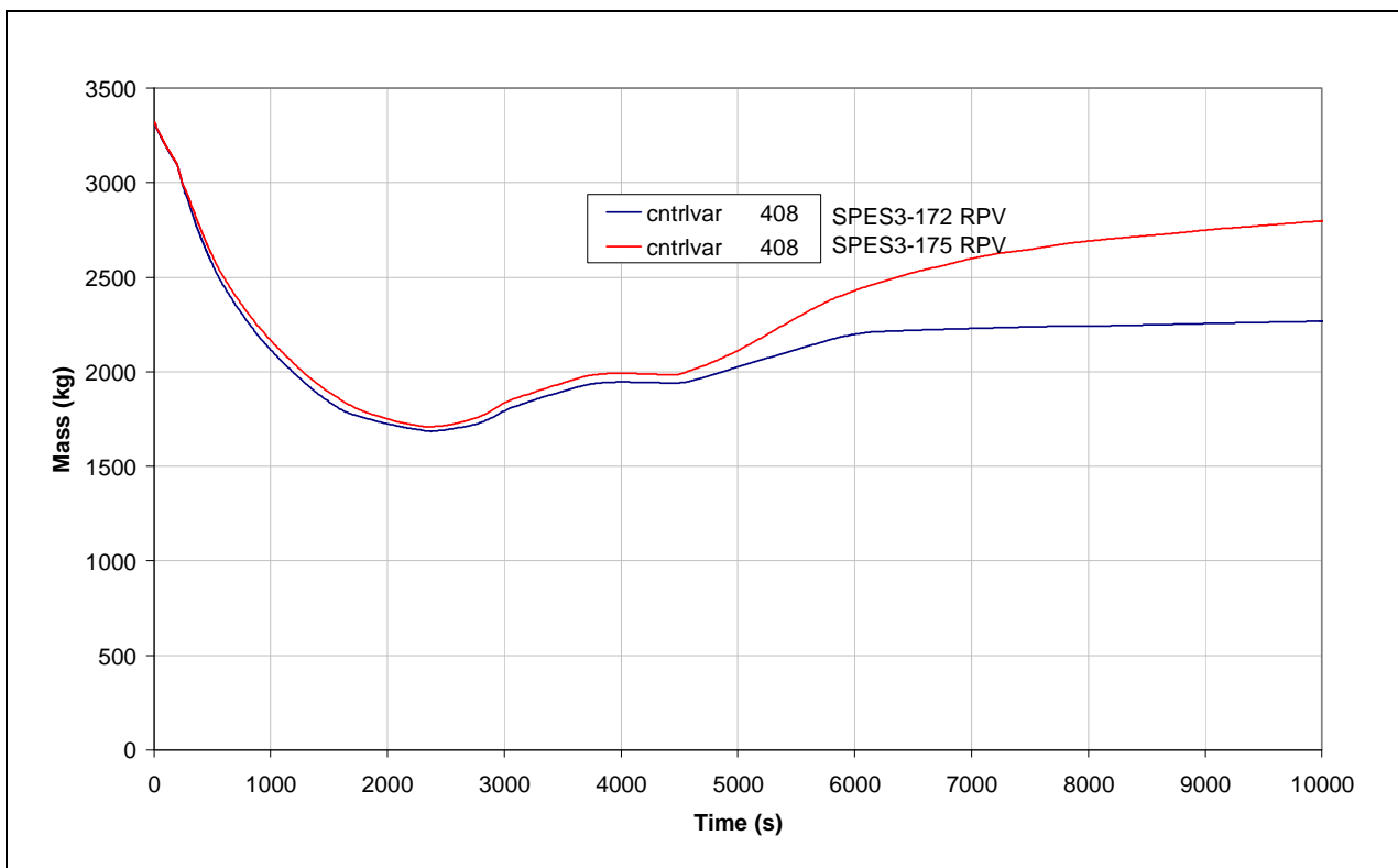
Fig.7. 52 - SPES3-172 and SPES3-175 RPV mass (window)
