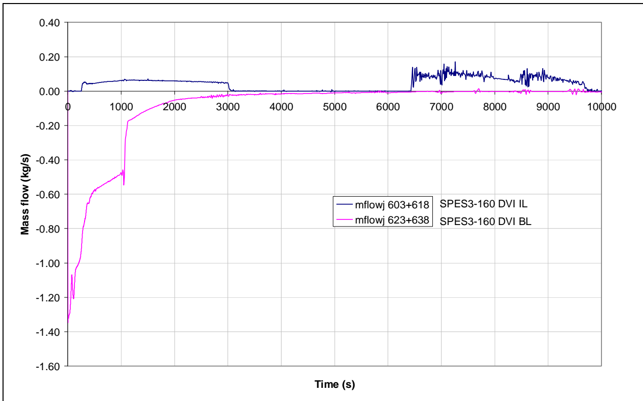
Fig.4.63 – SPES3-160 DVI line mass flow (window)
