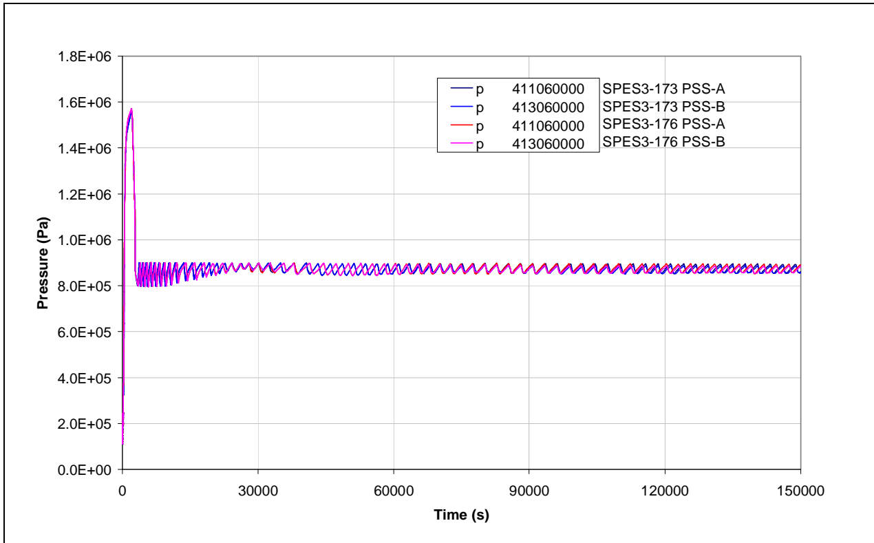
Fig.8. 27 – SPES3-173 and SPES3-176 PSS pressure
