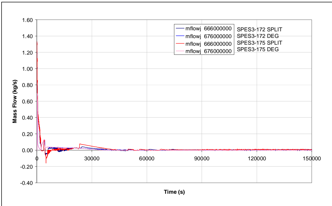
Fig.7. 4 - SPES3-172 and SPES3-175 DVI break mass flow
