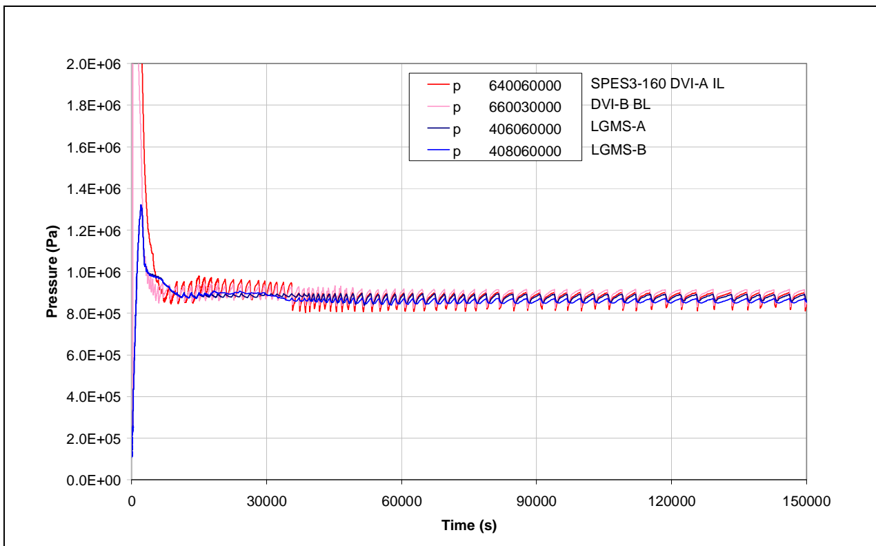
Fig.4.72 – SPES3-160 LGMS and DVI pressure (window)
