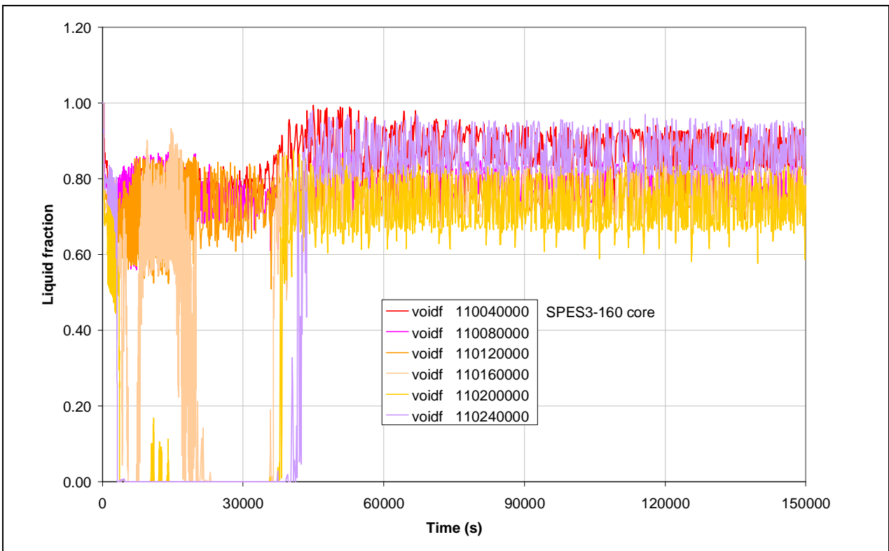
Fig.4.56 – SPES3-160 Core liquid fraction
