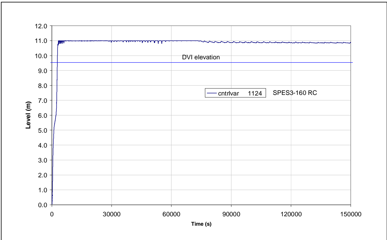
Fig.4.30 – SPES3-160 RC level
