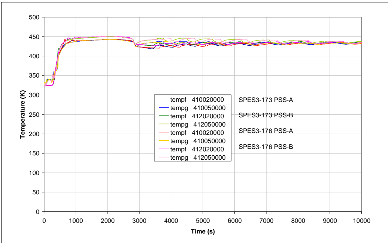
Fig.8. 41 – SPES3-173 and SPES3-176 PSS temperature (window)
