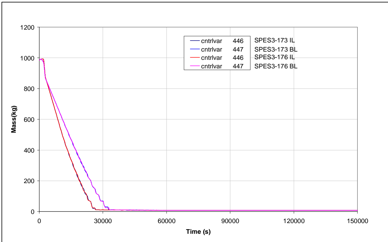
Fig.8. 81 – SPES3-173 and SPES3-176 LGMS mass
