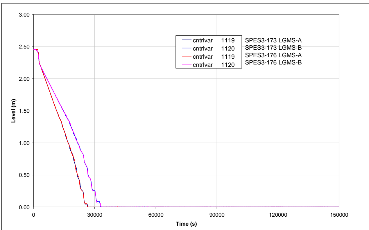
Fig.8. 80 – SPES3-173 and SPES3-176 LGMS level
