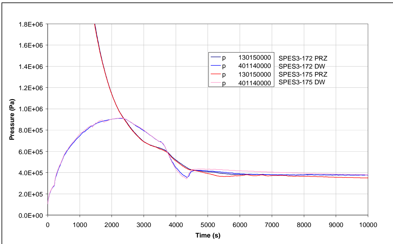
Fig.7. 14 - SPES3-172 and SPES3-175 PRZ and DW pressures (window)
