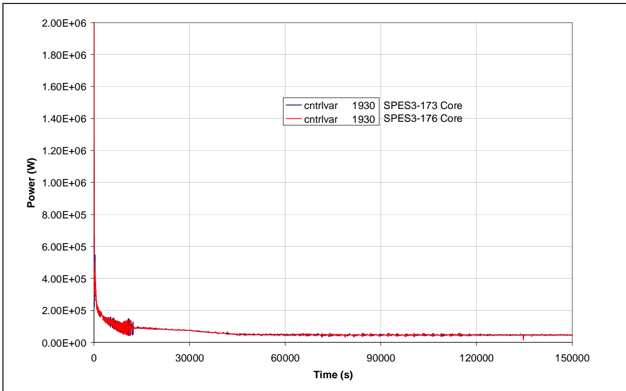
Fig.8. 45 – SPES3-173 and SPES3-176 core power
