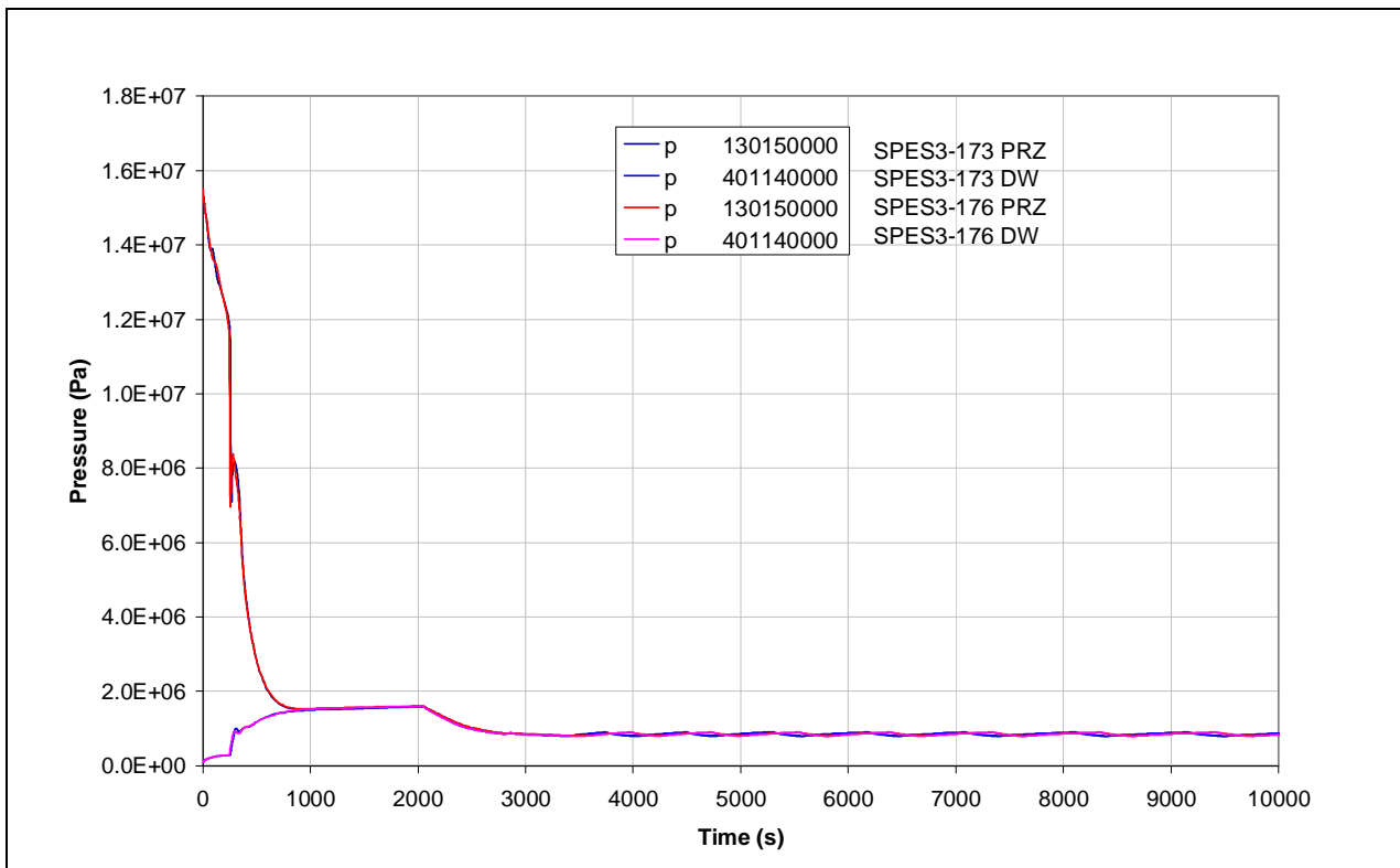
Fig.8. 14 – SPES3-173 and SPES3-176 PRZ and DW pressures
