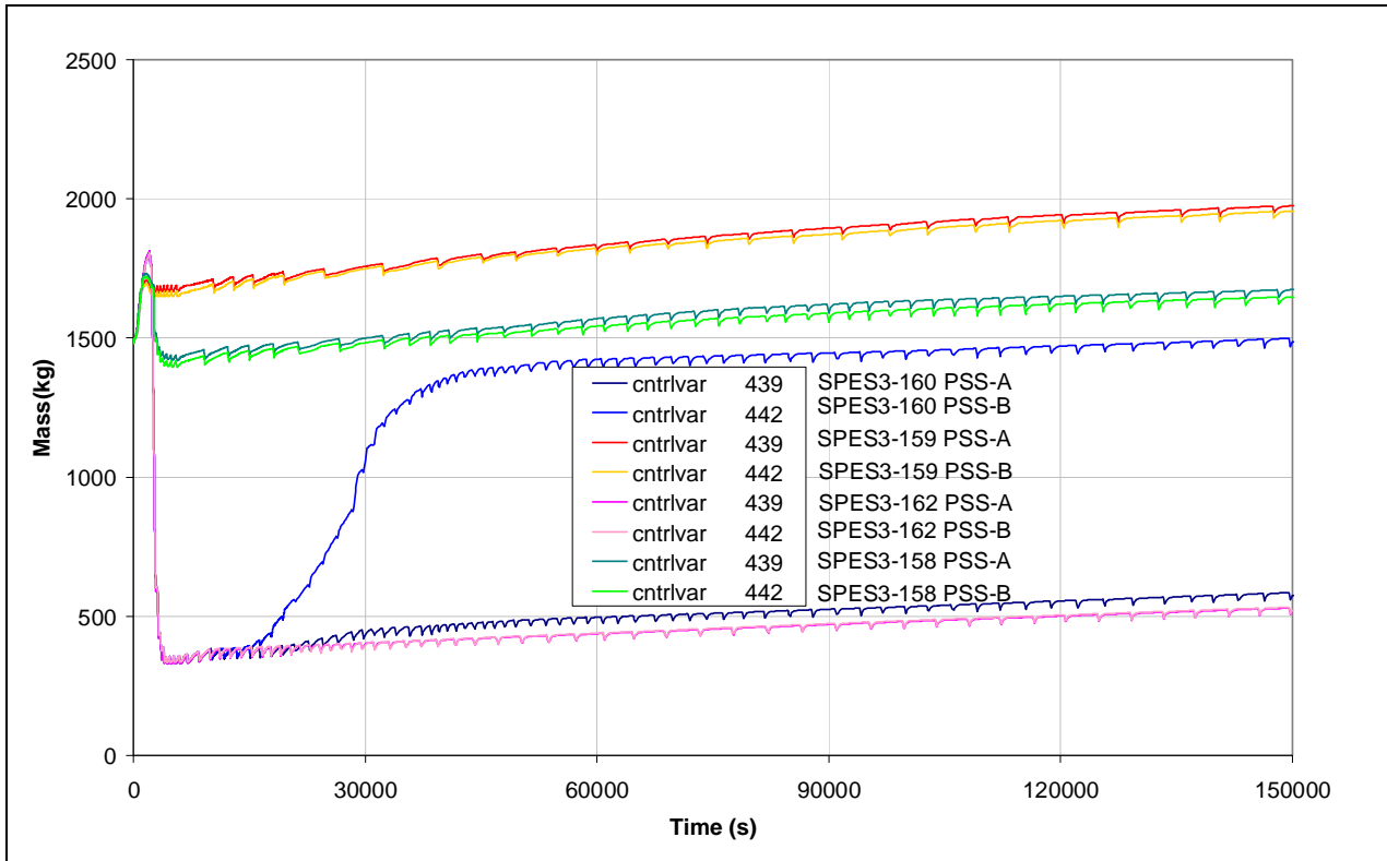
Fig.5. 7 – SPES3-159, 162, 158 and 160 PSS mass
