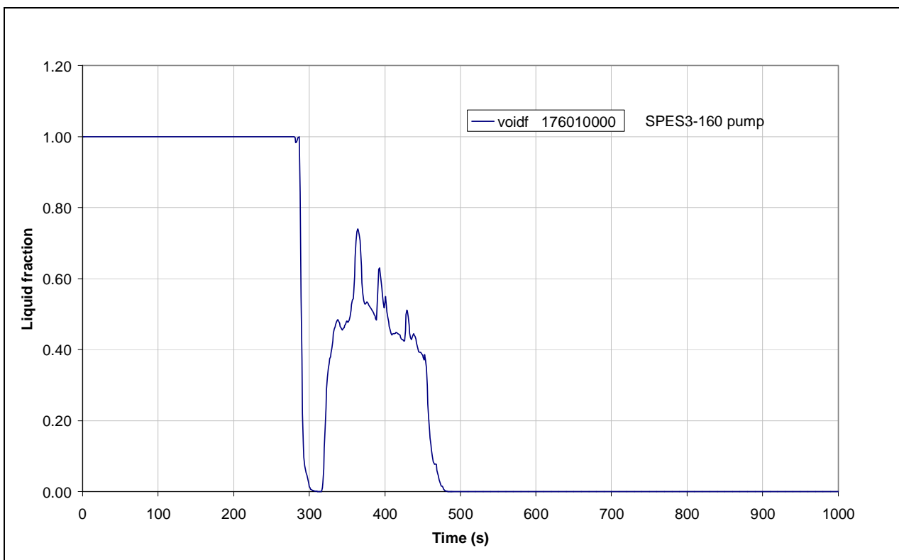
Fig.4.46 – SPES3-160 pump inlet liquid fraction
