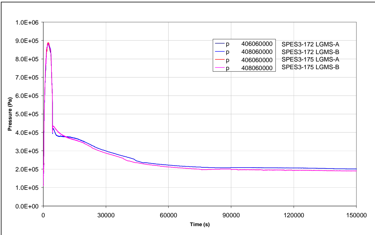
Fig.7. 25 - SPES3-172 and SPES3-175 LGMS pressure
