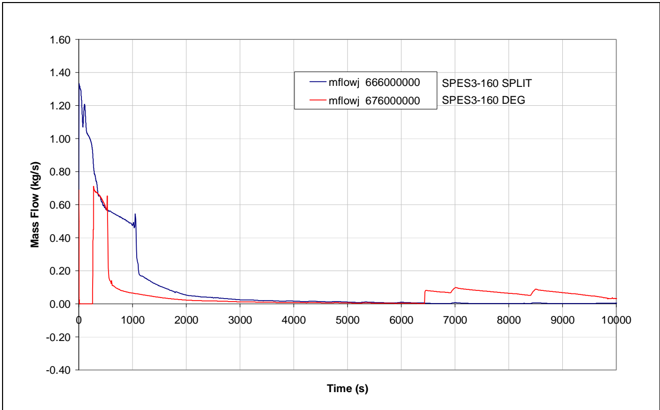
Fig.4.1 – SPES3-160 DVI line break flow (window)
