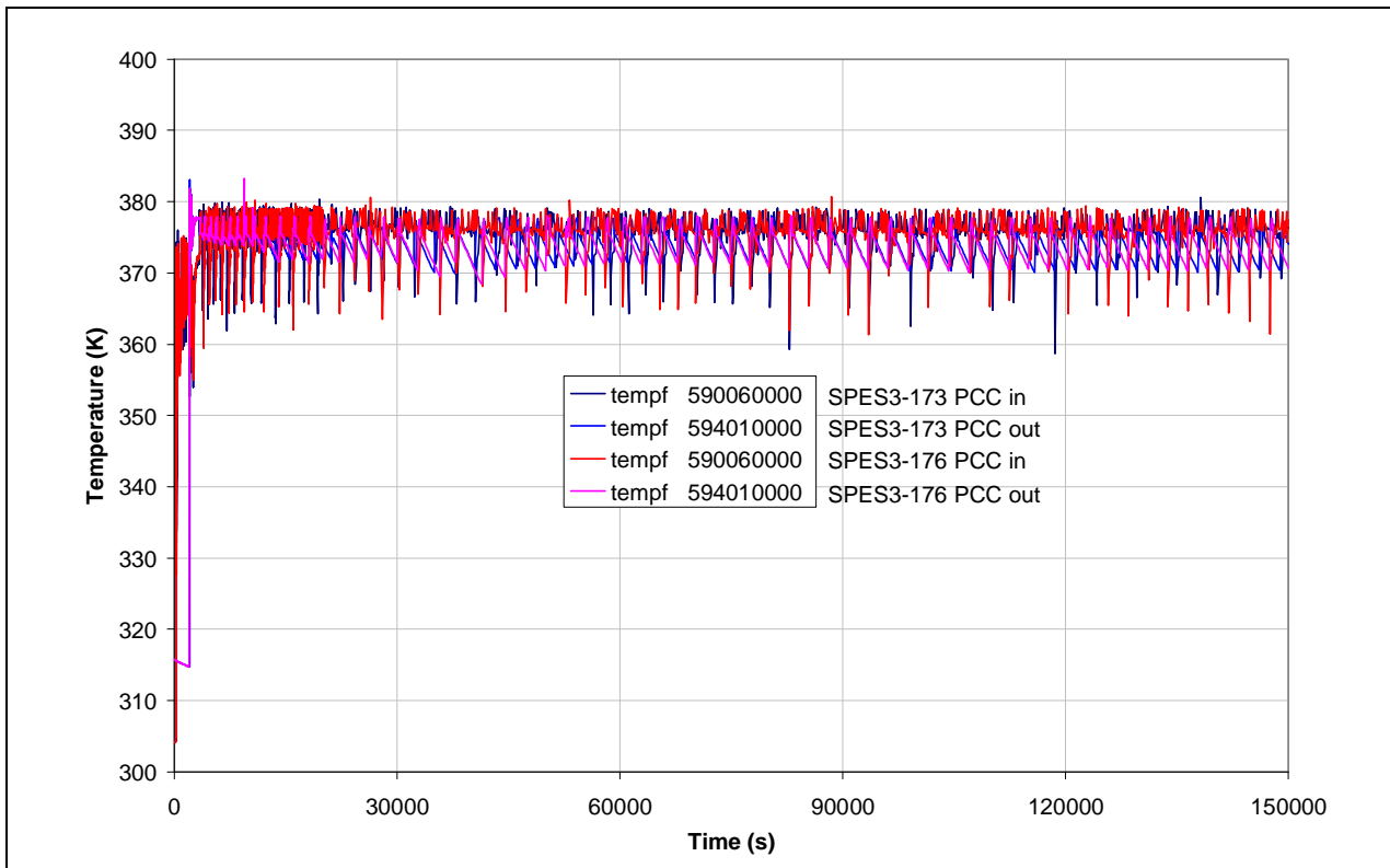
Fig.8. 77 – SPES3-173 and SPES3-176 PCC inlet and outlet temperature
