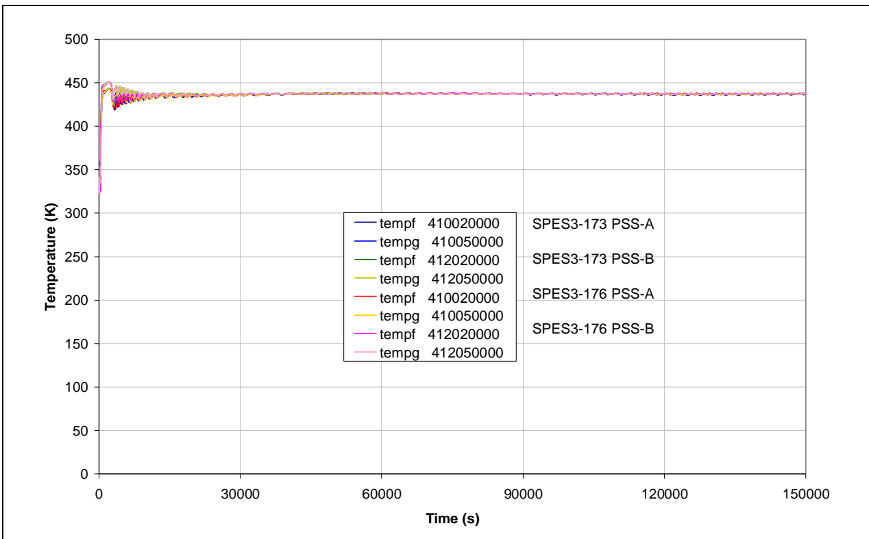
Fig.8. 42 – SPES3-173 and SPES3-176 PSS temperature
