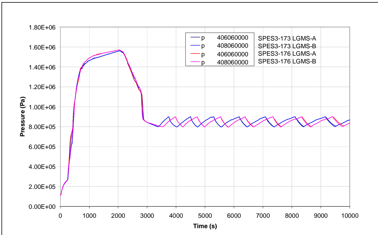
Fig.8. 28 – SPES3-173 and SPES3-176 LGMS pressure (window)
