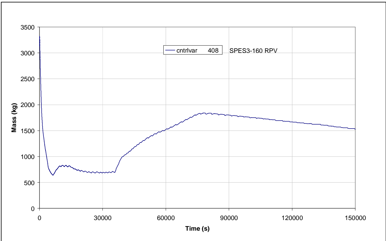
Fig.4.61 – SPES3-160 RPV mass
