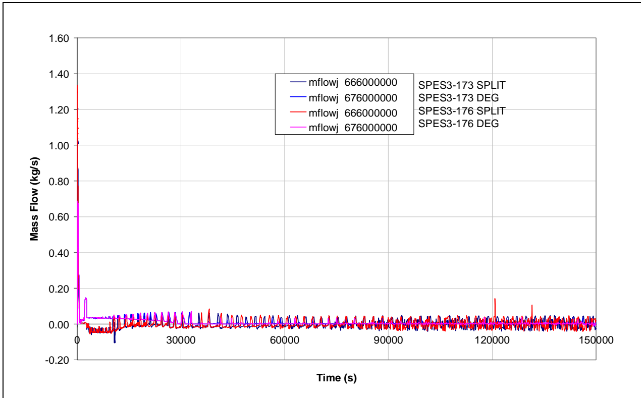
Fig.8. 3 – SPES3-173 and SPES3-176 DVI line break flow
