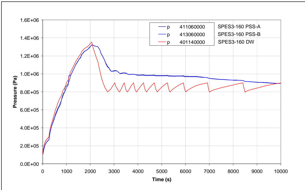
Fig.4.23 – SPES3-160 PSS and DW pressure (window)
