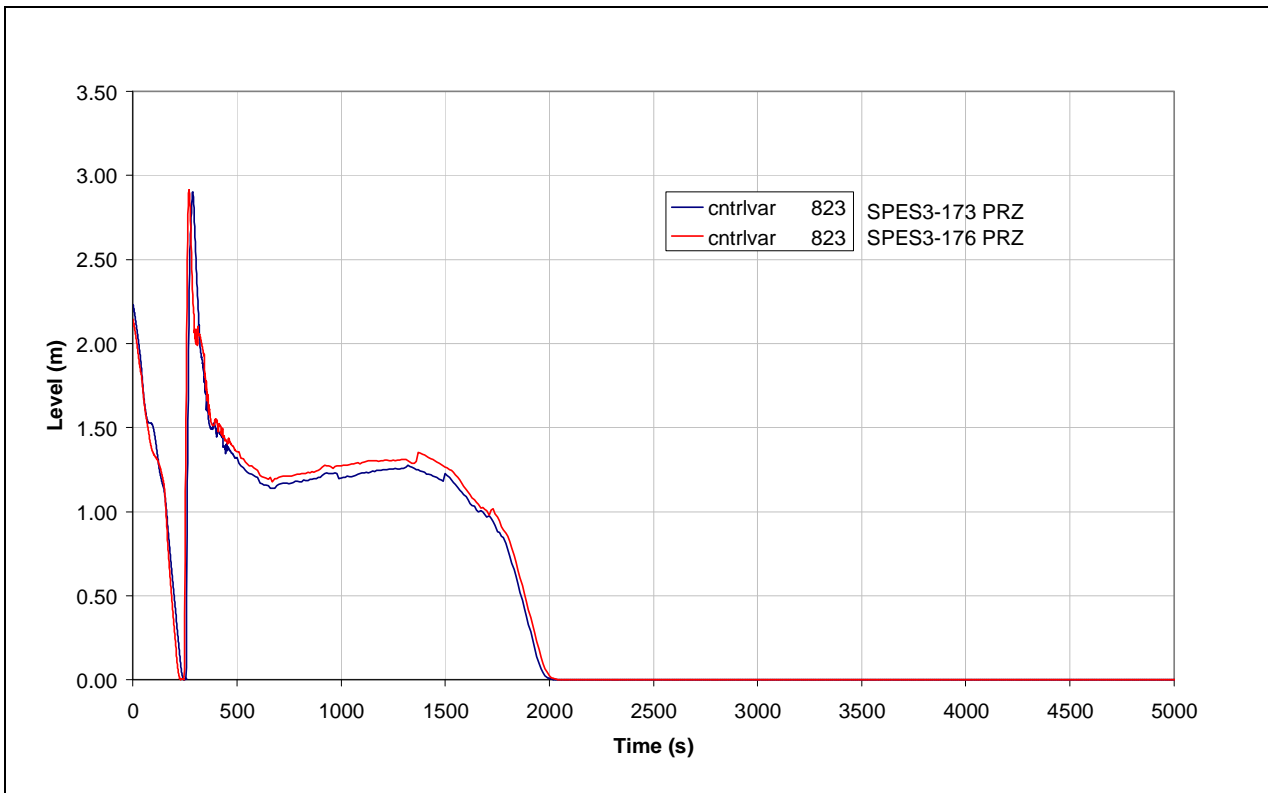
Fig.8. 53 – SPES3-173 and SPES3-176 PRZ level
