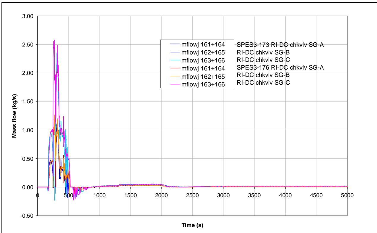
Fig.8. 58 – SPES3-173 and SPES3-176 RI-DC check valve mass flow (window)
