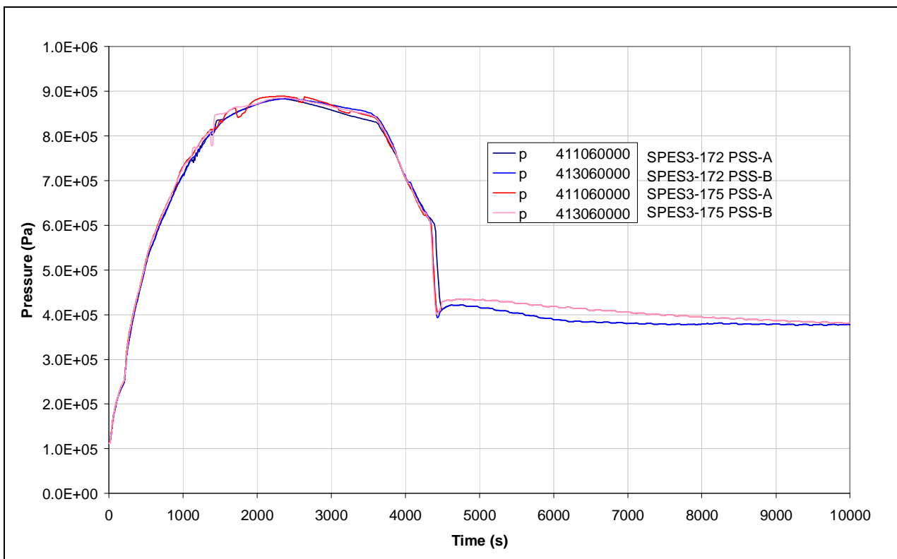
Fig.7. 22 - SPES3-172 and SPES3-175 PSS pressure (window)
