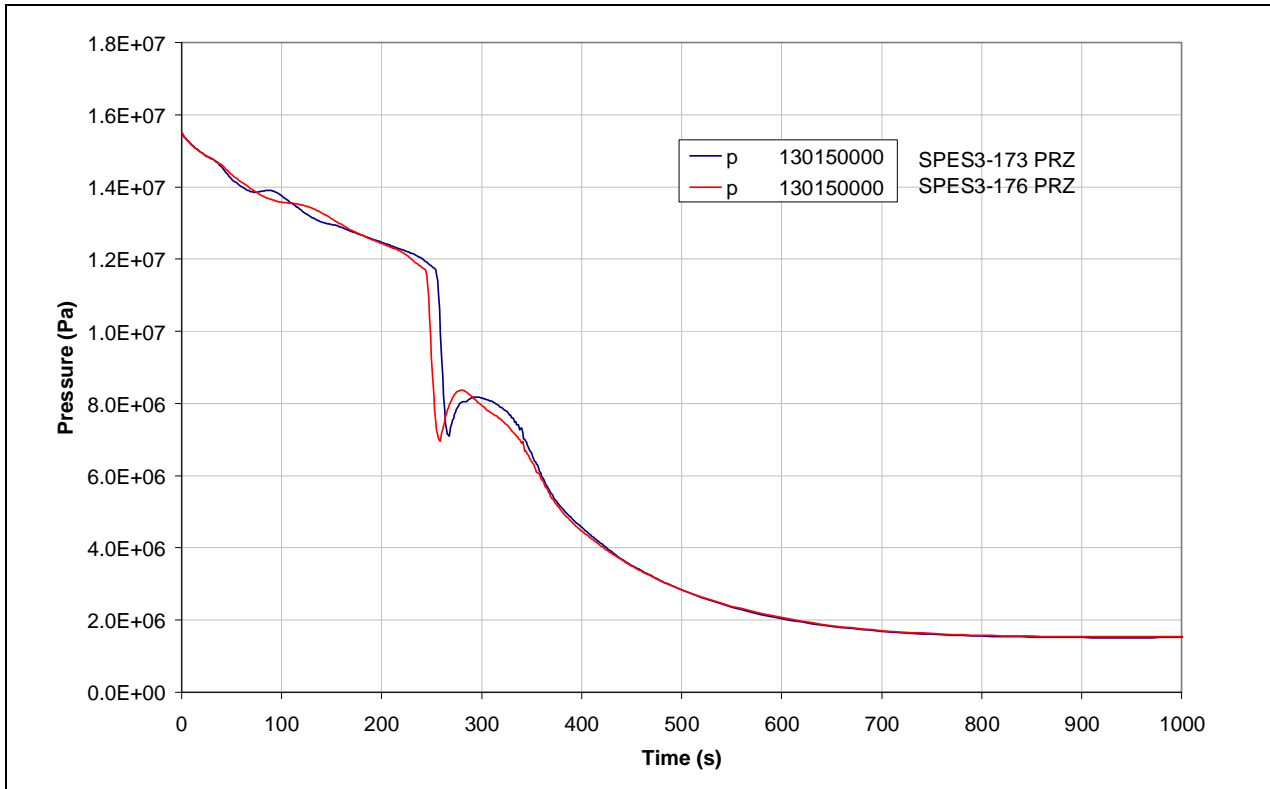
Fig.8. 15 – SPES3-173 and SPES3-176 PRZ pressure (window)
