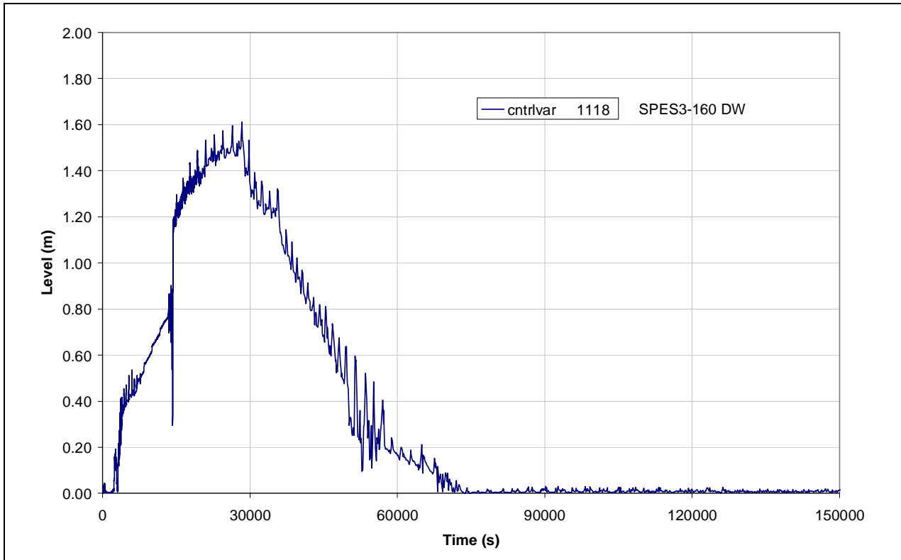
Fig.4.31 – SPES3-160 DW level
