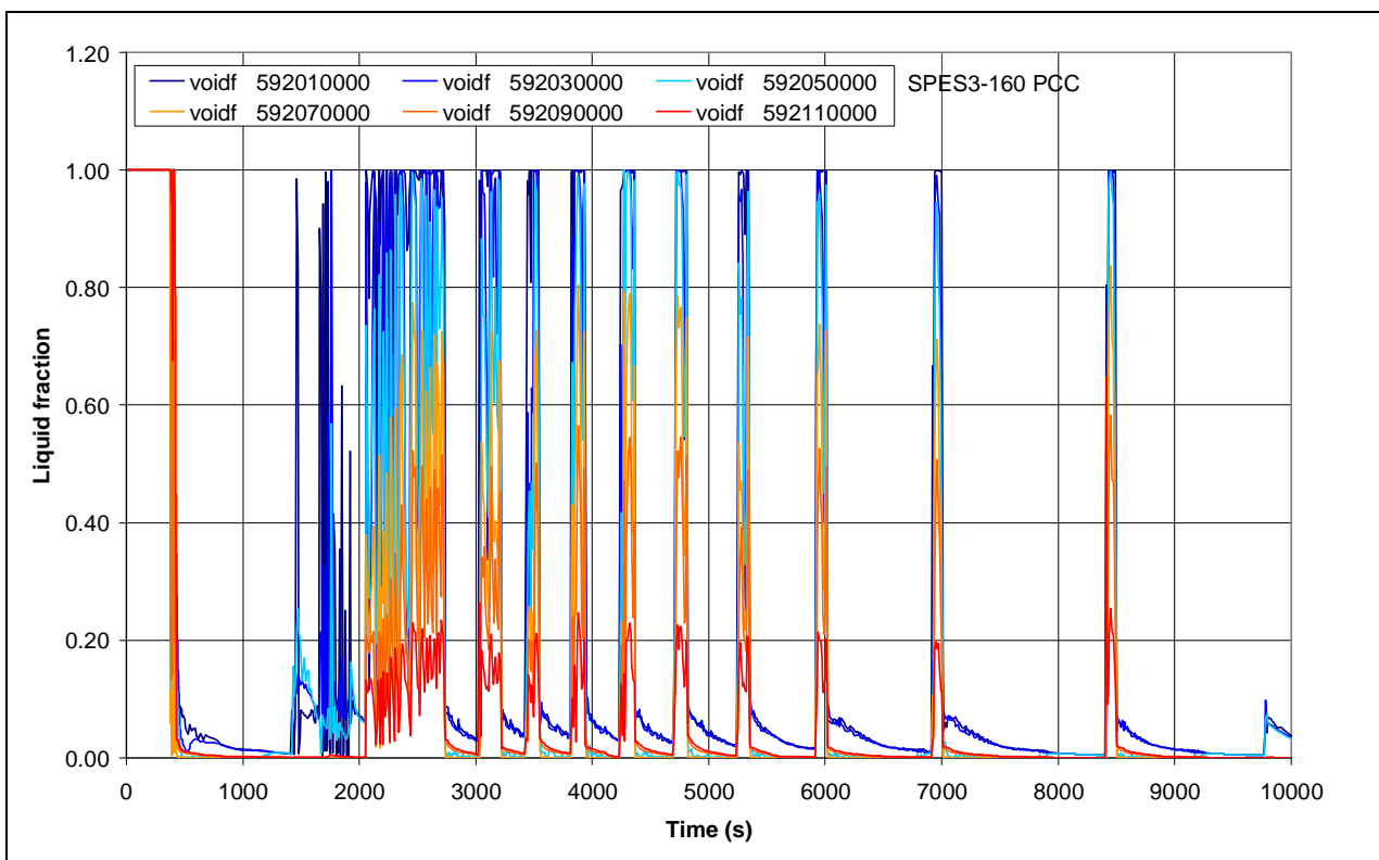
Fig.4.68 – SPES3-160 PCC liquid void fraction (window)
