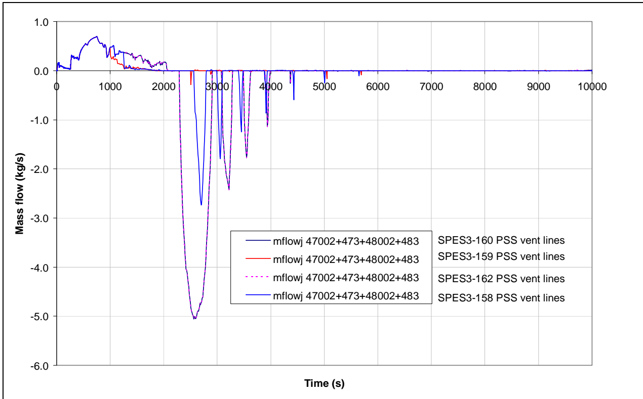
Fig.5. 5 – SPES3-159, 162, 158 and 160 PSS to DW mass flow (window)
