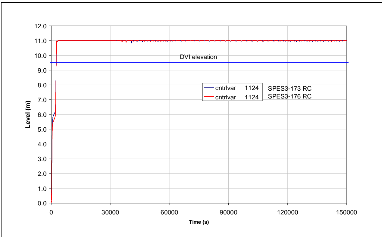
Fig.8. 38 – SPES3-173 and SPES3-176 RC level
