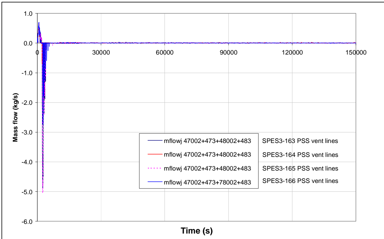
Fig.5. 20 – SPES3-163, 164, 165 and 166 PSS to DW mass flow
