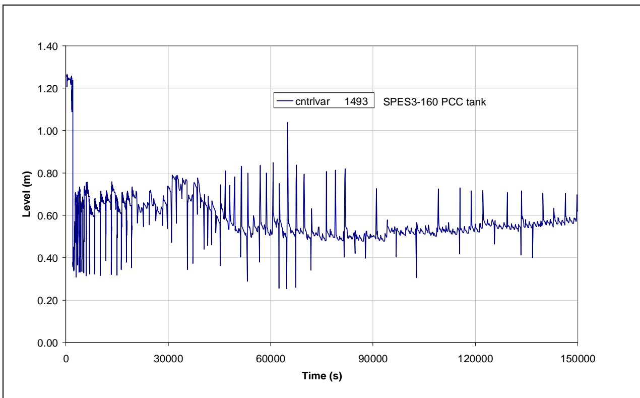
Fig.4.66 – SPES3-160 PCC tank level
