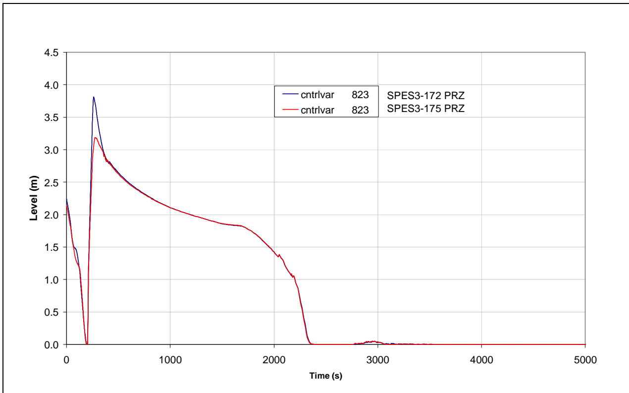
Fig.7. 45 - SPES3-172 and SPES3-175 PRZ level (window)
