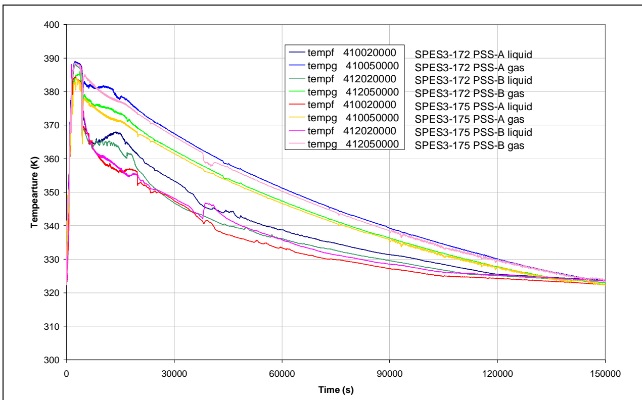
Fig.7. 30 - SPES3-172 and SPES3-175 PSS temperatures
