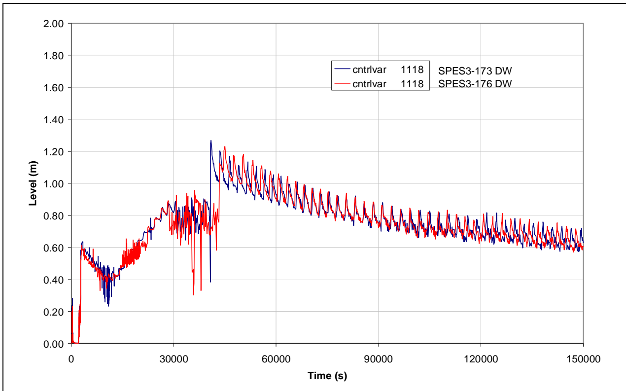
Fig.8. 39 – SPES3-173 and SPES3-176 DW level
