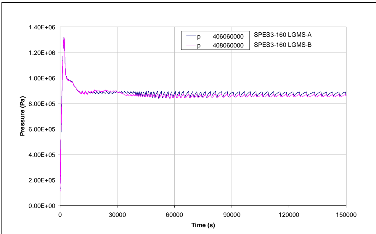
Fig.4.22 – SPES3-160 LGMS pressure
