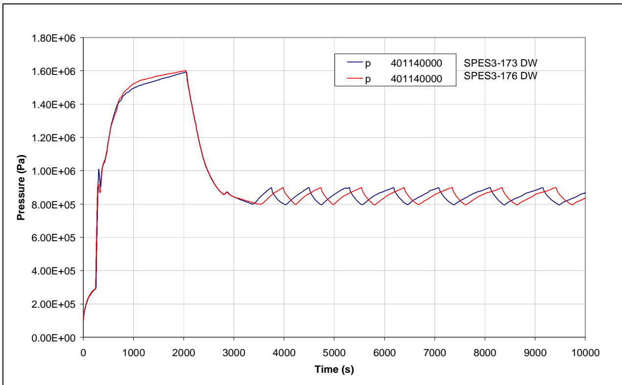
Fig.8. 18 – SPES3-173 and SPES3-176 DW pressure (window)
