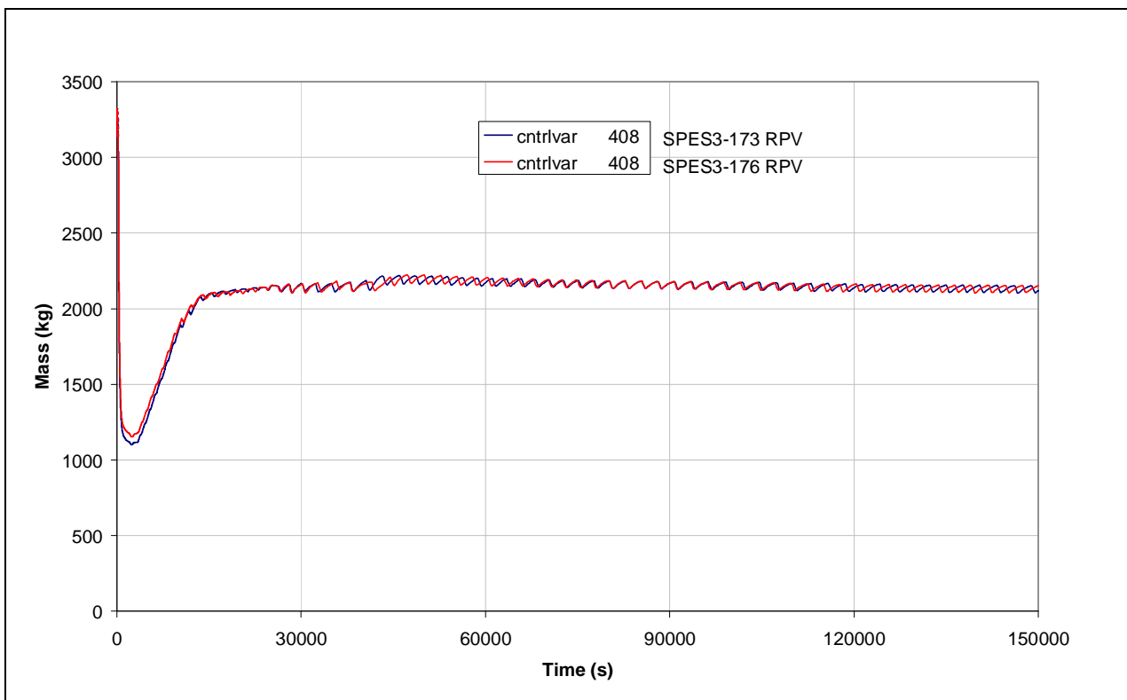
Fig.8. 60 – SPES3-173 and SPES3-176 RPV mass
