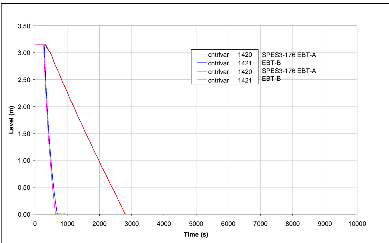
Fig.8. 62 – SPES3-173 and SPES3-176 EBT level
