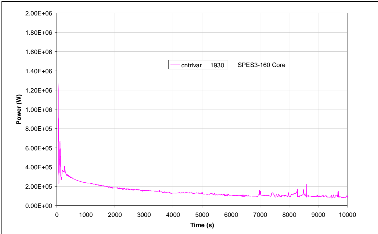
Fig.4.37 – SPES3-160 core power (window)
