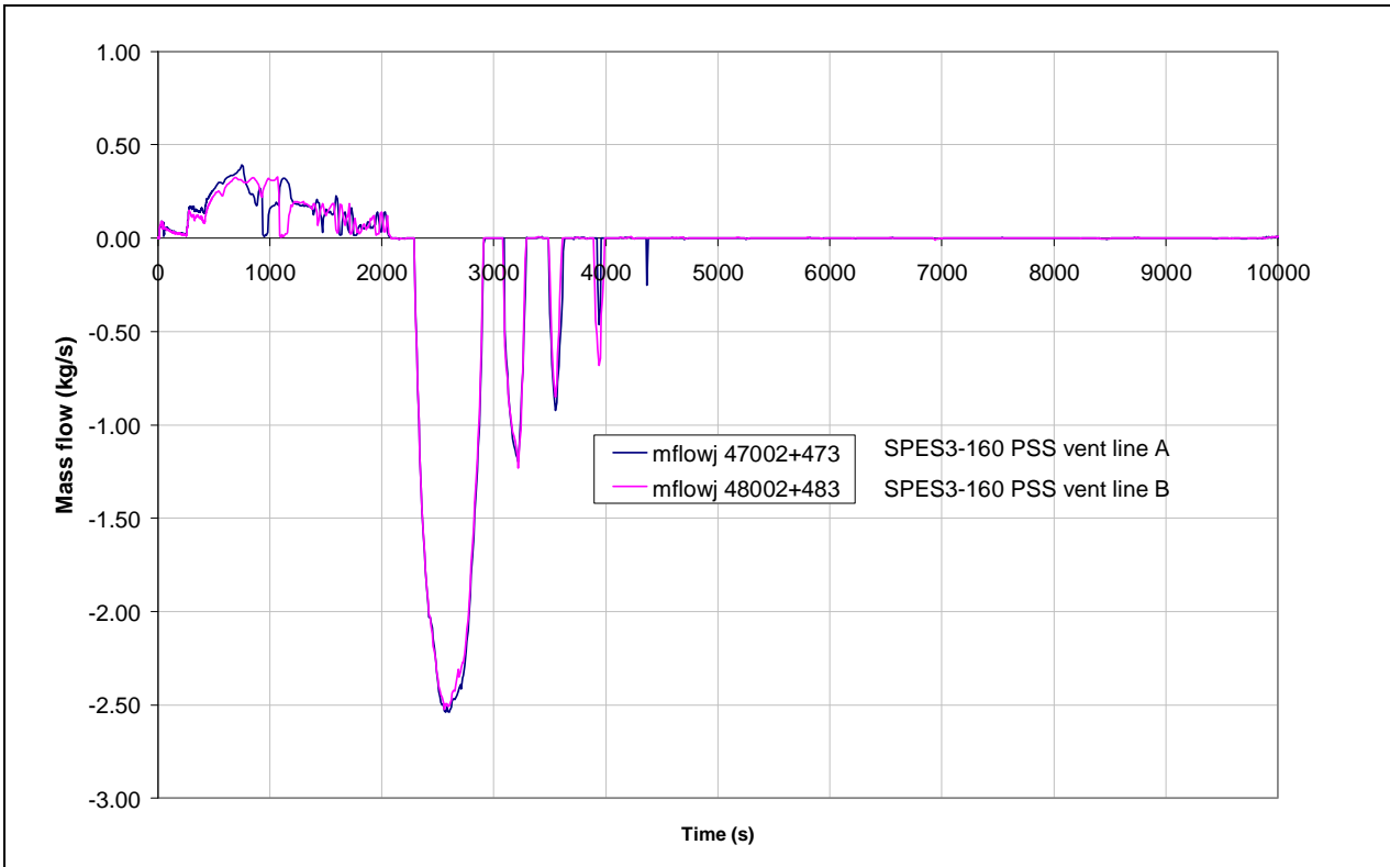
Fig.4.15 – SPES3-160 PSS to DW flow (window)
