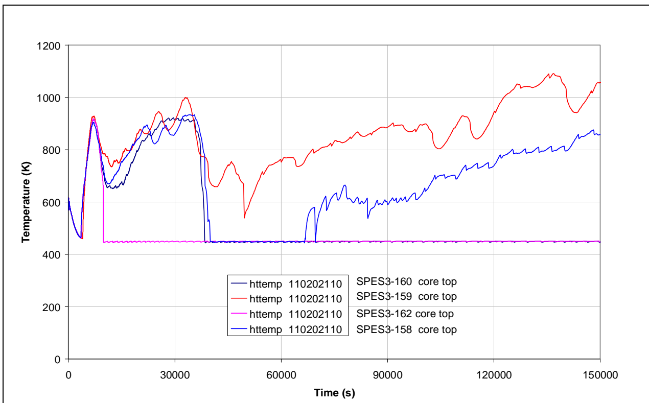
Fig.5. 14 – SPES3-159, 162, 158 and 160 Core heater rod clad surface temperature (hot rods)
