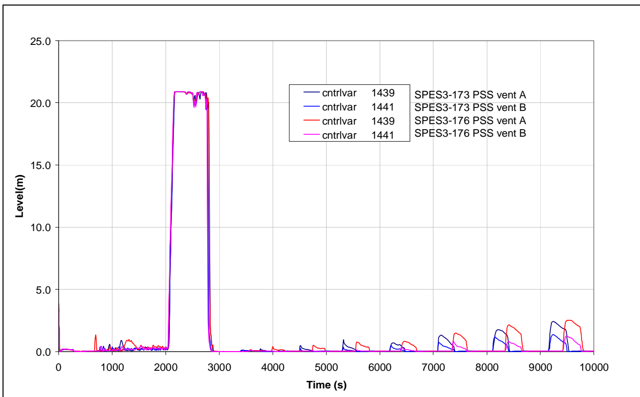
Fig.8. 32 – SPES3-173 and SPES3-176 PSS vent pipe level (window)
