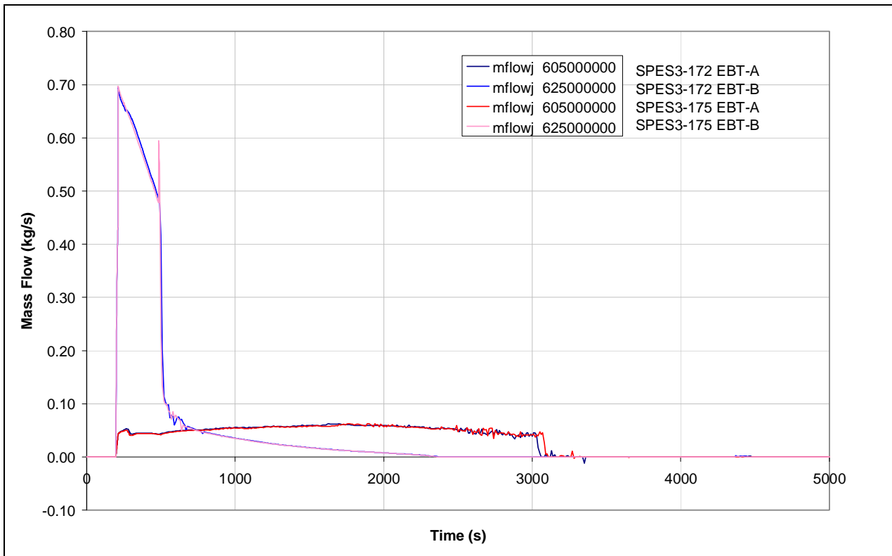
Fig.7. 5 - SPES3-172 and SPES3-175 EBT mass flow (window)
