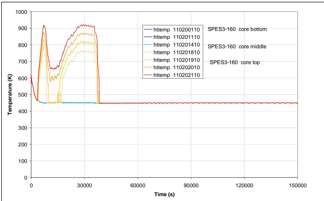
Fig.4.60 – SPES3-160 Core heater rod clad surface temperatures (hot rods)
