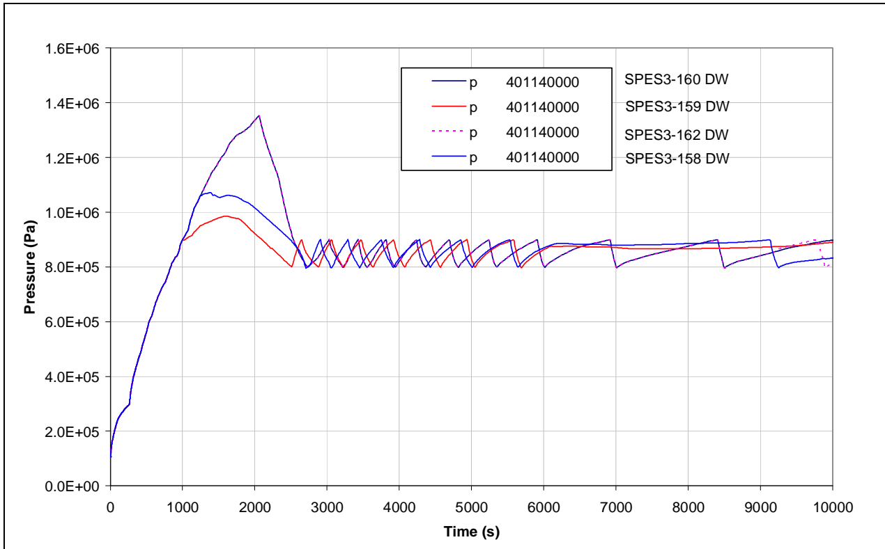
Fig.5. 1 – SPES3-159, 162, 158 and 160 DW pressure (window)
