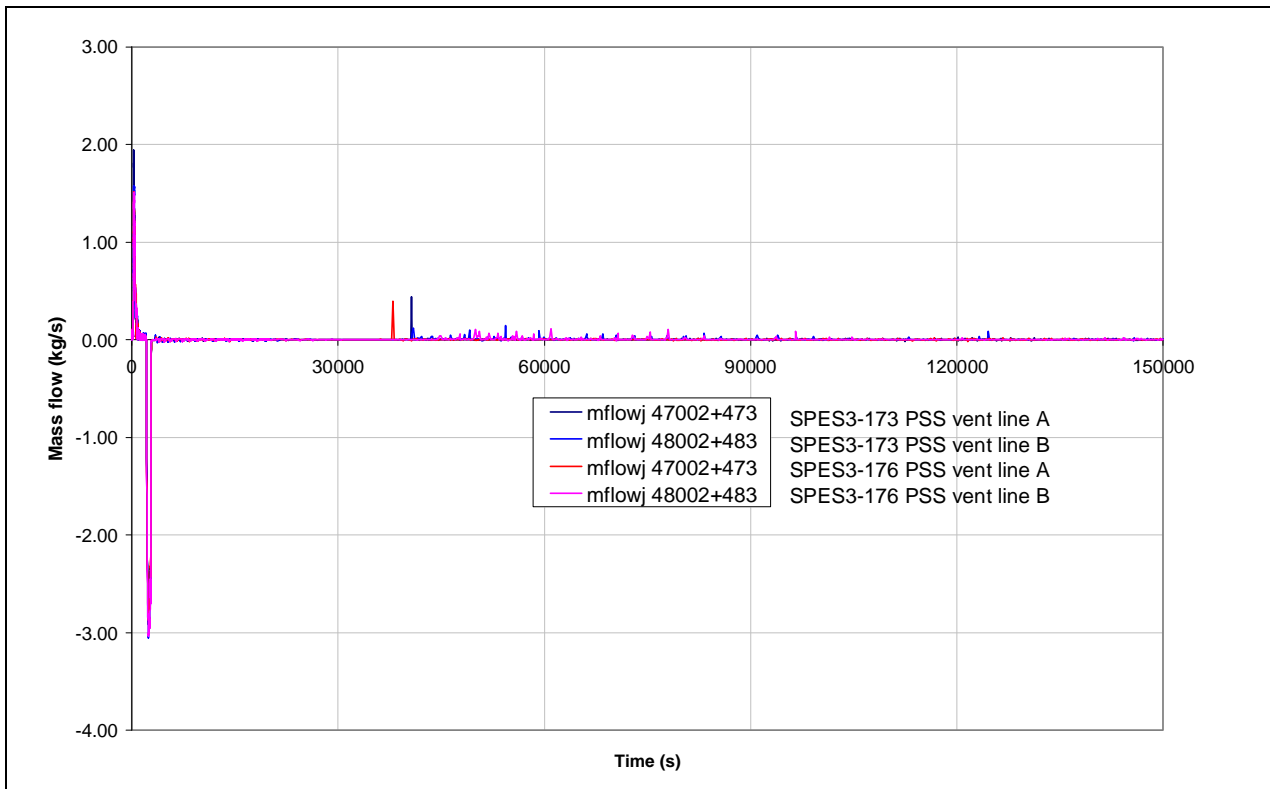
Fig.8. 23 – SPES3-173 and SPES3-176 PSS to DW mass flow
