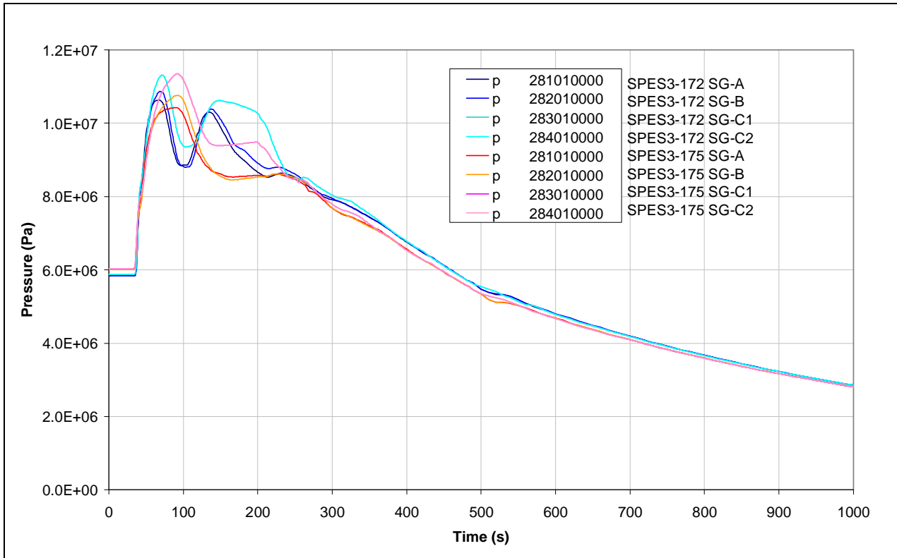
Fig.7. 41 - SPES3-172 and SPES3-175 SG ss outlet pressure (window)
