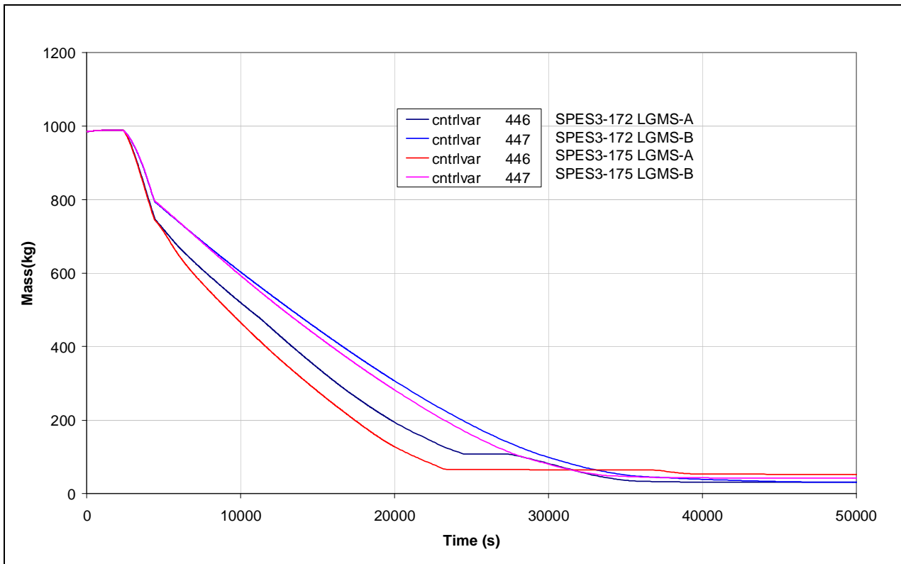
Fig.7. 71 - SPES3-172 and SPES3-175 LGMS mass (window)
