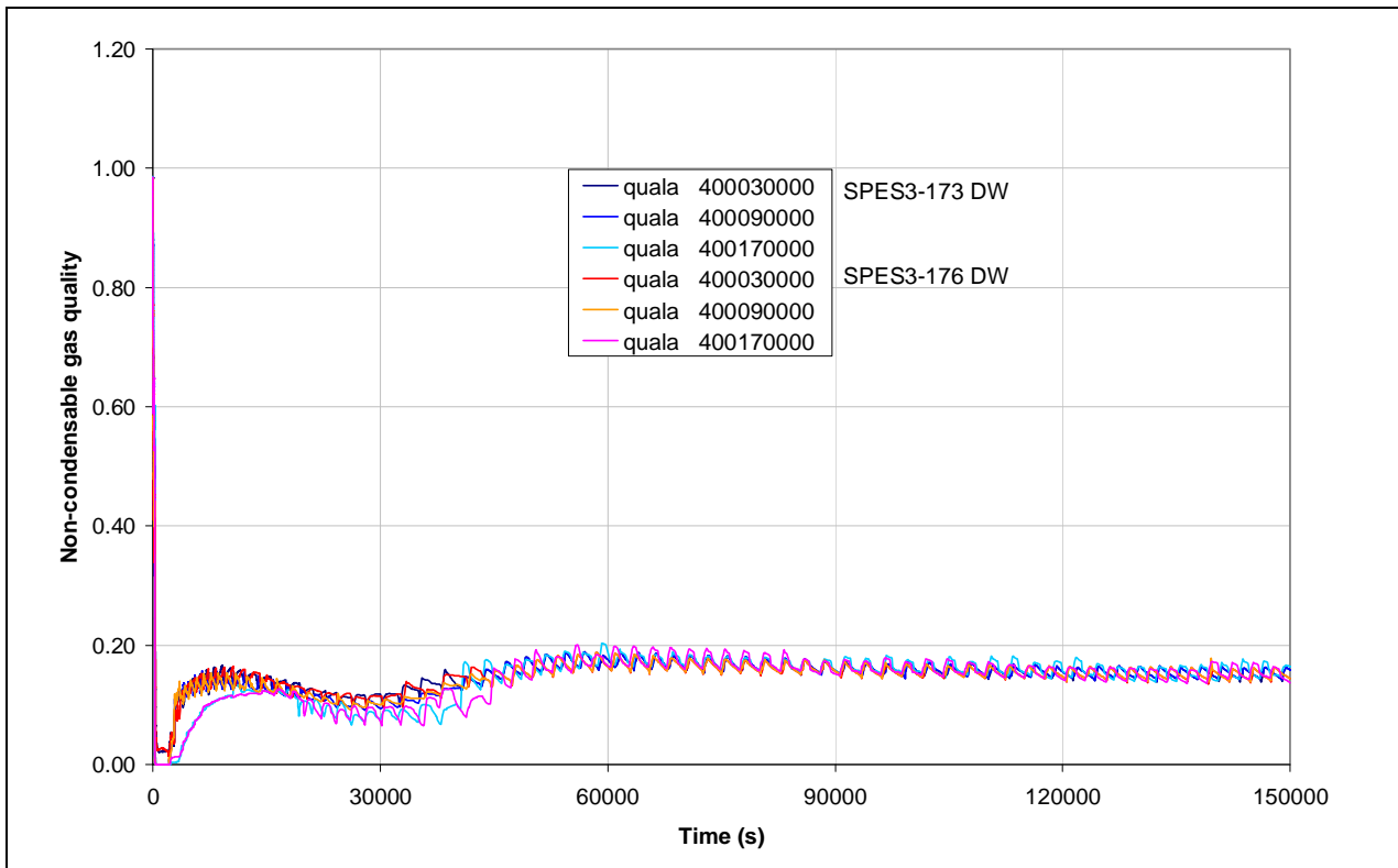
Fig.8. 25 – SPES3-173 and SPES3-176 DW non-condensable quality
