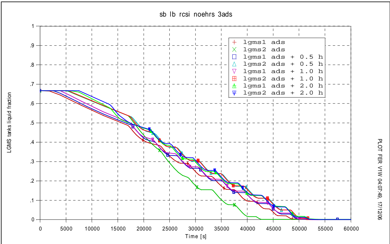
Fig.5. 33 – IRIS plant LGMS mass
