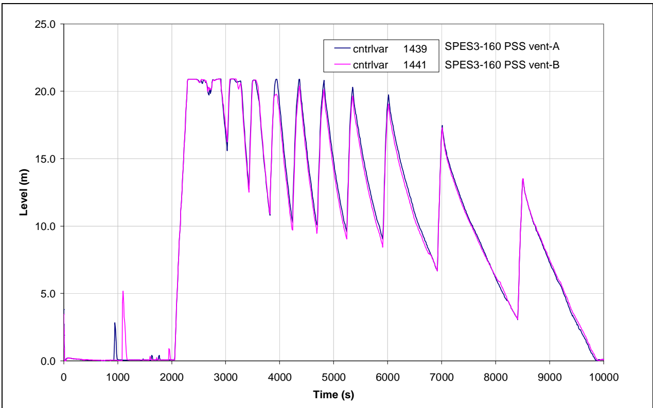
Fig.4.25 – SPES3-160 PSS vent pipe level (window)
