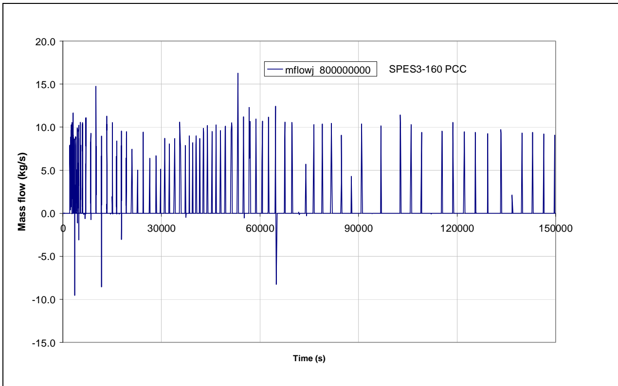
Fig.4.65 – SPES3-160 PCC mass flow
