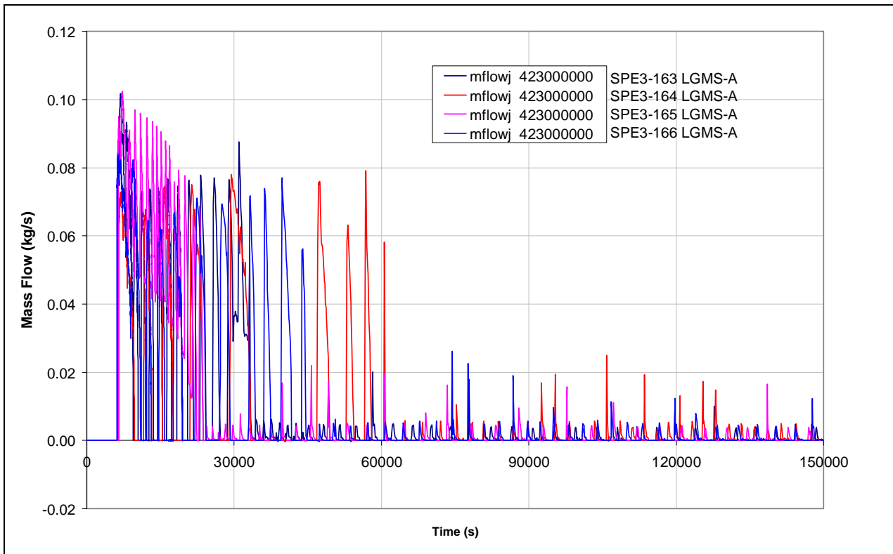
Fig.5. 23 – SPES3-163, 164, 165 and 166 LGMS to DVI line mass flow (intact loop)
