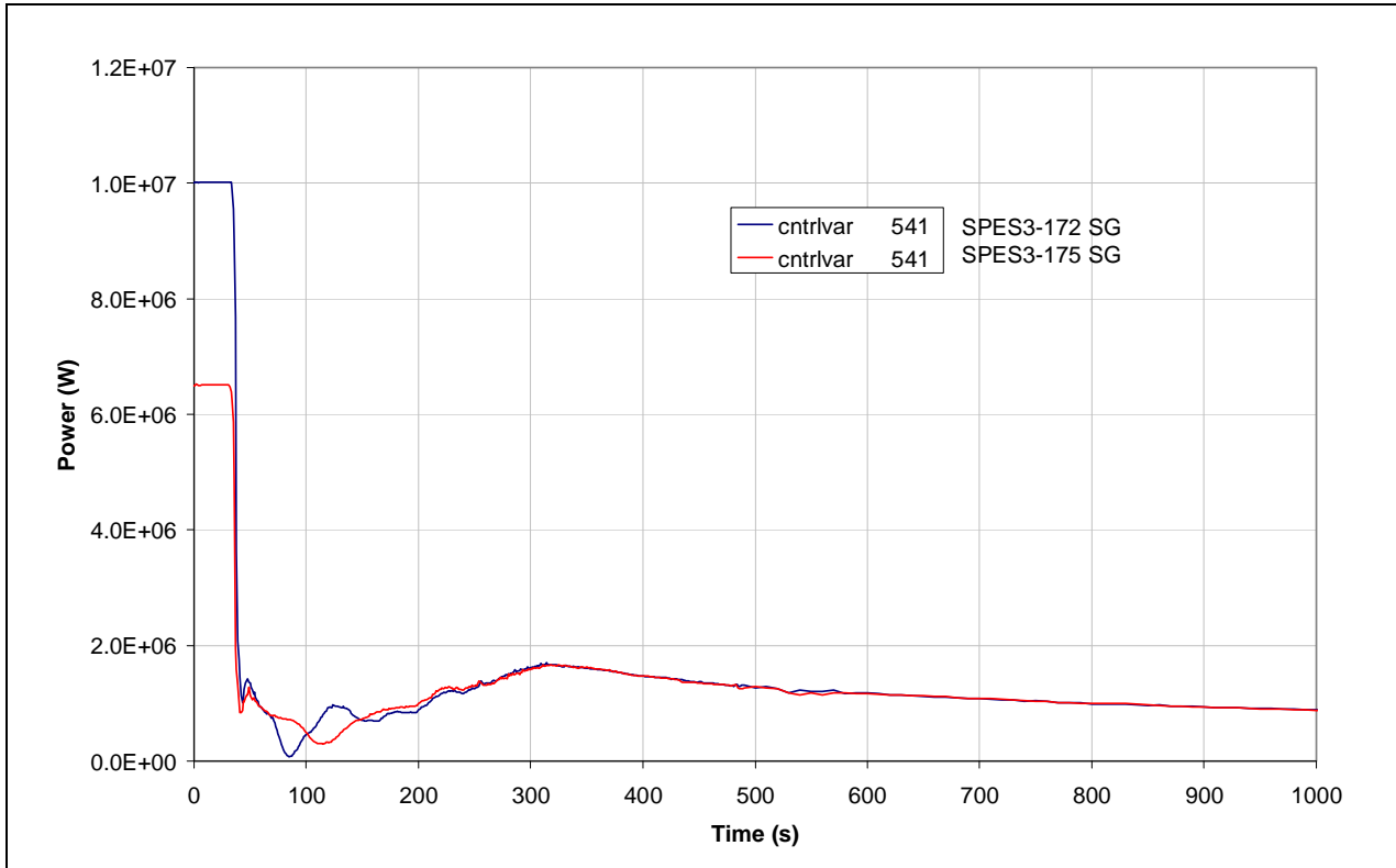
Fig.7. 33 - SPES3-172 and SPES3-175 SG power (window)
