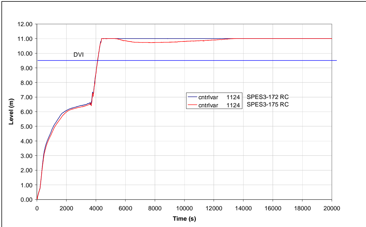
Fig.7. 7 - SPES3-172 and SPES3-175 RC level (window)
