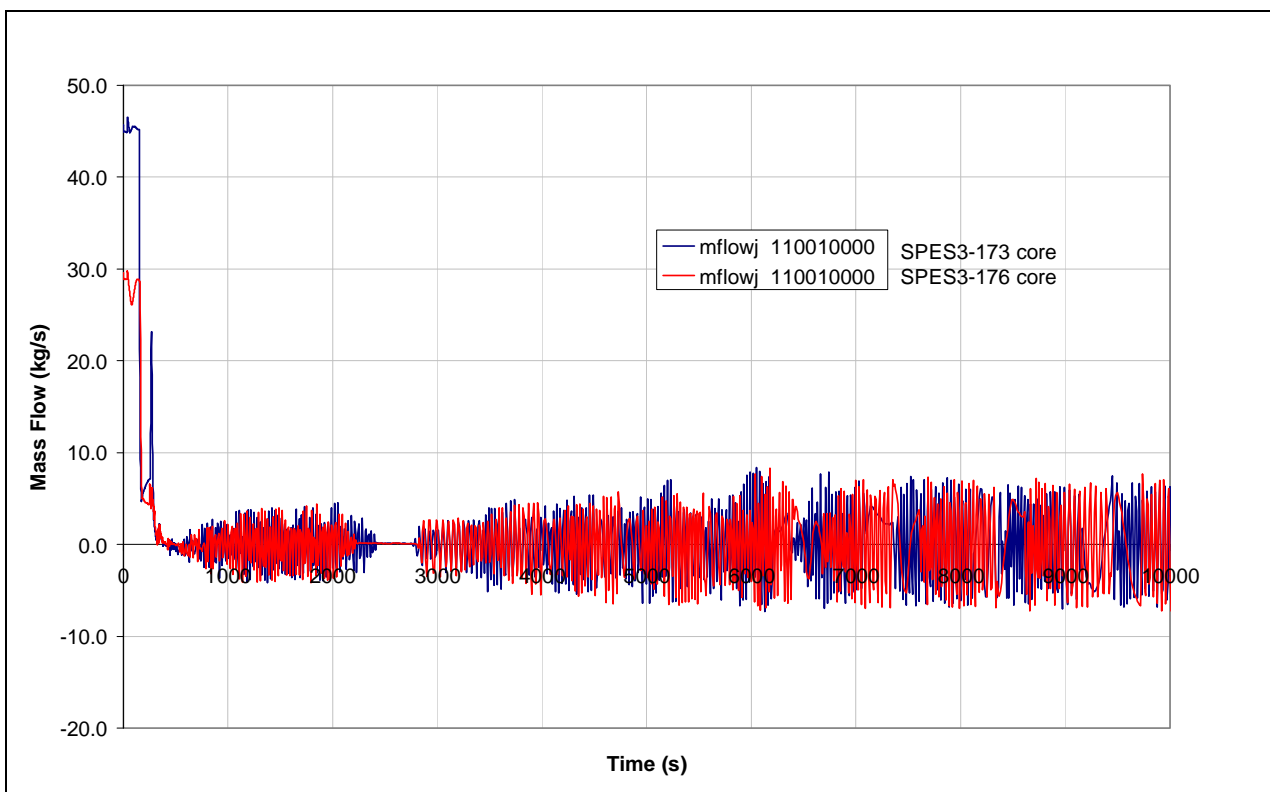
Fig.8. 56 – SPES3-173 and SPES3-176 core inlet flow (window)
