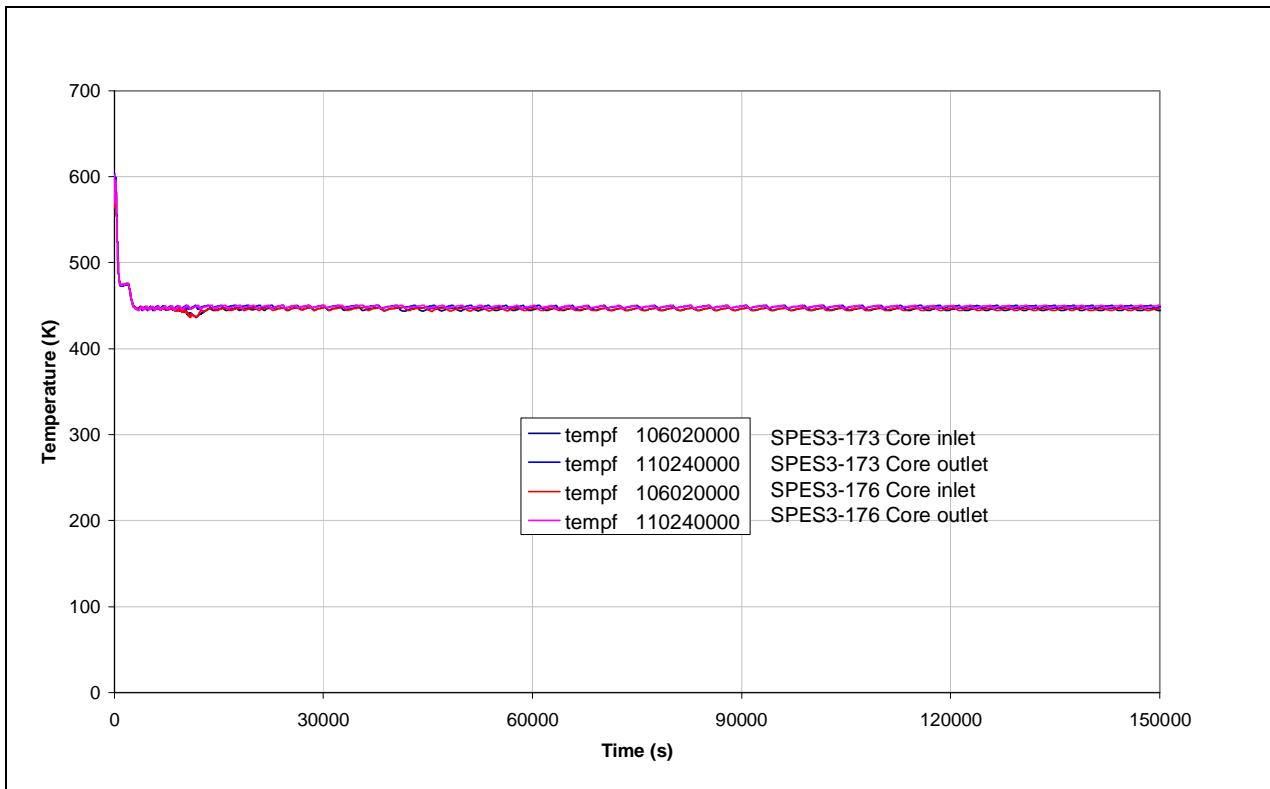
Fig.8. 70 – SPES3-173 and SPES3-176 Core inlet and outlet temperatures
