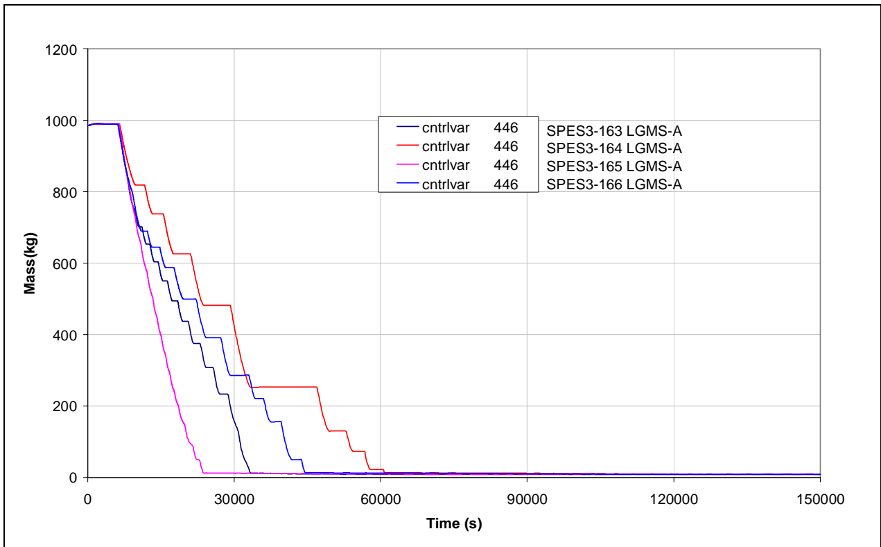
Fig.5. 22 – SPES3-163, 164, 165 and 166 LGMS-A mass (intact loop)
