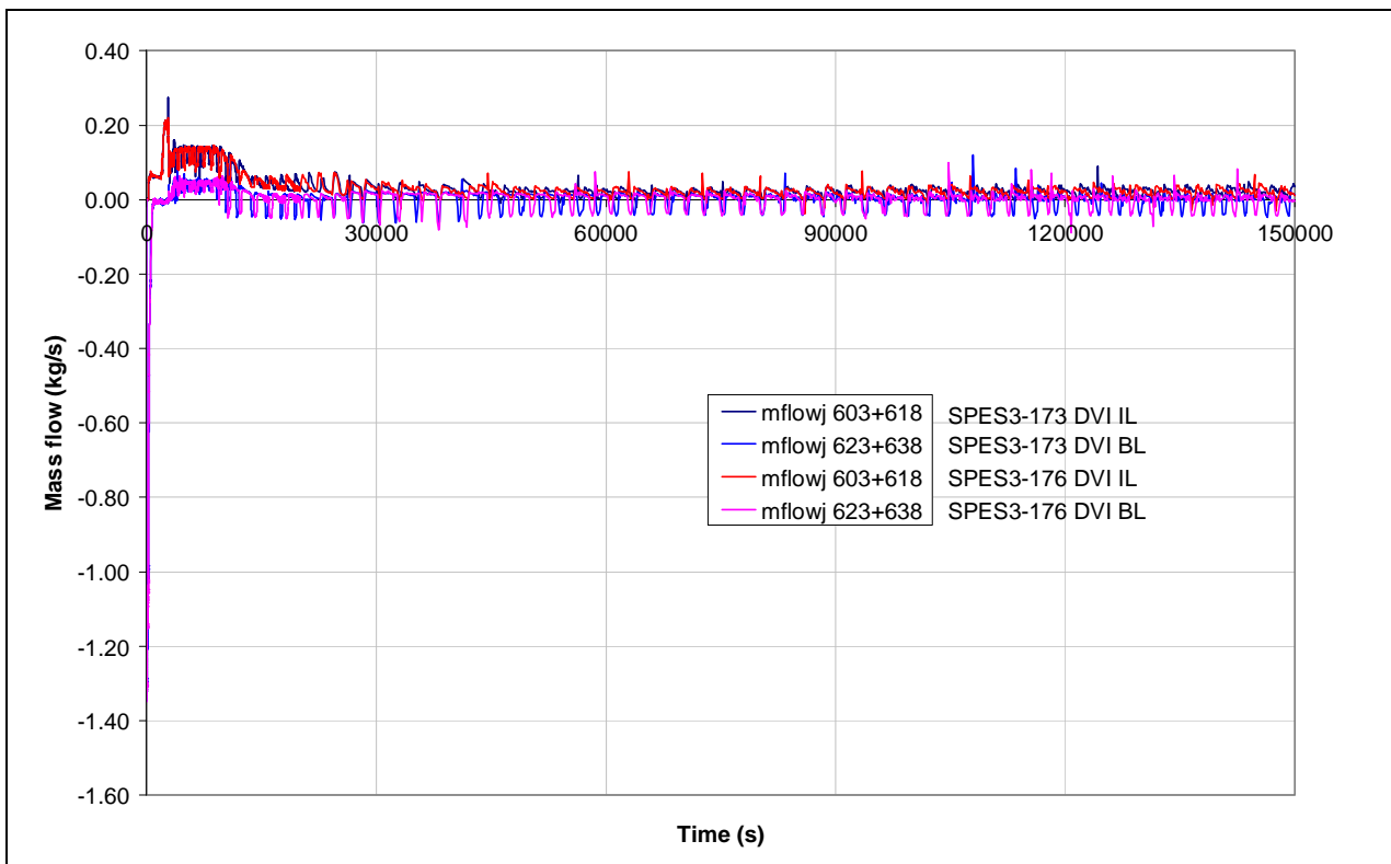
Fig.8. 68 – SPES3-173 and SPES3-176 DVI line mass flow
