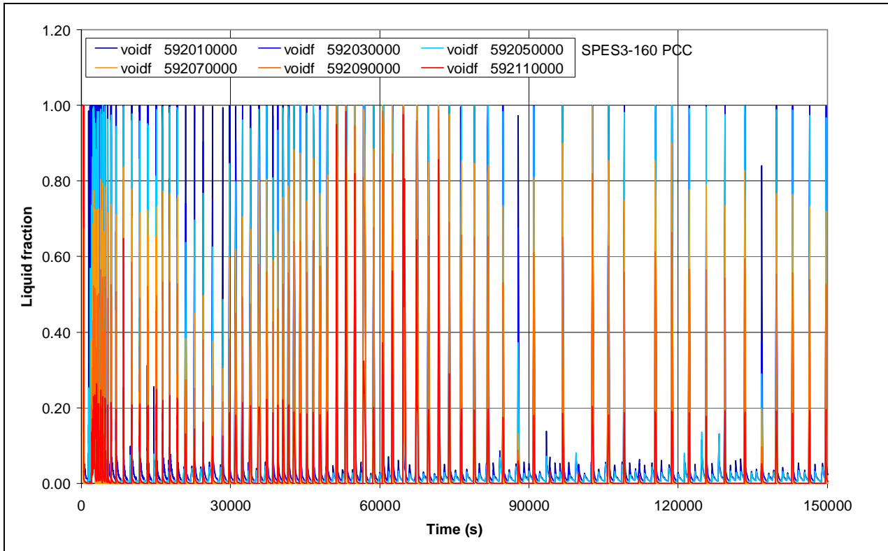
Fig.4.69 – SPES3-160 PCC liquid void fraction
