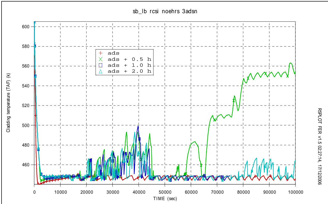
Fig.5. 31 – IRIS plant heater rod clad surface temperature (TAF)
