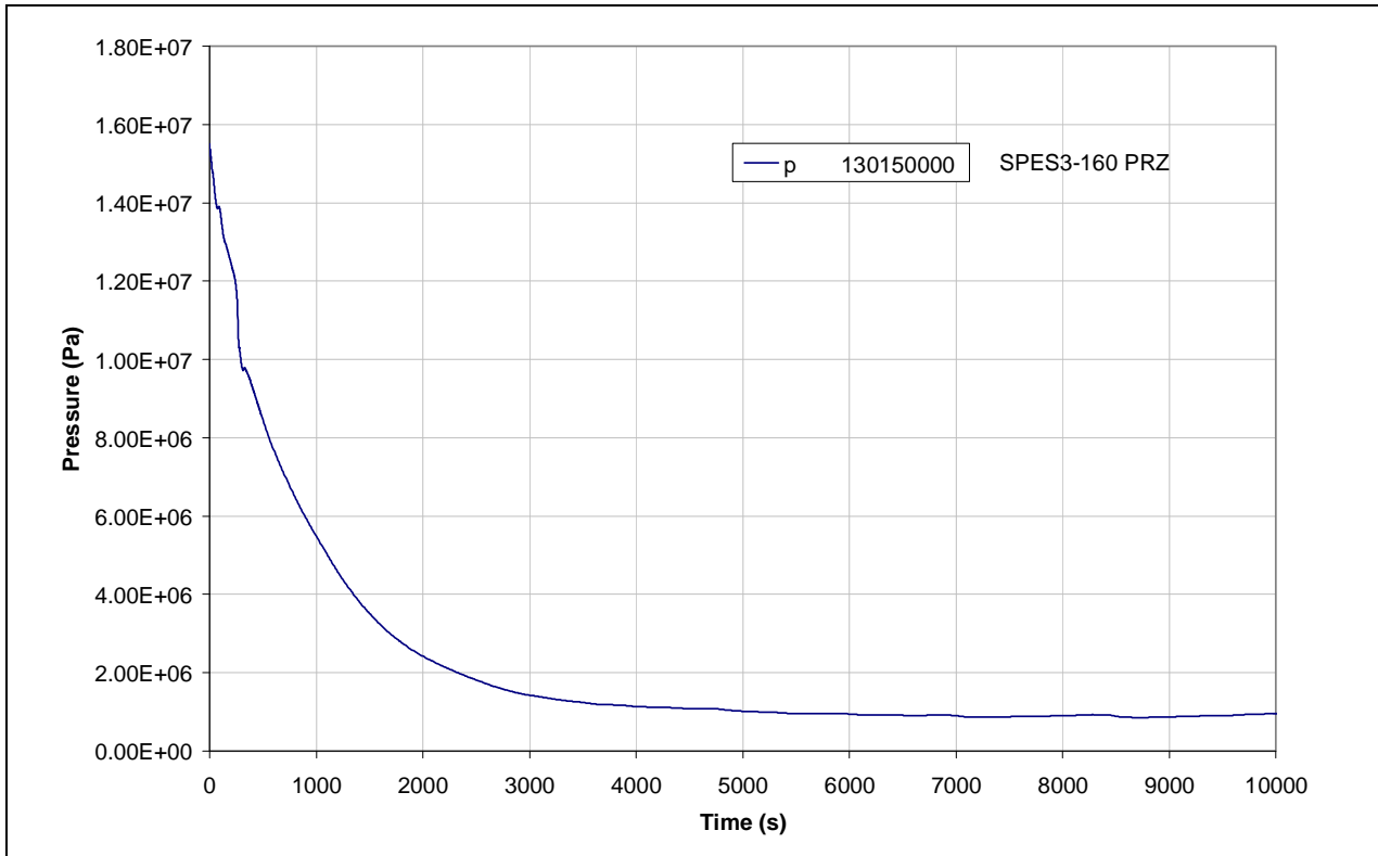
Fig.4.7 – SPES3-160 PRZ pressure (window)
