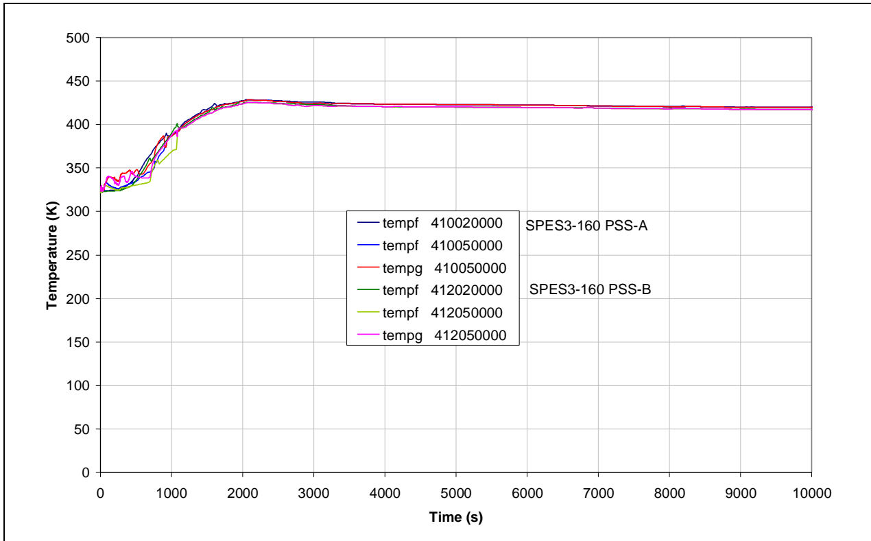
Fig.4.35 – SPES3-160 PSS temperature (window)
