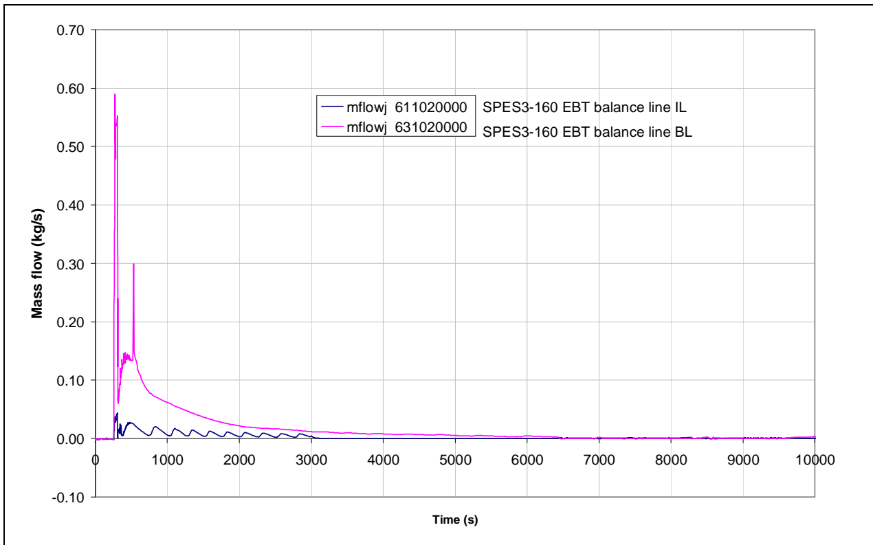
Fig.4.53 – SPES3-160 EBT balance line mass flow (mass flow)
