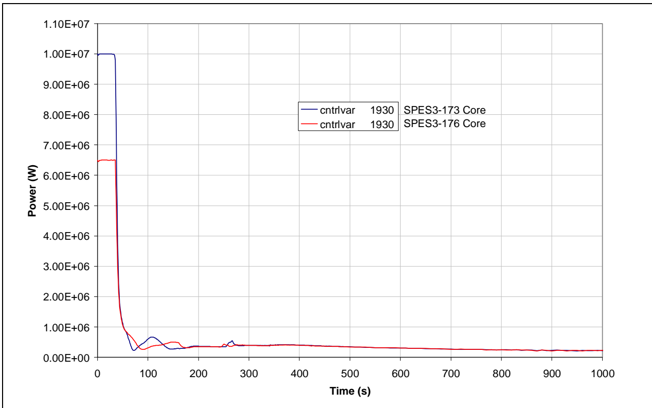
Fig.8. 43 – SPES3-173 and SPES3-176 core power (window)
