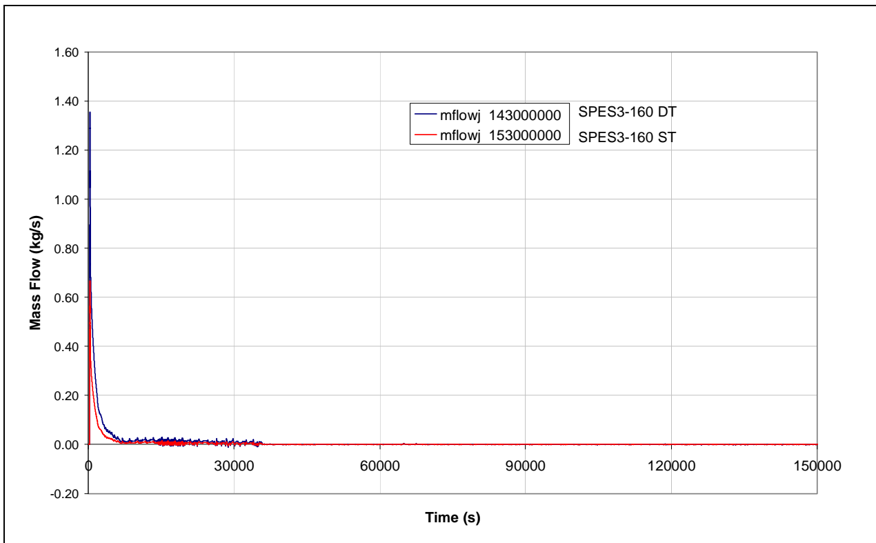
Fig.4.12 – SPES3-160 ADS Stage-I mass flow
