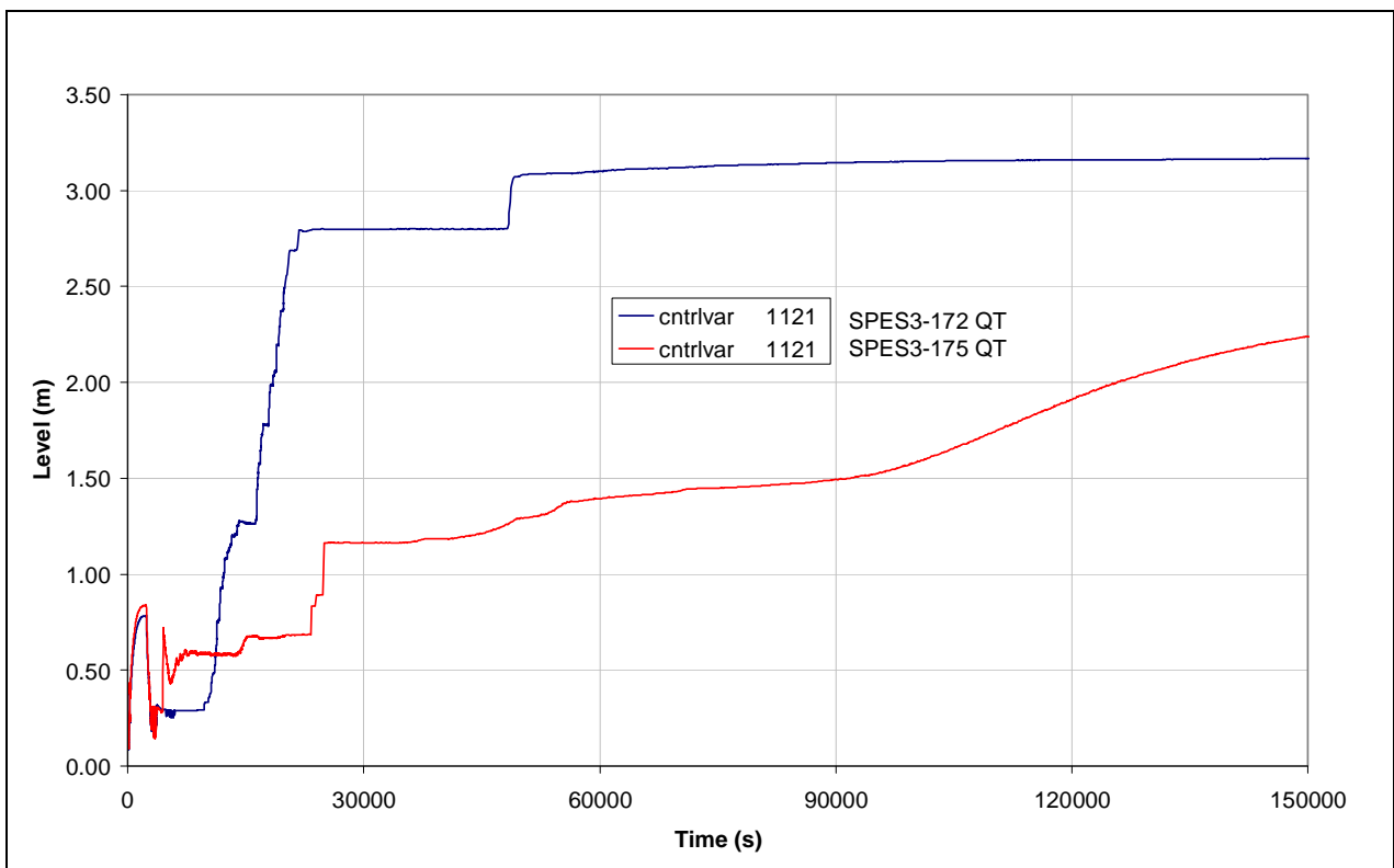
Fig.7. 70 - SPES3-172 and SPES3-175 QT level
