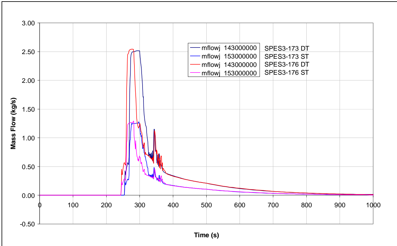
Fig.8. 7 – SPES3-173 and SPES3-176 ADS Stage-I mass flow (window)
