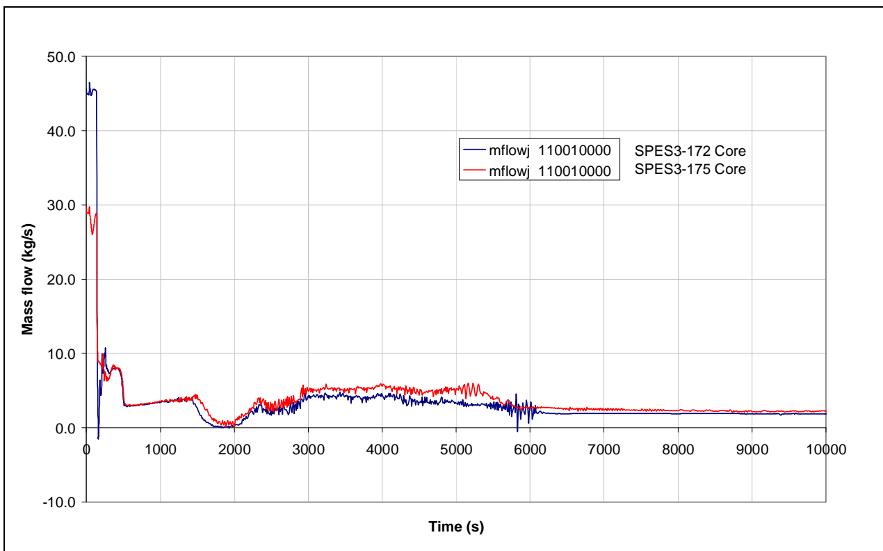
Fig.7. 48 - SPES3-172 and SPES3-175 Core inlet mass flow (window)
