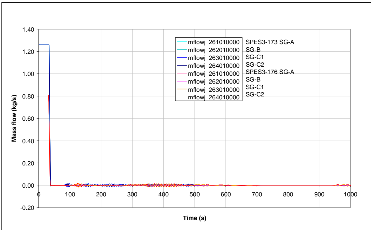
Fig.8. 48 – SPES3-173 and SPES3-176 SG ss mass flow (window)
