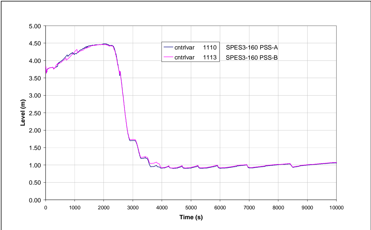
Fig.4.27 – SPES3-160 PSS level (window)
