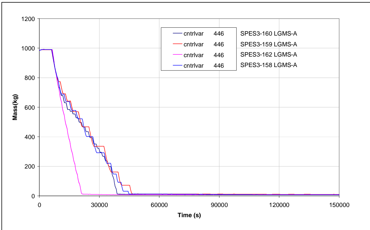
Fig.5. 8 – SPES3-159, 162, 158 and 160 LGMS-A mass (intact loop)
