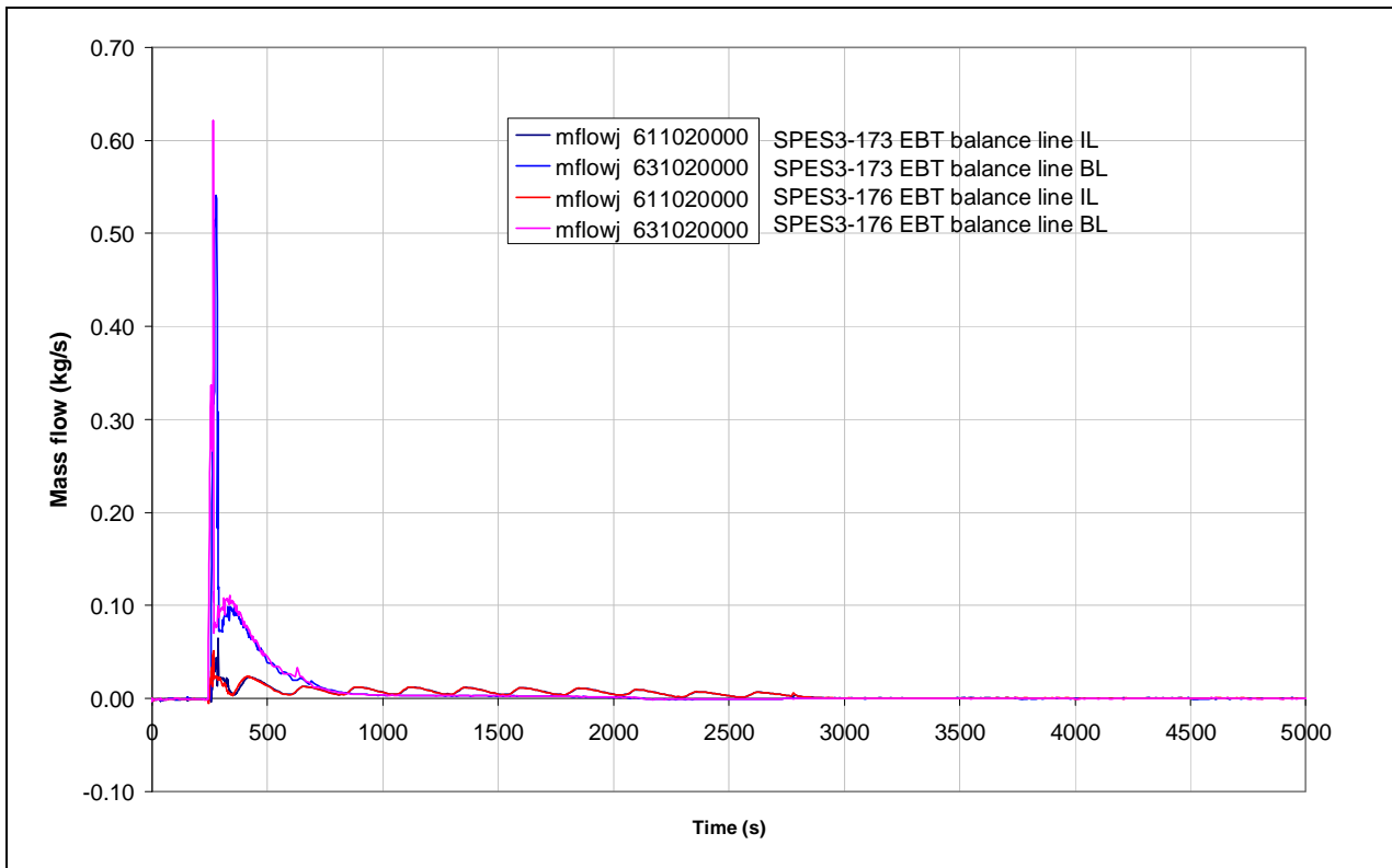
Fig.8. 63 – SPES3-173 and SPES3-176 EBT balance line mass flow (mass flow)
