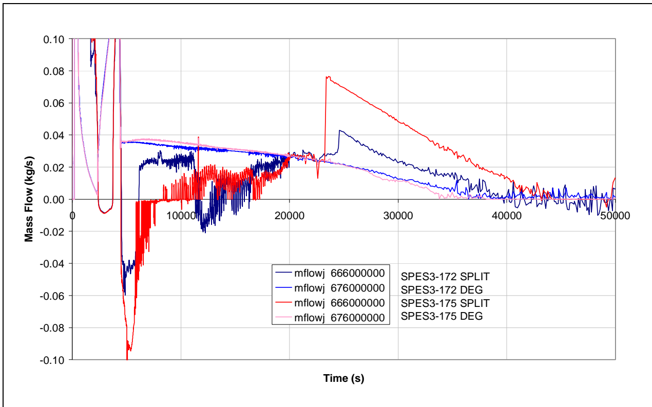
Fig.7. 3 - SPES3-172 and SPES3-175 DVI break mass flow (window)
