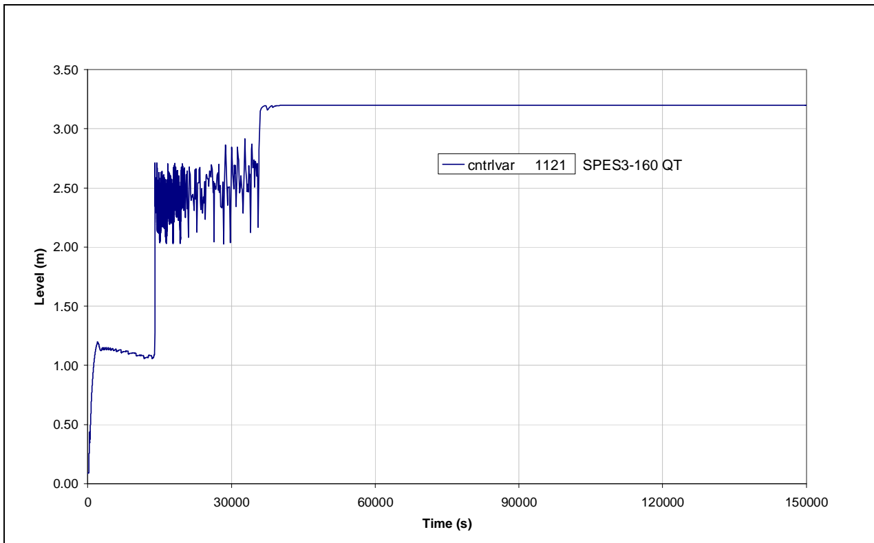
Fig.4.32 – SPES3-160 QT level
