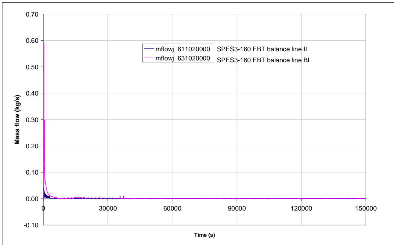
Fig.4.54 – SPES3-160 EBT balance line mass flow
