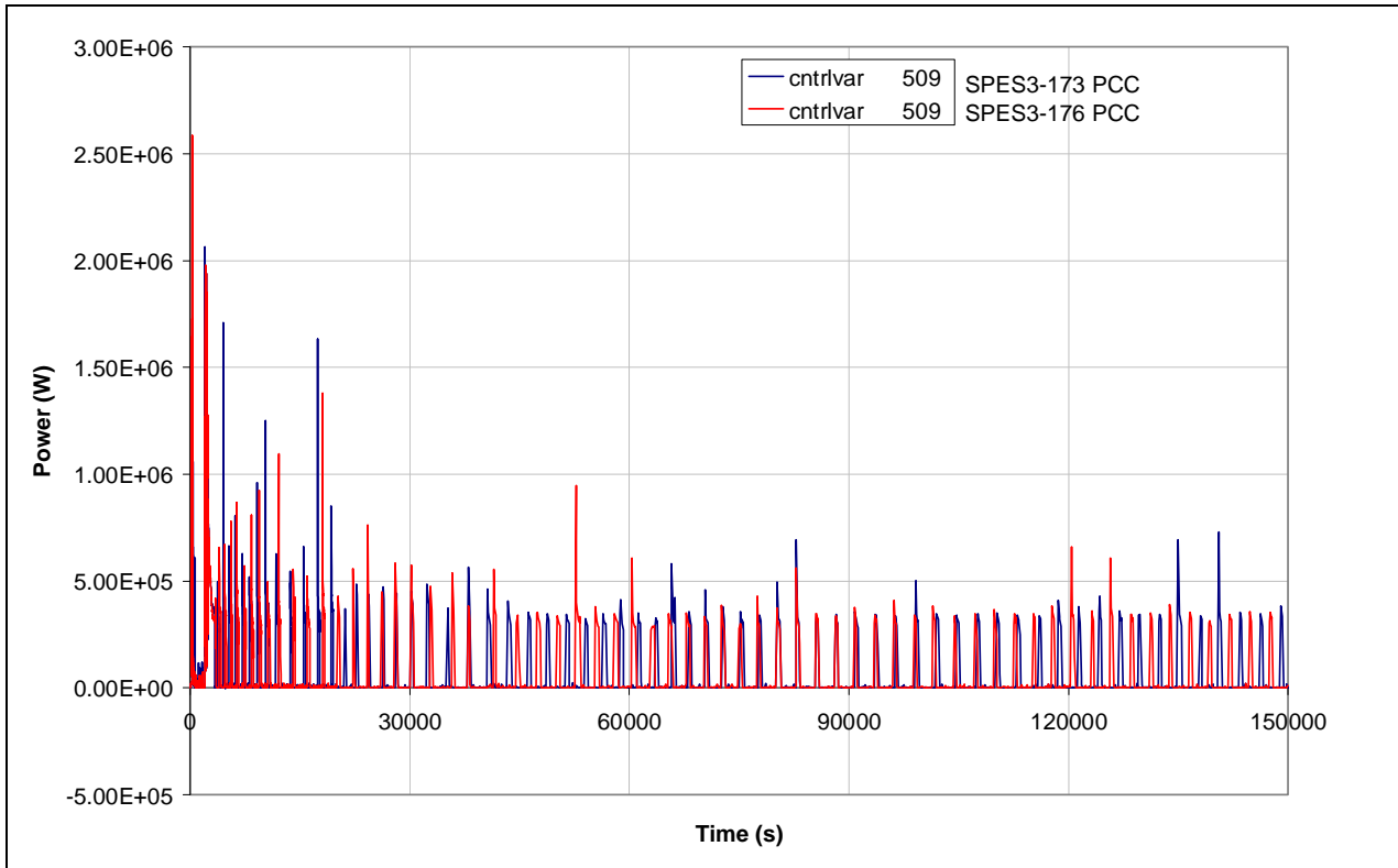
Fig.8. 21 – SPES3-173 and SPES3-176 PCC power
