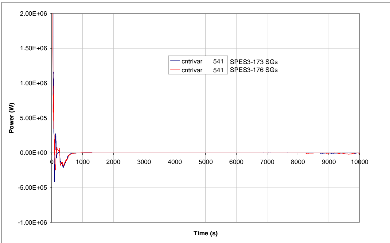
Fig.8. 47 – SPES3-173 and SPES3-176 SG power (window)
