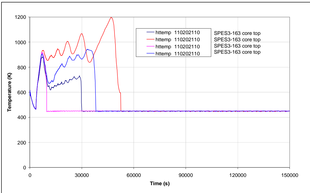
Fig.5. 28 – SPES3-163, 164, 165 and 166 Core heater rod clad surface temperature (hot rods)
