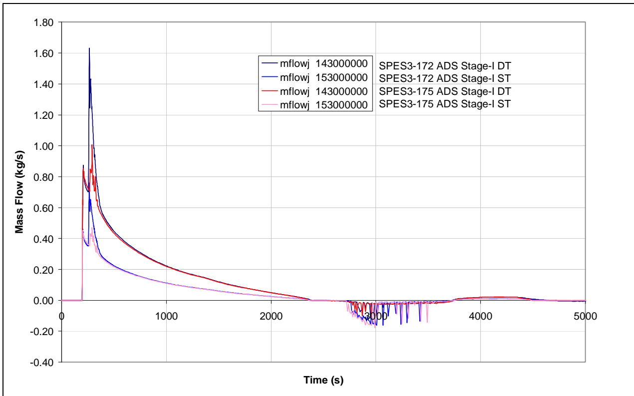
Fig.7. 13 - SPES3-172 and SPES3-175 ADS Stage-I mass flow (window)
