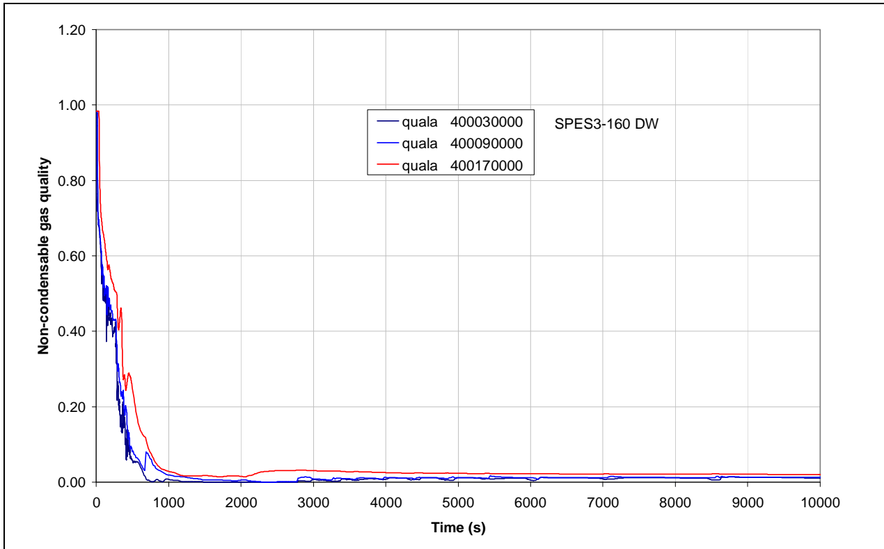
Fig.4.17 – SPES3-160 DW non-condensable gas quality (window)
