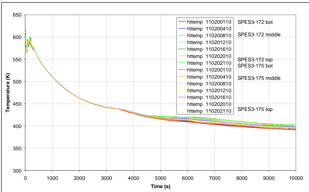
Fig.7. 64 - SPES3-172 and SPES3-175 Core heater rod surface temperature –hot rod (window)
