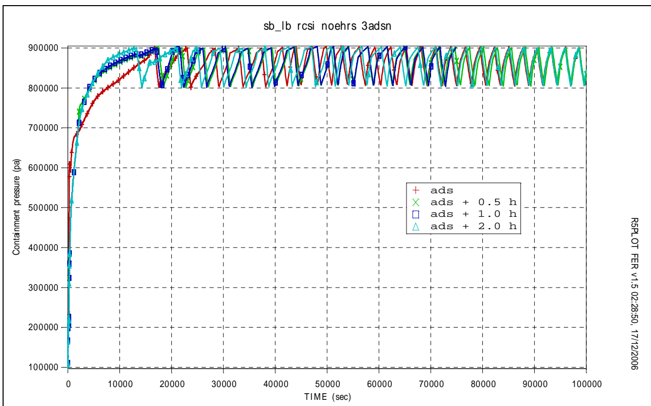
Fig.5. 32 – IRIS plant DW pressure
