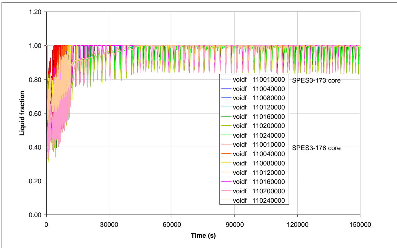
Fig.8. 65 – SPES3-173 and SPES3-176 Core liquid fraction
