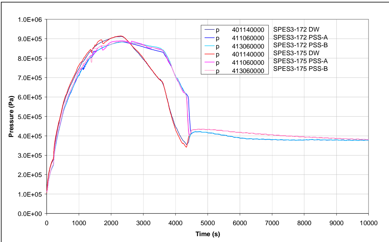
Fig.7. 26 - SPES3-172 and SPES3-175 DW and PSS pressure (window)
