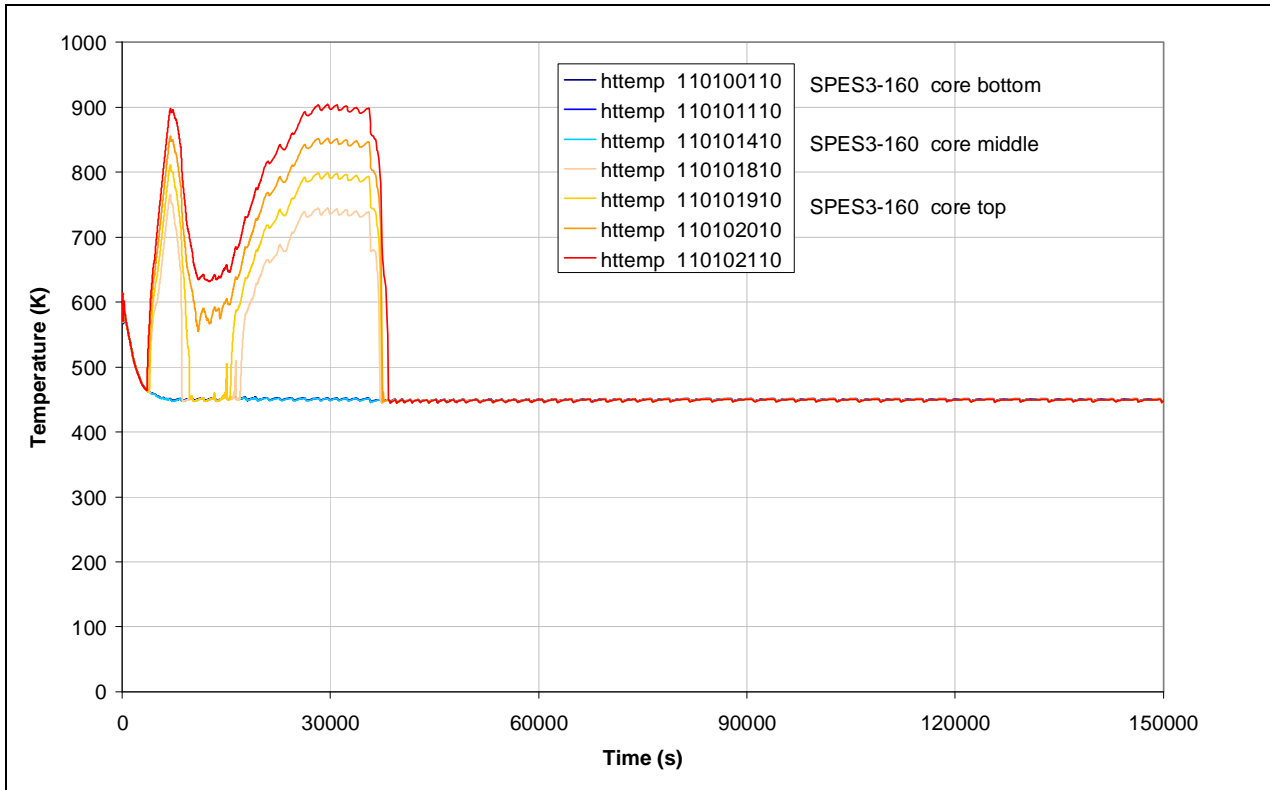
Fig.4.59 – SPES3-160 Core heater rod clad surface temperatures (normal rods)
