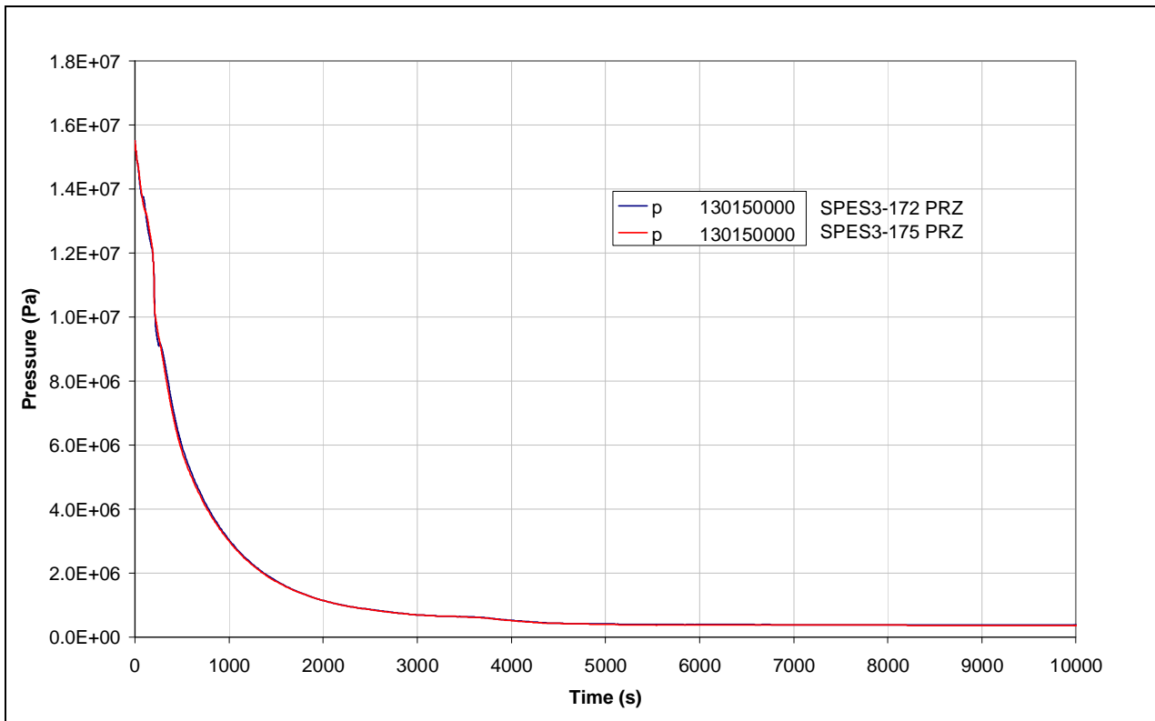
Fig.7. 9 - SPES3-172 and SPES3-175 PRZ pressure (window)
