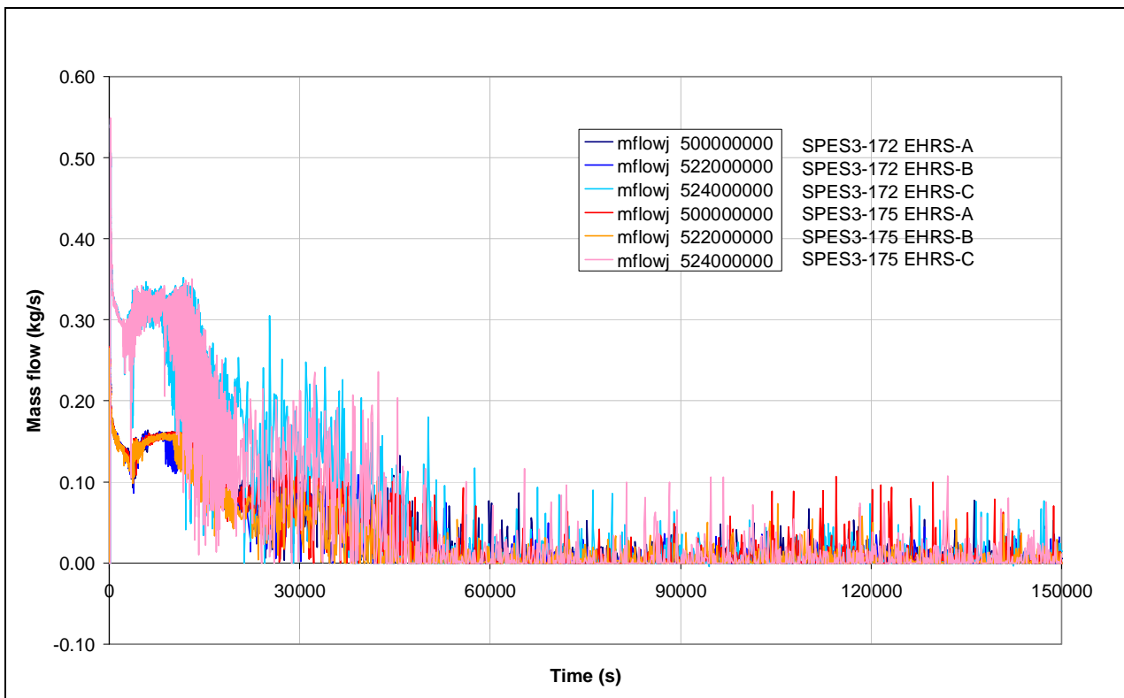
Fig.7. 38 - SPES3-172 and SPES3-175 EHRs cold leg mass flow
