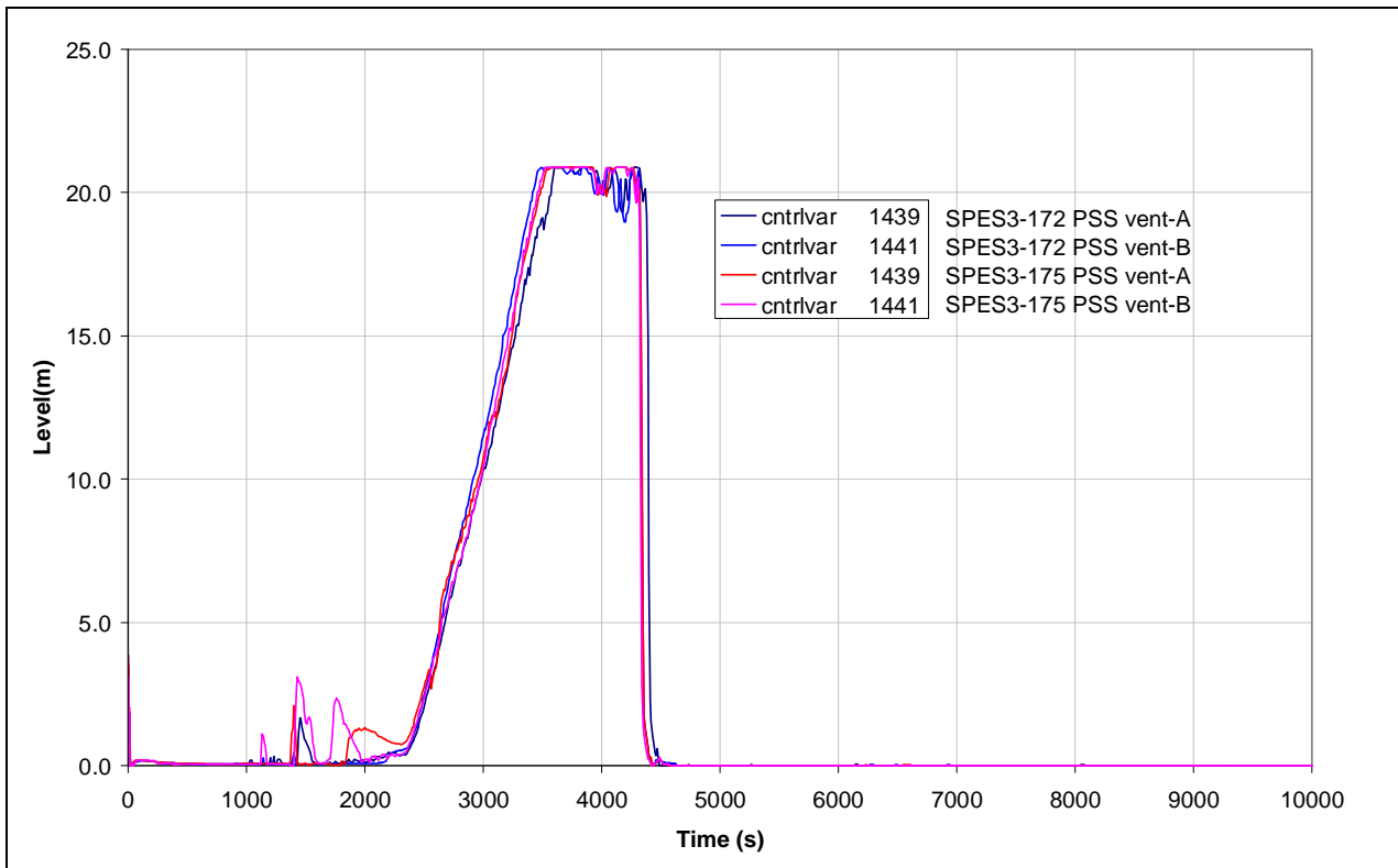
Fig.7. 28 - SPES3-172 and SPES3-175 PSS vent pipe level (window)
