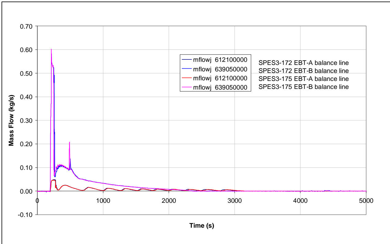
Fig.7. 59 - SPES3-172 and SPES3-175 EBT to RPV balance line mass flow (window)
