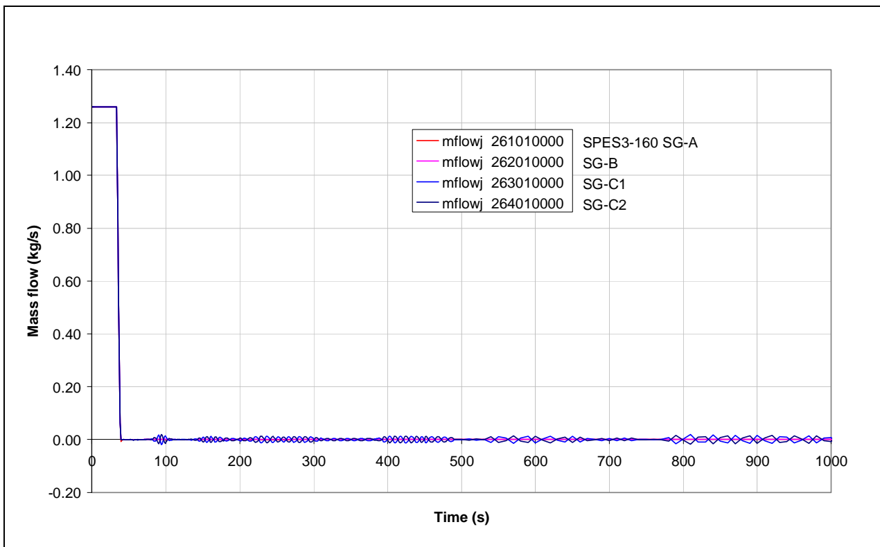
Fig.4.40 – SPES3-160 SG ss mass flow (window)
