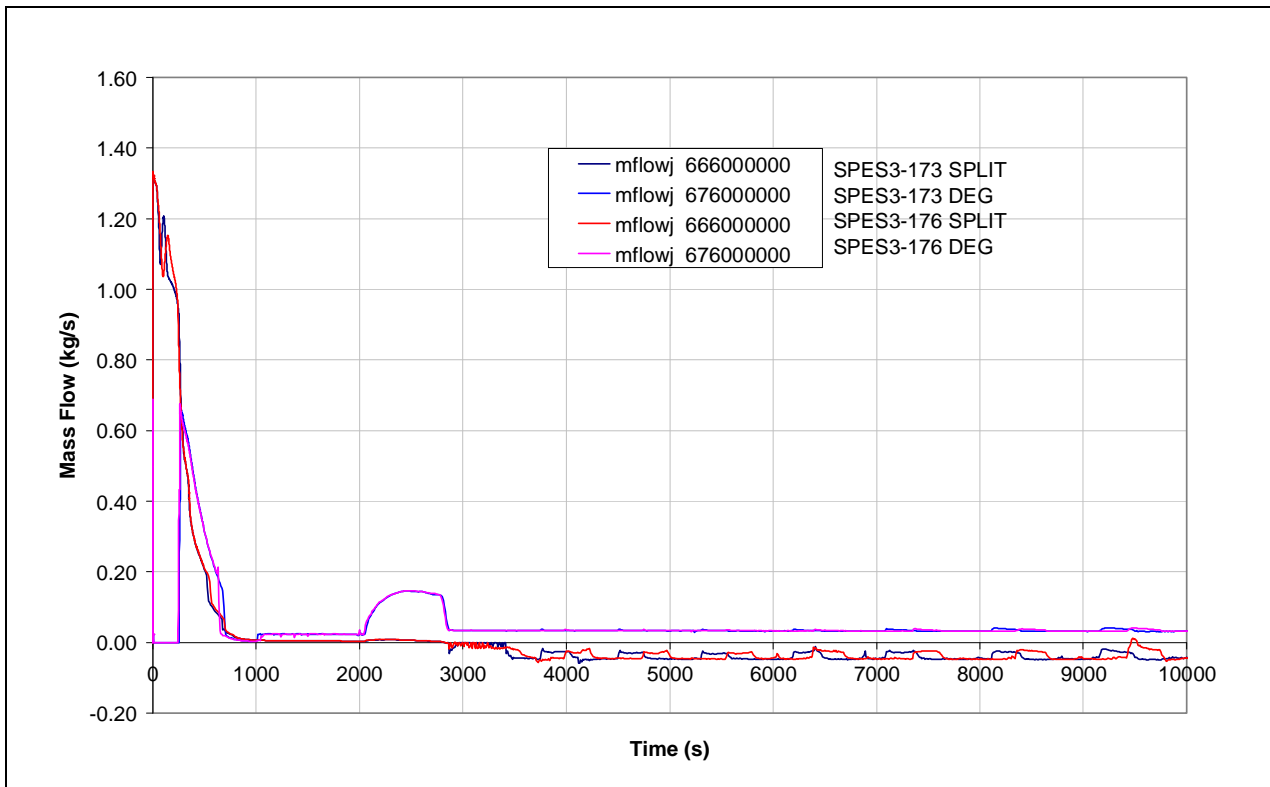
Fig.8. 2 – SPES3-173 and SPES3-176 DVI line break flow (window)
