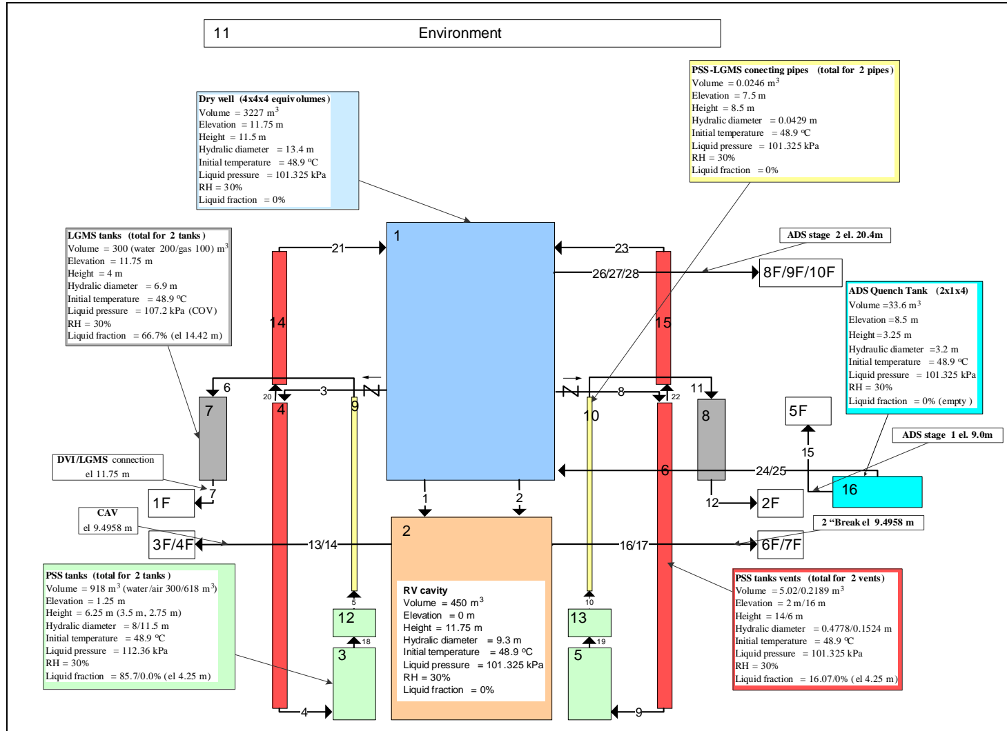
Fig.3. 11 – IRIS Containment system GOTHIC
