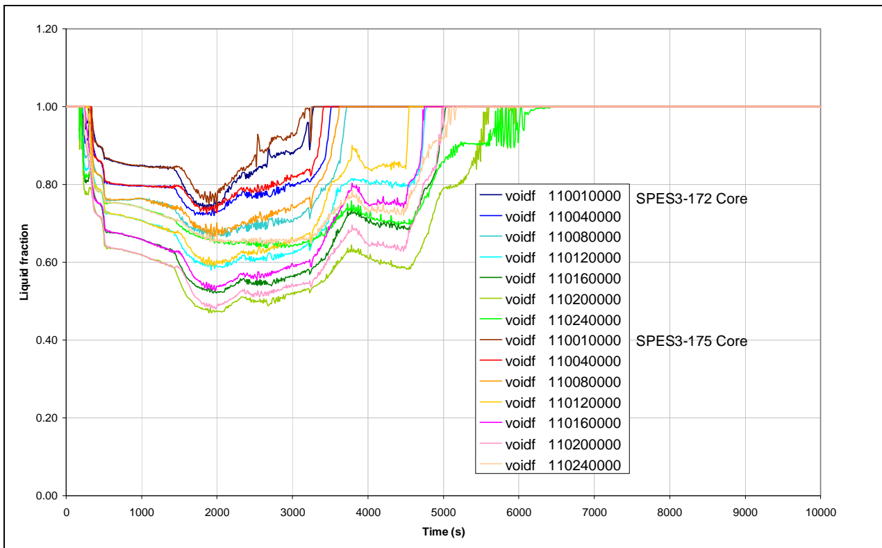
Fig.7. 54 - SPES3-172 and SPES3-175 Core liquid fraction (window)
