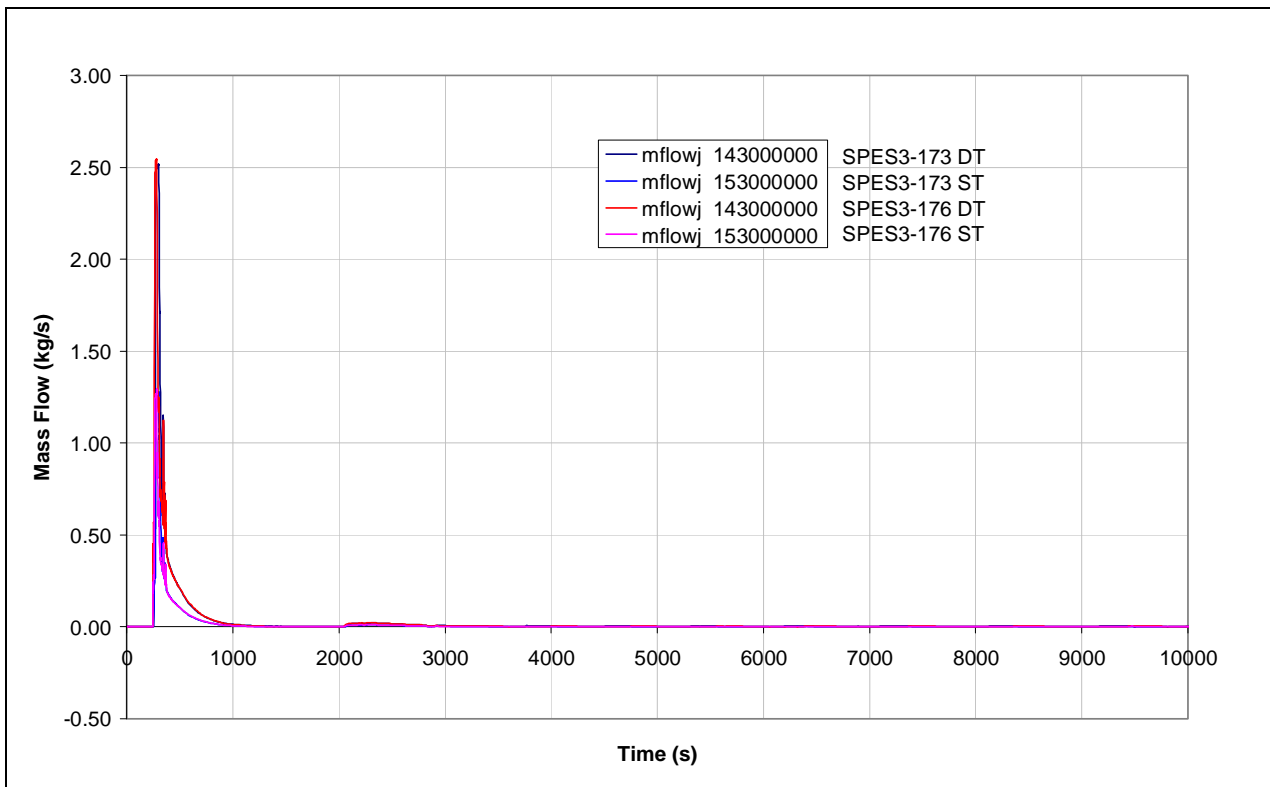
Fig.8. 8 – SPES3-173 and SPES3-176 ADS Stage-I mass flow (window)
