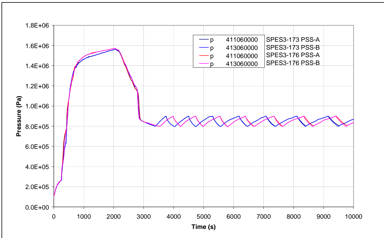
Fig.8. 26 – SPES3-173 and SPES3-176 PSS pressure (window)
