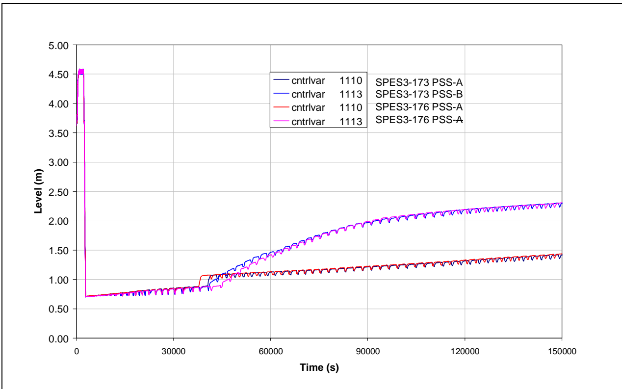
Fig.8. 35 – SPES3-173 and SPES3-176 PSS level
