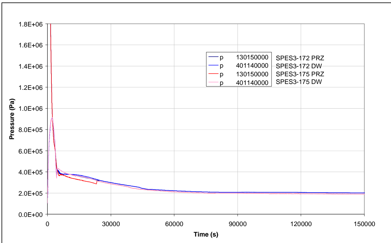
Fig.7. 16 - SPES3-172 and SPES3-175 PRZ and DW pressures
