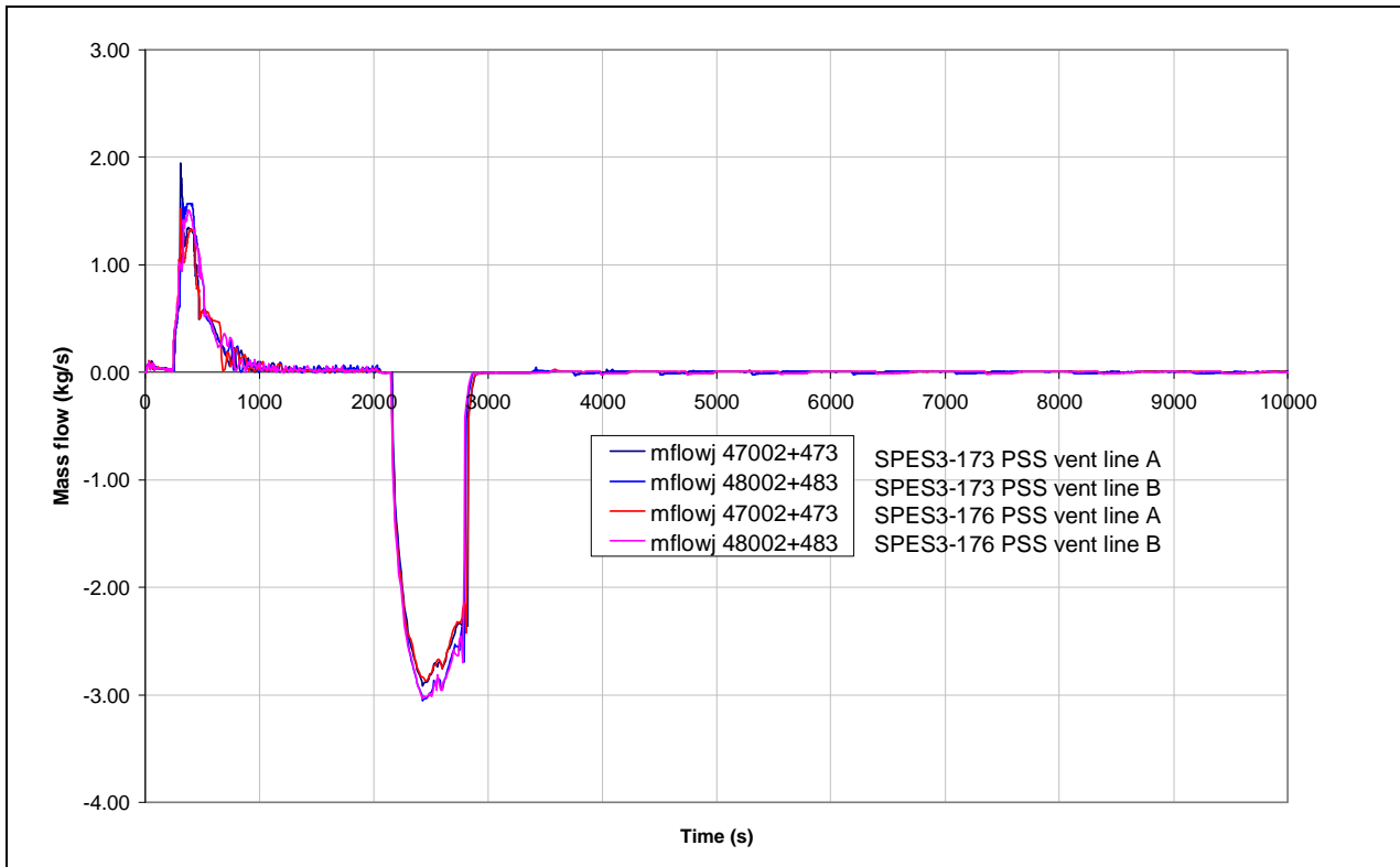
Fig.8. 22 – SPES3-173 and SPES3-176 PSS to DW mass flow (window)
