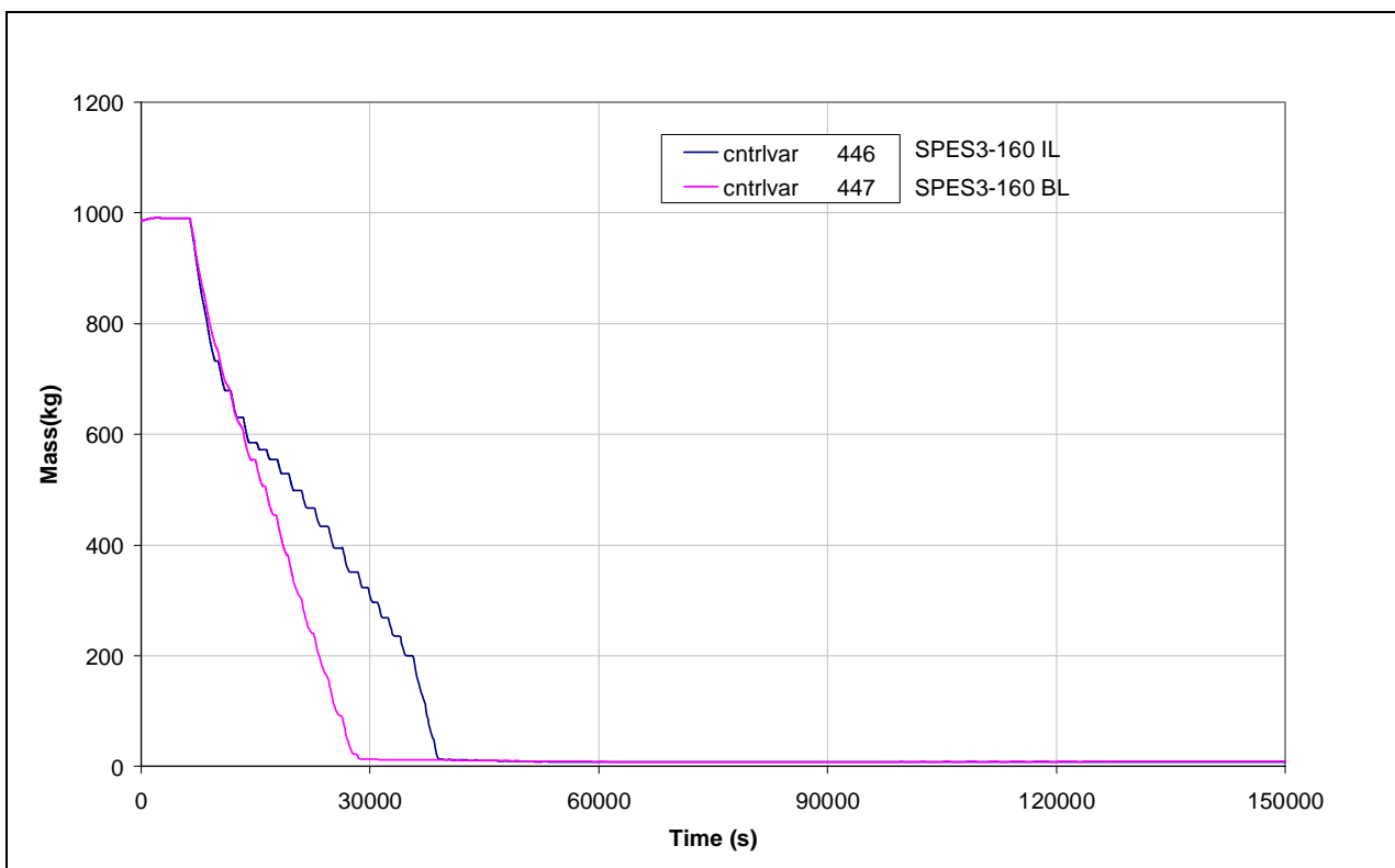
Fig.4.70 – SPES3-160 LGMS mass
