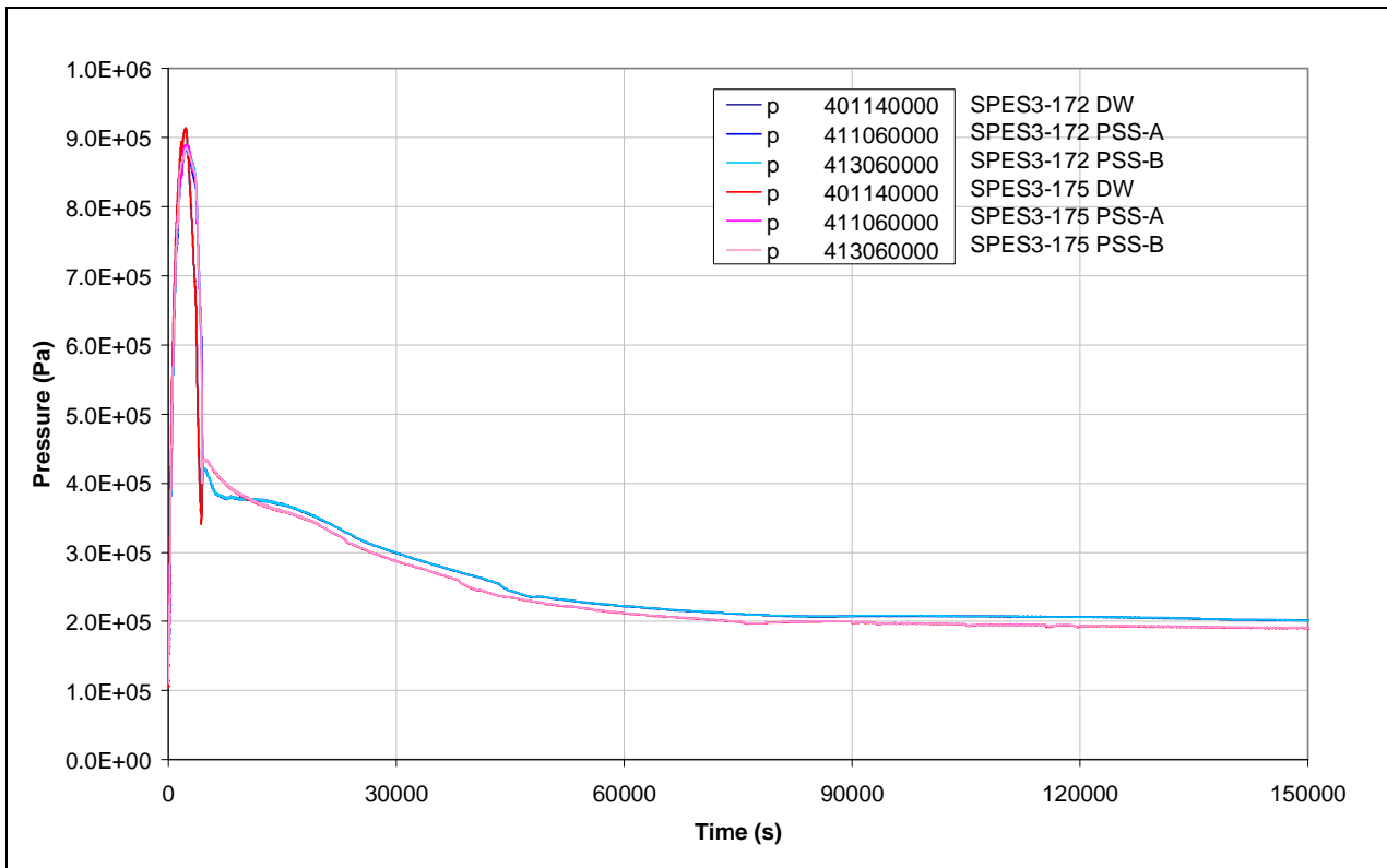
Fig.7. 27 - SPES3-172 and SPES3-175 DW and PSS pressure
