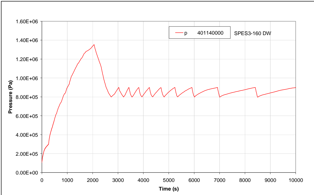
Fig.4.9 – SPES3-160 DW pressure (window)
