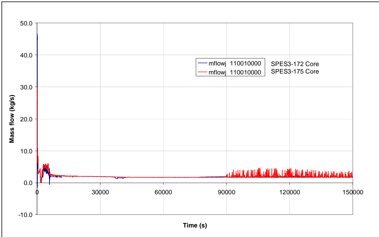
Fig.7. 49 - SPES3-172 and SPES3-175 Core inlet mass flow
