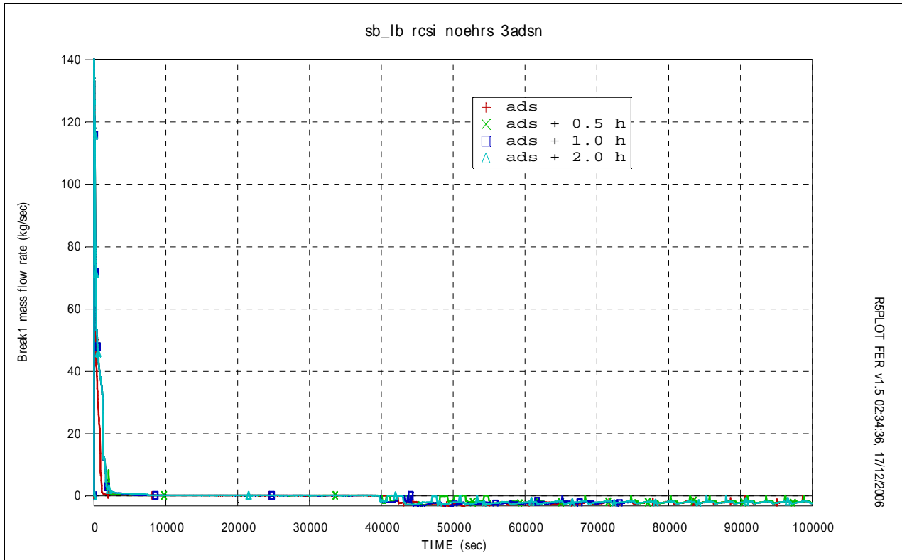
Fig.5. 35 – IRIS plant break mass flow (RPV side)
