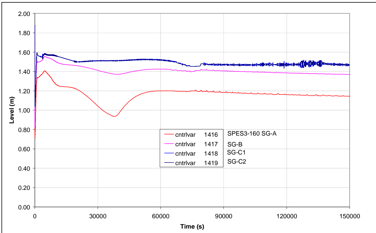
Fig.4.44 – SPES3-160 SG-A ss level
