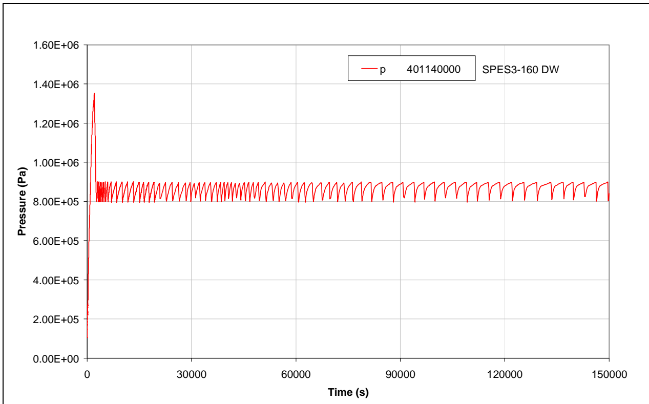
Fig.4.10 – SPES3-160 DW pressure
