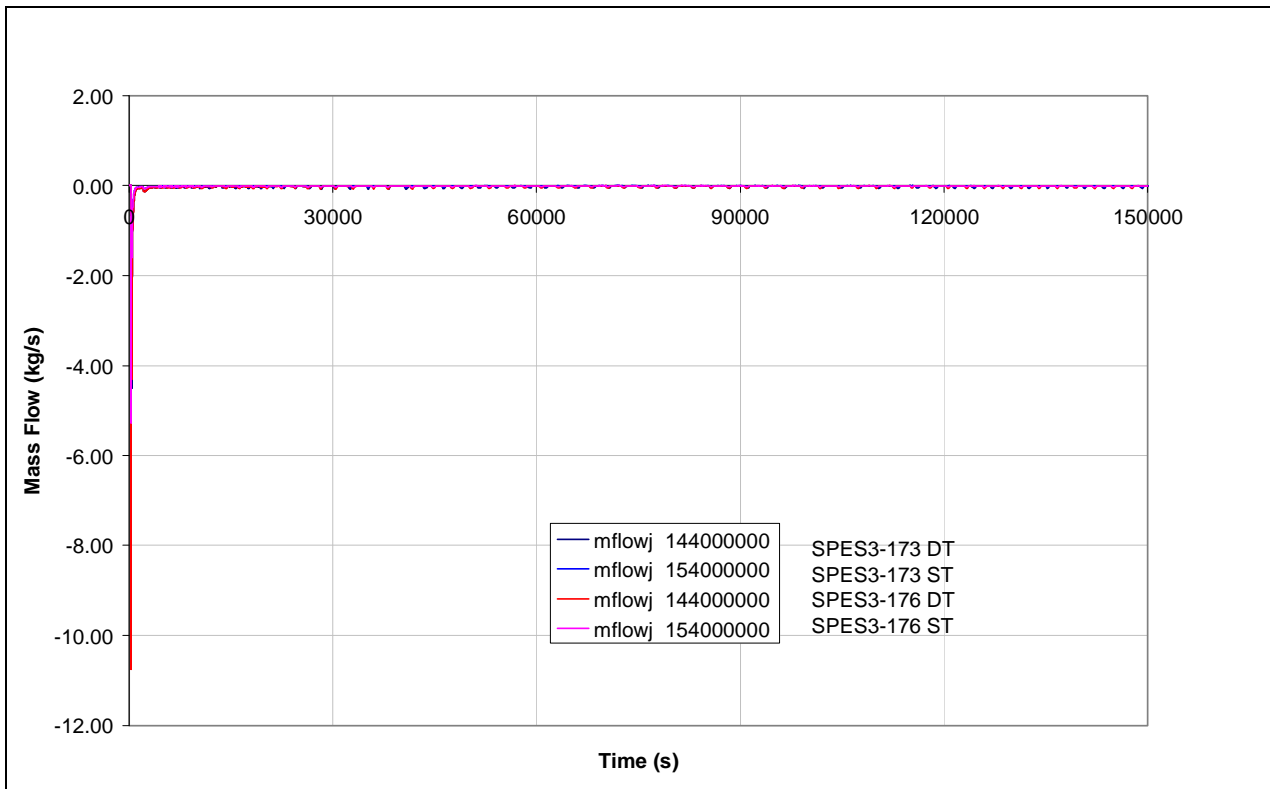
Fig.8. 11 – SPES3-173 and SPES3-176 ADS Stage-II mass flow
