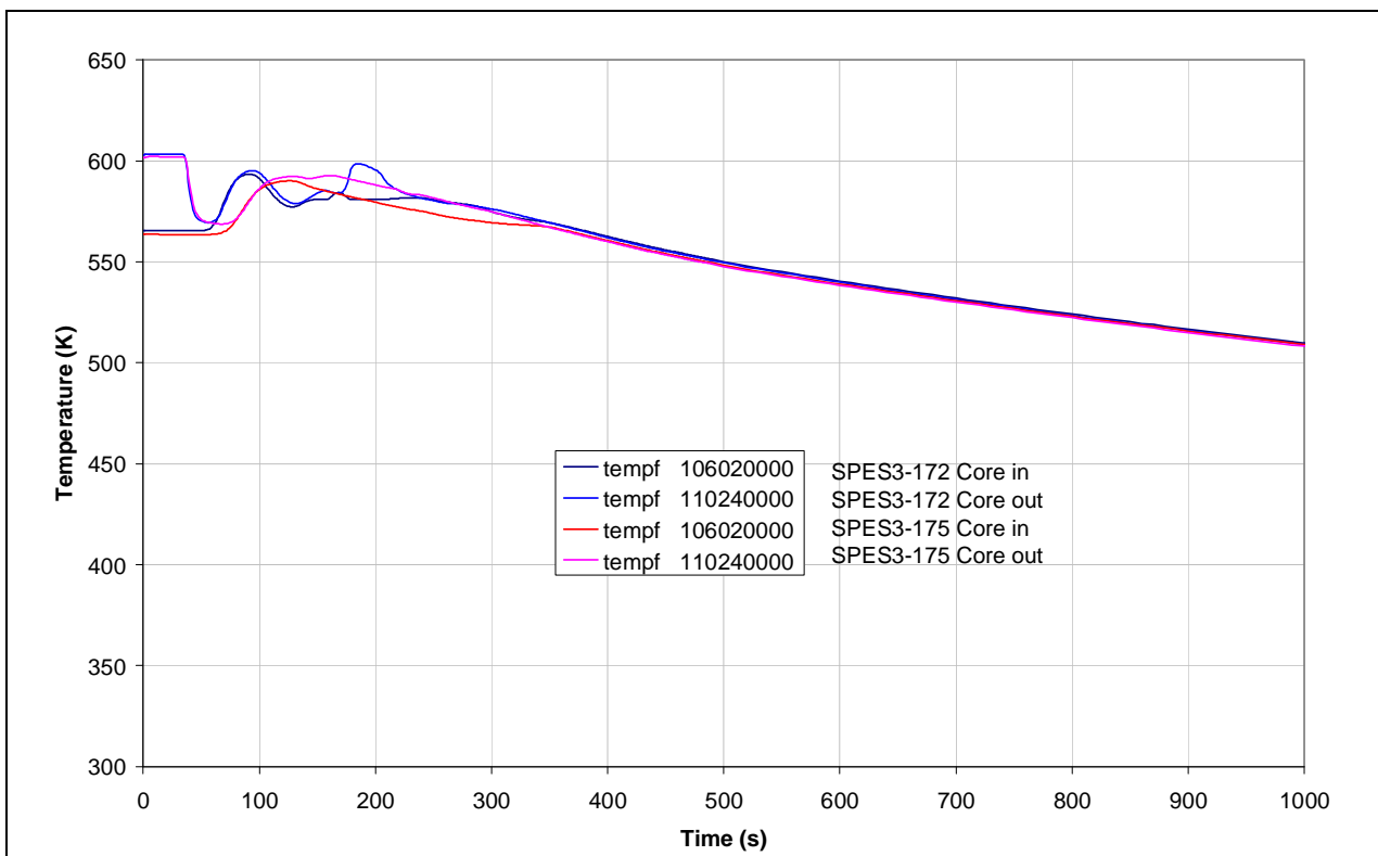
Fig.7. 60 - SPES3-172 and SPES3-175 Core inlet and outlet fluid temperature (window)
