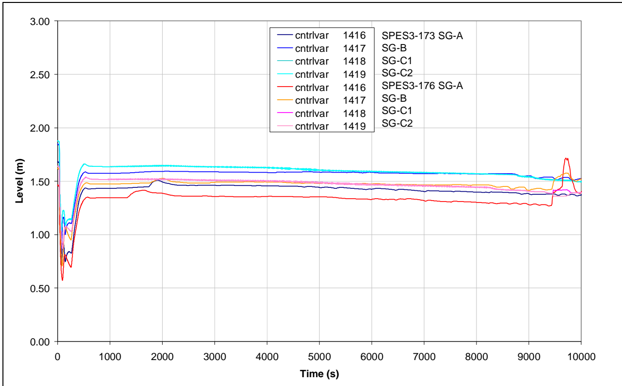
Fig.8. 51 – SPES3-173 and SPES3-176 SGs level (window)
