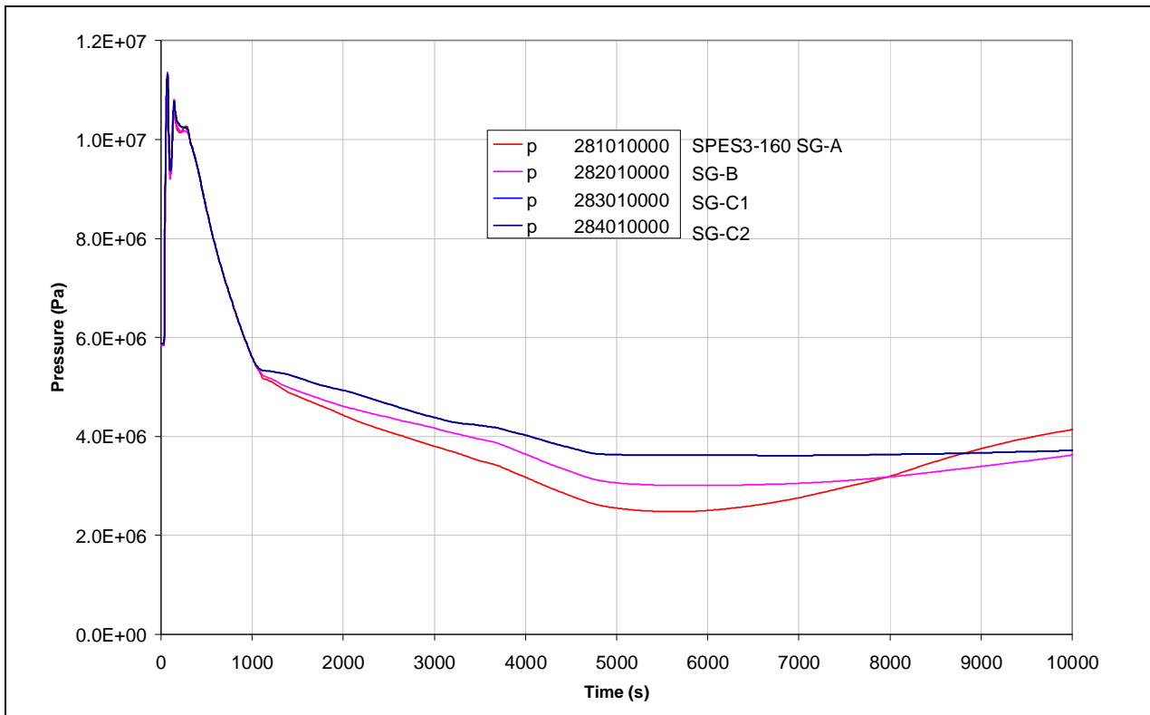
Fig.4.41 – SPES3-160 SG ss outlet pressure (window)
