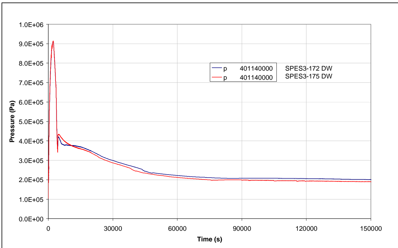
Fig.7. 12 - SPES3-172 and SPES3-175 DW pressure
