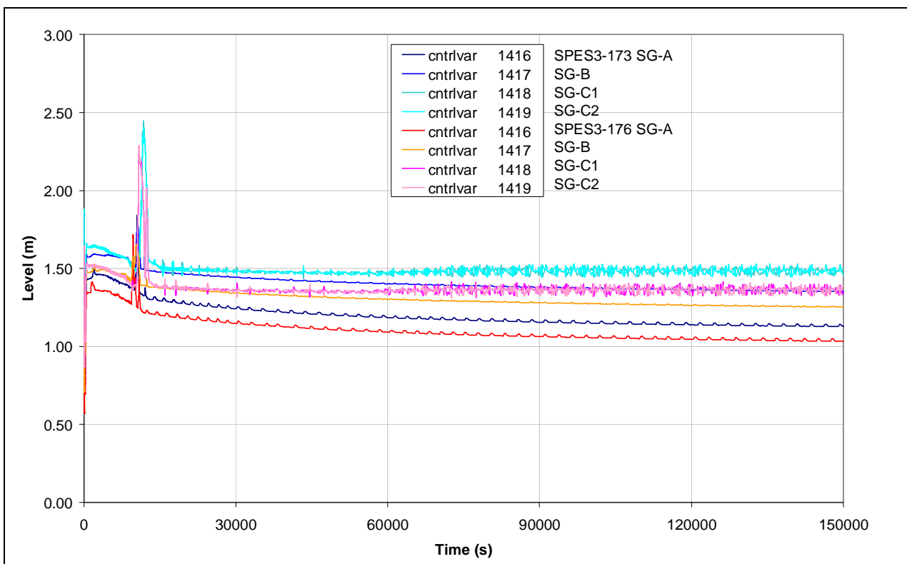
Fig.8. 52 – SPES3-173 and SPES3-176 SGs level
