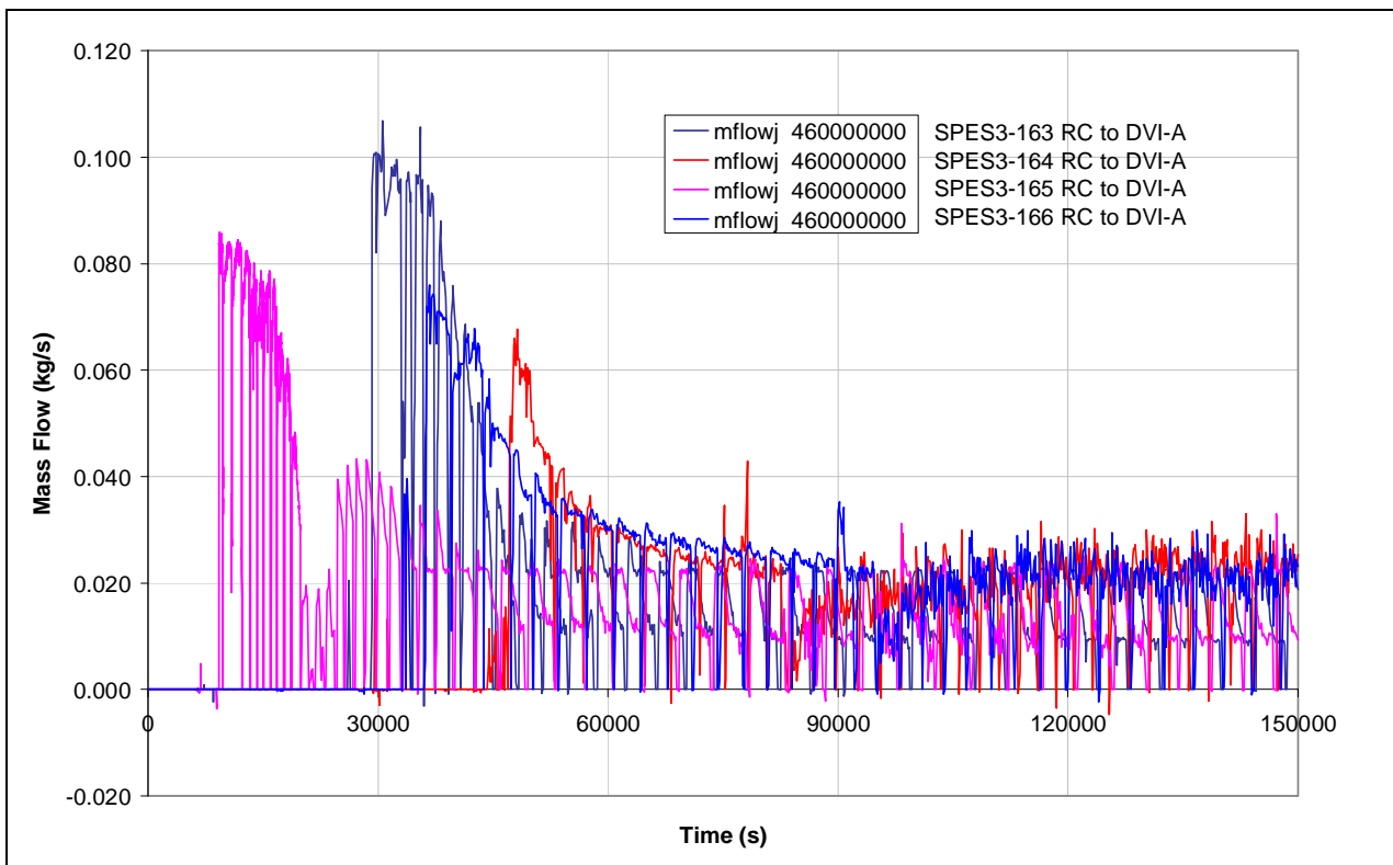
Fig.5. 24 – SPES3-163, 164, 165 and 166 RC to DVI line mass flow (intact loop)
