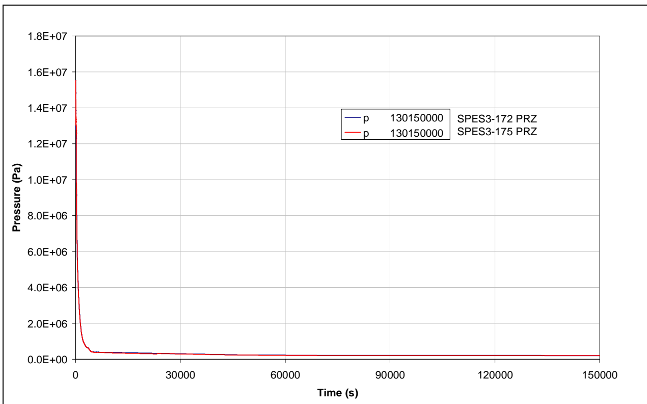
Fig.7. 10 - SPES3-172 and SPES3-175 PRZ pressure
