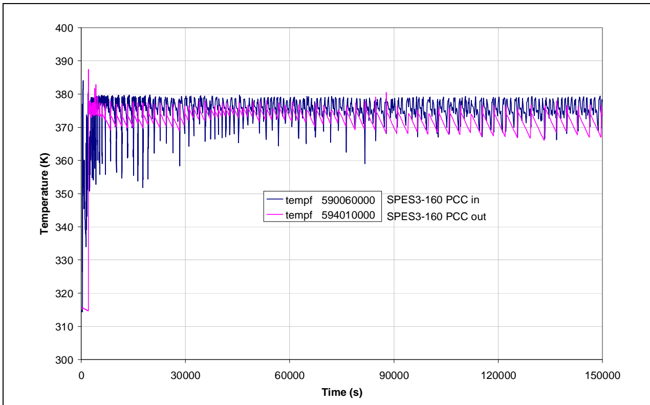
Fig.4.67 – SPES3-160 PCC inlet and outlet temperature
