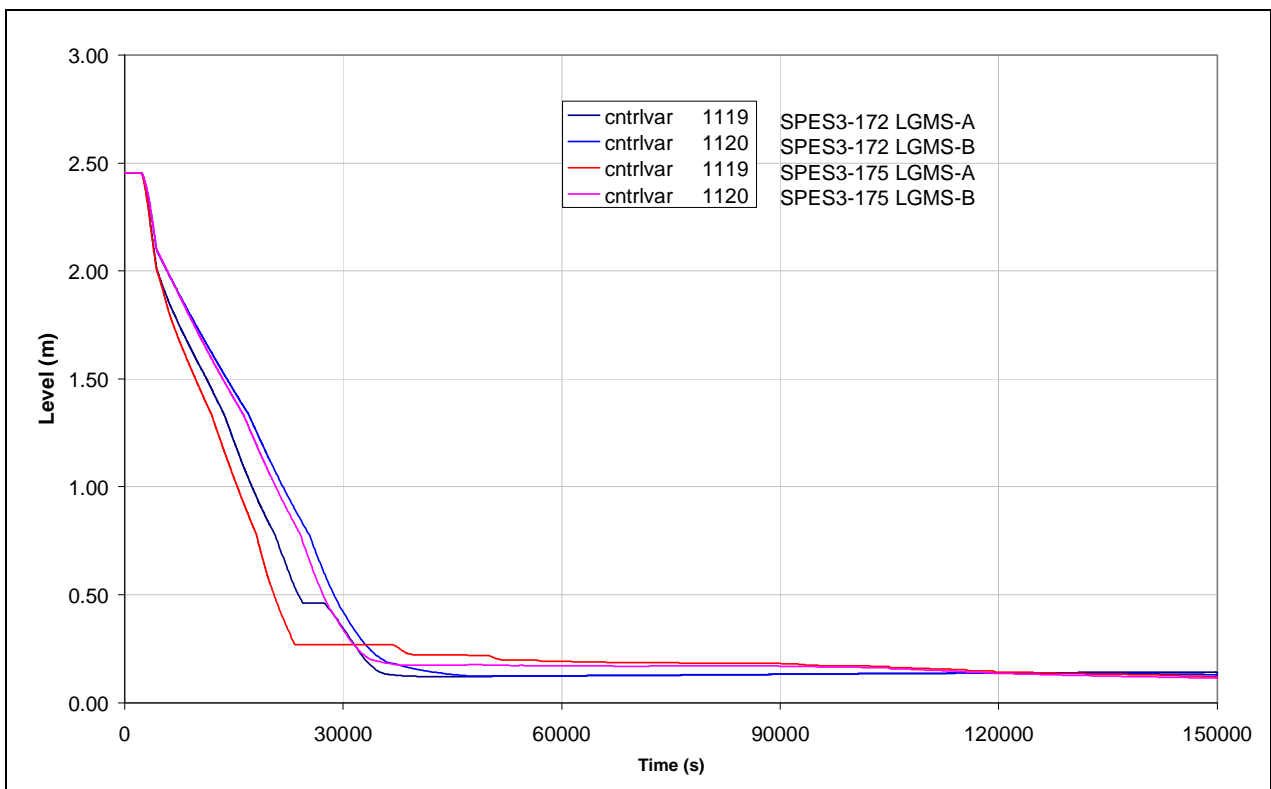
Fig.7. 66 - SPES3-172 and SPES3-175 LGMS level
