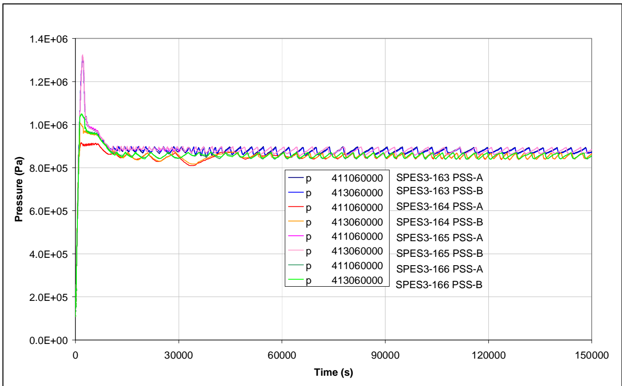
Fig.5. 18 – SPES3-163, 164, 165 and 166 PSS pressure
