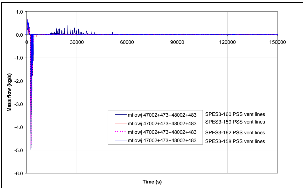
Fig.5. 6 – SPES3-159, 162, 158 and 160 PSS to DW mass flow
