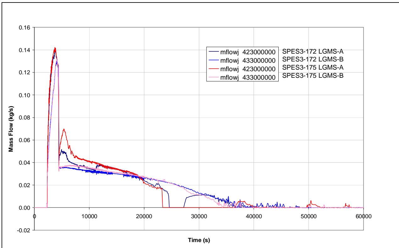
Fig.7. 6 - SPES3-172 and SPES3-175 LGMS mass flow (window)
