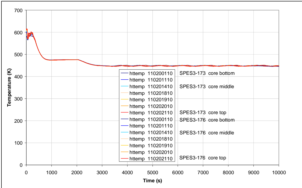
Fig.8. 73 – SPES3-173 and SPES3-176 Core heater rod clad surface temperatures (hot rods) (window)
