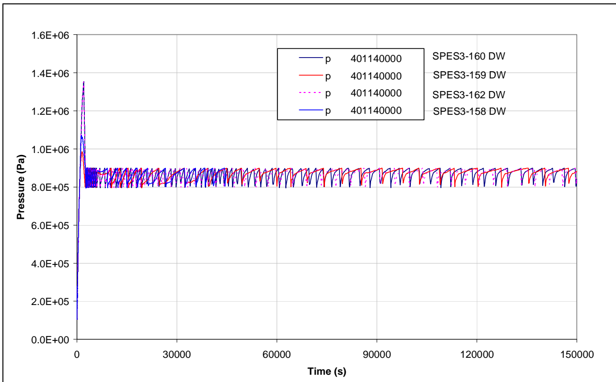
Fig.5. 2 – SPES3-159, 162, 158 and 160 DW pressure
