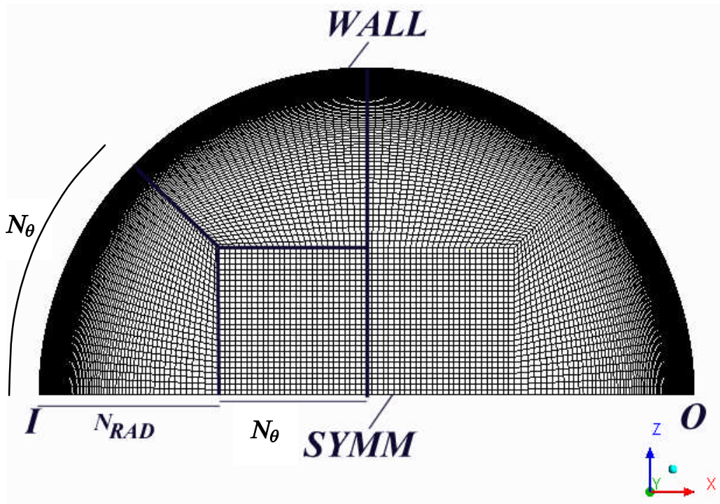
Fig. 2 Mesh (number 4) used to perform the computations. The grid is of the multi-block structured type. The total number of cells in the whole cross section would be N_{SEC}=4 \cdot N_\theta (N_\theta+2 N_{RAD}) , but only one half of the section is simulated.
