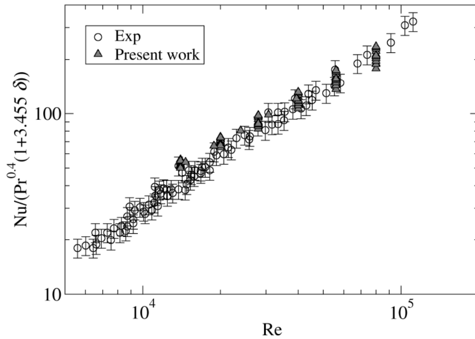
Fig. 10 Comparison of the reduced average Nusselt number Nu Pr^{-0.4} (1+3.455\delta)^{-1} obtained by numerical simulations using the RSM model with experimental data by Xin and Ebadian for two values of the curvature ( \delta=0.027, 0.08 ) and 0.7 \leq Pr \leq 5 .
