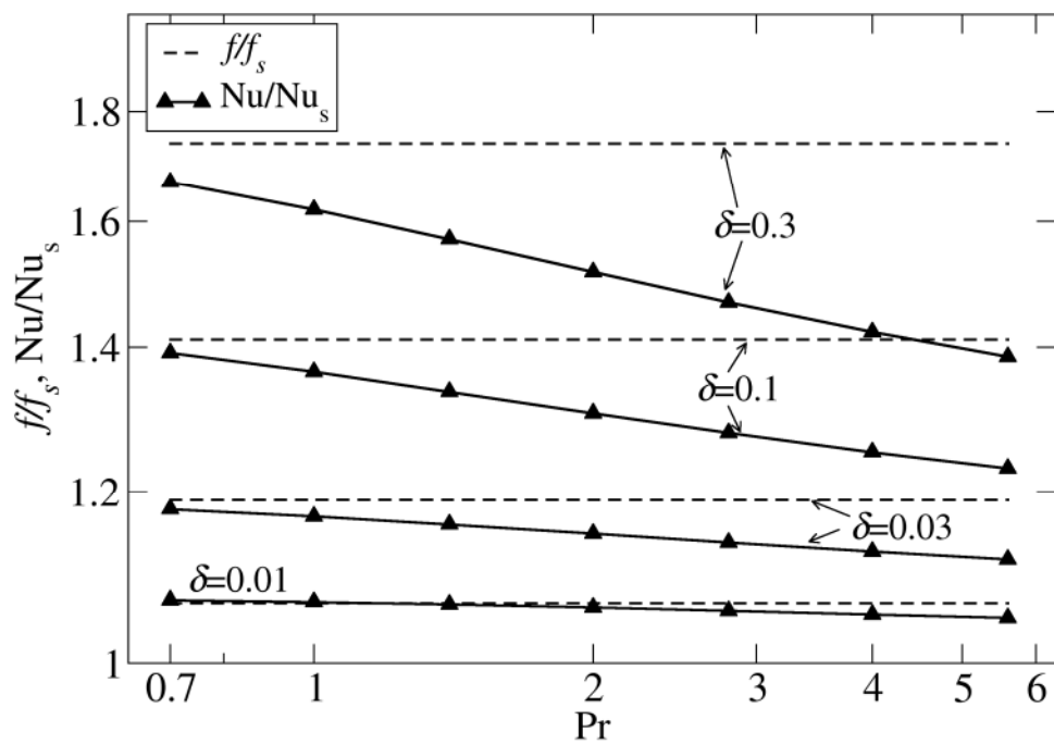
Fig. 16 Doubly logarithmic plot of the RSM-computed relative friction coefficient ff_s and Nusselt number Nu/Nu_s as functions of Pr for Re=2 \cdot 10^4 and different values of \delta .
