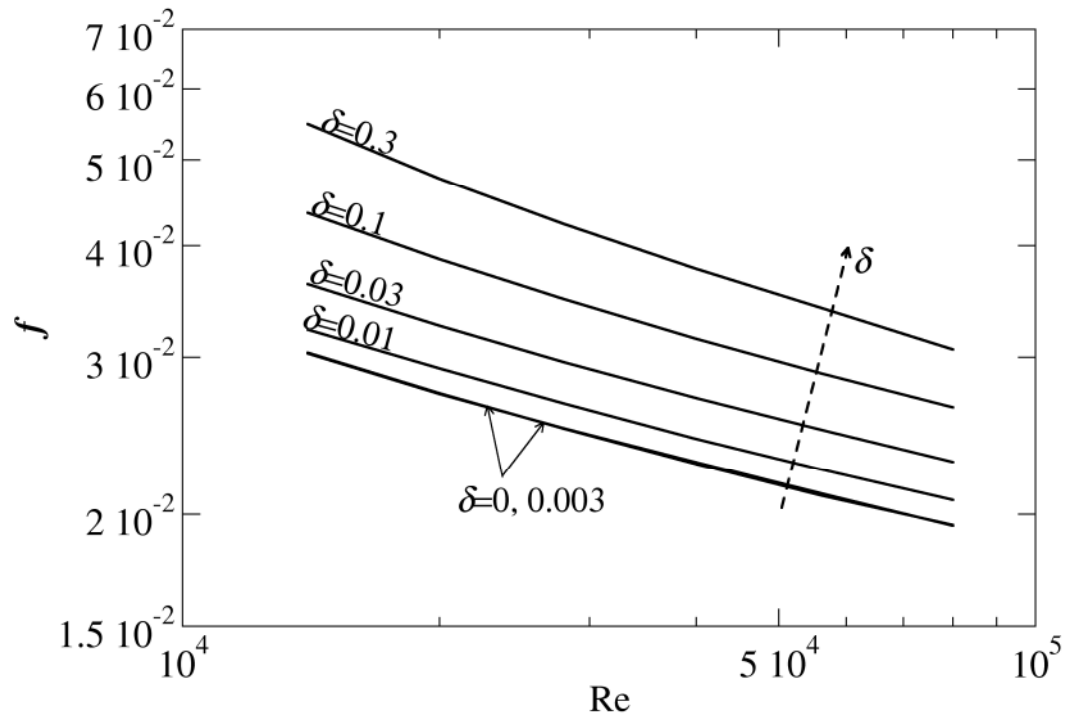
Fig. 11 Darcy-Weisbach friction coefficient as a function of the Reynolds number at different curvatures \delta for the whole the computational data set. Results for \delta=0.003 and \delta=0 (straight tube) are practically coincident.
