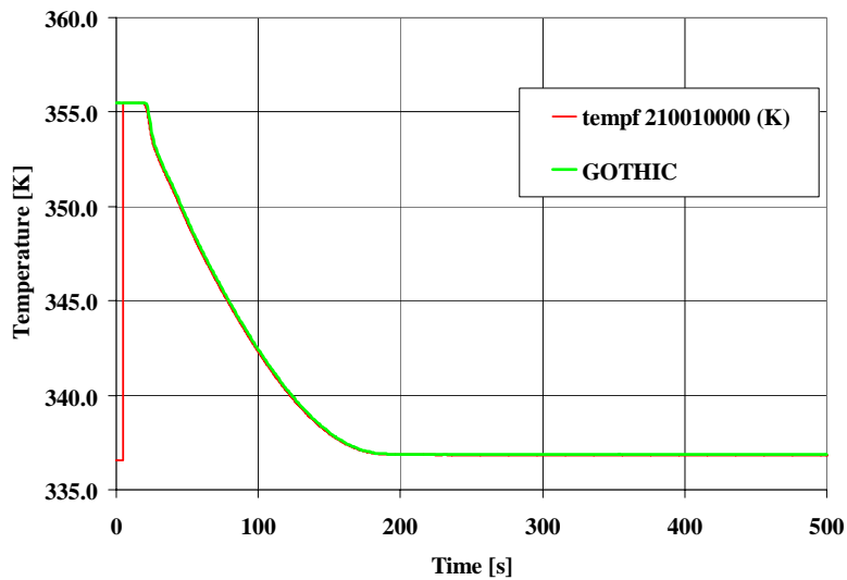
Figure 16. Sample case n. 2 – Liquid temperature
