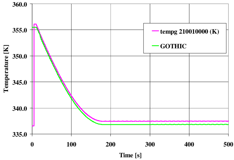
Figure 14. Sample case n. 2 – Atmosphere temperature
