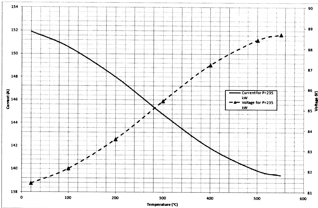
Figure 2. Required voltage / current values per FPS for delivering a constant power (235 kW).
