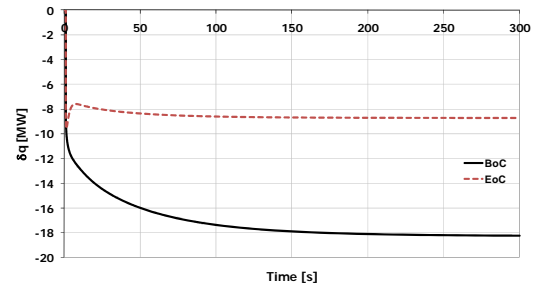
Fig. 5. Reactor power variation following an enhancement by 10 K of core inlet temperature.
