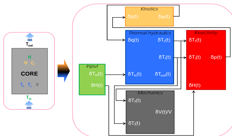
Fig. 20. DEMO core block scheme.
