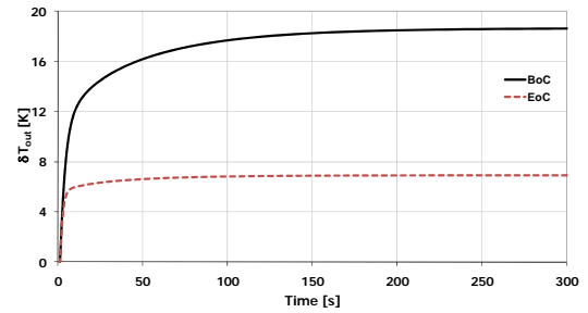
Fig. 22. Core outlet temperature variation following a step reactivity insertion of 50 pcm.
