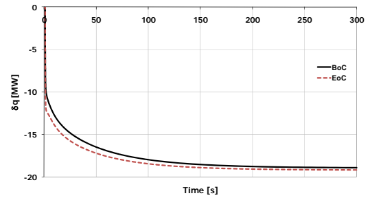
Fig. 11. Reactor power variation following an enhancement by 10 K of core inlet temperature.
