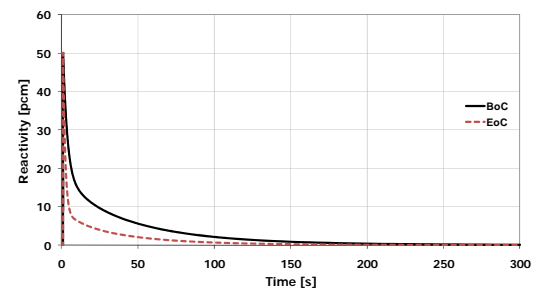
Fig. 36. Core reactivity variation following an externally given perturbation of 50 pcm.
