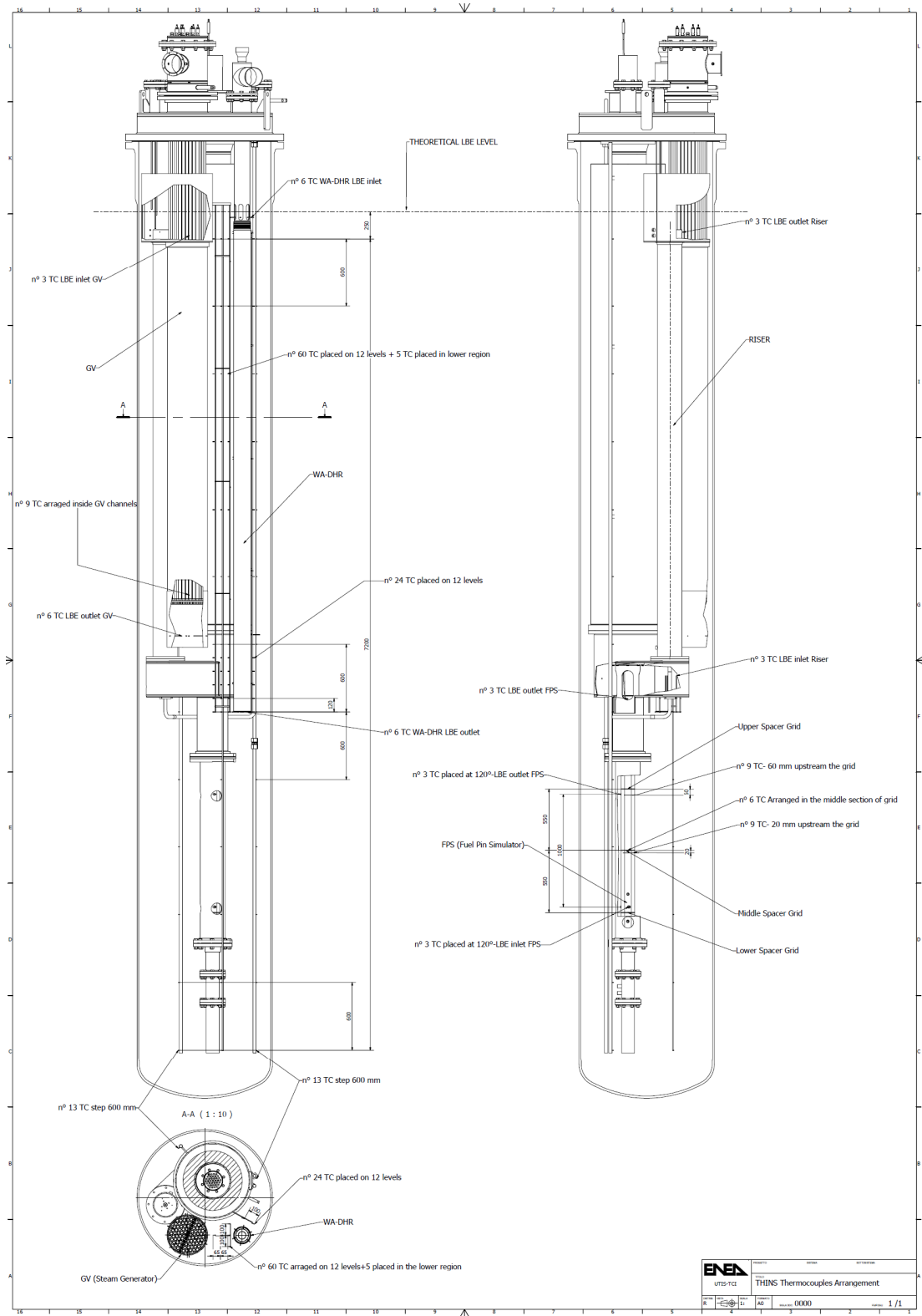
Figure 69. Sketch of the upgrade ICE test section with the installed instrumentations.
