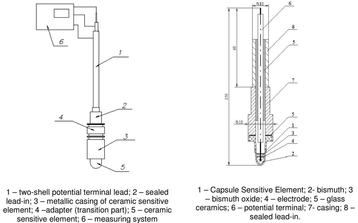
Figure 31 View of the ICE oxygen sensors
