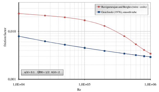
Fig. 68 – Wire coils, enhancement of the friction number.
