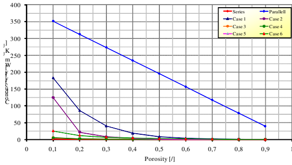
a)...overall porosities
