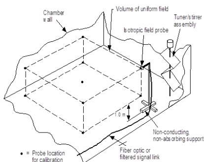
Reverberation chambers for EMC tests
