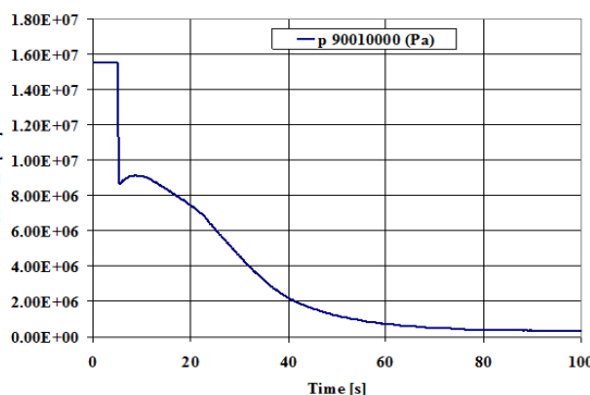
b) blowdown with gravity driven injection
